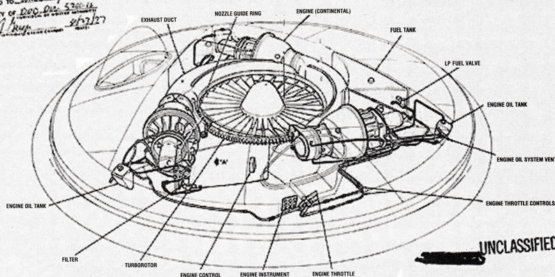
FIG. 14 POWERPLANT INSTALLATION
