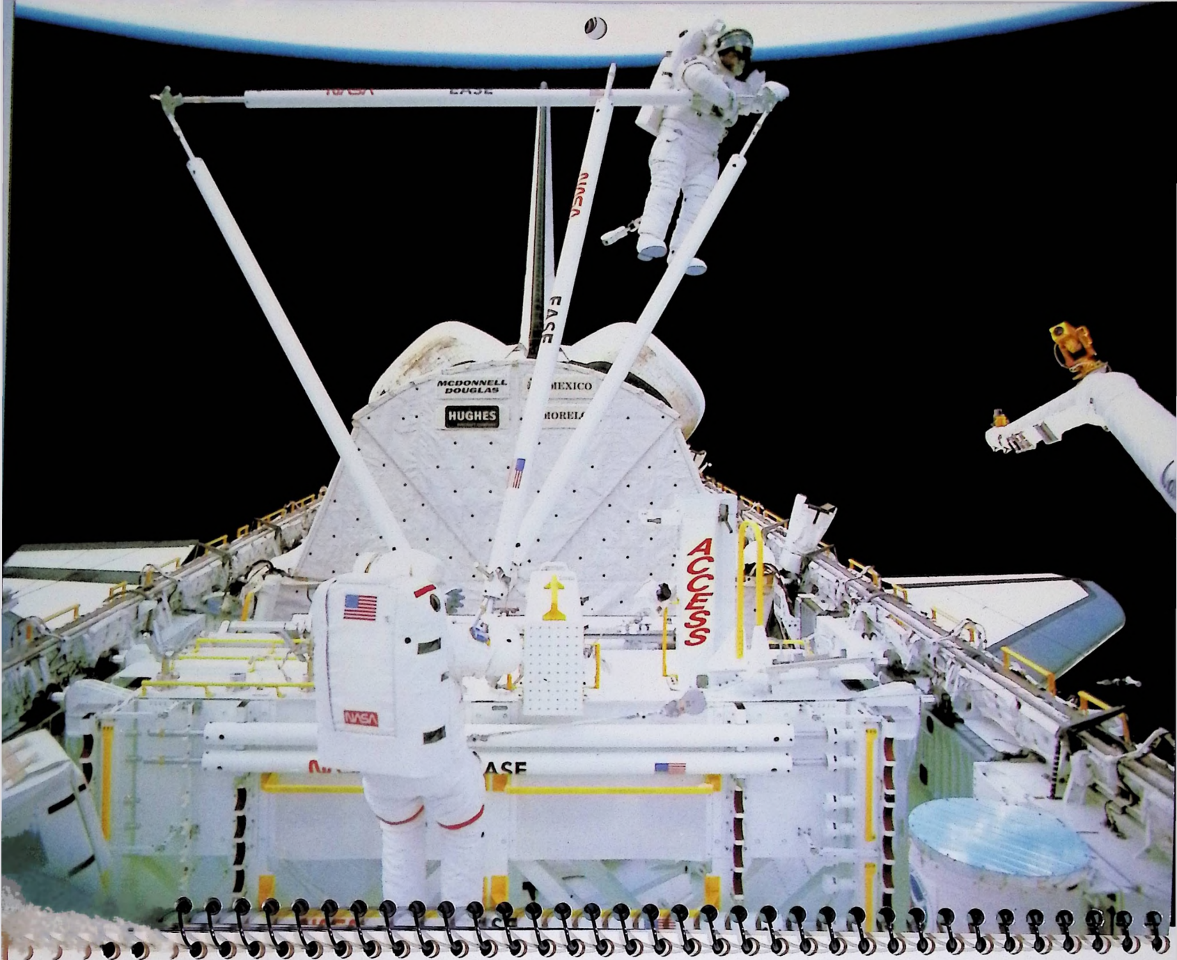
Astronauts perform EVA in shuttle's cargo bay
