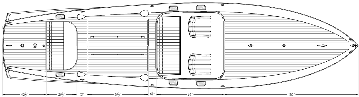
1928 29' LONG DECK RUNABOUT V2.0
