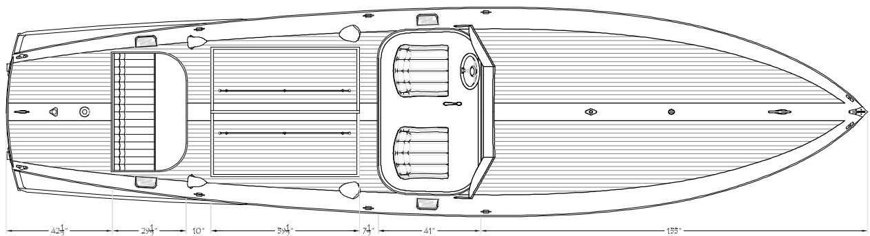
1928 29' RACING RUNABOUT DECK PLAN
