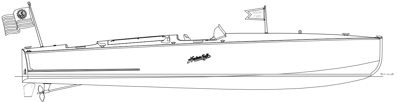
1928 29' RACING RUNABOUT OUTBOARD PROFILE
