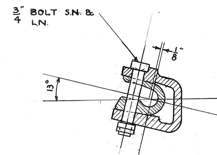
SECTION "A-A" SHOWING BRAKE HANGER SUSPENSION ARRANGEMENT SCHAEFFER TYPE-W-I.
