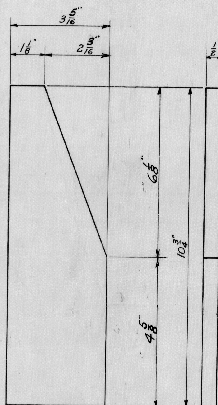
STRIKER SIDE SUPPORT - REAR 6 \frac{1}{4} \times \frac{1}{2} \times 0 - 10 \frac{3}{8} (1 CUTS 2)
