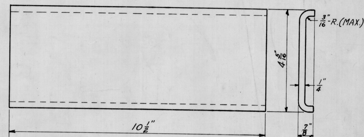
COUPLER WEAR PLATE 10 \frac{1}{2} \times \frac{1}{4} \times 0 - 6
