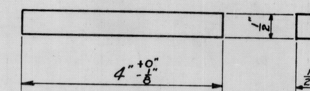
CARRIER IRON STOP \frac{1}{2} \times \frac{1}{2} \times 0 - 4
