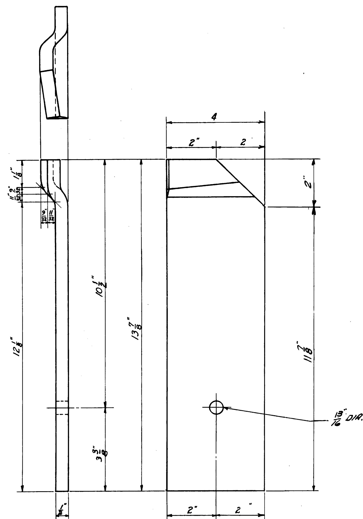
STRIKER SIDE SUPPORT - FRONT
