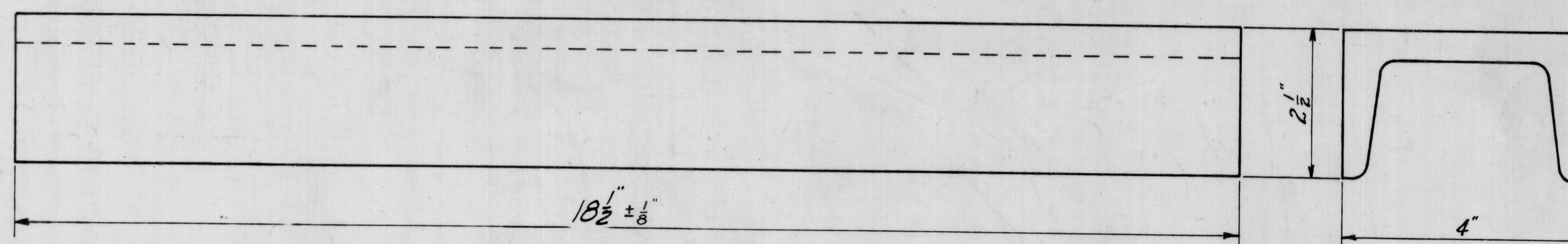
COUPLER CARRIER 4 \times 13.8 \times 1 - 6 \frac{1}{2} L
