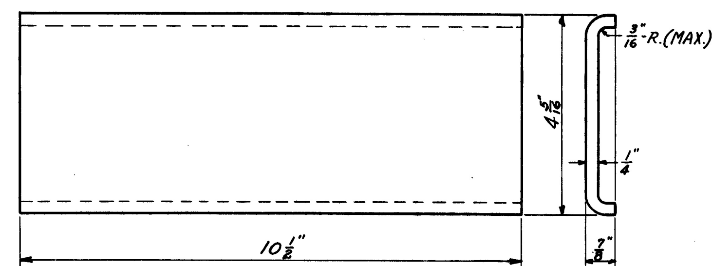
COUPLER WEAR PLATE
