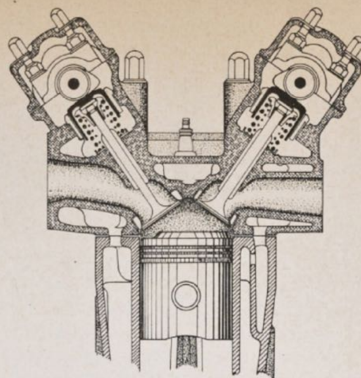
DRAWING BY ROBERT N. HOEPPNER CUTAWAY of the combustion chamber
