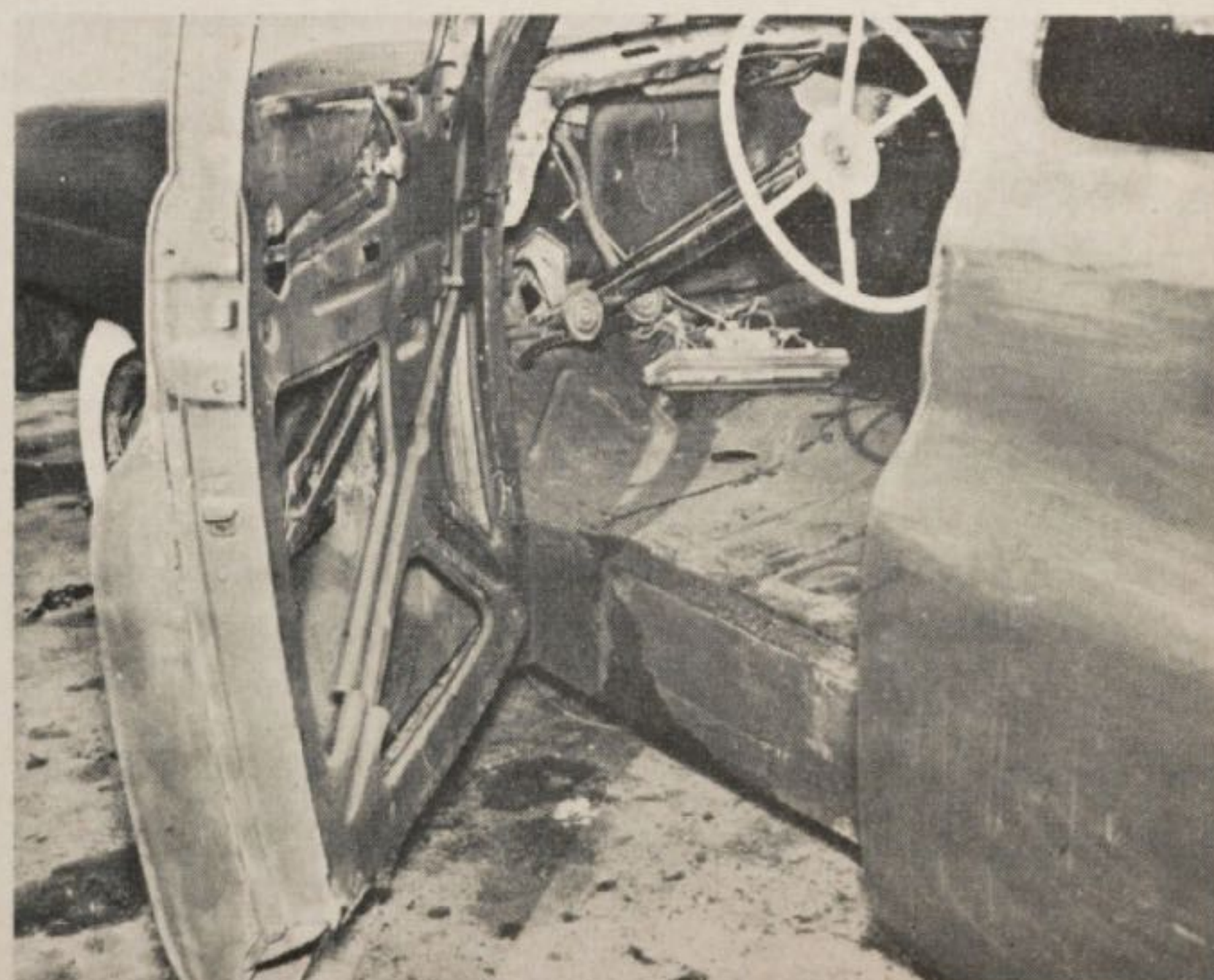
LOWERING of Ayala '40 Ford coupe is aided by extreme (eight-inch) channeling. Steering column has been shortened
