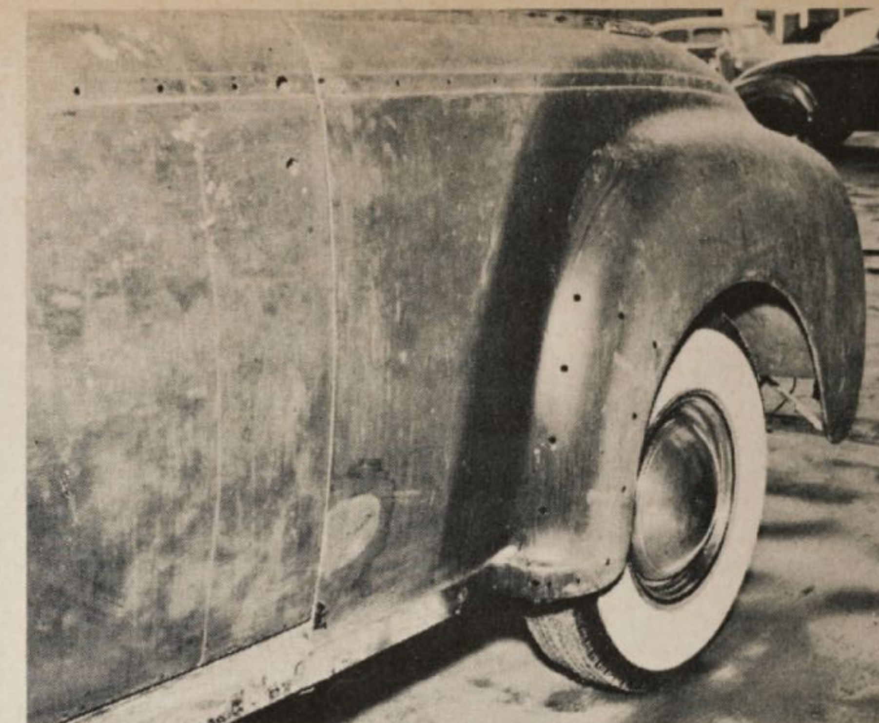
PHOTOGRAPHS BY THOMAS J. MEDLEY BODY and fender of late-model Dodge has been prepared for filling and sealing. All chrome strips have been removed
