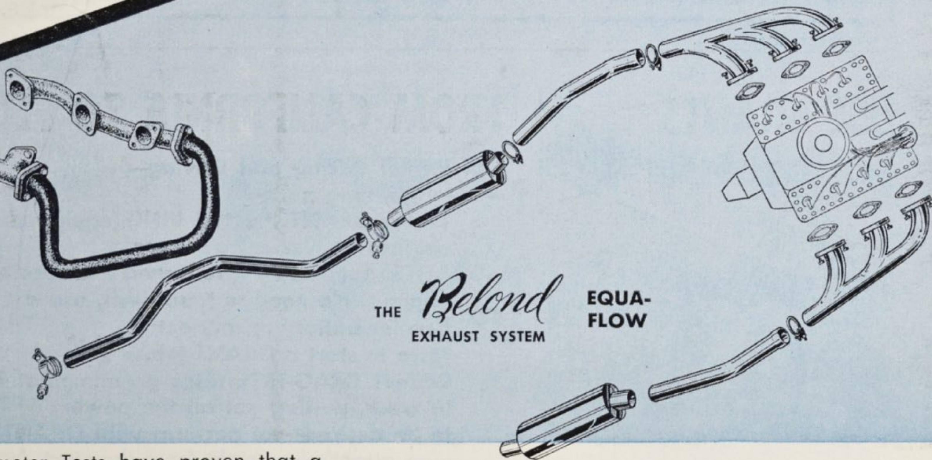
TYPICAL STANDARD FORD OR MERCURY EXHAUST SYSTEM
