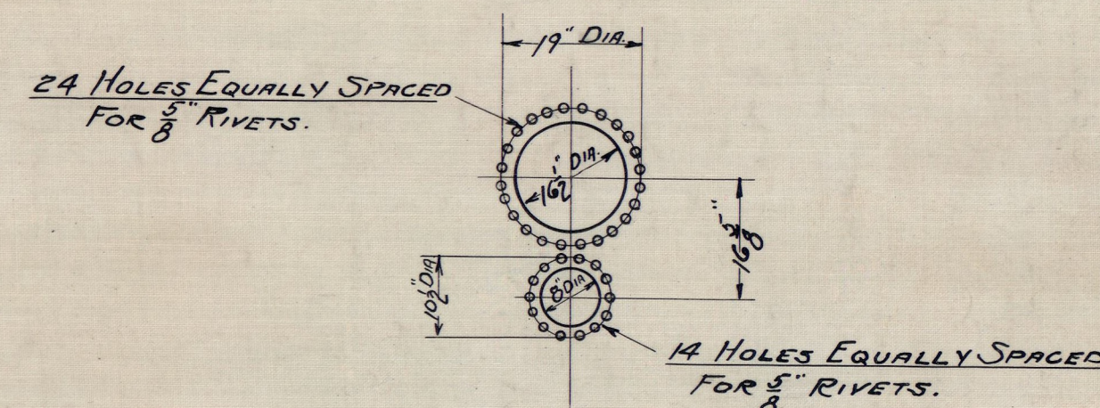
DETAIL OF MANHOLE AND SAFETY VALVE RIVET CIRCLE
