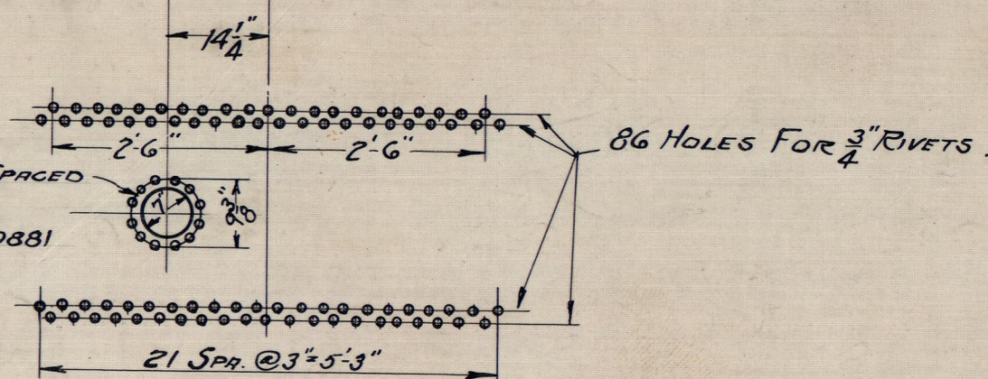
DETAIL OF ANCHOR & OUTLET HOLES.
