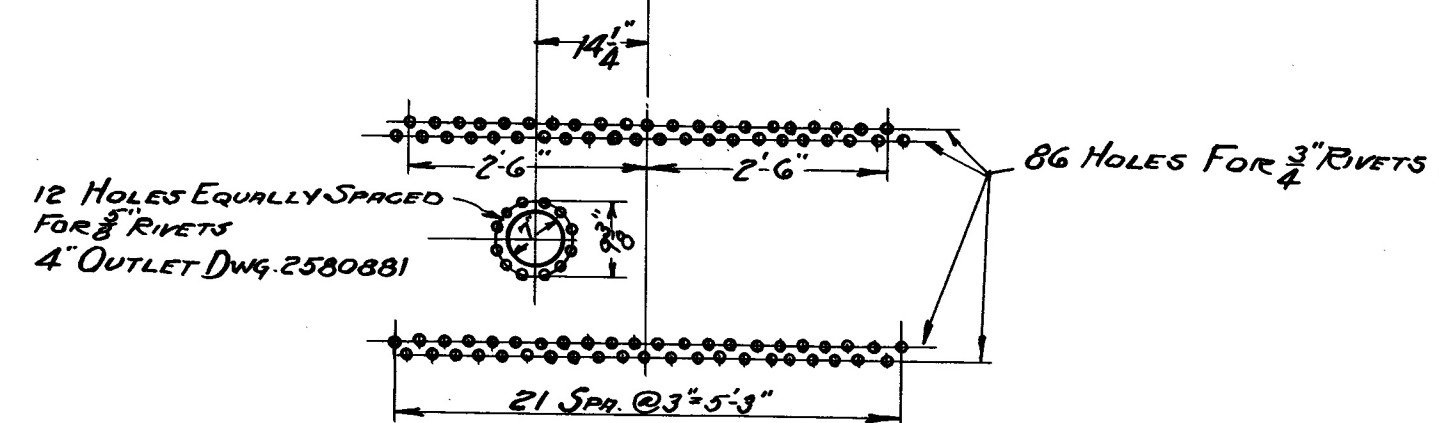
DETAIL OF ANCHOR & OUTLET HOLES.
