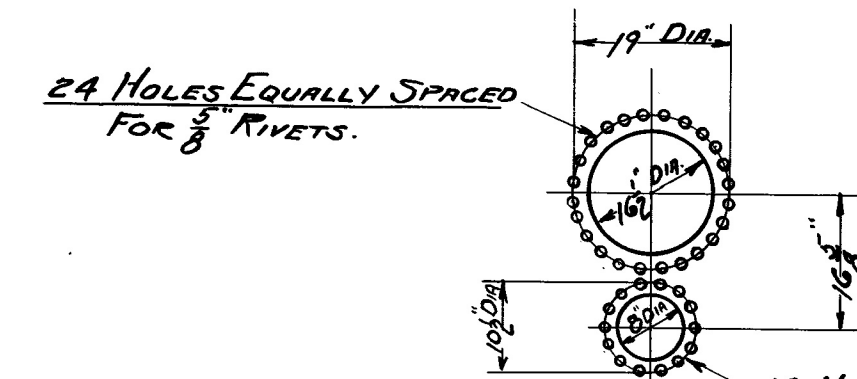
DETAIL OF MANHOLE AND SAFETY VALVE RIVET CIRCLE
