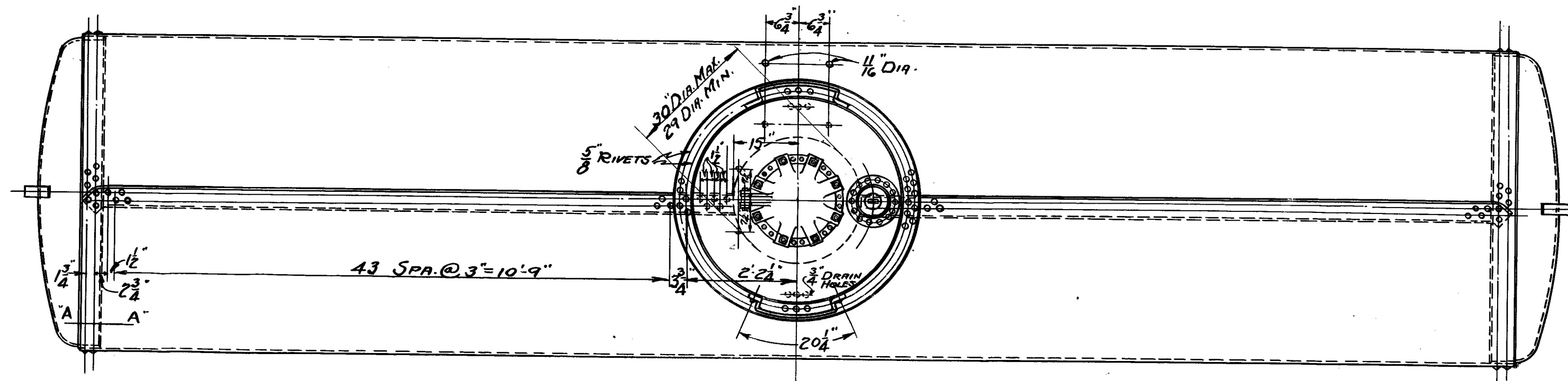
DOME RING 3142010 DOME COVER 3142009
