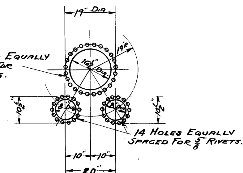
DETAIL OF MANHOLE AND SAFETY VALVE RIVET CIRCLES.
