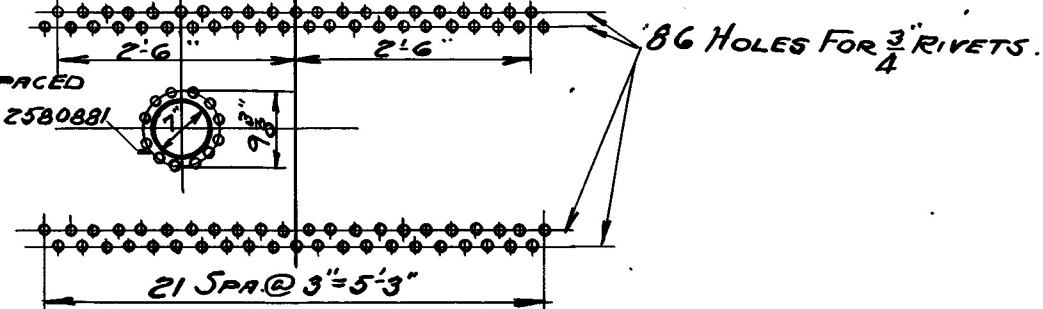
DETAIL OF ANCHOR & OUTLET HOLES.
