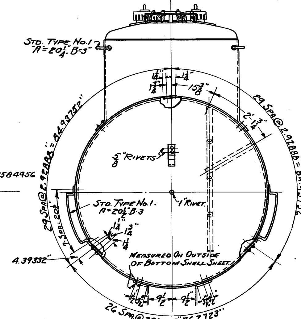
DETAIL OF MANHOLE AND SAFETY VALVE RIVET CIRCLES.
