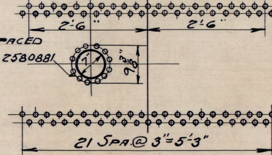
DETAIL OF ANCHOR & OUTLET HOLES.
