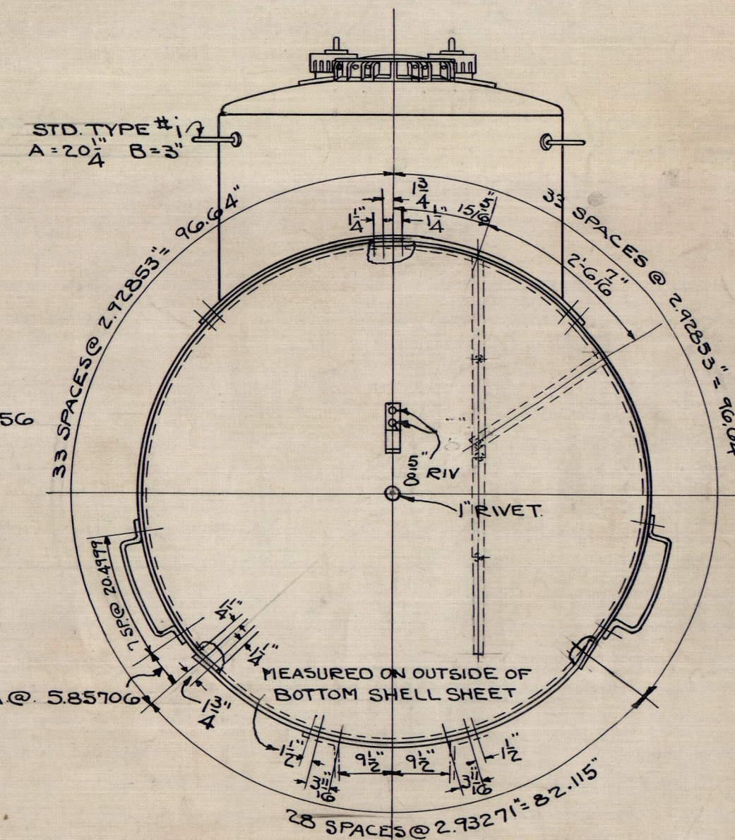
DETAIL OF MANHOLE AND SAFETY VALVE RIVET CIRCLES
