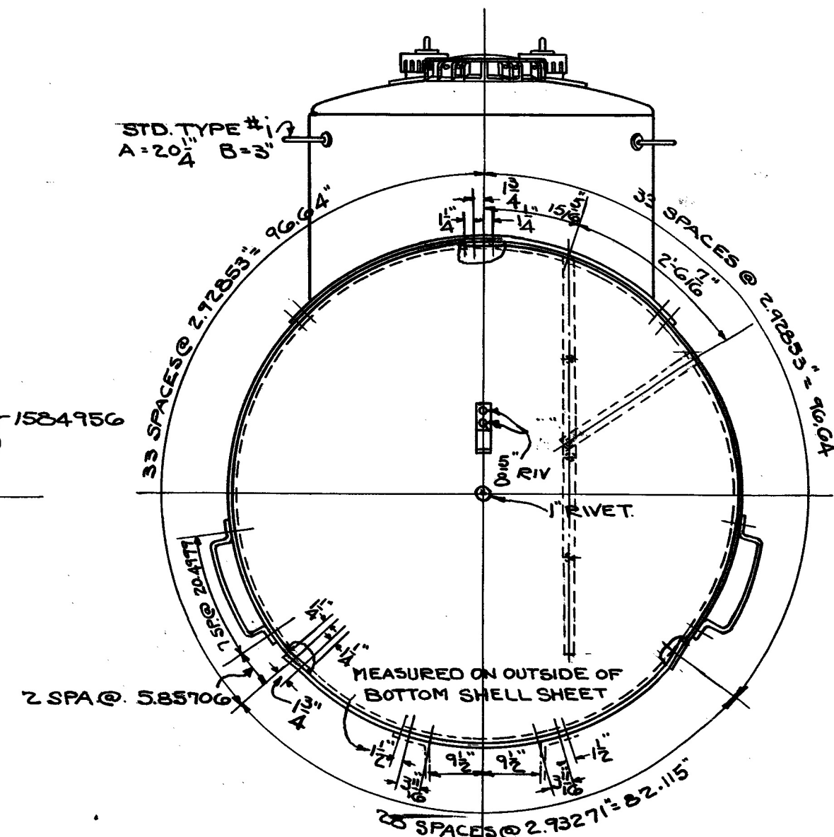
DETAIL OF MANHOLE AND SAFETY VALVE RIVET CIRCLES
