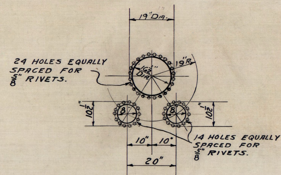
DETAIL OF MANHOLE AND SAFETY VALVE RIVET CIRCLES
