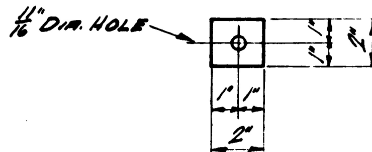
END SHEET & SIDE SILL FILLER 2" x 10" x 0" L x 0" T (O.H.S.) 4 - PER CAR
