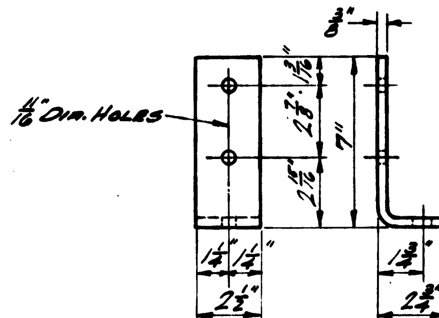
DOOR POST & SIDE SILL CONN. 2 1/2" x 2 1/2" x 0" L x 0" T (O.H.S.) 4 - PER CAR
