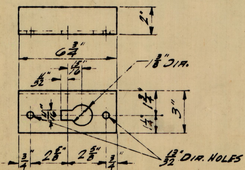
SIDE GRAB REINFORCEMENT 3" x 2" x 3/16" L x 0'-6 3/4" (O.H.S.) 4 - PER CAR
