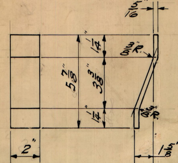
SIDE POST & SIDE PLT. CONN. 2" x 5 1/2" x 0'-6 1/4" (O.H.S.) 16 - PER CAR
