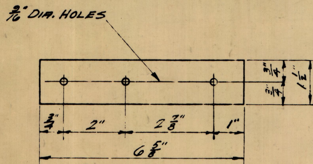
FILLER-TOP OF DOOR POST 1 1/2" x 0.076" x 0'-6 5/8" (1-CUTS 44) 4 - PER CAR
