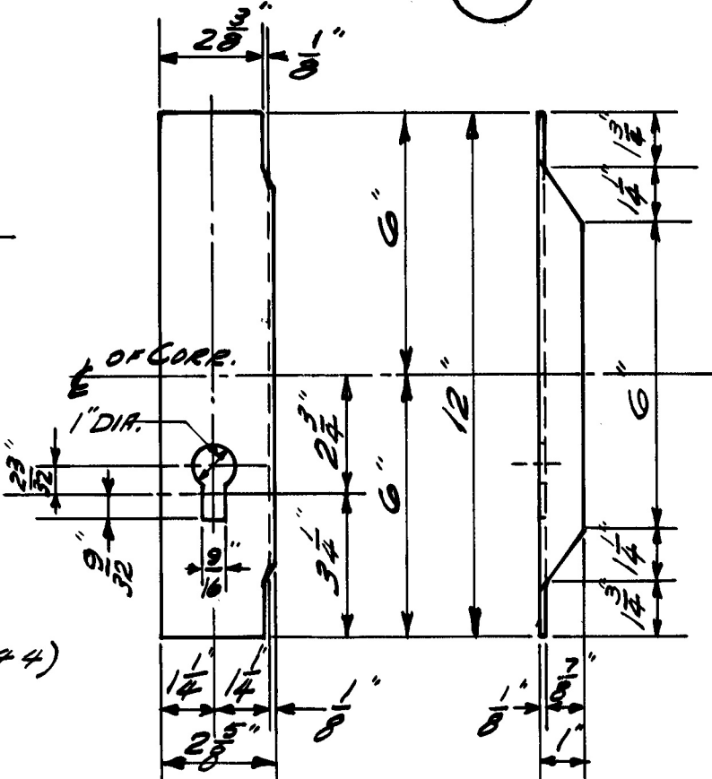
BOLTING CLIP @ INTERMEDIATE TOP 12" x 1/4" x 0" L x 0" T (O.H.S.) 8 - PER CAR
