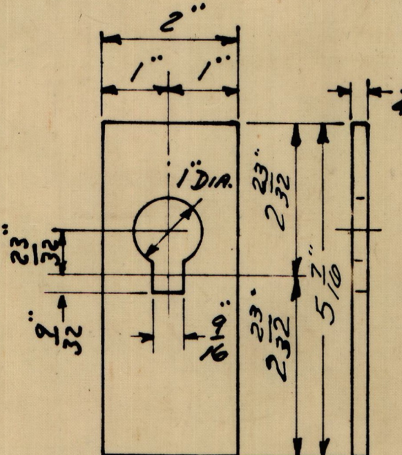
BOLTING CLIP @ STEEL END-INTER. 2" x 1/4" x 0'-5 3/16" (1-CUTS 44) 12 - PER CAR
