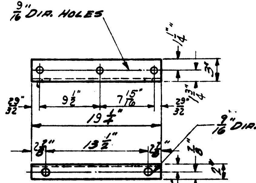
END RUNNING BOARD SUPPT. 3" x 2" x 1/8" L x 1" T (O.H.S.) 2 - PER CAR
