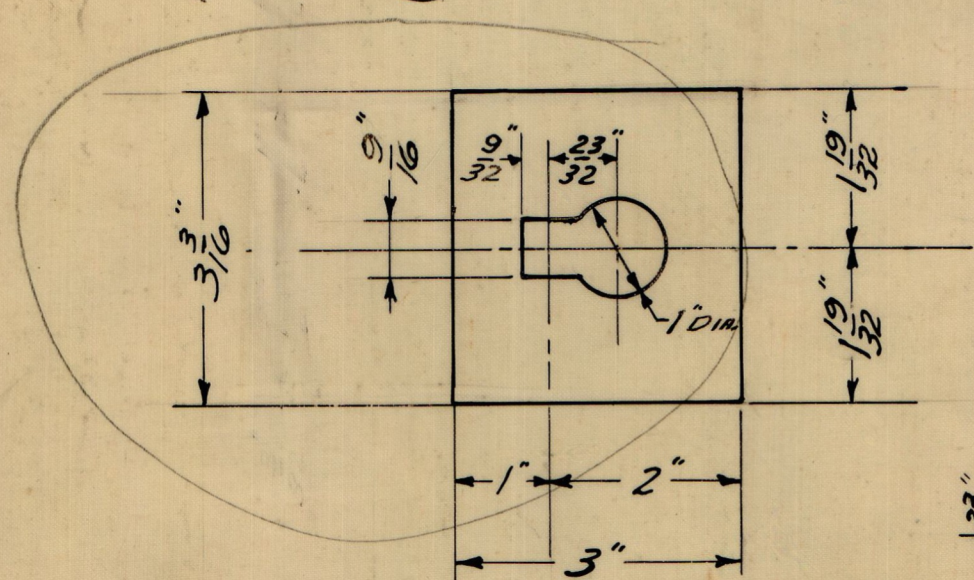
BOLTING CLIP @ STEEL END 3" x 1/4" x 12'-2 1/2" (1-CUTS 44) 12 - PER CAR
