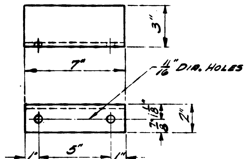
THRESHOLD FILLER SUPPT. 3" x 2" x 1/8" L x 0" T (L.R.H.T.) 4 - PER CAR
