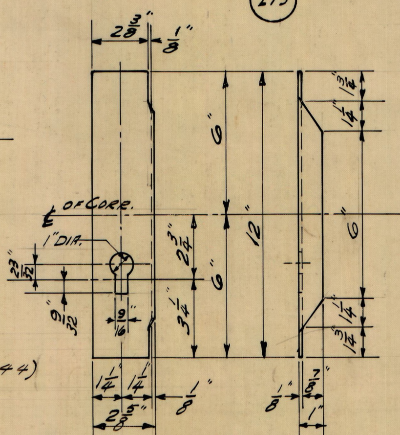
BOLTING CLIP @ INTERMEDIATE TOP 12" x 1/4" x 0'-3 1/2" (1-CUTS 44) 8 - PER CAR
