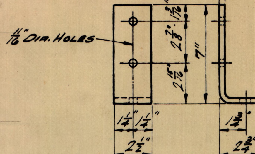
DOOR POST & SIDE SILL CONN. 2 1/2" x 2 1/2" x 0'-9 1/4" (O.H.S.) 4 - PER CAR
