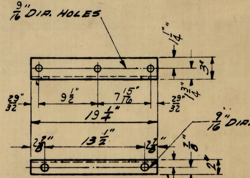
END RUNNING BOARD SUPPT. 3" x 2" x 3/16" L x 1'-7 1/4" (O.H.S.) 2 - PER CAR
