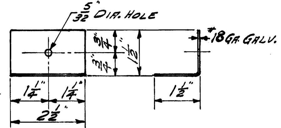
BULKHEAD SIDE SUPPORT PROTECTION ANGLE 2 1/2" x 1/4" x 0" L x 0" T (O.H.S.) 4 - PER CAR (HOT DIPPED GALVANIZED)
