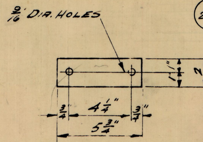
FILLER-TOP INTER. POST 2" x 0.076" x 0'-5 3/4" (1-CUTS 44) 4 - PER CAR
