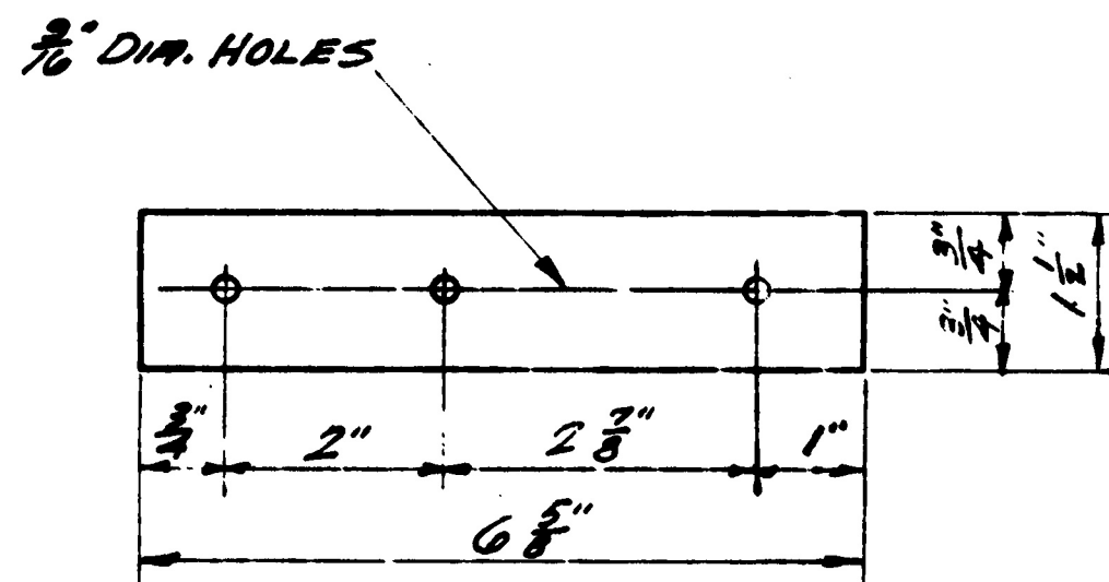
FILLER-TOP OF DOOR POST 1 1/2" x 0" L x 0" T (O.H.S.) 4 - PER CAR
