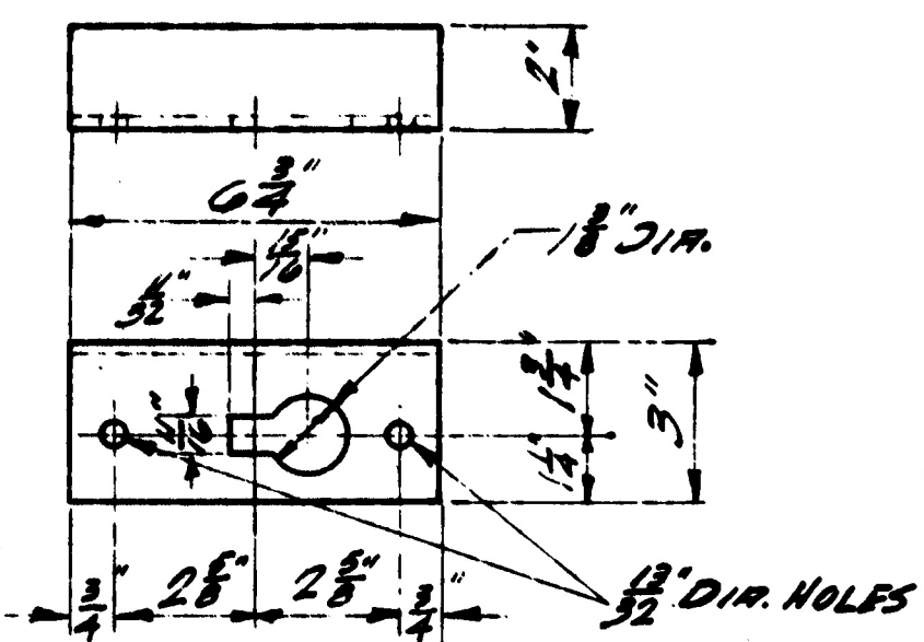
SIDE GRAB REINFORCEMENT 3" x 2" x 1/8" L x 0" T (O.H.S.) 4 - PER CAR
