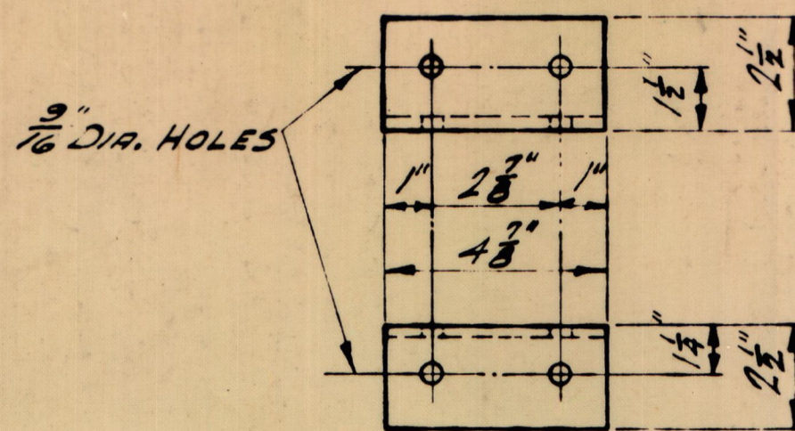
DOOR POST & SIDE SILL CONN. 2 1/2" x 2 1/2" x 1/4" L x 0'-4 1/2" (O.H.S.) 4 - PER CAR
