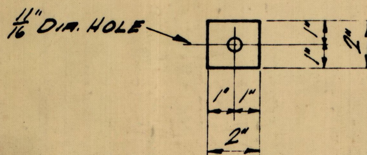
END SHEET & SIDE SILL FILLER 2" x 10" x 0'-2" (O.H.S.) 4 - PER CAR
