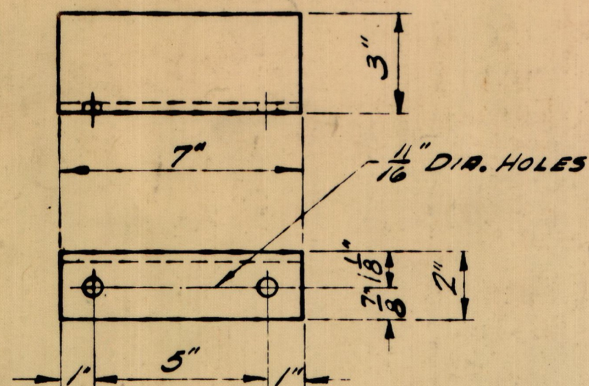
THRESHOLD FILLER SUPPT. 3" x 2" x 1/16" L x 0'-7" (L.R.H.T.) 4 - PER CAR
