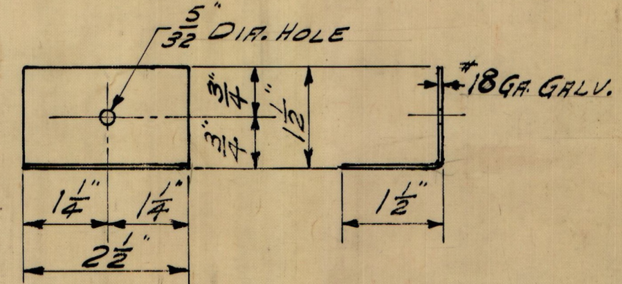
BULKHEAD SIDE SUPPORT PROTECTION ANGLE 2 1/2" x 1/4" x 0'-3" (1-CUTS 44) 4 - PER CAR (HOT DIPPED GALVANIZED)
