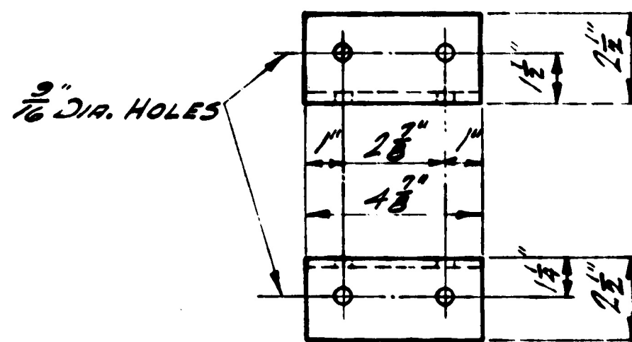
DOOR POST & SIDE SILL CONN. 2 1/2" x 2 1/2" x 1/4" L x 0" T (O.H.S.) 4 - PER CAR
