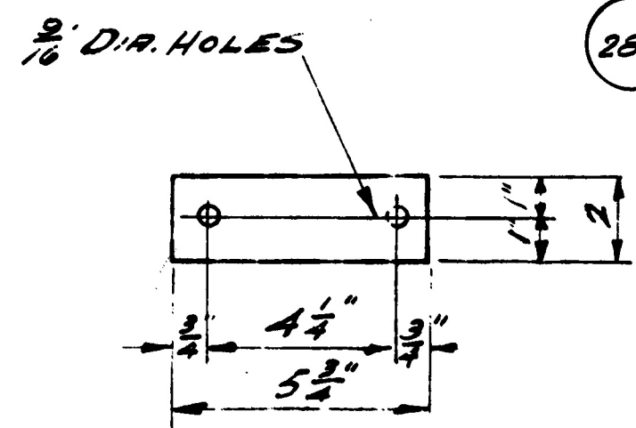
FILLER-TOP INTER. POST 2" x 0" L x 0" T (O.H.S.) 4 - PER CAR
