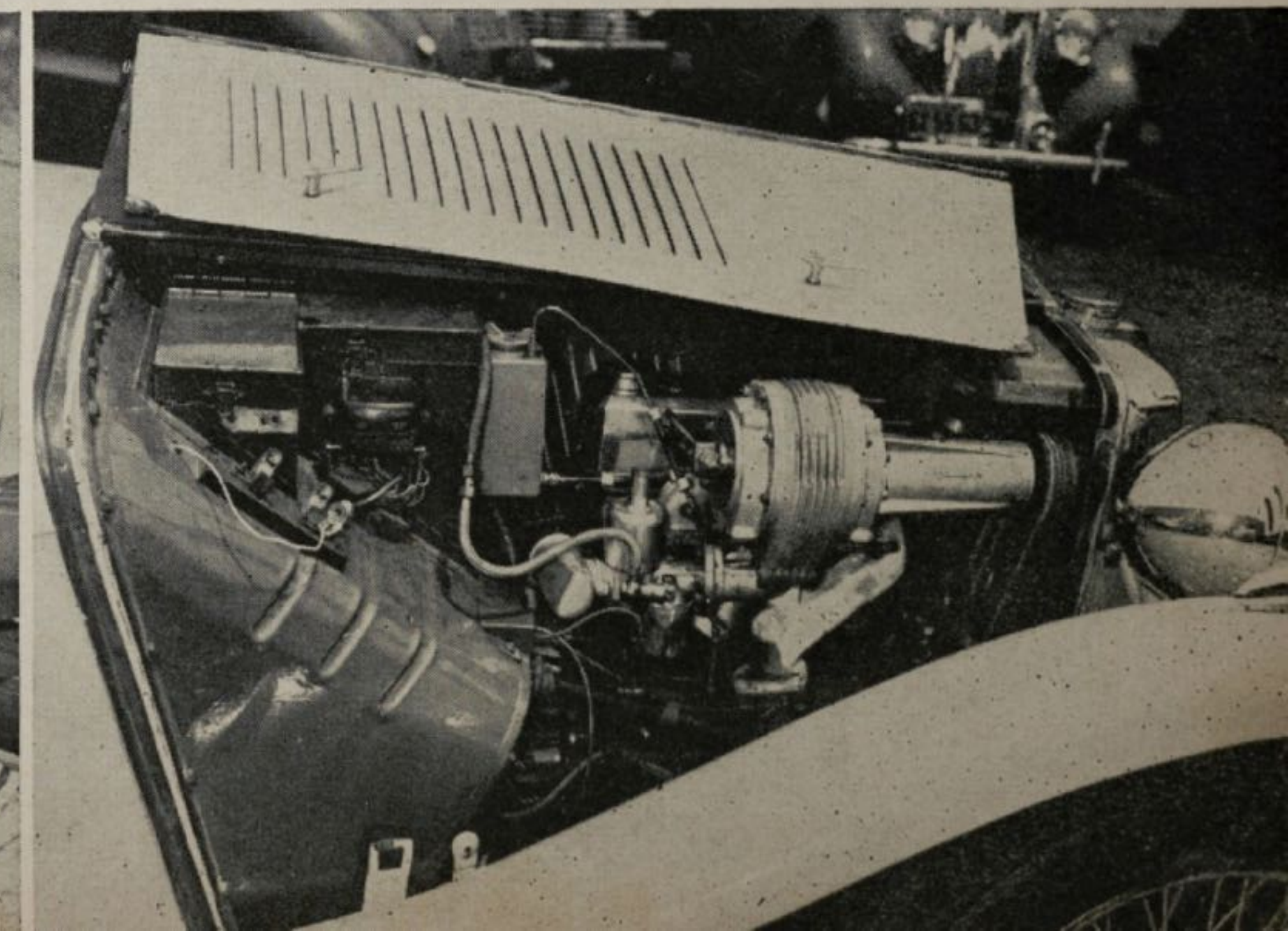
BLOWN —A Shorrock supercharger is shown installed on the engine of this MG. The use of a blower increases the top speed by about 15 mph and greatly increases acceleration.
