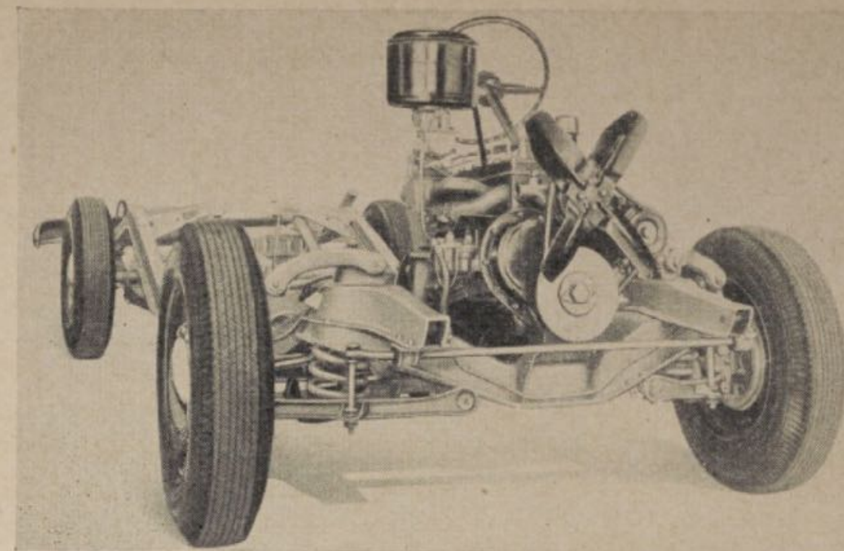
CHASSIS of the Champion shows new suspension system.
