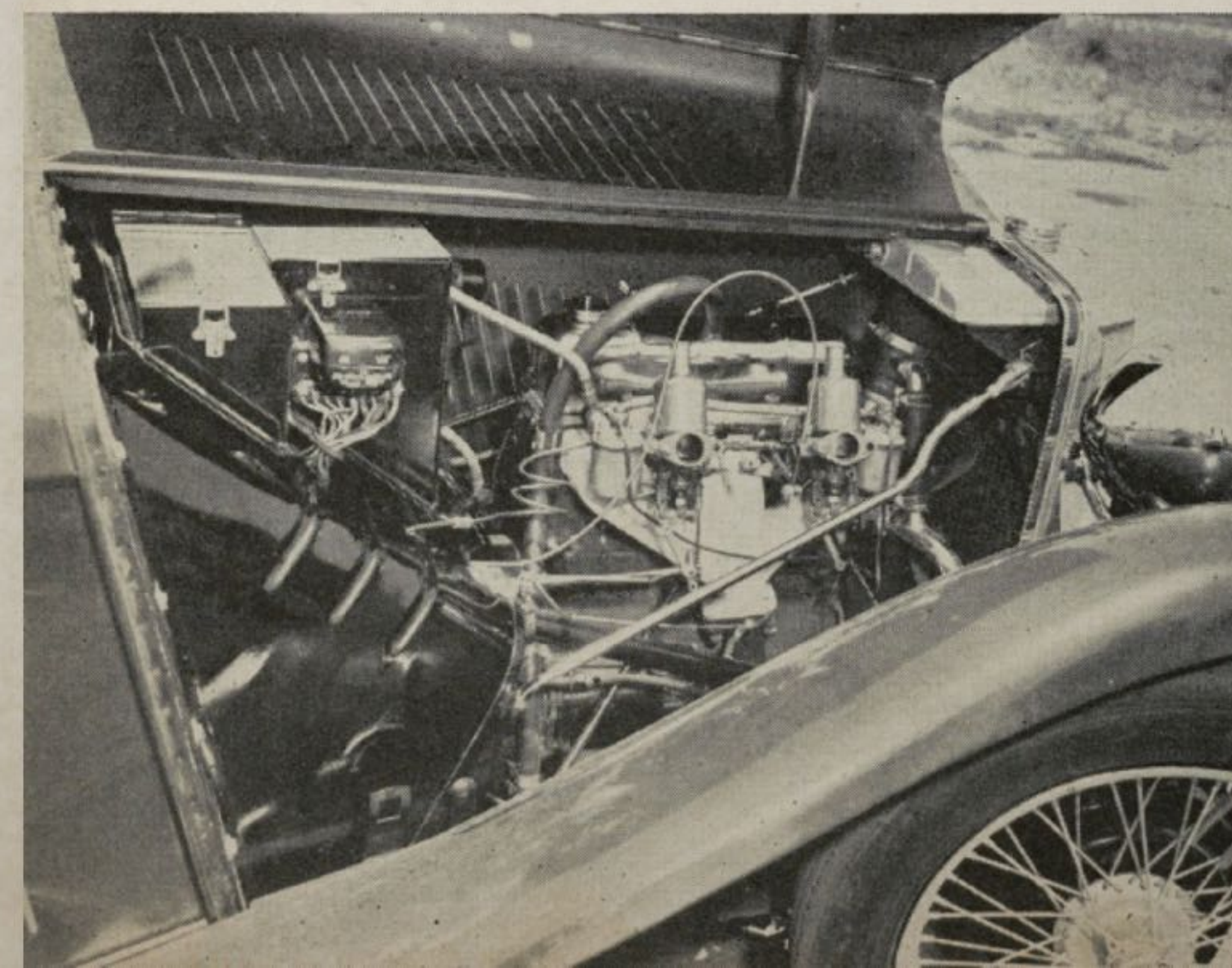
UNBLOWN —The compact engine of the unblown MG is shown here. Note the dual downdraft carburetors, and the toolboxes mounted on the firewall. Engine is a four-cylinder in-line.
