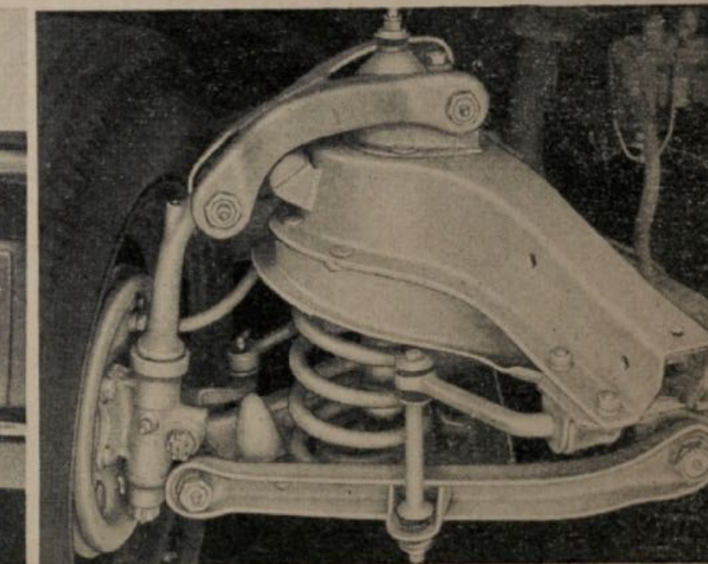
CLOSEUP of new front end suspension.
