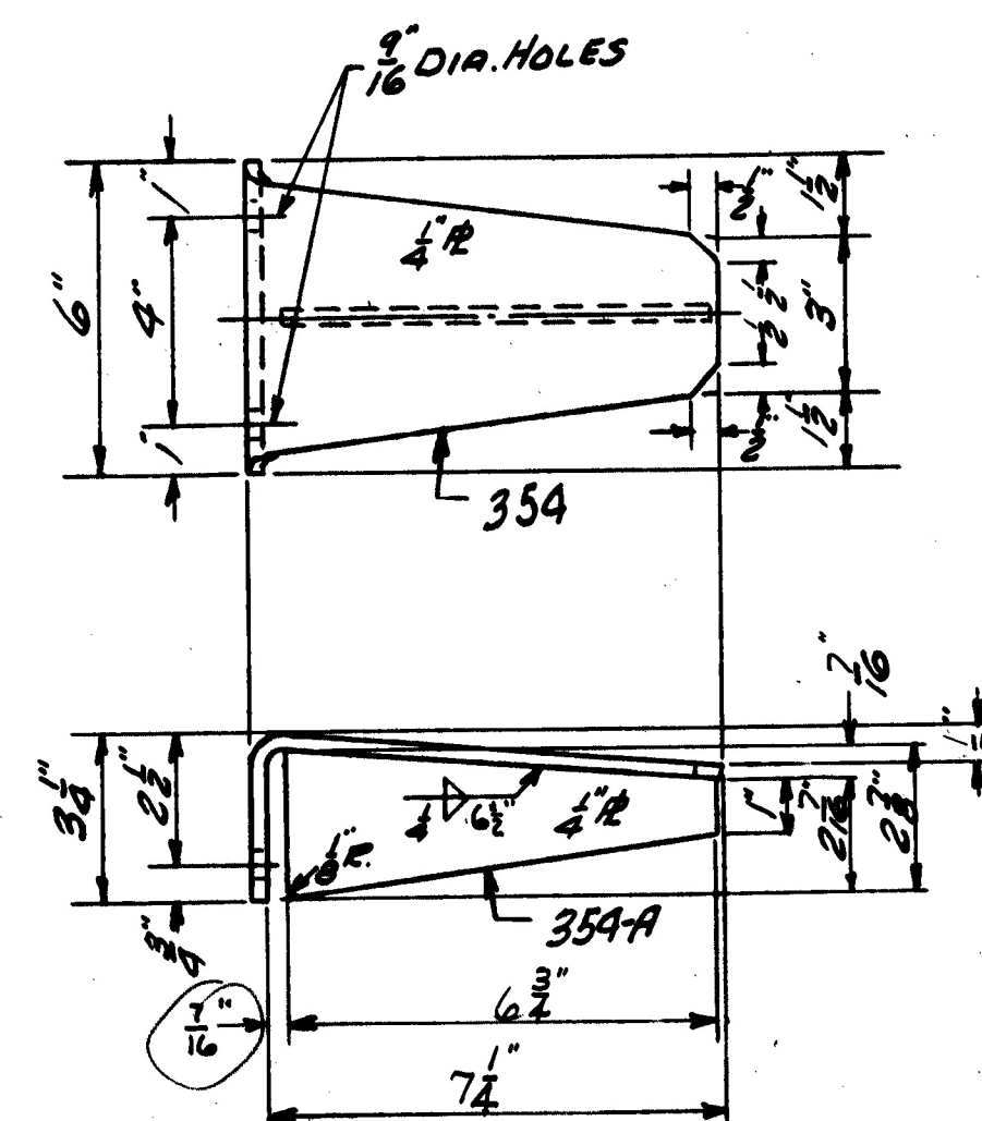
HATCH COVER STOP 10 3/8" x 1/4" x 8 5/8" (1-CUTS 22) (354) 8 PER CAR HATCH COVER STOP BRACE 6 3/4" x 1/4" x 1'-4 1/4" (1-CUTS 8) (354 A) 8 PER CAR
