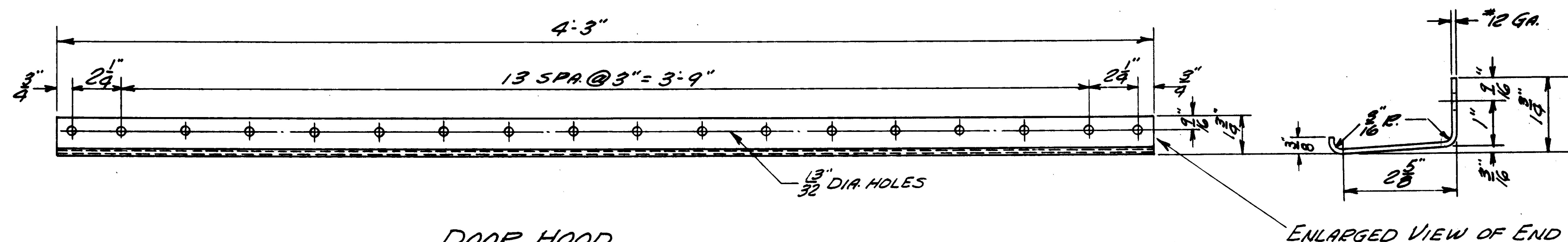
DOOR HOOD 4" x #12 GA x 4'-3" (C.B.S.) (351) 2 PER CAR
