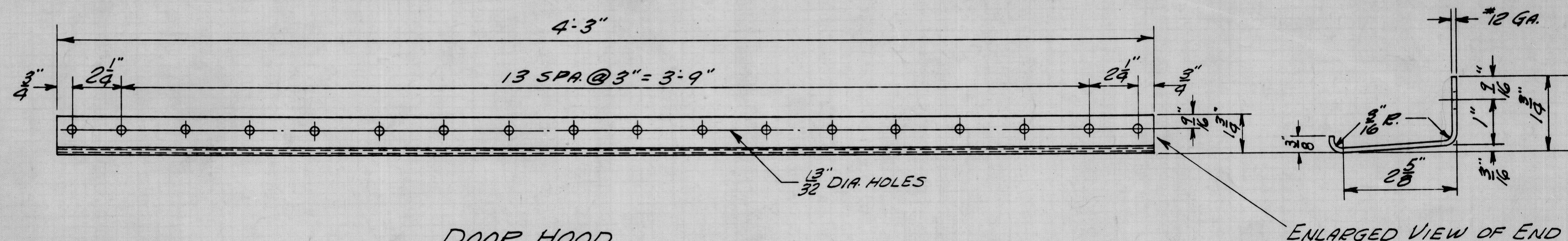
DOOR HOOD 4 7/8" x #12 GA x 4'-3" (C.B.S.) (351) 2-PER CAR
