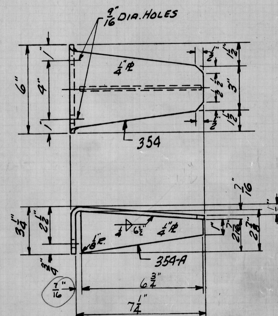
HATCH COVER STOP 10 3/8" x 1/4" x 8-5 1/2" (1-CUTS 22) (354) 8-PER CAR
