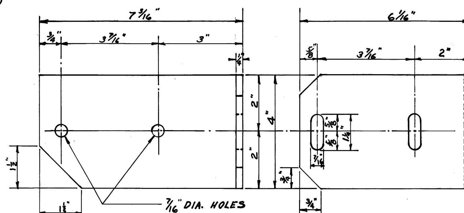
RETAINER VALVE BRACKET 4" x 1/4" x 1'-1" O.H.S. (355) 1 PER CAR
