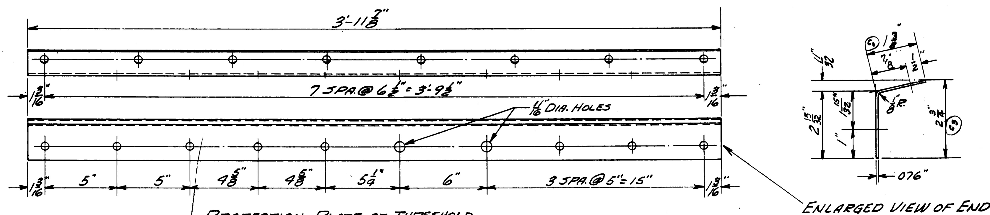
PROTECTION PLATE AT THRESHOLD 4 1/2" x .076 x 3'-11 7/8" (L.A.H.T.) (352) 2 PER CAR
