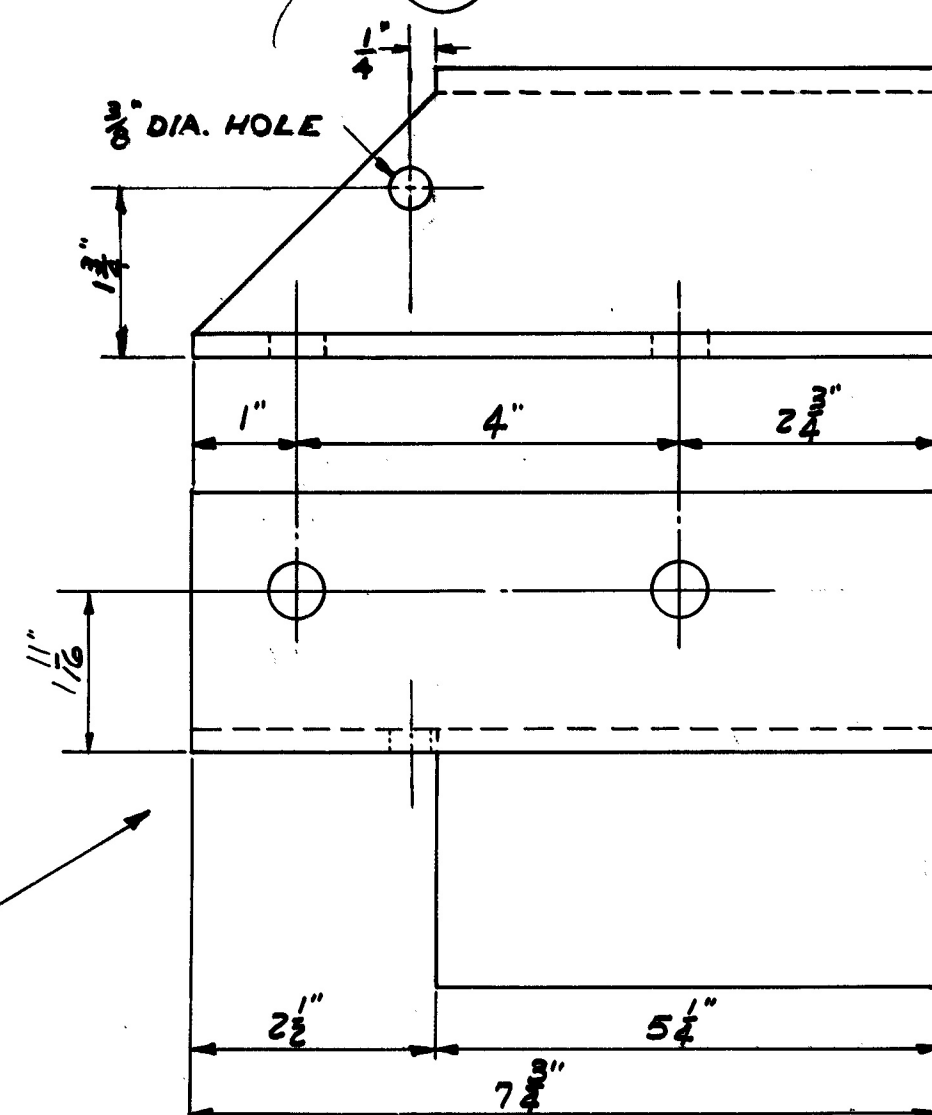
PROTECTION PLATE AT THRESHOLD 4 1/2" x .076 x 3'-11 7/8" (L.A.H.T.) (352) 2 PER CAR
