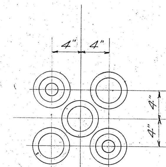
SPRING GROUP 5 OUTER COIL SPRINGS 2 INNER COIL SPRINGS
