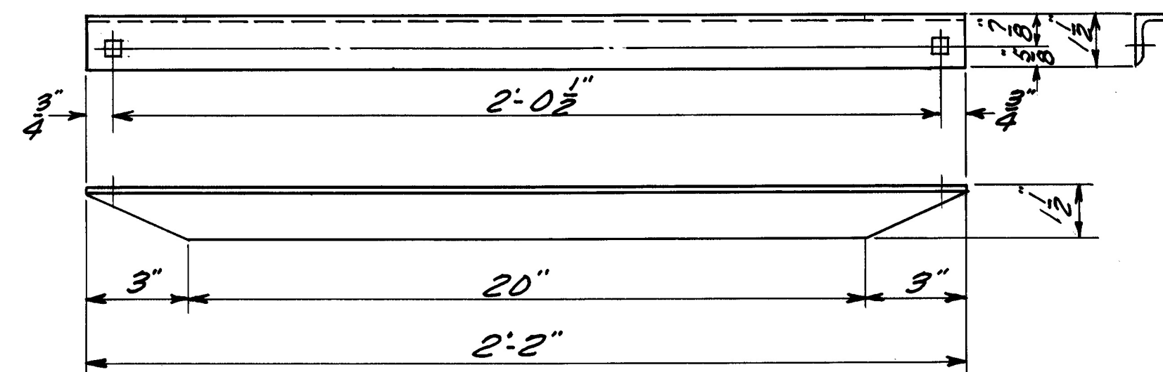
HATCH COVER STIFF. ANGLE 1 1/2" x 1 1/2" x 3/16" x 2'-2" (O.H.S.) 335 4- PER CAR
