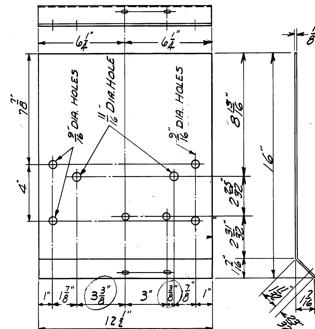
HATCH COVER BACKING 12 1/2" x 8" x 1 1/8" (O.H.S.) 334 4- PER CAR 2- AS SHOWN 2- REVERSE 334 A
