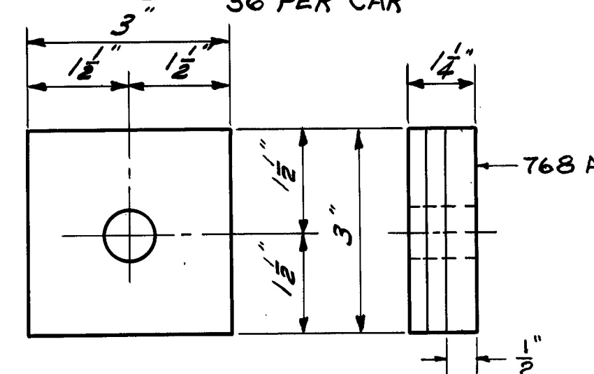
STEEL END WOOD FILLER
