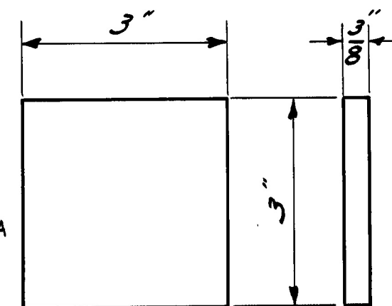
ROOF INSULATION CLEAT 3" x 3/8" x 0'-3" 762-60-PER CAR
