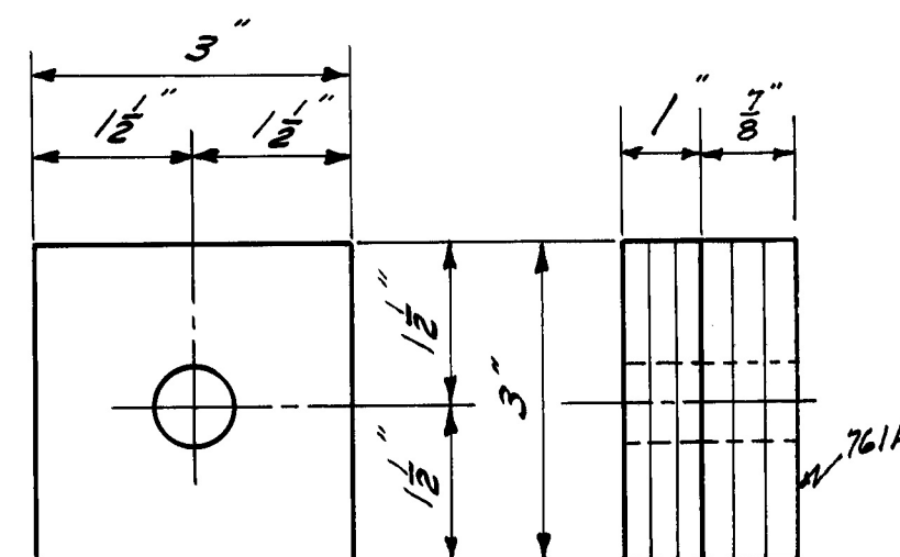
ENDS-TOP 3" x 1" x 0'-3" 761-8-PER CAR
