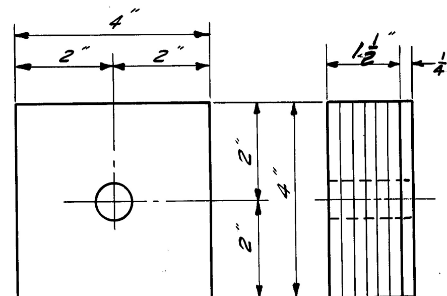
SIDE AT BELT RAILS
