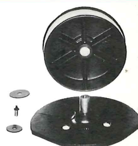
8. Larger corner rollers on adjustable mounting base. 14" corner idler reduces chain wear. Equipped with replaceable bronze oilite bearings and grease fitting. Shafts in corner base are easily replaced if necessary.
