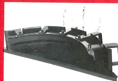
4. Heavy steel reverse curve is equipped with 5 wrap around steel cement locks and large steel wear surface on gutter bottom. Adjustable heavy steel angle iron chain guide with added wear strip assures smooth chain movement.
