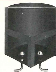
7. Reuseable inside corner form serves as simple guide in anchor bolt placement and neat simple pattern for concrete work.
