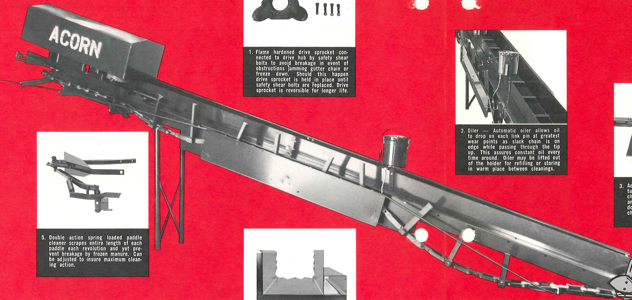
6. Heavy gauge elevators are 12" deep seamless steel sections eliminating leaks and needless corrosive damage in seams. Greater strength is added by use of full length formed steel elevator beam plus additional insert at outer end of beam for added transmission support.
