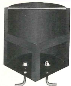
7. Reuseable inside corner form serves as simple guide in anchor bolt placement and neat simple pattern for concrete work.
