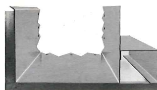
6. Heavy gauge elevators are 12" deep seamless steel sections eliminating leaks and needless corrosive damage in seams. Greater strength is added by use of full length formed steel elevator beam plus additional insert at outer end of beam for added transmission support.
