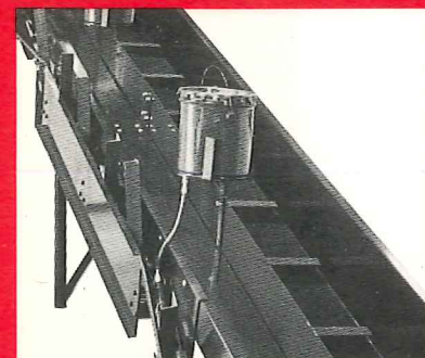
2. Oiler — Automatic oiler allows oil to drop on each link pin at greatest wear points as slack chain is on edge while passing through the tip up. This assures constant oil every time around. Oiler may be lifted out of the holder for refilling or storing in warm place between cleanings.
