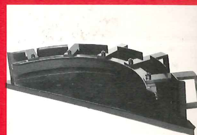
4. Heavy steel reverse curve is equipped with 5 wrap around steel cement locks and large steel wear surface on gutter bottom. Adjustable heavy steel angle iron chain guide with added wear strip assures smooth chain movement.
