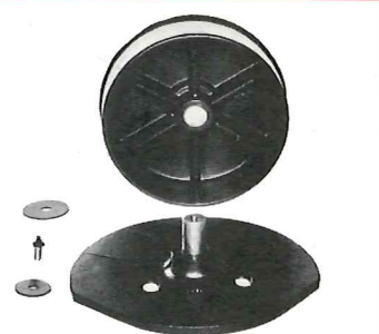
8. Larger corner rollers on adjustable mounting base. 14" corner idler reduces chain wear. Equipped with replaceable bronze oilite bearings and grease fitting. Shafts in corner base are easily replaced if necessary.
