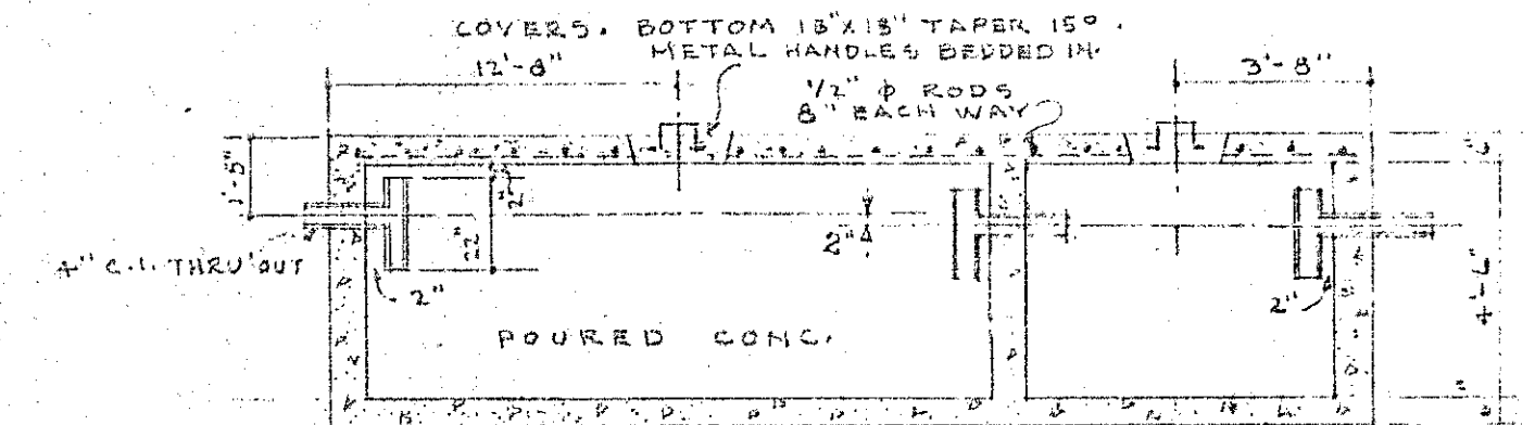
SECTION SCALE \frac{1}{4}'' = 1'-0''
