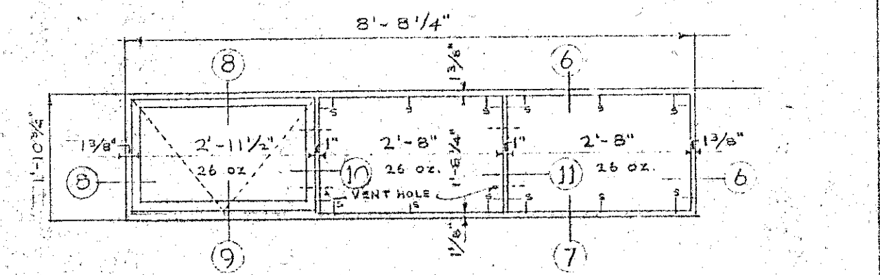
BOY'S WASHROOM WINDOW ELEVATION SCALE 1/2\"/>
