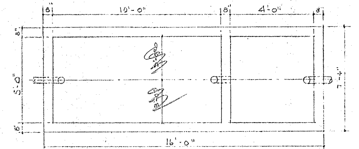
PLAN SCALE \frac{1}{4}'' = 1'-0''
