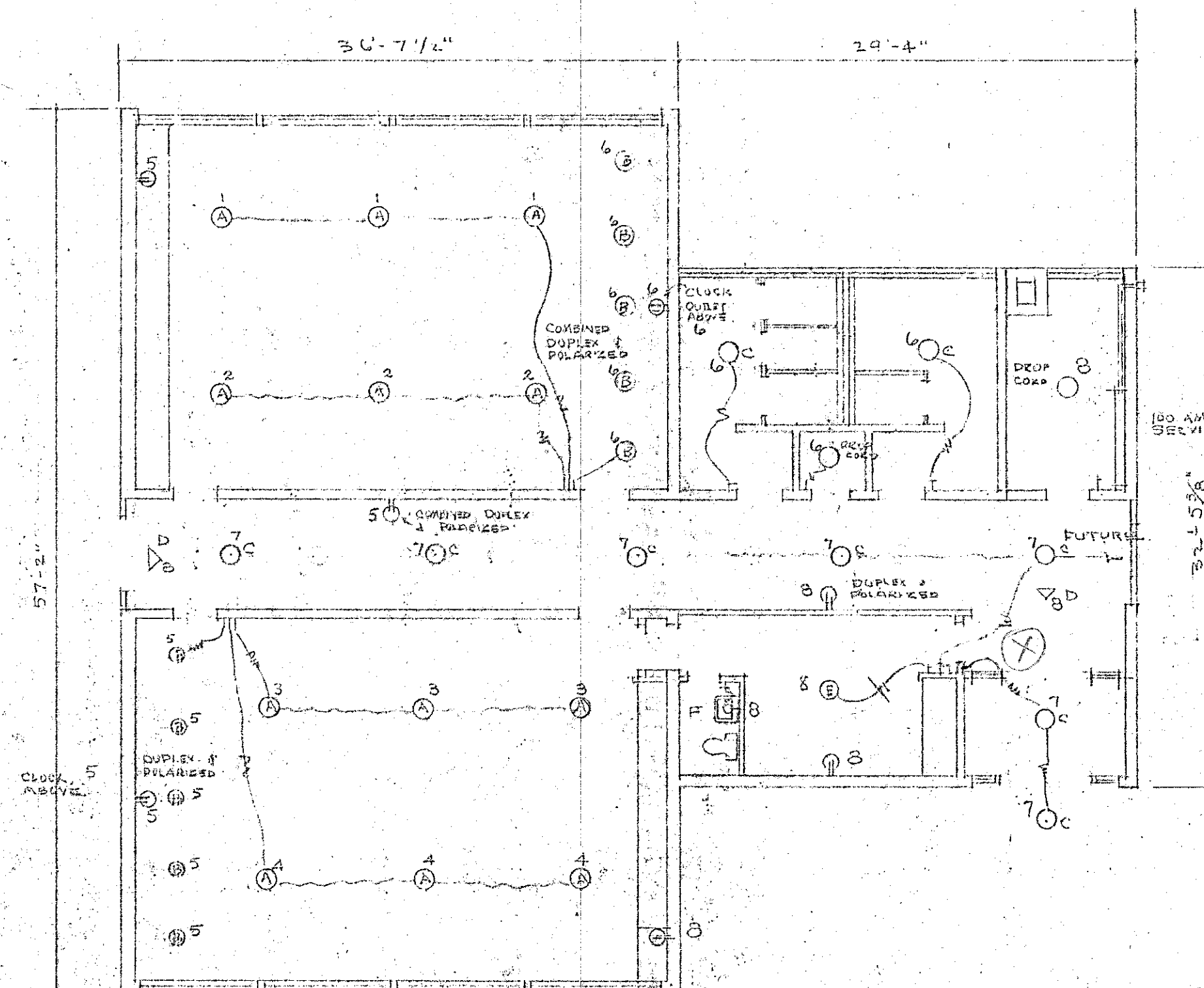
ELECTRICAL PLAN
