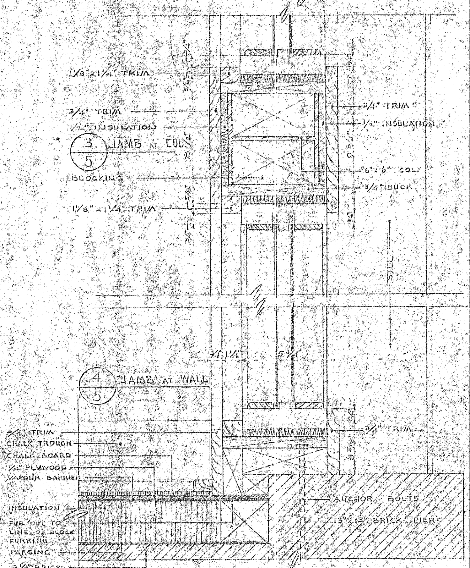
WINDOW SECTIONS SCALE 1/8\"/>
