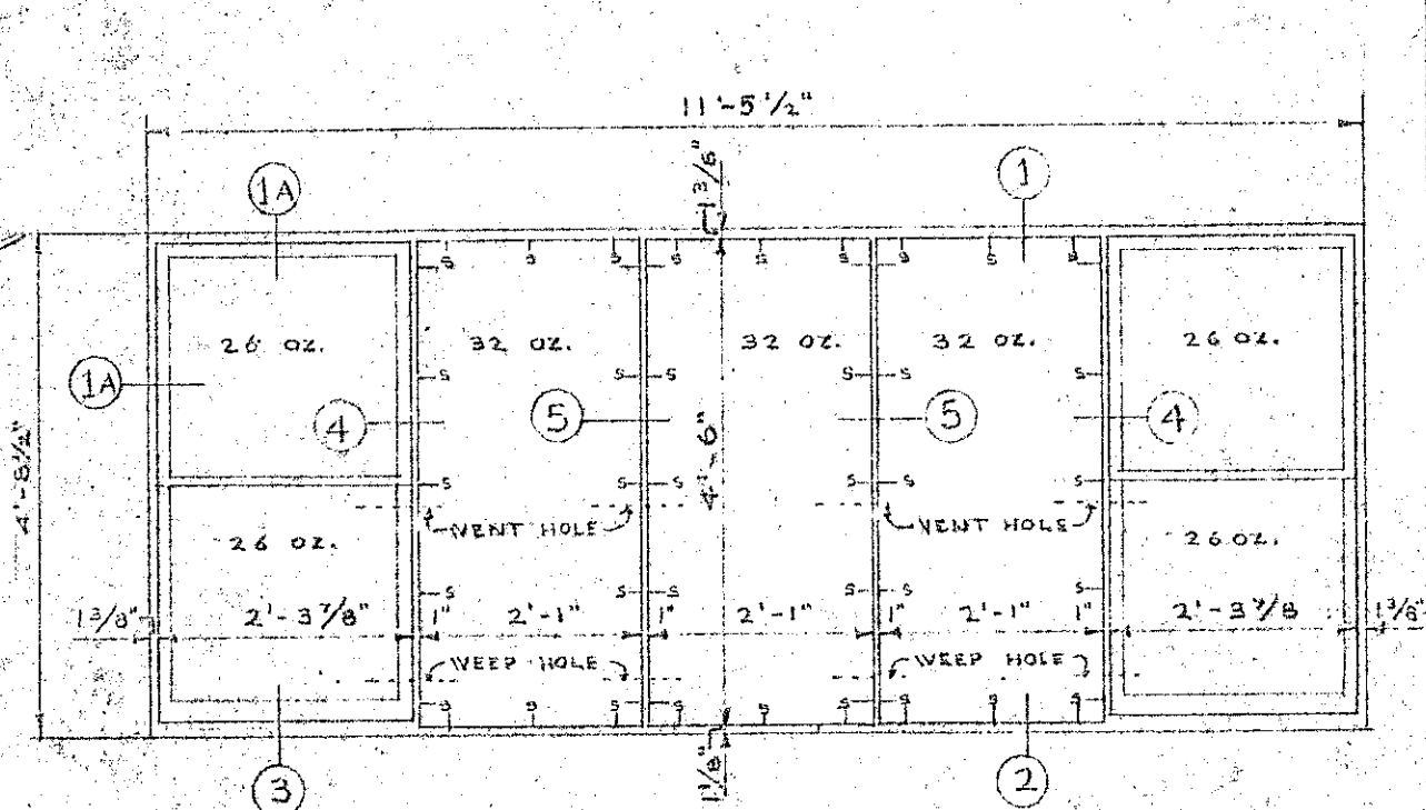
TEACHERS' RM. WINDOW ELEVATION SCALE 1/2\"/>
