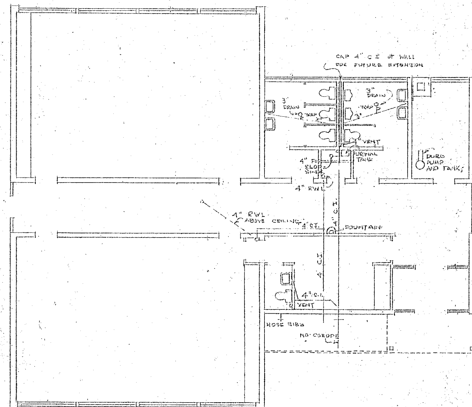
PLUMBING PLAN SCALE \frac{1}{8}'' = 1'-0''
