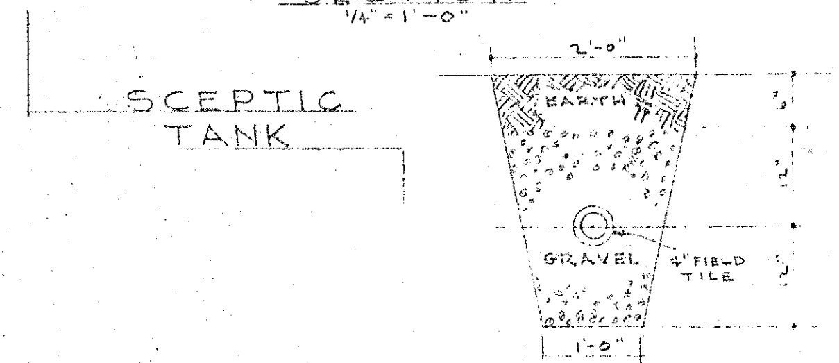
TYPICAL SECTION THRU DISPOSAL BED SCALE \frac{3}{4}'' = 1'-0''
