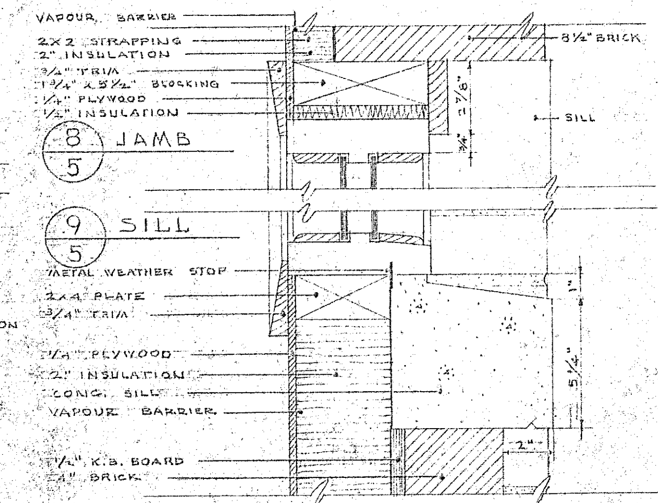
WINDOW SECTIONS SCALE 3/8\"/>
