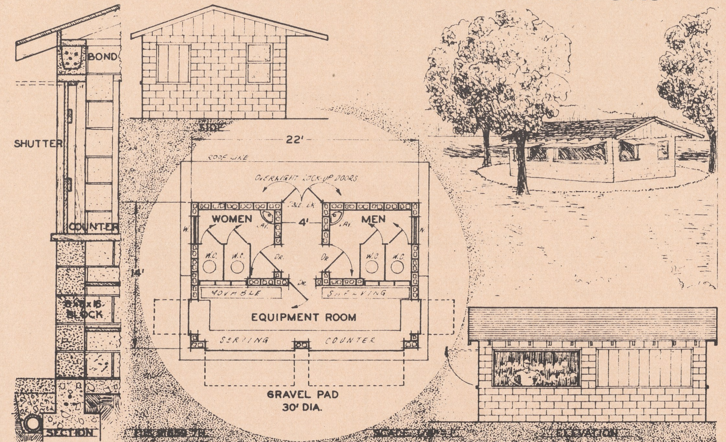
PROPOSED REST-ROOM AND EQUIPMENT BUILDING
