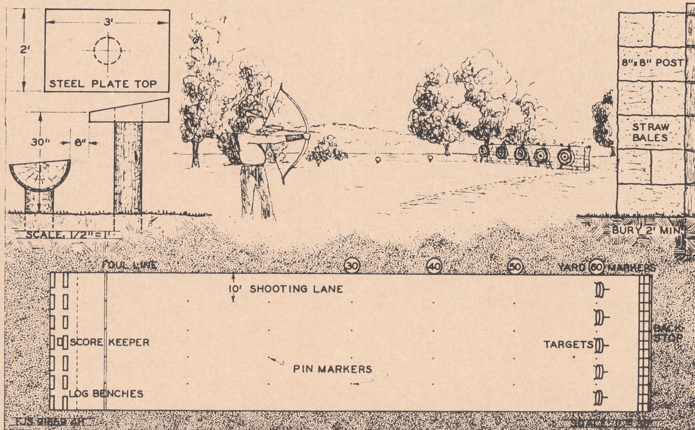
PROPOSED ARCHERY RANGE
