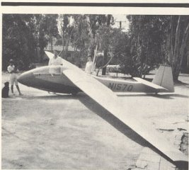
Pictured above is Ranchoite Joel Prescott and his recently completed B G 12 sailplane that he built at home. Using only simple hand tools, the project required over five hundred hours to complete and it was successfully test flown at Elsinore early this month. The aircraft has a wingspan of 50 feet, is 22 feet long and weighs approximately 325 pounds. Seen admiring Daddy's beautiful yellow and blue creation are his wife Elizabeth, daughter Ruth, and family pets. There is much interest in Soaring as a sport in Rancho Santa Fe.
