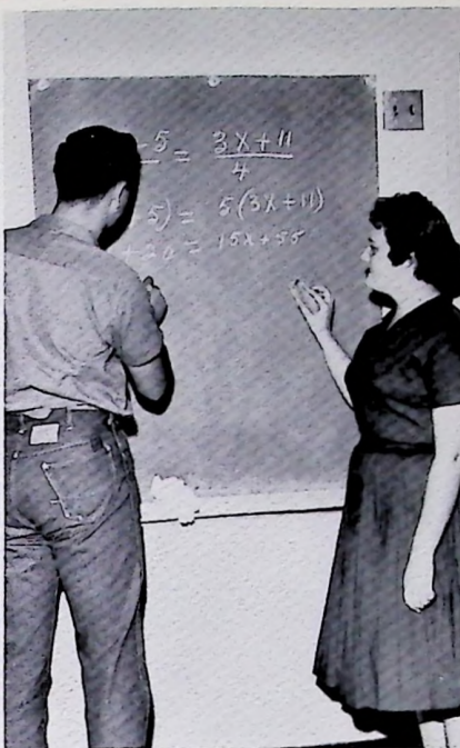
The last rung on the ladder - college algebra.
