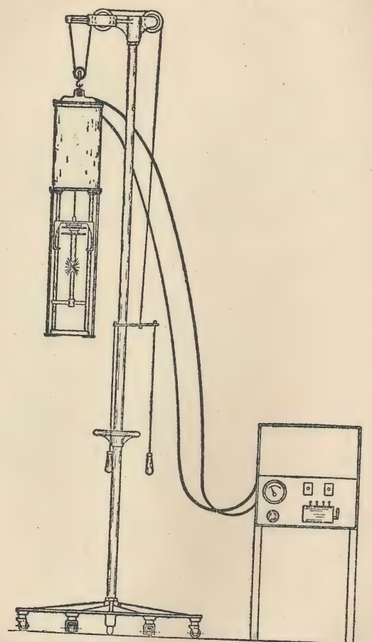
(FIG. 3.) "WESTMINSTER" SUN RAY LONG-FLAME ARC LAMP.
