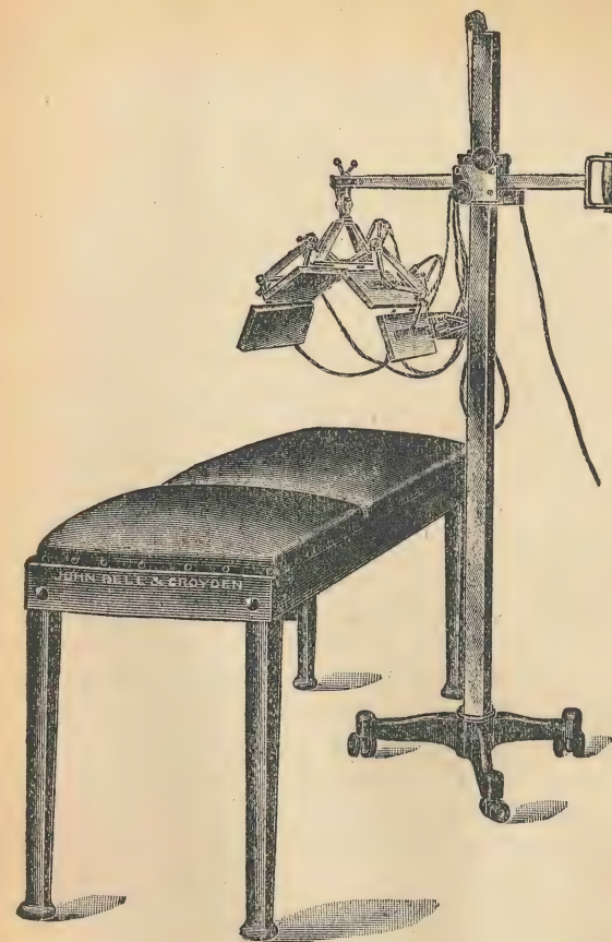
(FIG. 13.) "ARNOLD" INFRA-RED LAMP, HOSPITAL TYPE.
