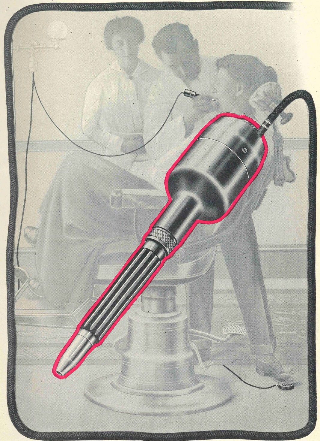
This shows the Shelton Dental Engine in operation—also the foot switch, and an exact size view of the engine which is remarkable because of its small size and many desirable characteristics.
