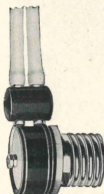
Cat. No. 523. Victor-Coolidge Cathode Terminal with swivel head (Fig. 1). Cat. No. 524. Victor-Coolidge Cathode Terminal (unadjustable) (Fig. 2).
