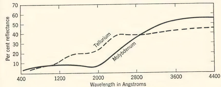
FIG. 8. Reflection from evaporated films of molybdenum and tellurium. (J. B. Sabine, loc. cit.)
