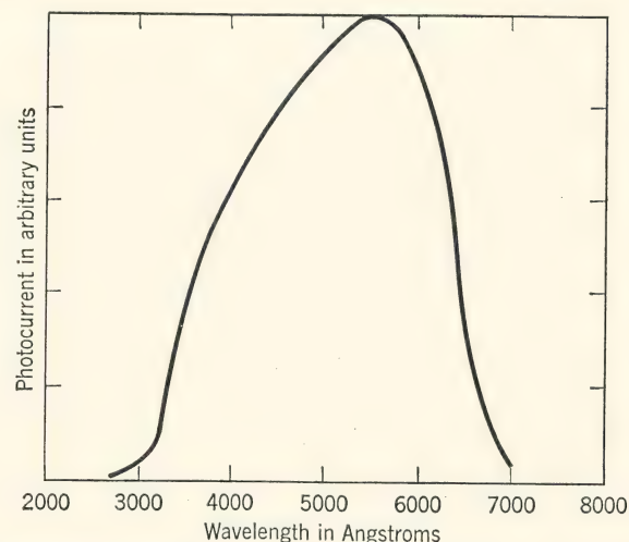
FIG. 13. Spectral response of selenium photovoltaic cell. ( Gen. Elec. Bulletin GEA-24670.)
