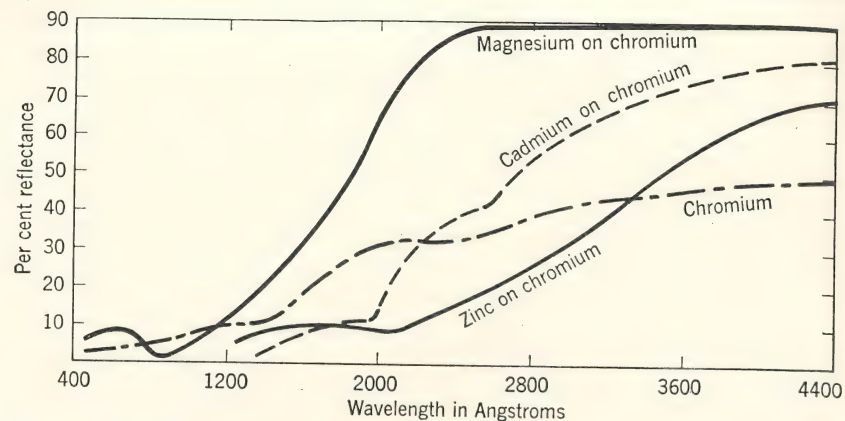
FIG. 9. Reflection from evaporated films of cadmium, magnesium, zinc, and chromium. (J. B. Sabine, loc. cit.)
