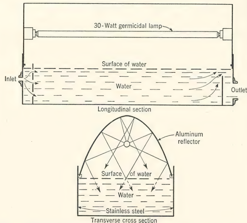
FIG. 11. Water sterilization installation. (M. Luckiesh, Gen. Elec. Rev. , 47 , 49, 1944.)
