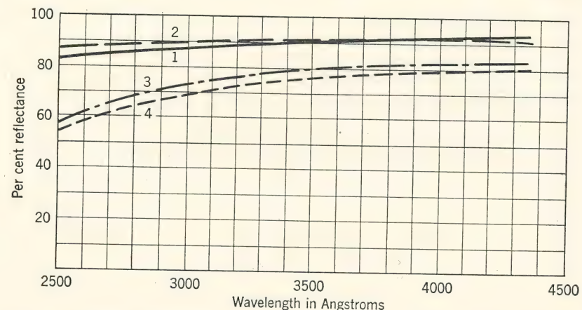
FIG. 2. Spectral reflectance of aluminum with and without Alzak treatment. 1. Bright rolled 2s sheet. 2. Same diffusely etched and brightened. 3. Same as 2 with anodic coating 0.00016". 4. Same as 2 with anodic coating 0.00022". (M. Luckiesh, Germicidal, Erythral and Infrared Energy , D. Van Nostrand Co., New York, 1946.)
