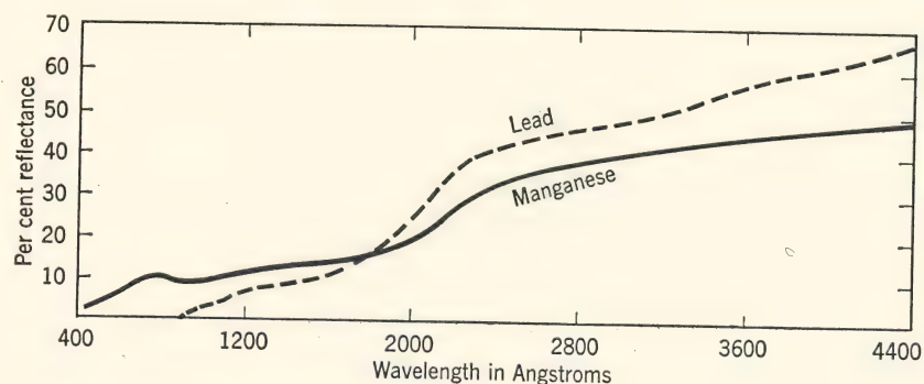
FIG. 5. Reflection from evaporated films of lead and manganese. (J. B. Sabine, loc. cit.)
