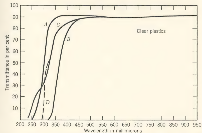
FIG. 18. Spectral transmittance of several clear plastics. A. Methyl methacrylate, thickness 1.47 mm. B. Allyl alcohol, thickness 3.05 mm. C. Cellulose acetate butyrate, thickness 0.41 mm. D. Cellulose acetate, thickness 0.50 mm. ( Natl. Bur. Standards Circ. 471, 1948. )
