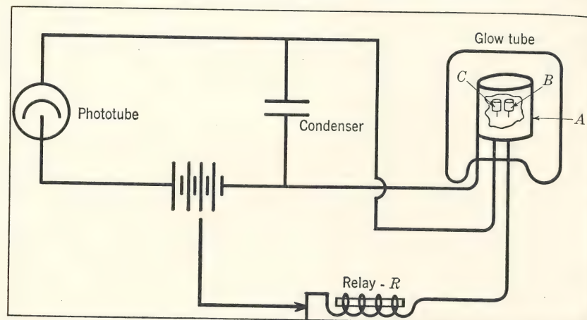
FIG. 5. Rentschler click-meter circuit. ( J. Am. Inst. Elec. Engrs. , 49 , 113, 1930.)
