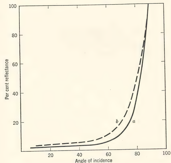
FIG. 13. a . Reflection of ultraviolet (3082 A) from the surface of glass at various angles of incidence. b . Reflection of ultraviolet from the surface of water at various angles of incidence.
