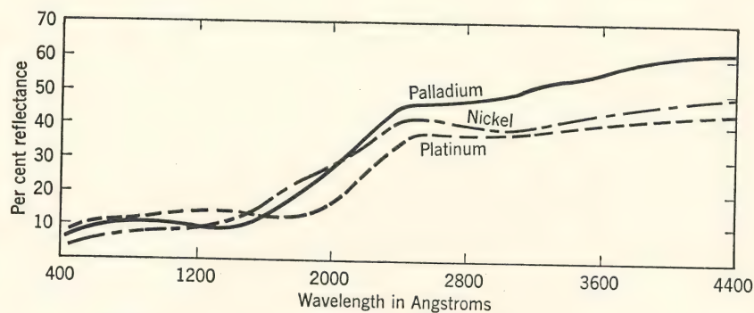
FIG. 4. Reflection from evaporated films of platinum, palladium, and nickel. (J. B. Sabine, loc. cit.)
