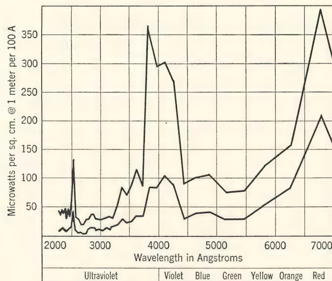
FIG. 36. Spectral energy distribution of carbon arc with strontium-cored carbons (National E). Upper curve, 60 amperes alternating current, 50 volts across arc. Lower curve, 30 amperes alternating current, 50 volts across arc. ( National Carbon Co. Catalog , Section A-4300.)
