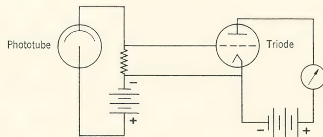
FIG. 3. Simple phototube amplifier circuit.
