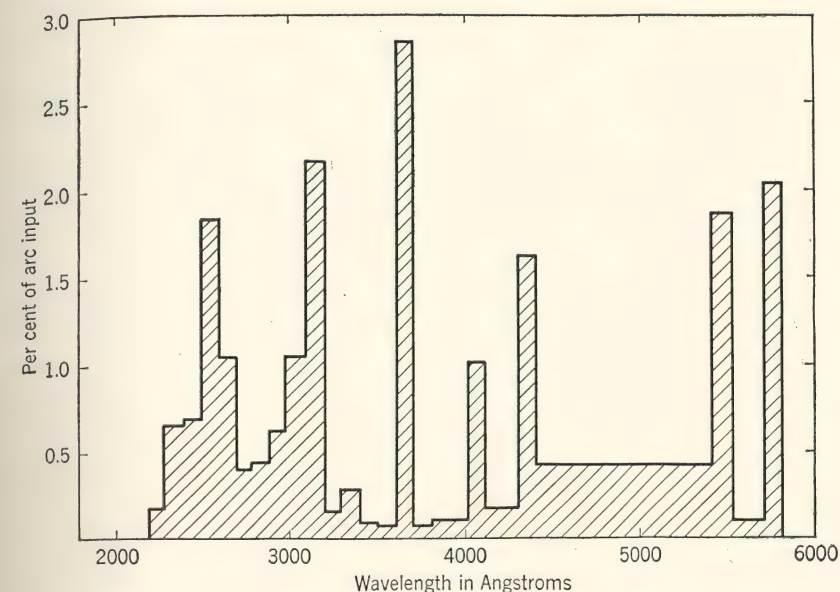
FIG. 12. Energy distribution in spectrum of UA-2 mercury vapor arc in quartz. ( Gen. Elec. Lamp Bulletin LD-1. )
