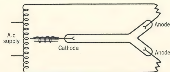
FIG. 10. A-c operated pool-type mercury arc.
