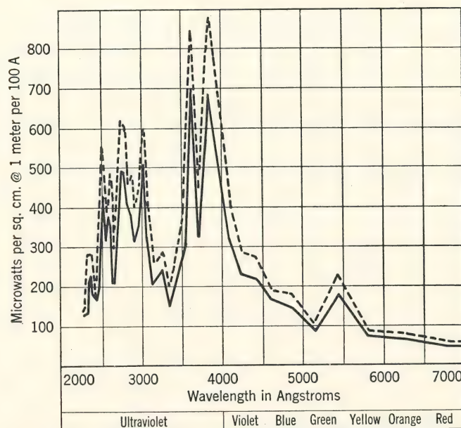
FIG. 39. Spectral energy distribution of carbon arc with polymetallic-cored carbons for high currents (National W). Upper curve, 80 amperes alternating current, 60 volts across arc. Lower curve, 80 amperes alternating current, 50 volts across arc. (National Carbon Co. Catalog, Section A-4300.)
