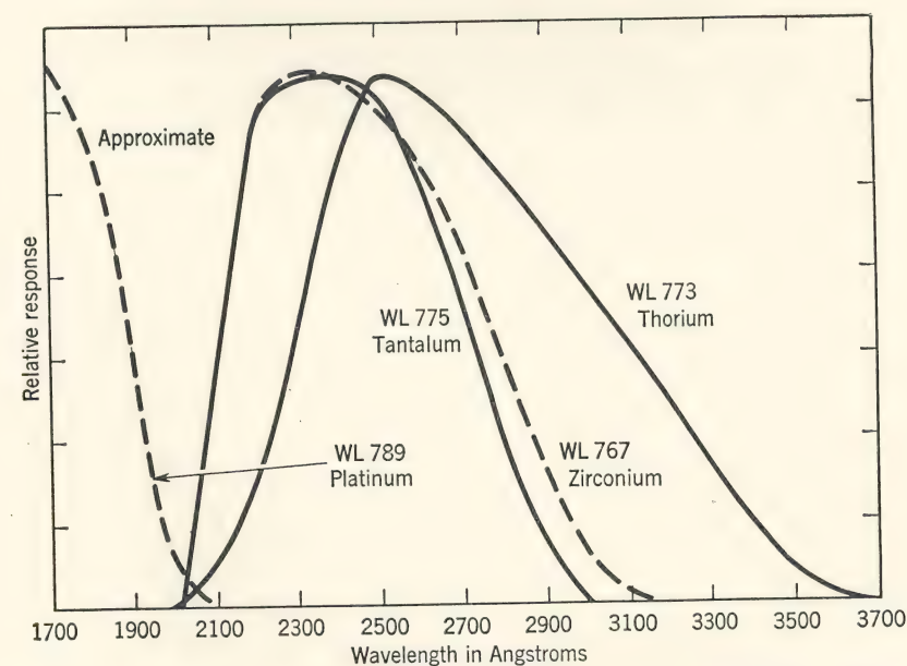
FIG. 10. Spectral response curves of some ultraviolet-sensitive phototubes. (Westinghouse Electric Corp., Data Sheet 86-080.)
