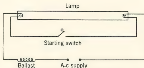
FIG. 21. Starting circuit for germicidal lamps.
