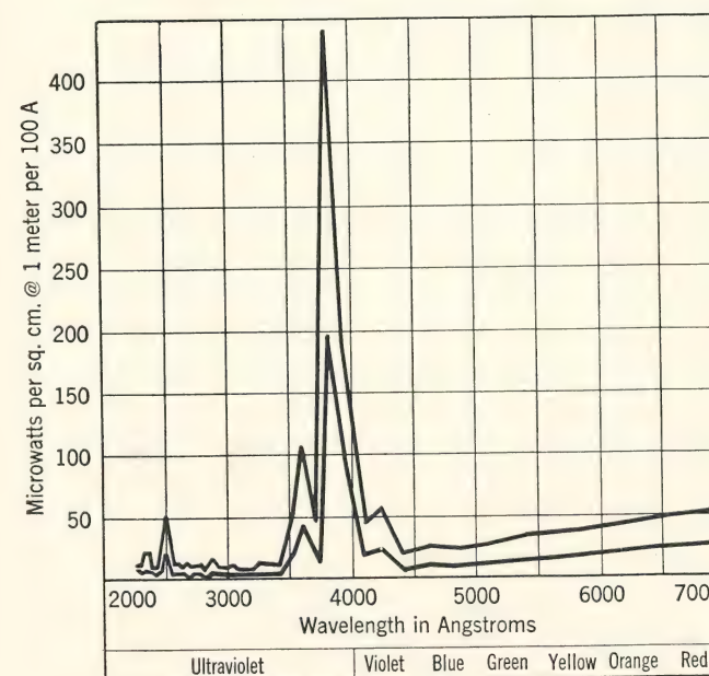
FIG. 35. Spectral energy distribution of carbon arc with core of soft carbon (National D). Upper curve, 60 amperes alternating current, 50 volts across arc. Lower curve, 30 amperes alternating current, 50 volts across arc. ( National Carbon Co. Catalog, Section A-4300. )
