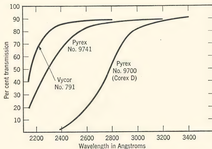
FIG. 6. Transmission of 1 mm thickness of Pyrex and Vycor glasses. (M. E. Nordberg, J. Am. Ceram. Soc. , 30 , 184, 1947.)
