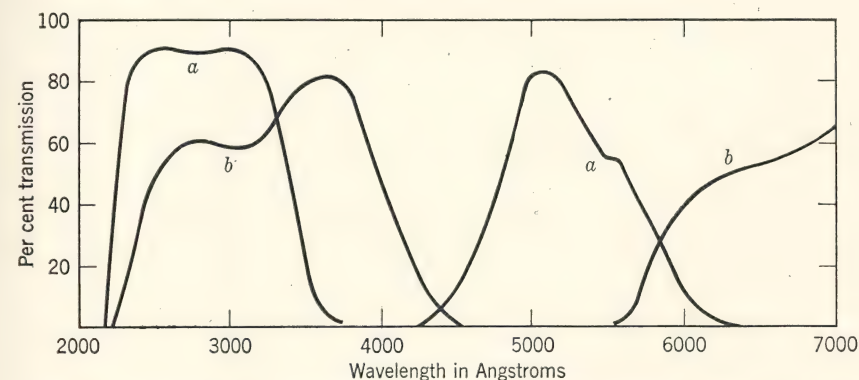
FIG. 13. Transmission of solutions of nickelous and cobaltous sulfate. a. 1 cm of \text{NiSO}_4 \cdot 6\text{H}_2\text{O} , 500 grams per liter. b. 1 cm of \text{CoSO}_4 \cdot 7\text{H}_2\text{O} , 300 grams per liter. (M. Kasha, J. Optical Soc. Am. , 38 , 929, 1948.)
