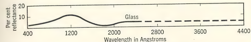
FIG. 12. Reflection from glass at normal incidence. (J. B. Sabine, loc. cit.)
