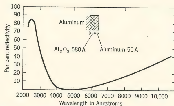
FIG. 17. Reflectivity of reflection type of interference filter. (G. Hass, J. Optical Soc. Am. , 39 , 539, 1949.)
