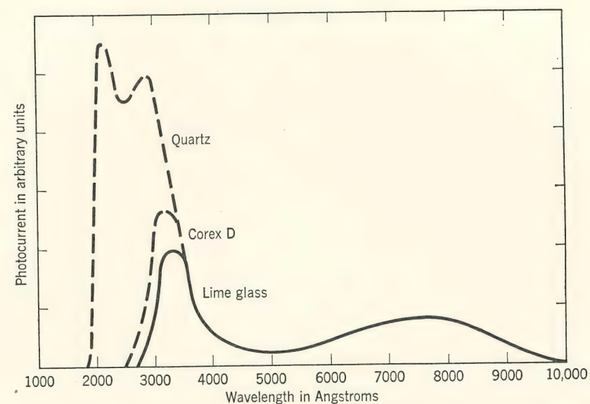
FIG. 9. Effect of envelope material on spectral response of S-1 photo surfaces. (V. K. Zworykin and E. G. Ramberg, Photoelectricity and Its Applications , John Wiley and Sons, New York, 1949.)
