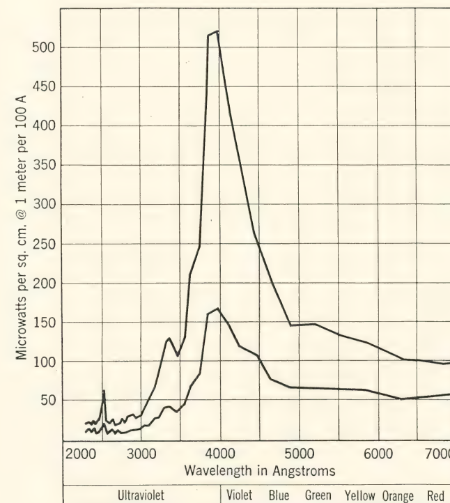
FIG. 31. Spectral energy distribution of carbon arc with cerium-cored carbons (National Sunshine). Upper curve, 60 amperes alternating current, 50 volts across arc. Lower curve, 30 amperes alternating current, 50 volts across arc. (National Carbon Co. Catalog, Section A-4300.)
