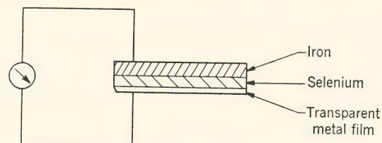
FIG. 11. Photovoltaic cell. Schematic diagram.
