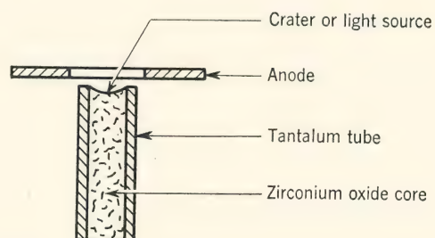
FIG. 25. Electrodes of zirconium concentrated arc.
