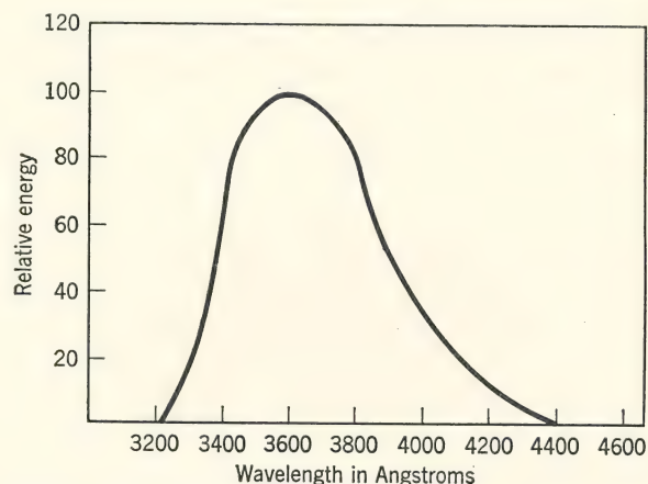
FIG. 17. Radiation from BL lamps. (H. Froelich, Trans. Electrochem. Soc. , 91 , 241, 1947.)
