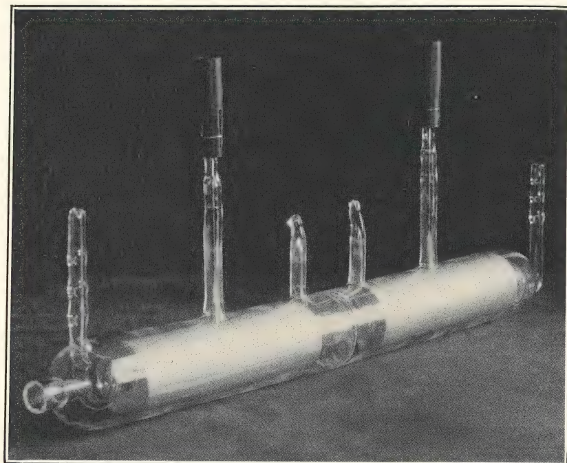
FIG. 27. Hydrogen arc in quartz. Emission is through windows at ends of tube. Vertical tubes at end are for water circulation. (Courtesy of Hanovia Chemical and Mfg. Co.)
