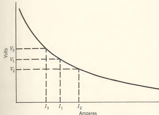
FIG. 2. Instability of an arc.
