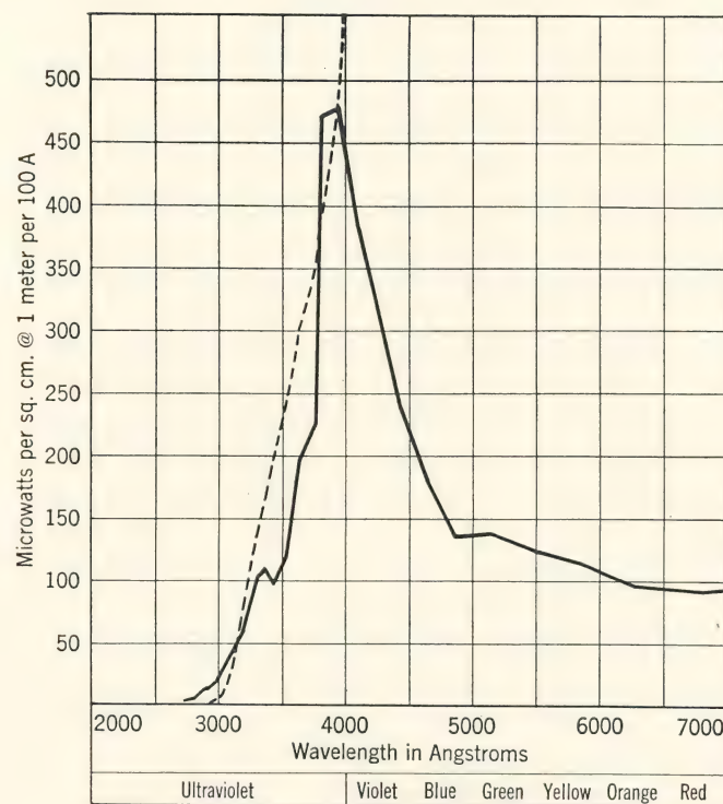
FIG. 32. National Sunshine Carbon with Corex filter compared with natural sunlight. Solid line, with Corex D filter. Dotted line, natural sunlight. (National Carbon Co. Catalog, Section A-4300.)
