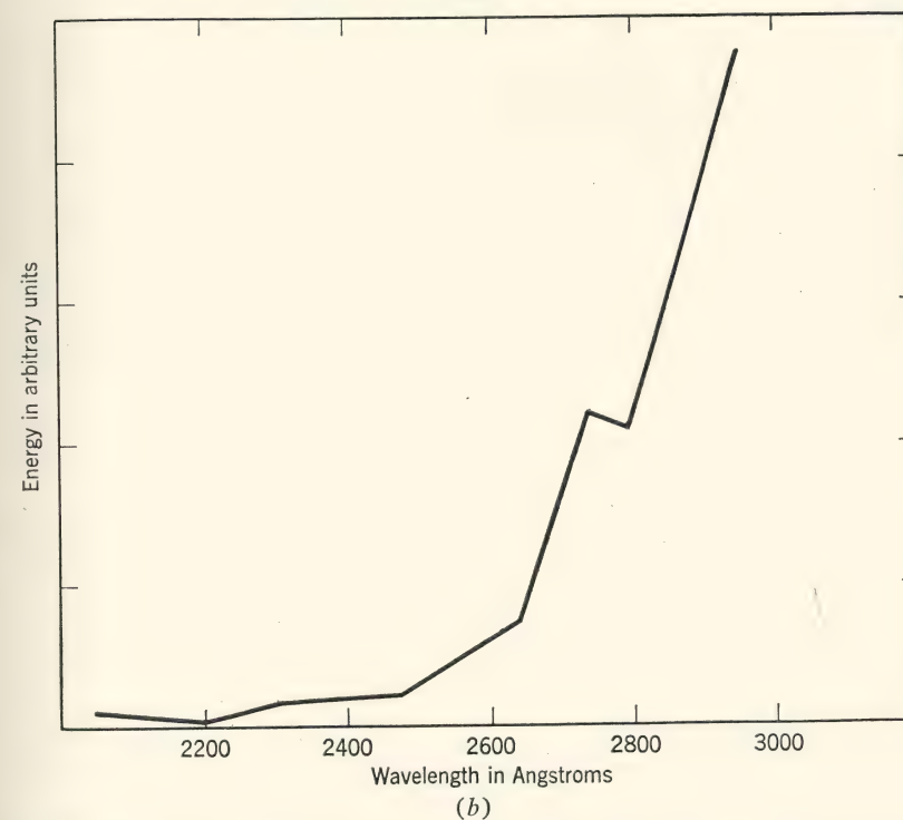
FIG. 26. Spectrum of zirconium arc. a. 100-watt arc in glass. b. 1000-watt Telco arc in air. (Courtesy of Western Union Telegraph Co.)
