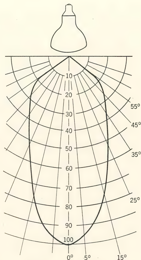
FIG. 17. Angular distribution of energy in the beam of the RS lamp. ( Gen. Elec. Lamp Bulletin LD-1. )
