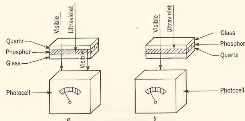
FIG. 14. Luckiesh-Taylor conversion-type ultraviolet meter.
