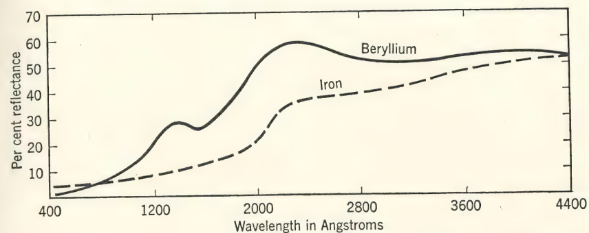
FIG. 6. Reflection from evaporated films of beryllium and iron. (J. B. Sabine, loc. cit.)
