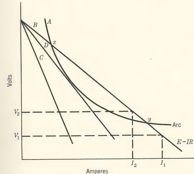
FIG. 4. Conditions for stability of an arc. (P. Copeland and W. H. Sparing, J. Applied Phys. , 16, 302, 1945.)
