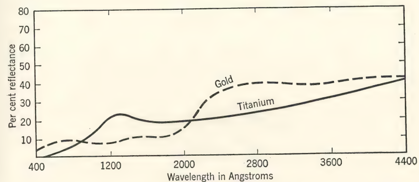
FIG. 7. Reflection from evaporated films of gold and titanium. (J. B. Sabine, loc. cit.)
