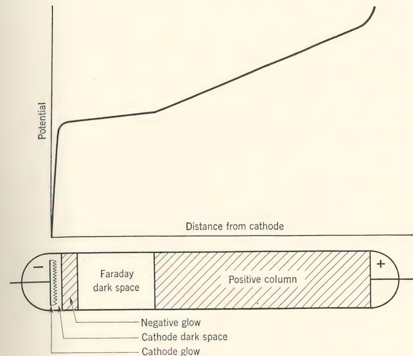
FIG. 6. Potential distribution in a glow discharge.
