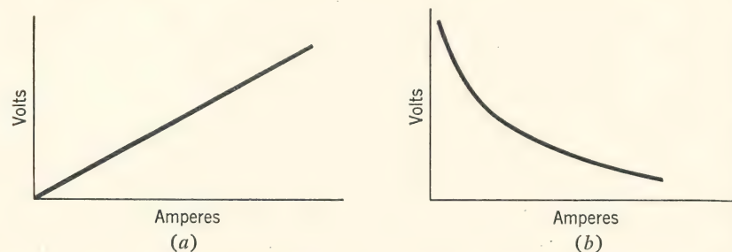
FIG. 1. Volt ampere characteristics. a. Relation between current and voltage for an ohmic resistance. b. Relation between current and voltage for an arc.
