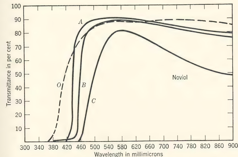
FIG. 21. Spectral transmittance of Noviol glass. Noviol O, thickness 2.63 mm. Noviol A, thickness 1.90 mm. Noviol B, thickness 2.89 mm. Noviol C, thickness 3.05 mm. ( Natl. Bur. Standards Circ. 471, 1948.)
