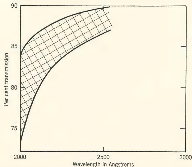
FIG. 8. Limits of the transmission of thirty-one samples of fused quartz obtained from two different manufacturers. Samples \frac{1}{16} in. thick. No correction for reflection. (Courtesy of E. A. Taft.)
