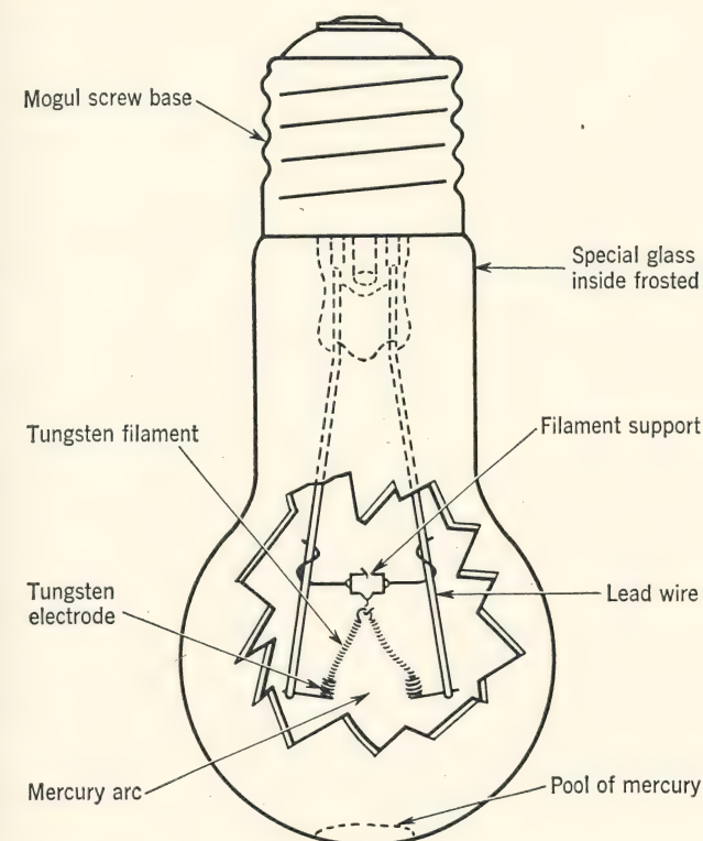
FIG. 13. Construction of S-1 Lamp. ( Gen. Elec. Lamp Bulletin LD-1.)
