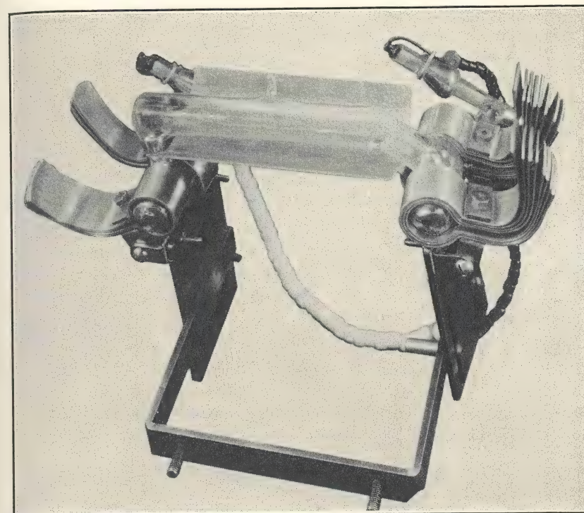
FIG. 9. Pool-type quartz mercury arc for vertical or horizontal operation. Now superseded. (Courtesy of Hanovia Chemical and Mfg. Co.)
