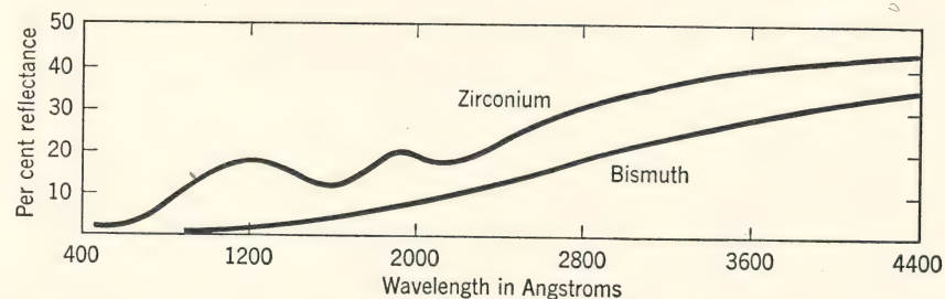
FIG. 11. Reflection from evaporated films of bismuth and zirconium. (J. B. Sabine, loc. cit.)
