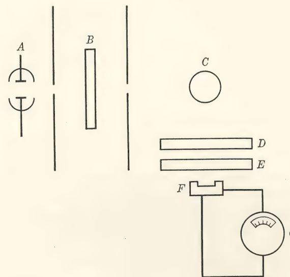
FIG. 18. Fluorometer. A. Ultraviolet source. B. Filter to exclude visible radiation. C. Sample. D, E. Filter to exclude ultraviolet. F. Photocell detector. G. Galvanometer.
