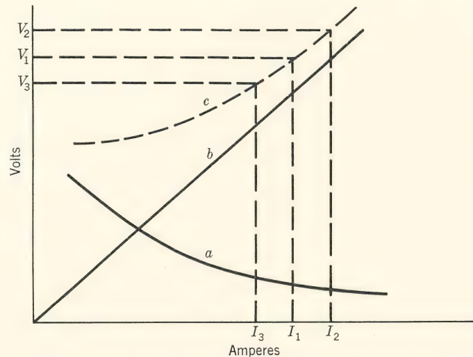
FIG. 3. Stability of an arc with a ballast resistance. a . Arc characteristic. b . Ballast characteristic. c . Combined characteristic.
