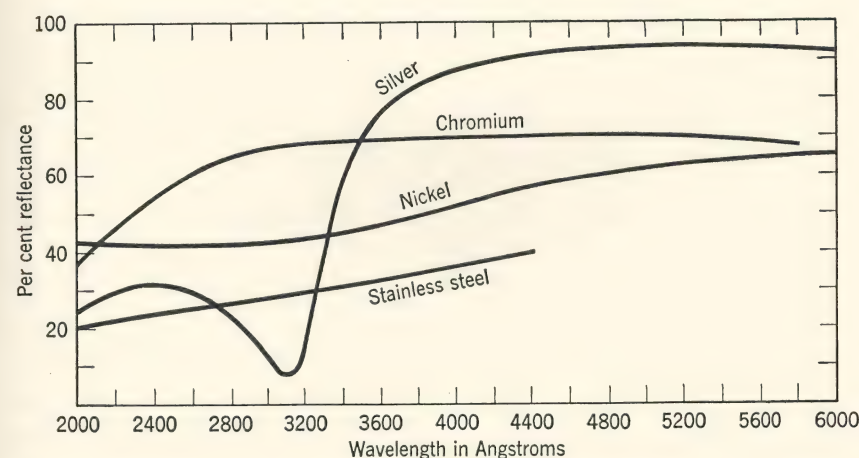
FIG. 1. Reflection from silver, chromium, nickel, and stainless steel. (M. Luckiesh, J. Optical Soc. Am. , 19 , 1, 1929.)
