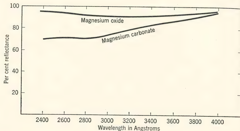
FIG. 16. Reflection from magnesium oxide and magnesium carbonate. (F. Benford, S. Schwartz, and G. Lloyd, J. Optical Soc. Am. , 38 , 964, 1948.)
