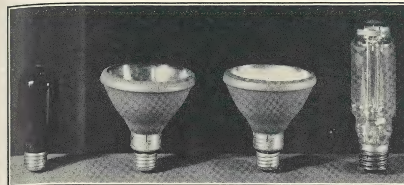
FIG. 16. High-pressure mercury lamps using the same type of arc in different types of bulbs. (Courtesy of General Electric Co.)
