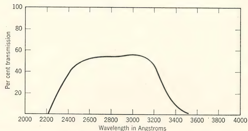
FIG. 14. Transmission of filter consisting of a 5-cm path of aqueous solution containing 240 grams per liter of \text{NiSO}_4 \cdot 6\text{H}_2\text{O} and 45 grams per liter of \text{CoSO}_4 \cdot 7\text{H}_2\text{O} . (M. Kasha, J. Optical Soc. Am. , 38 , 929, 1948.)
