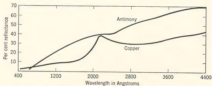
FIG. 10. Reflection from evaporated films of antimony and copper. (J. B. Sabine, loc. cit.)
