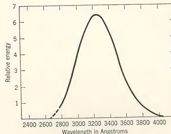
FIG. 16. Radiation from E lamps. (H. Froelich, Trans. Electrochem. Soc. , 91 , 241, 1947.)
