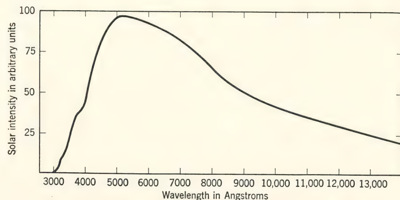
FIG. 12. Solar energy distribution for midsummer noonday sun in Washington, D. C. (Calculated from W. E. Forsythe, Measurement of Radiant Energy , McGraw-Hill Book Co., New York, 1937.)
