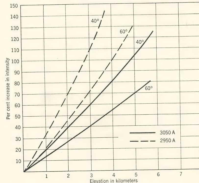
FIG. 16. Effect of elevation above sea level on ultraviolet intensity for different values of solar altitude.
