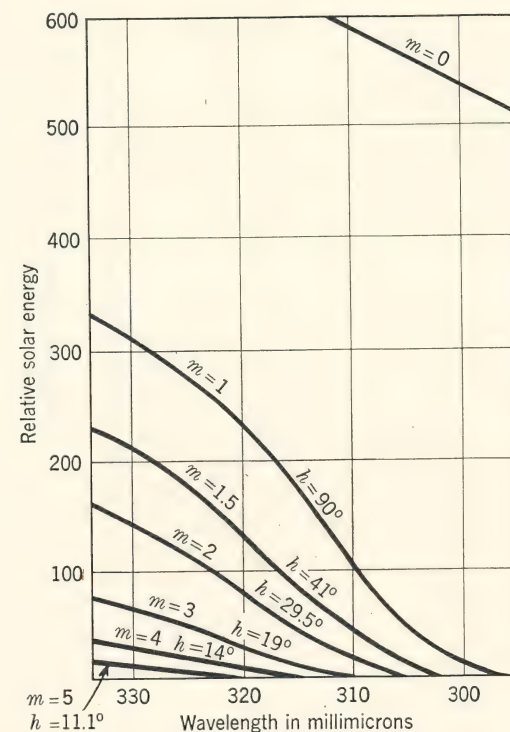
FIG. 17. Calculated values of ultraviolet intensity for different values of air mass. (K. Büttner and E. Sutter, Strahlentherapie , 45, 451, 1932.)
