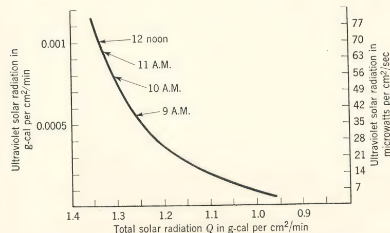
FIG. 11. Ultraviolet less than 3132 Å relative to the total solar radiation. (W. W. Coblentz and R. Stair, J. Research Natl. Bur. Standards , 17 , 1, 1936.)
