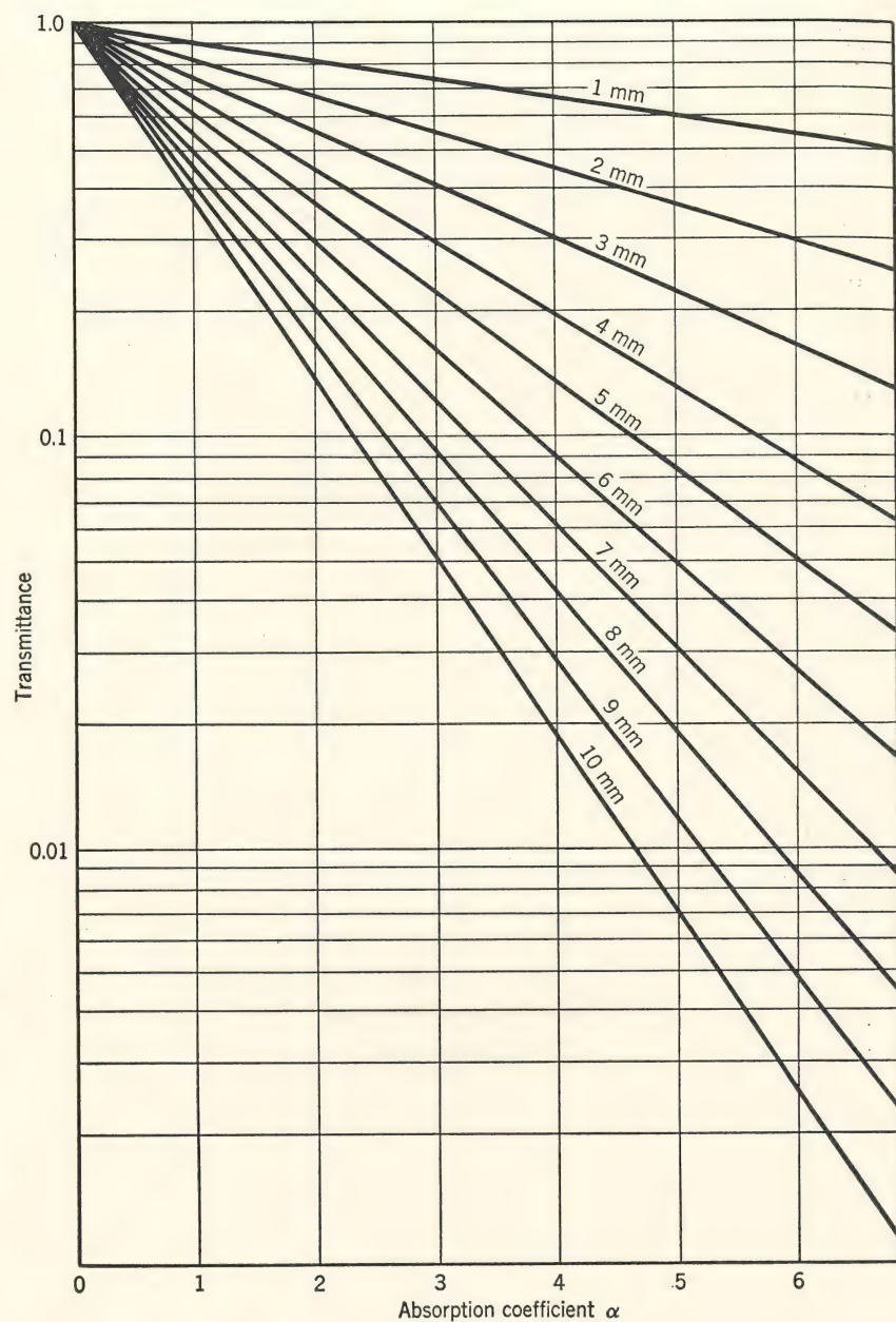
FIG. 1. Transmittance as a function of absorption coefficient for various thicknesses of absorbing medium.
