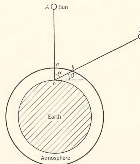
FIG. 2. Relation between air mass and solar elevation.
