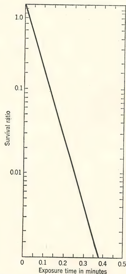
FIG. 5. Survival ratio as a function of exposure time for B. coli exposed to 100 \mu\text{W} per \text{cm}^2 of 2537 Å radiation.
