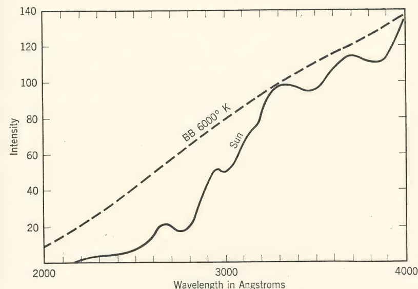
FIG. 1. Comparison of solar energy distribution in the ultraviolet outside the earth's atmosphere with that of a black body at 6000^{\circ}\text{K} . (E. O. Hulburt, J. Optical Soc. Am. , 37 , 414, 1947.)
