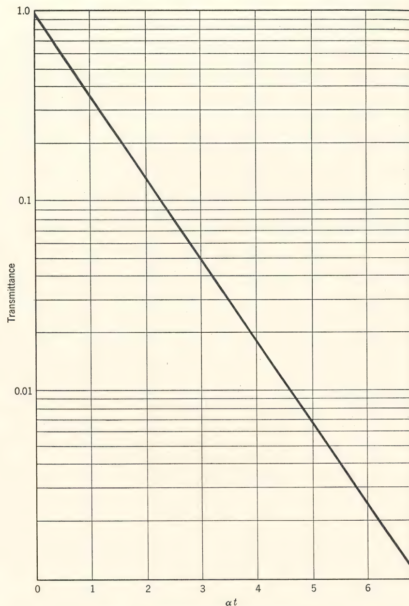
FIG. 3. Transmittance as a function of \alpha t .
