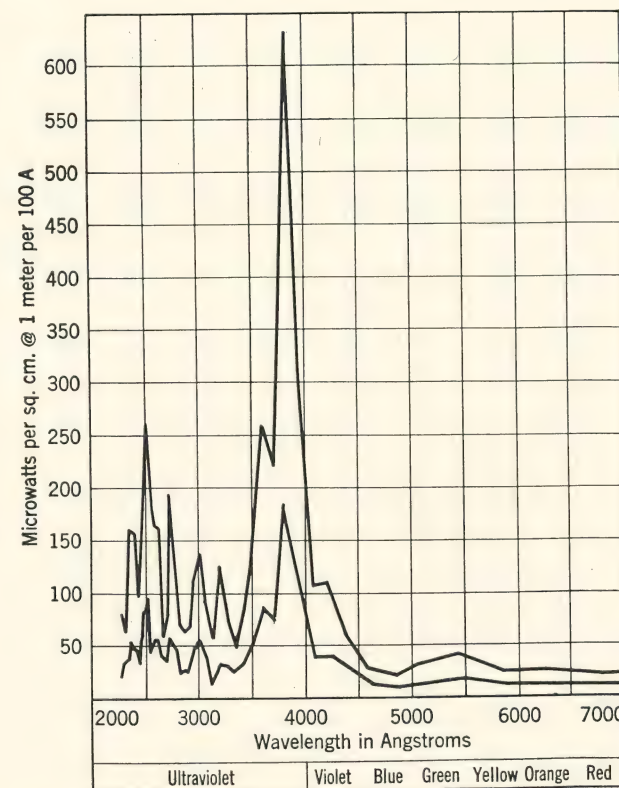
FIG. 33. Spectral energy distribution of carbon arc with iron-cored carbons (National B). Upper curve, 60 amperes alternating current, 50 volts across arc. Lower curve, 30 amperes alternating current, 50 volts across arc. (National Carbon Co. Catalog, Section A-4300.)
