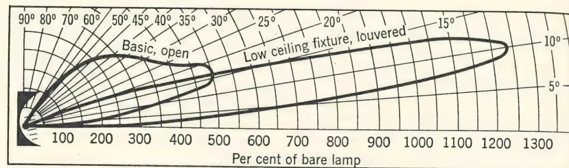
FIG. 9. Distribution of radiation from typical fixture. ( Gen. Elec. Lamp Bulletin LD-14.)
