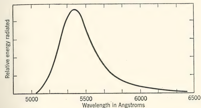
FIG. 7. Energy distribution in the emission spectrum of fluorescent zinc silicate.
