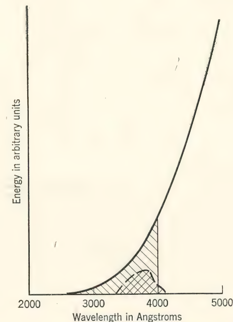
FIG. 4. Effect of filter on radiation from incandescent lamp. Shaded region, available ultraviolet energy; cross-hatched region, ultraviolet transmitted by filter.
