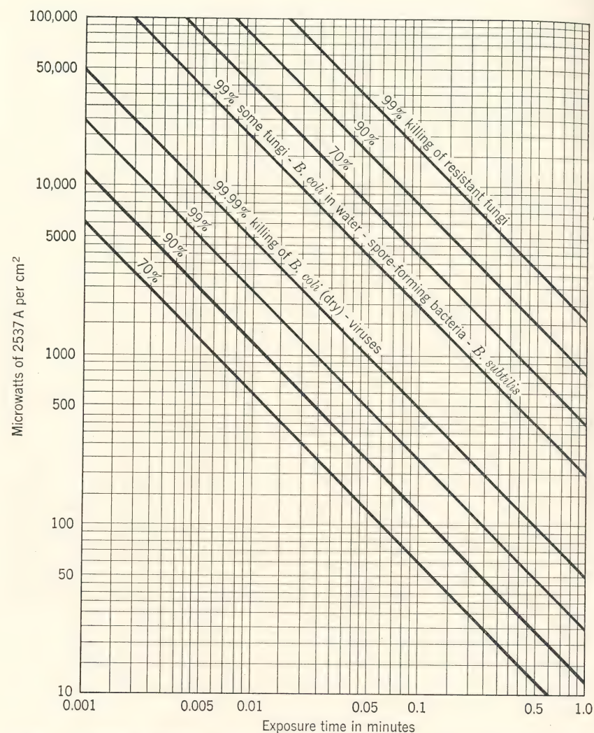
FIG. 6. Ultraviolet intensity and exposure time required to give various values of survival ratios for bacteria and molds. (Gen. Elec. Lamp Bulletin LD-14.)
