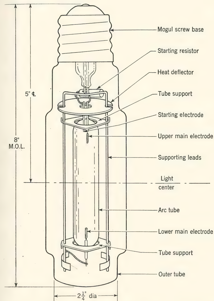
Fig. 15. Construction of a typical high-pressure mercury arc. (Courtesy of General Electric Co.)
