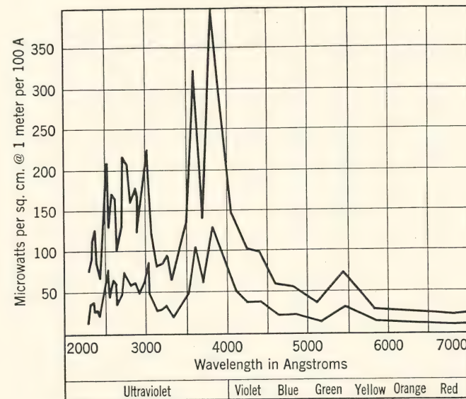
FIG. 38. Spectral energy distribution of carbon arc with polymetallic-cored carbons (National U). Upper curve, 60 amperes alternating current, 50 volts across arc. Lower curve, 30 amperes alternating current, 50 volts across arc. ( National Carbon Co. Catalog , Section A-4300.)
