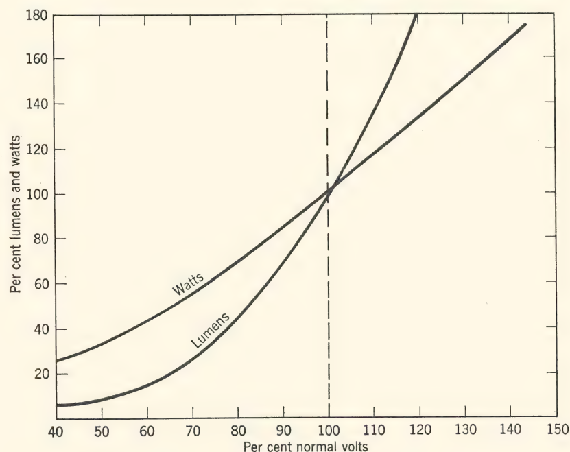
FIG. 5. Effect of voltage variation on output of incandescent lamp. ( Gen. Elec. Lamp Bulletin LD-1. )
