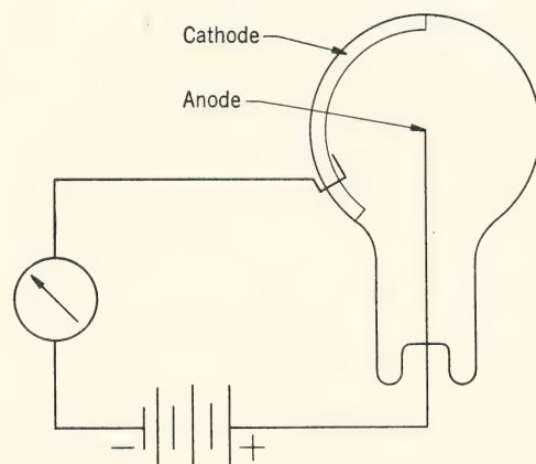
FIG. 1. Photoelectric tube and circuit.
