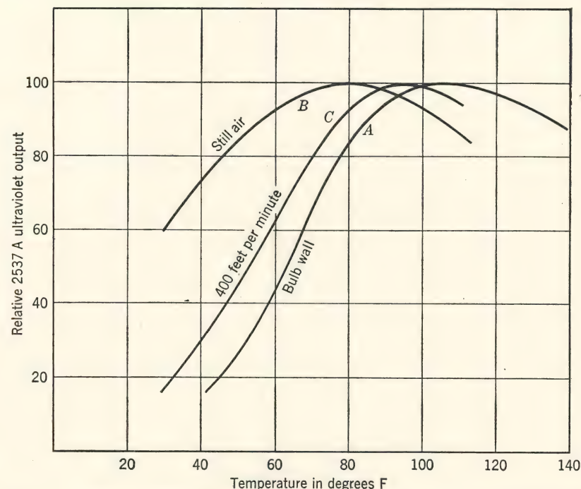
FIG. 22. Effect of ambient temperature on output of Sterilamps. (Westinghouse Electric Corp., Data Sheet ASC-159, 1951.)
