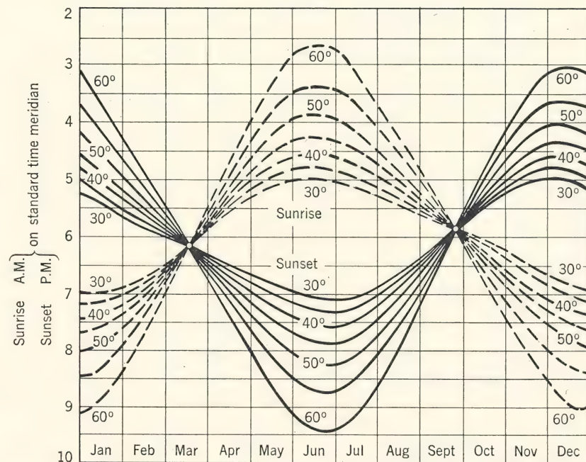
FIG. 15. Time of sunrise and sunset at various latitudes in the northern hemisphere. (F. Benford, Illum. Eng. , 42, 527, 1947.)
