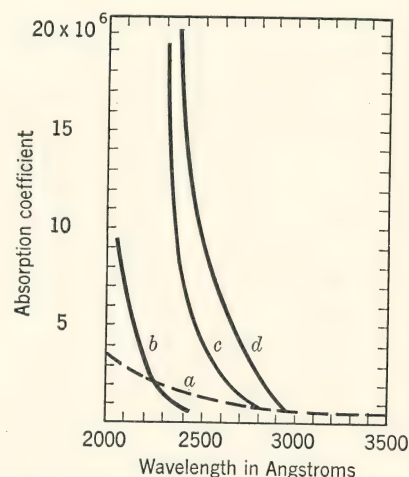
FIG. 24. Absorption coefficient for air as a function of wavelength. a . Calculated. c . Observed, clear atmosphere. b . Extension of c to 2050 Å; ordinates should be multiplied by 10. d . Observed, hazy atmosphere. (L. H. Dawson, L. P. Granath, and E. O. Hulburt, Phys. Rev. , 34 , 136, 1929.)
