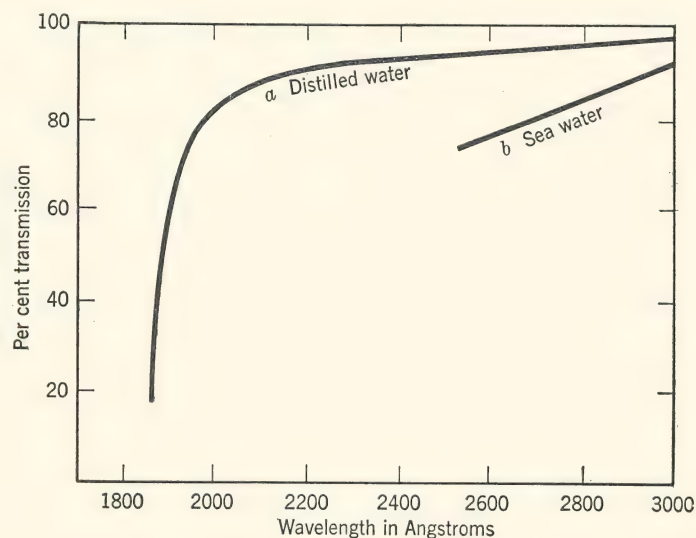
FIG. 19. Transmission of 20 mm of water. a. Distilled water. ( International Critical Tables .) b. Sea water. (E. O. Hulburt, J. Optical Soc. Am. , 17, 15, 1928.)
