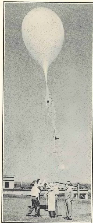
FIG. 5. Radio sonde. (Courtesy of General Electric Co.)
