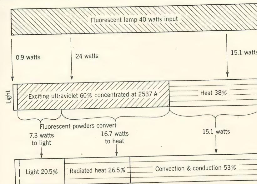
FIG. 15. Energy transformation in a 40-watt fluorescent lamp.
