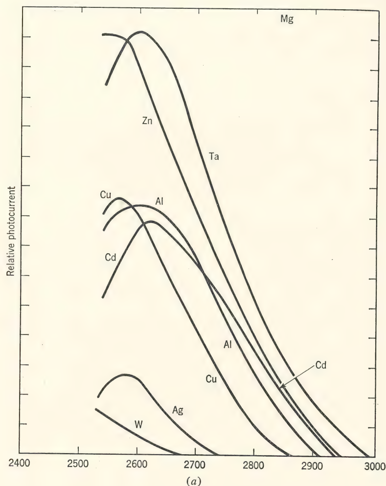
FIG. 7. a and b . Spectral response curves for various metals. (After H. Rentschler, J. Am. Inst. Elec. Engrs. , 49, 576, 1936.)
