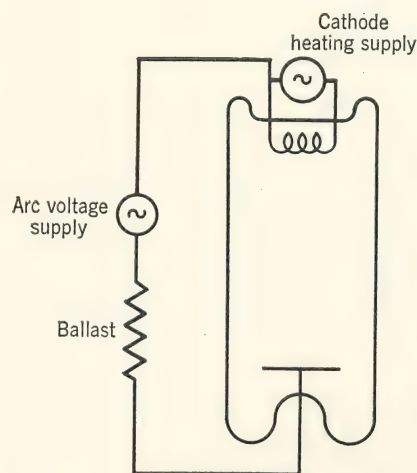
FIG. 8. Arc with separately excited cathode.
