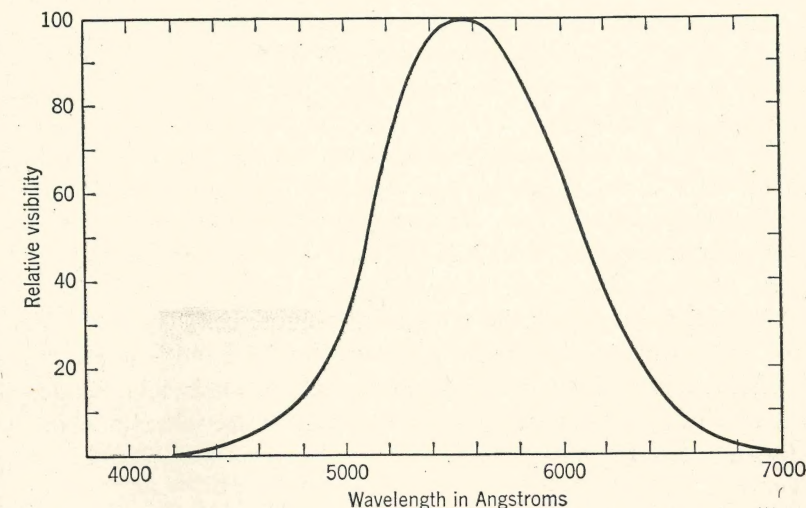
Fig. 2. Relative visibility curve for the average human eye.
