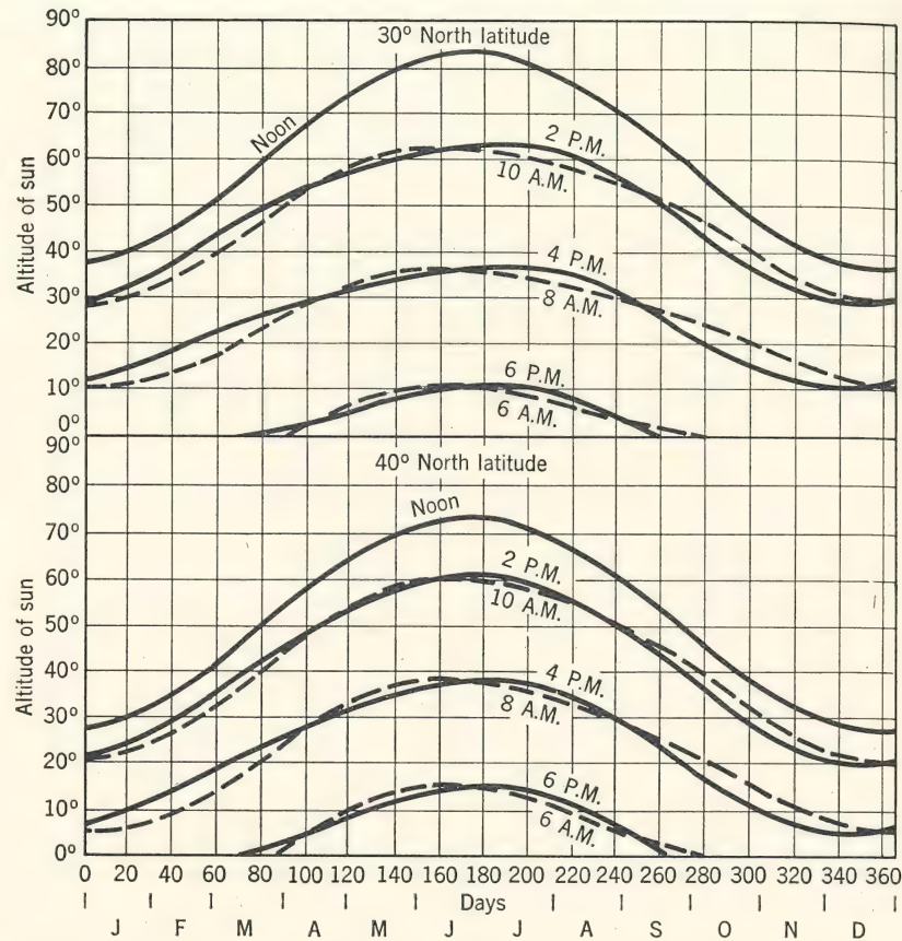
FIG. 3a. Solar altitude at various hours of the day throughout the year at north latitude 30° and 40°. (F. Benford, Illum. Eng. , 42, 527, 1947.)
