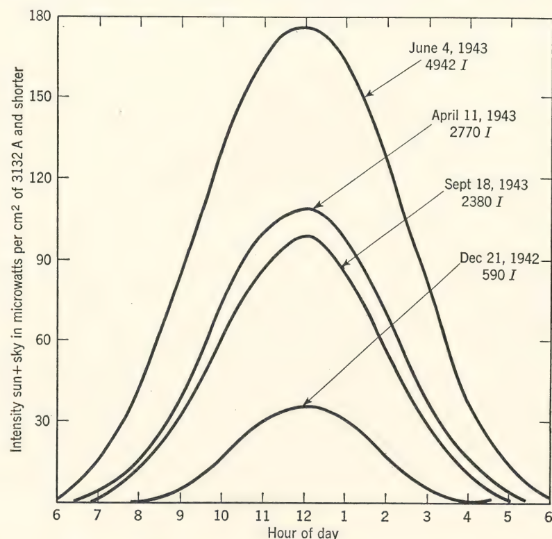
FIG. 10. Total intensity of ultraviolet of wavelength less than 3132 Å from the sun and from the sky incident on a horizontal plane on four very clear days at different seasons in Washington, D. C. (W. W. Coblentz and R. Stair, J. Research Natl. Bur. Standards , 33 , 21, 1944.)
