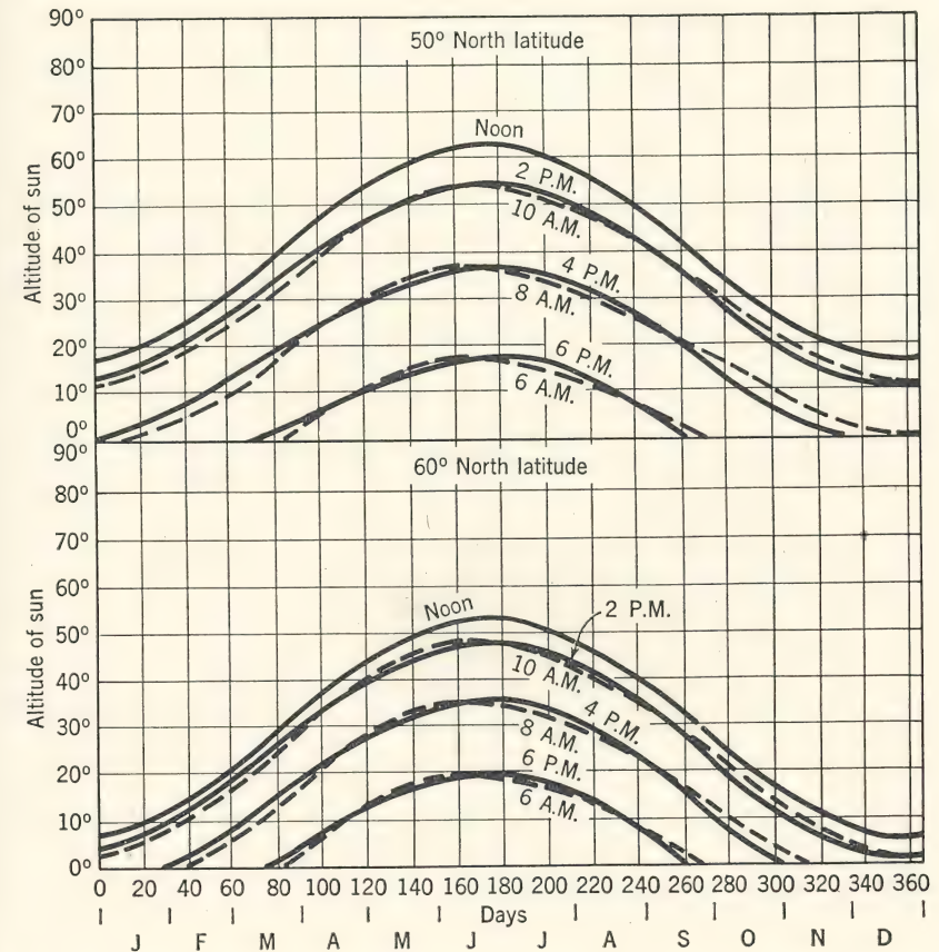
FIG. 3b. Solar altitude at various hours of the day throughout the year at north latitude 50° and 60°. (F. Benford, Illum. Eng. , 42, 527, 1947.)
