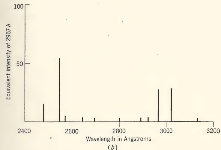
FIG. 9. a. Energy distribution in the various lines of the spectrum of a quartz mercury arc. b. Relative effectiveness of the lines of the quartz mercury arc shown in Fig. 9a in producing erythema.
