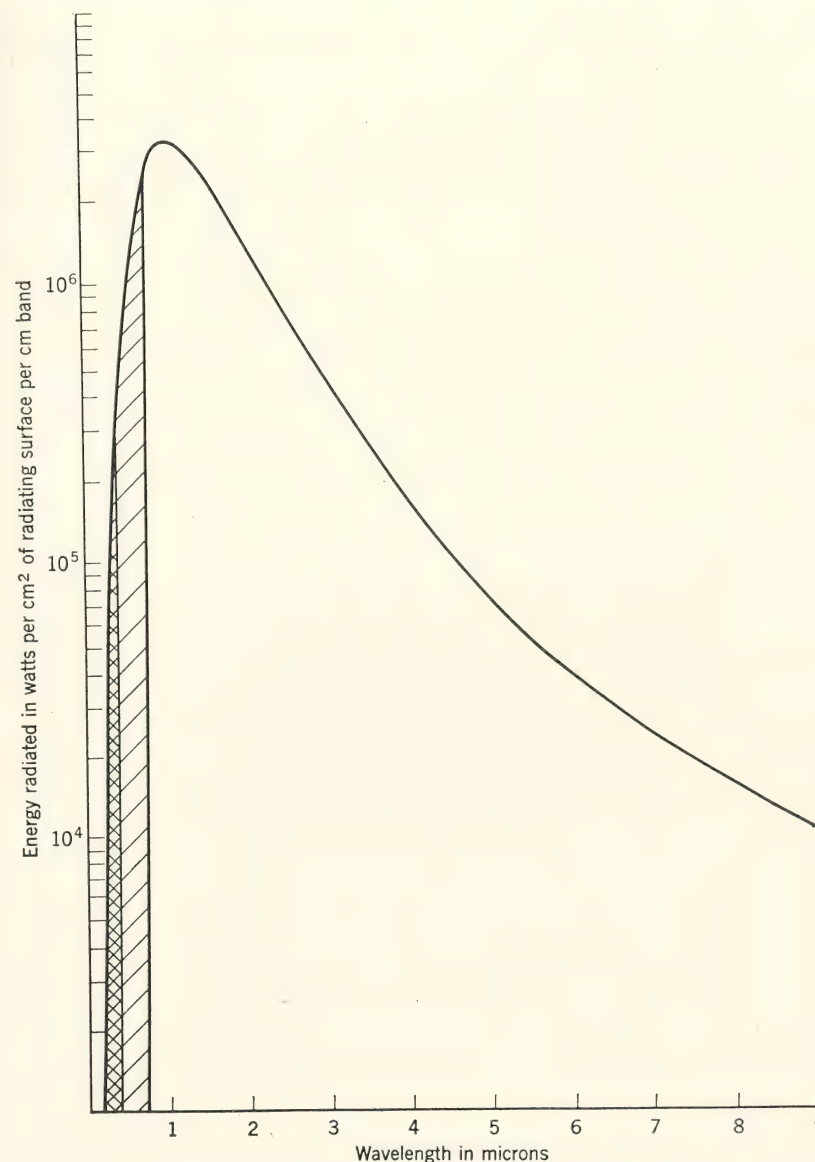
FIG. 1. Planck's distribution law for a black-body radiator at 3000°K. Shaded area, visible radiation; cross-hatched area, ultraviolet radiation.
