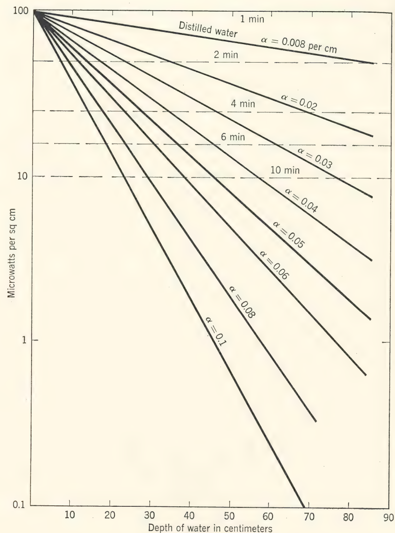
FIG. 12. Intensity of 2537 Å radiation as a function of depth below the surface of water for the various values of absorption coefficient.
