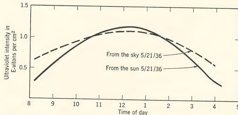
FIG. 7. Intensity of ultraviolet radiation on a horizontal surface from the sun and from the sky at various hours throughout the day. (M. Luckiesh, Germicidal, Erythemat and Infrared Energy , D. Van Nostrand Co., New York, 1946.)
