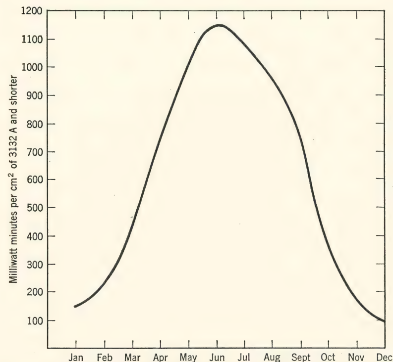
FIG. 14. Integrated monthly ultraviolet of wavelength less than 3132 Å throughout the year. (W. W. Coblenz and R. Stair, J. Research Natl. Bur. Standards , 33 , 21, 1944.)
