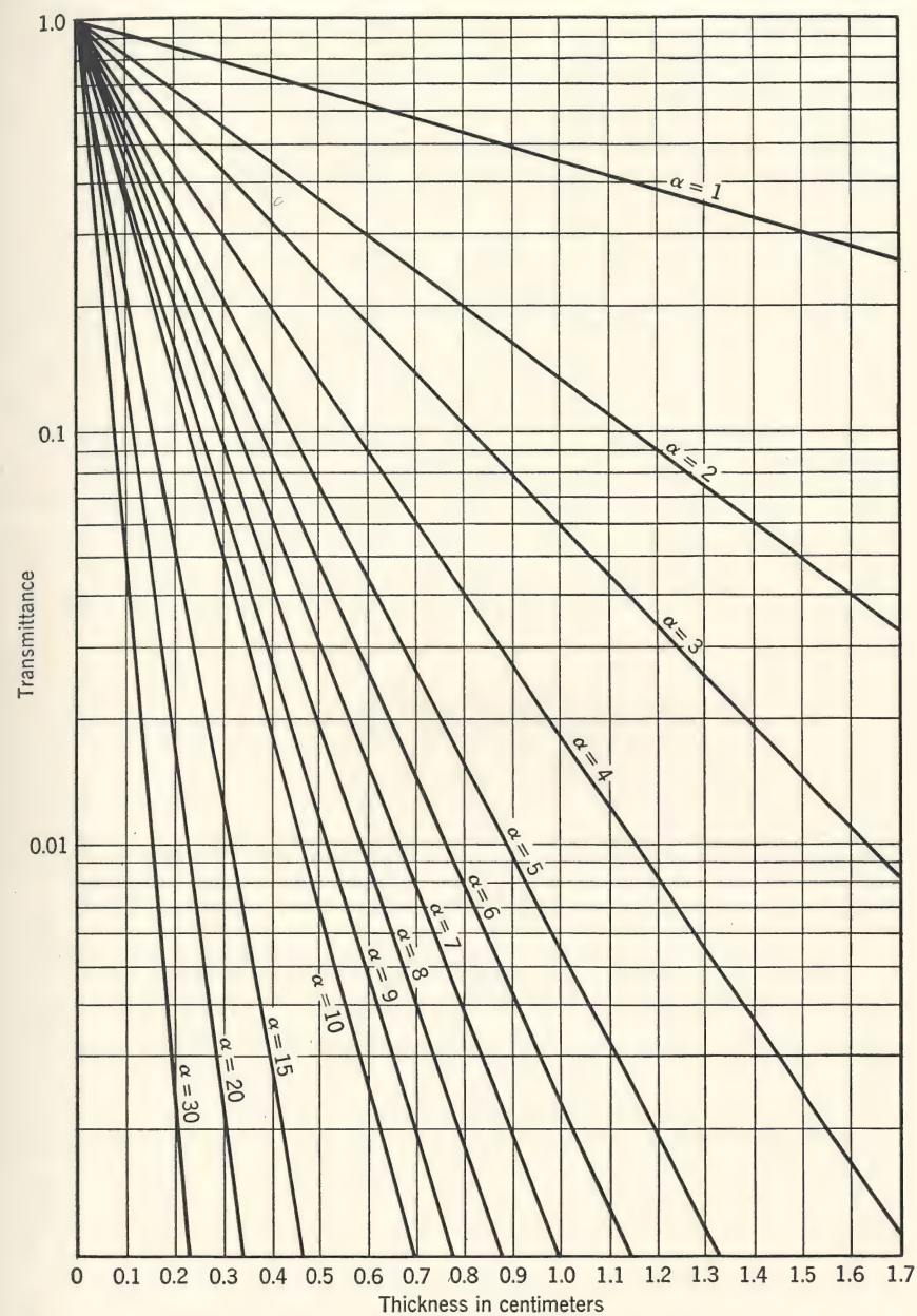
FIG. 2. Transmittance as a function of thickness for various values of absorption coefficient.
