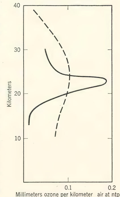
FIG. 6. Ozone concentration of the atmosphere as a function of altitude. These curves show the extremes measured by different observers.
