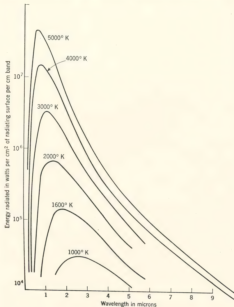
FIG. 2. Energy distribution for a black body at various temperatures.
