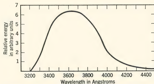
FIG. 24. Emission spectrum of cerium-activated calcium phosphate phosphor. (H. Froelich, Trans. Electrochem. Soc. , 91 , 241, 1947.)
