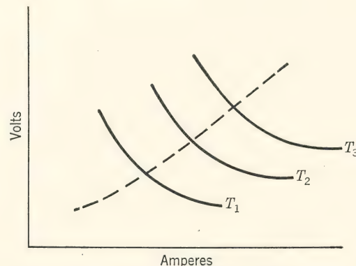
FIG. 5. Static and dynamic arc characteristics.
