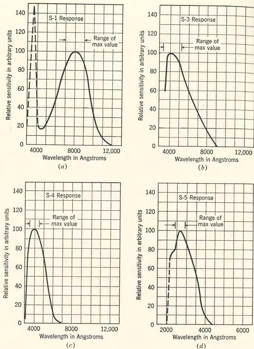
FIG. 8. Spectral response curves of various commercial phototubes. a-d. RCA Bulletin CRPS-102-A.
