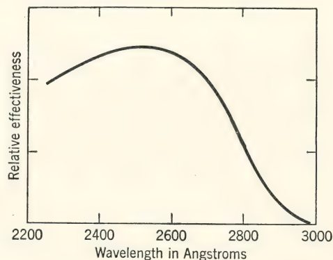
FIG. 15. Excitation spectrum of willemite.
