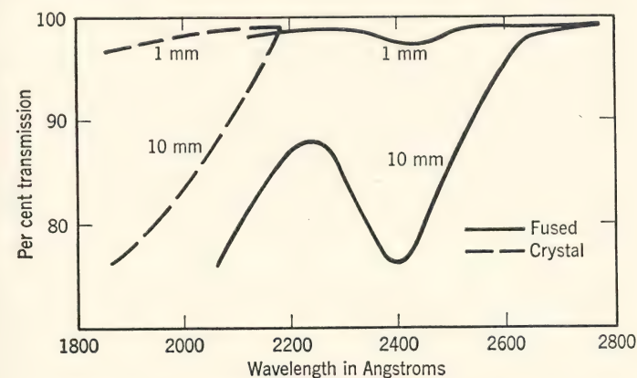
FIG. 7. Transmission for crystal and fused quartz. (A. Schraub, Physik. Z. , 43 , 64, 1942; T. Lyman, Spectroscopy of the Extreme Ultraviolet , Longmans, Green and Co., New York.)
