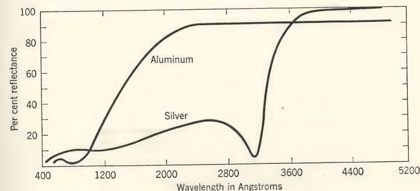
FIG. 3. Reflection from evaporated films of silver and aluminum. (J. B. Sabine, Phys. Rev. , 55 , 1064, 1939.)
