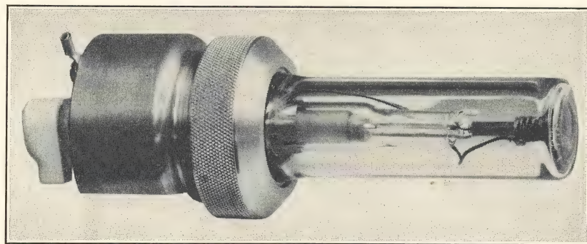
FIG. 18. Water-cooled high-pressure (110 atmospheres) mercury arc showing lamp in water jacket. (Courtesy of General Electric Co.)
