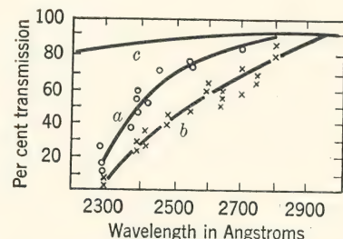
FIG. 23. Transmission through 400 meters of air. a . Good visibility. b . Poor visibility. c . Calculated. (L. H. Dawson, L. P. Granath, and E. O. Hulburt, Phys. Rev. , 34 , 136, 1929.)
