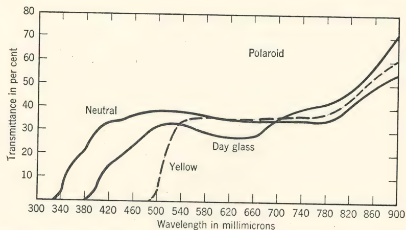
FIG. 22. Spectral transmittance of Polaroid glasses. Neutral Polaroid, thickness 5.20 mm. Polaroid Day glass, thickness 2.28 mm. Yellow Polaroid, thickness 5.65 mm. (Natl. Bur. Standards Circ. 471, 1948.)
