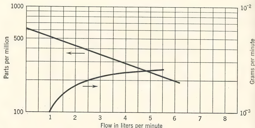
FIG. 13. Concentration of ozone produced from oxygen by low-pressure mercury quartz arc as a function of rate of flow of oxygen. (L. R. Koller, J. Applied Phys. , 16 , 816, 1945.)
