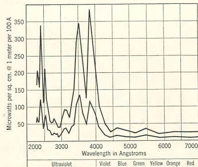
FIG. 37. Spectral energy distribution of carbon arc with cobalt-cored carbons (National K). Upper curve, 60 amperes alternating current, 50 volts across arc. Lower curve, 30 amperes alternating current, 50 volts across arc. ( National Carbon Co. Catalog , Section A-4300.)
