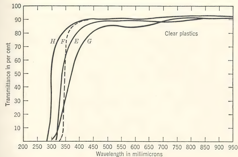
FIG. 17. Spectral transmittance of several clear plastics. E. Cellulose nitrate, thickness 0.80 mm. F. Cellulose propionate, thickness 0.23 mm. G. Ethyl cellulose, thickness 0.79 mm. H. Polystyrene, thickness 0.45 mm. ( Natl. Bur. Standards Circ. 471, 1948. )
