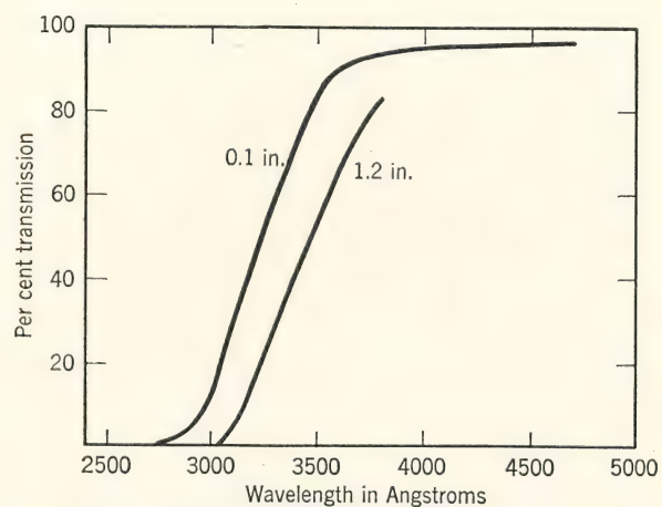
FIG. 16. Transmission of Plexiglass. (Calculated from Rohm and Haas Catalog .)
