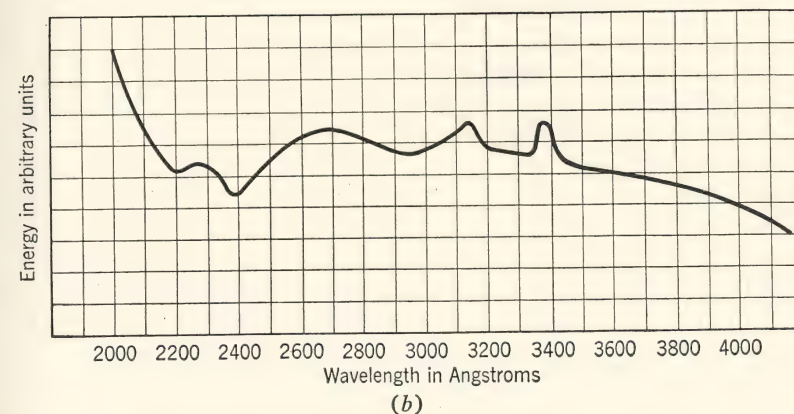
FIG. 28. a . Energy from hydrogen arc available through monochromator. Arc operated at 3.4 amps, 70 volts direct current. (Courtesy of E. A. Taft and L. Apker.) b . Energy distribution in hydrogen-arc spectrum. (Calculated from Taft and Apker.)
