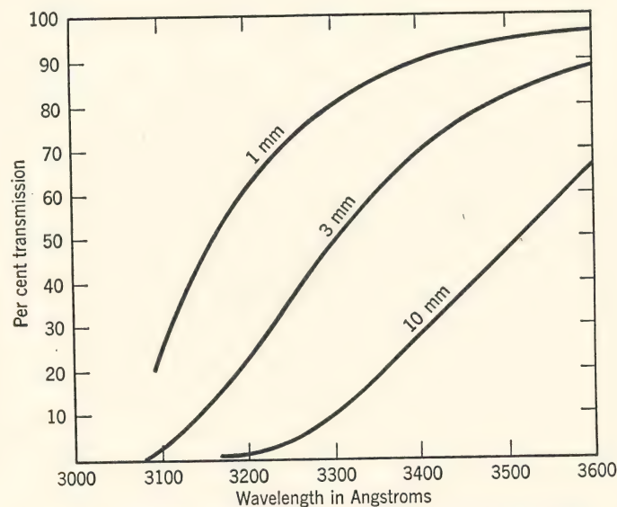
FIG. 4. Transmission for various thicknesses of window glass.
