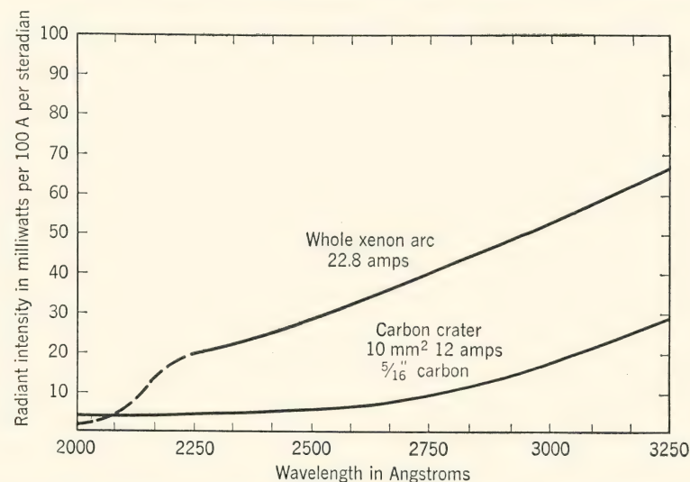
FIG. 29. Comparison of spectrum of high-pressure xenon arc with corresponding area of carbon-arc crater. (W. A. Baum and L. Dunkelman, J. Optical Soc. Am. , 40, 782, 1950.)
