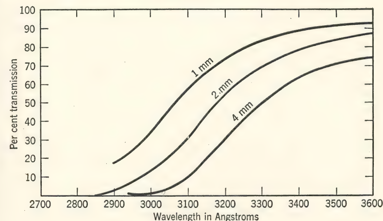
FIG. 5. Transmission for various thicknesses of Pyrex clear chemical glass No. 774.
