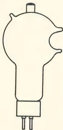
FIG. 20. Thin glass window in phototube bulb.
