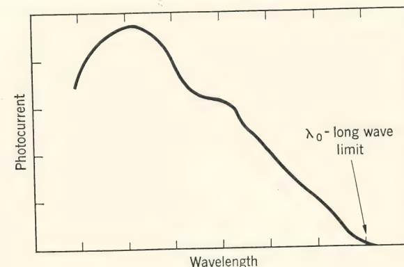
FIG. 6. Phototube spectral response curve.
