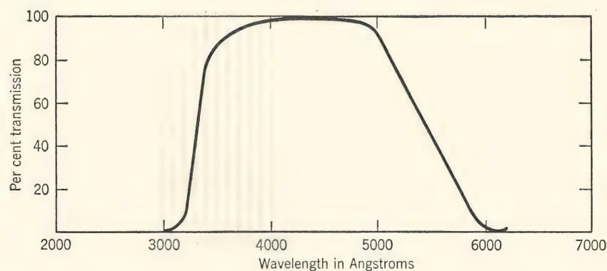
FIG. 15. Transmission of cupric sulfate: 5 cm of solution of \text{CuSO}_4 \cdot 5\text{H}_2\text{O} , 100 grams per liter. (M. Kasha, J. Optical Soc. Am. , 38 , 929, 1948.)
