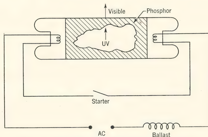
FIG. 14. Construction and circuit for fluorescent lamp.
