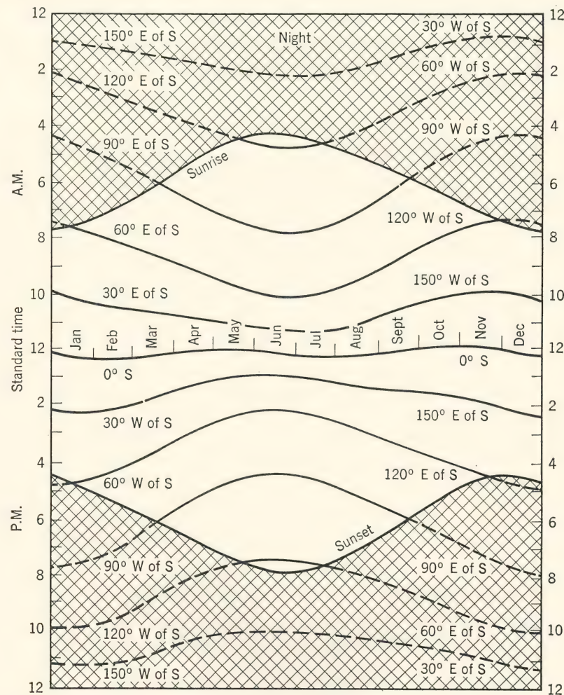
FIG. 18. Chart for determining incidence of sunshine on any vertical plane at 45^\circ north latitude. (F. Benford and J. E. Bock, Trans. Illum. Eng. Soc. , 34 , 200, 1939.)
