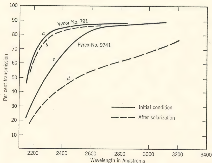
FIG. 11. Effect of solarization on Vycor and Pyrex glasses. (M. E. Nordberg, J. Am. Ceram. Soc. , 30 , 174, 1947.)
