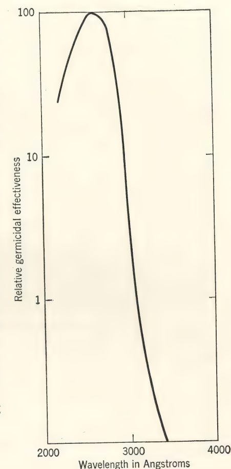
FIG. 3. The bactericidal effectiveness curve showing the relative effectiveness of various wavelengths in killing bacteria. (M. Luckiesh, Germicidal, Erythema and Infrared Energy , D. Van Nostrand Co., New York, 1946.)
