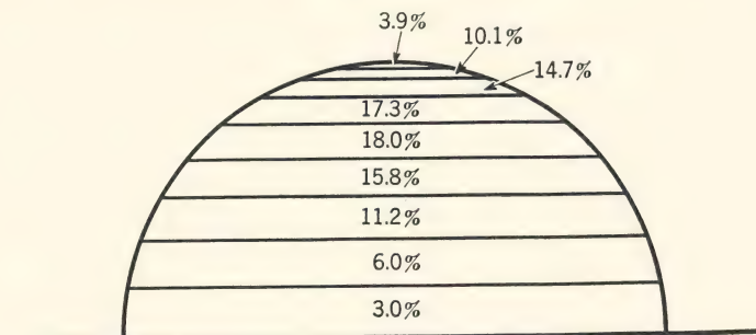
FIG. 9. Intensity of radiation falling on a horizontal surface from different 10-degree zones of the sky. (M. Luckiesh, Germicidal, Erythemat and Infrared Energy , D. Van Nostrand Co., New York, 1946, page 52.)
