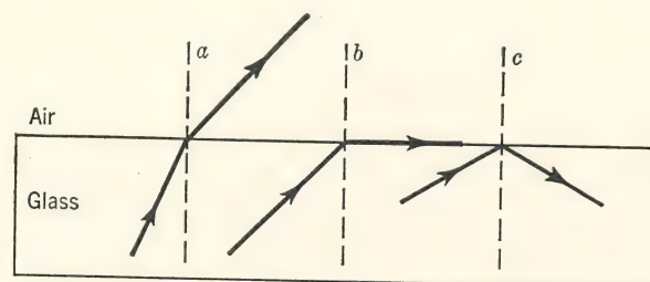
FIG. 14. Total internal reflection.
