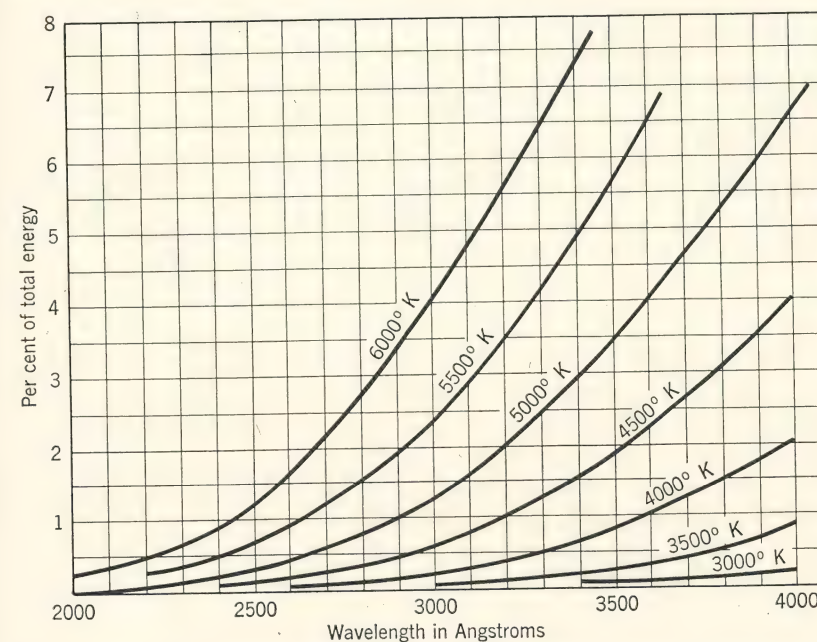
FIG. 3. Per cent of total energy radiated by a black body between wavelength 0 and wavelength \lambda . (L. L. Holladay, J. Optical Soc. Am. , 17 , 329, 1928.)
