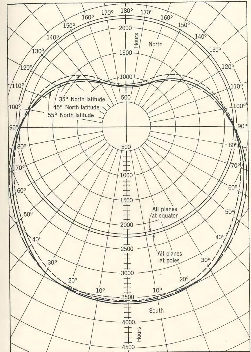
FIG. 19. Total annual hours of sunshine received on vertical surfaces facing various points on the horizon at different latitudes. (F. Benford and J. E. Bock, Trans. Illum. Eng. Soc. , 34 , 200, 1939.)
