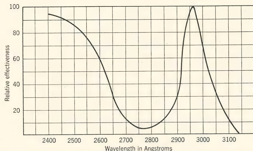
FIG. 8. The erythema curve showing the relative effectiveness of equal amounts of energy in different parts of the spectrum in producing erythema. (M. Luckiesh, L. L. Holladay and A. H. Taylor, Trans. Illum. Eng. Soc. , 26 , 703, 1931.)
