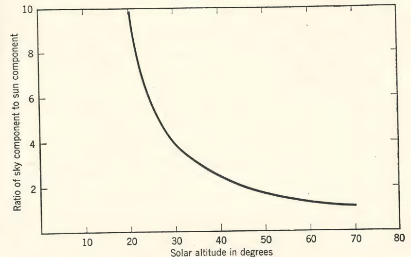
FIG. 8. Ratio of sky component to direct solar radiation as a function of solar altitude. (M. Luckiesh, Germicidal, Erythemat and Infrared Energy , D. Van Nostrand Co., New York, 1946.)
