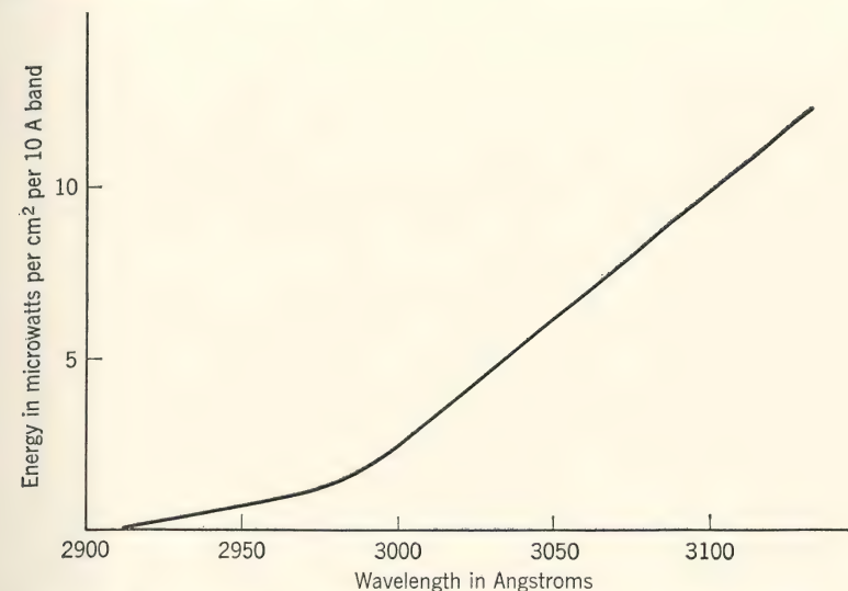
FIG. 10. Energy distribution in the solar spectrum at Tucson, Arizona.
