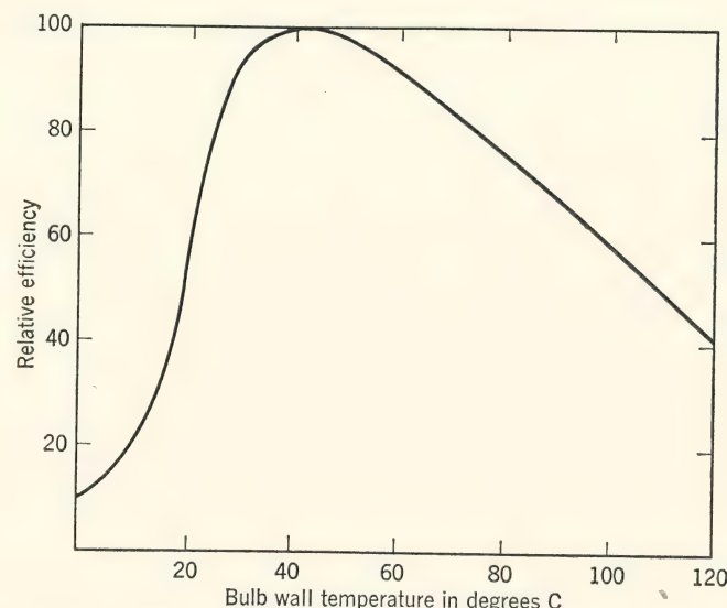
FIG. 19. Relative efficiency of production of mercury resonance radiation (2537 Å) for different temperatures of the tube wall for a discharge tube 1 in. in diameter. (W. E. Forsythe, Denison Univ. Bull. XXVI, 13, 1941.)
