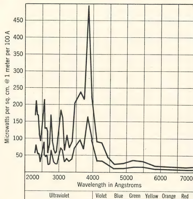
FIG. 34. Spectral energy distribution of carbon arc with carbons containing iron, nickel, aluminum, and silicon in the core (National C). Upper curve, 60 amperes alternating current, 50 volts across arc. Lower curve, 30 amperes alternating current, 50 volts across arc. National Carbon Co. Catalog, Section A-4300. )
