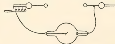
FIG. 6.—Shows an X-ray tube connected in series with a multiple spark gap, attached to a Static Machine.
