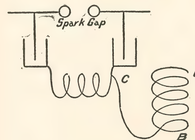
FIG. 19.—OUDIN RESONATOR.
