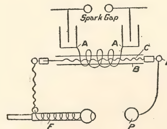
FIG. 18.—Above figure illustrates a Tesla Transformer. As designed by Nicola Tesla, the two coils were insulated from each other with oil. Dr. Henry G. Piffard modified this construction for medical use by using a hard rubber or glass tube to separate the primary from the secondary windings. The current from the terminal "D" has the same character as the current from the top of the resonator. He also found that, by a second winding on a separate handle and attaching it to one terminal of the Tesla and connecting the patient with the other terminal of the Tesla, a still longer spray could be obtained. This he called an intensifying handle.
