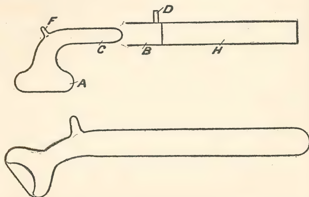
FIGS. 23 AND 24.—Illustrate the ordinary plain vacuum electrode.
