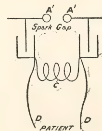
FIG. 28.—The above figure illustrates the essential parts necessary to obtain the d'Arsonval high-frequency current. Terminals marked "spark gap" are connected with a source of high voltage current, "A" represents a Leyden jar, "C" a coil of very heavy copper wire, connecting the outside of the Leyden jars together. The frequency of the current is dependent upon the following factors: First, amount of tin foil surface; second, length and size of coil which joins the outer coatings of the Leyden jars together. The number of times that a spark passes between "A" and "A" does not change the frequency of the current. The less tin foil used and the shorter and larger the wire which joins the jars together, the higher will be the frequency of the current. When the patient is connected with the terminals "D D," he receives what is known as the d'Arsonval shunt or derived high-frequency current.
