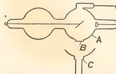
FIG. 38.—"A" represents a bulb of lead glass. "B" a window of soda glass which allows X-rays to be passed through it. "C" a lead glass shield which fits on to the projection of the main tube, thus confining the rays to an area equal to the opening at the end of "C." This tube was designed by Dr. H. G. Piffard, and is intended to protect the operator as well as the parts of the patient it is desired not to ray.
