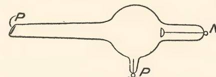
FIG. 41.—A modification of the Derma tube designed by Doctor Caldwell. The rays from this tube are much more penetrating than from the Derma tube, owing to the fact that the cathode stream strikes on a platinum plate at the end of the projection. This tube is intended particularly for treating cavities. Owing to it becoming very hot, however, a glass jacket containing water is required which reduces its efficiency very much.
