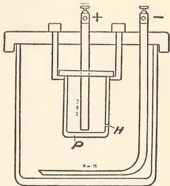
FIG. 11.—Represents the Caldwell Interrupter. This consists of an inner porcelain jar "P" having one or more holes through it "H." In the outer jar is placed a lead electrode marked "—" In the inner jar is placed another electrode marked "+." The solution used is sulphuric acid and water. When the current is passed from the inner jar to the outer jar through "H" the current is interrupted. This type is not used as much as formerly owing to the breakage of the inner jars and to the fact that the hole "H" gradually wears a little larger, and after a while becomes so large that the current does not interrupt.
