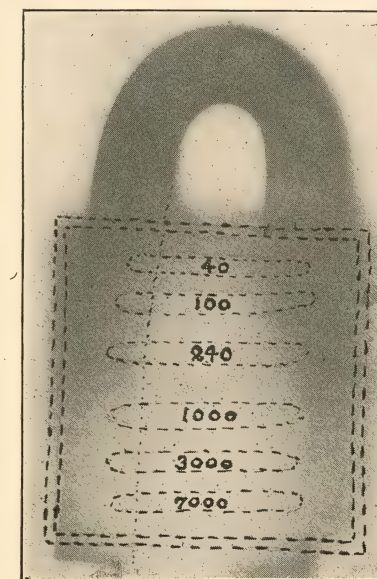
FIG. 8.—Radiograph showing Degrees of Penetration of a thick sheet of Lead and a Steel Magnet by Tubes of Radium of Different Radioactivities.
