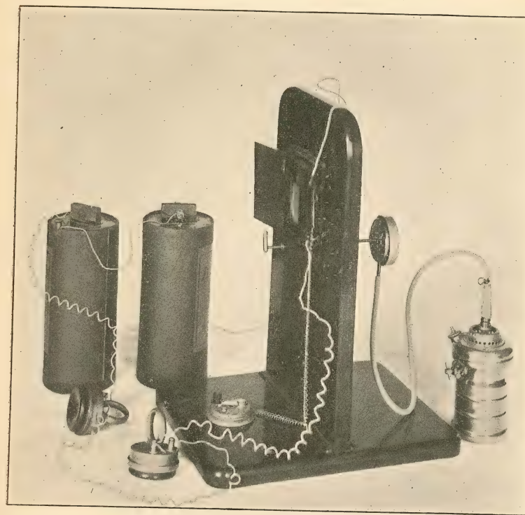
FIG. 20.—Manometric Acetylene Flame Transmitter with Selenium Cell, etc. —(a battery of about 24 volts employed.)
