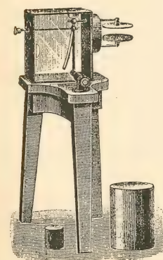
FIG. 5 —Curie's Electroscope for the study of Radio-activity
