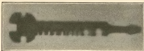
FIG. 9.—Radiograph of Steel Tool made by Radium Acting Through Two Thick X-ray Plate Envelopes.
