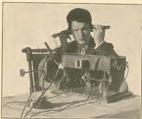
FIG. 27.—Mr Ernest Ruhmer Listening to his Photographophone.
