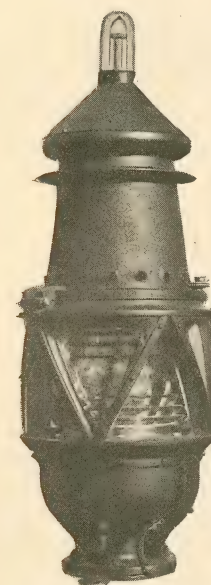
FIG. 23.—Pintsch Gas Buoy Controlled by a Ruhmer Selenium Cell, Battery and Switch Mechanism.
