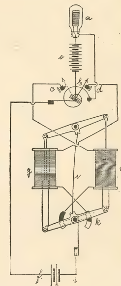
FIG. 24.—Diagram of Circuits of "Selenium" Buoy.
