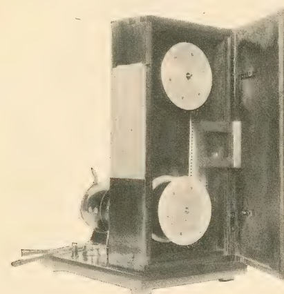
FIG. 26.—Showing Interior of Ruhmer's Photographophone.
