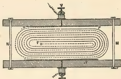
FIG. 19.—Mercadier's cell (block and dotted lines represent the two ribbons of brass).
