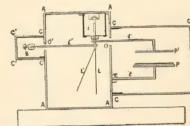
FIG. 5 —Curie's Electroscope for the study of Radio-activity
