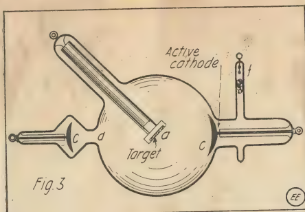
One Form of Commercial High-Frequency X-Ray Bulb of the Single-focus Type, Utilizing An Active Cathode "C", Also a Small Cut-off Cathode "C'". The Inverse Cathodic Stream from "C'" Is Choked Off and Dispersed by the Constricted Glass Neck "D", Which Acts As a Valve.
