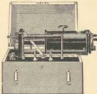
Dr. Goelet's latest Induction Apparatus, made by The Kidder Mfg. Co.
