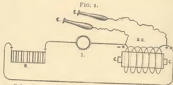
B. Galvanic battery. I. Interrupter. S.C. Secondary coil. —X and +X. Terminals of coil. C. Core and primary coil. E. E. Electrodes.
