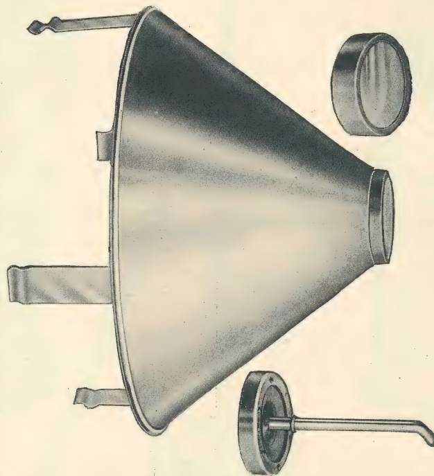
The Caps in which are fixed the Quartz Lens and the Quartz Rod fit over the mouth of the Concentrator Hood. The spring metal straps on the left snap over the rim of the Reflector Hood of the Lamp.
