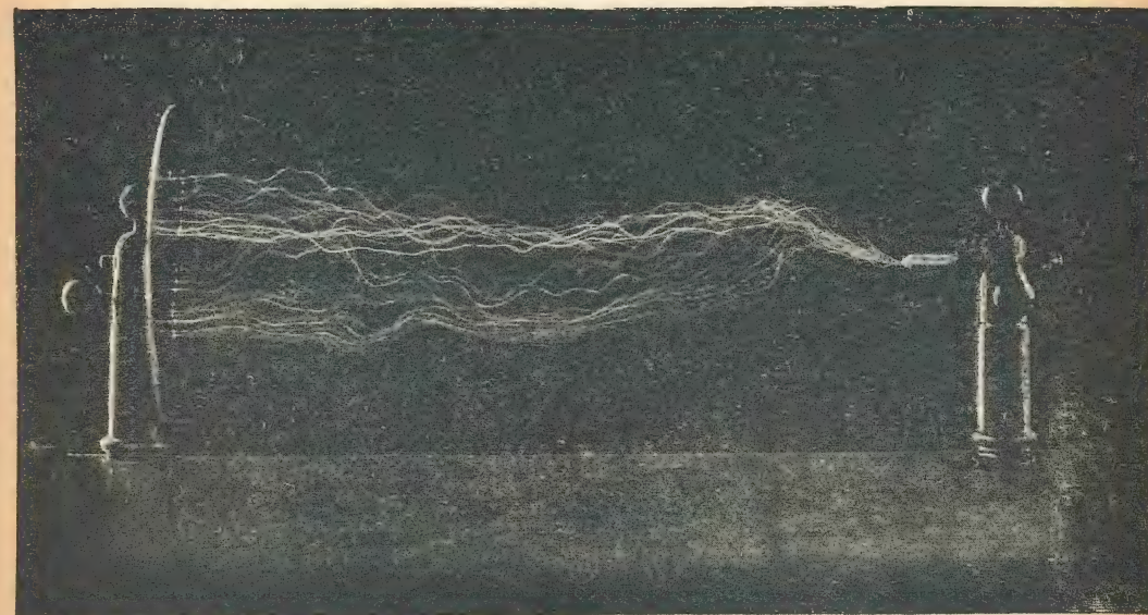
This illustration shows the discharge obtained from a coil connected with a mercury jet (turbine) interrupter. The exposure was \frac{1}{10} second. An illustration of the discharge obtained with a Wehnelt electrolytical interrupter will be found on page 58.
