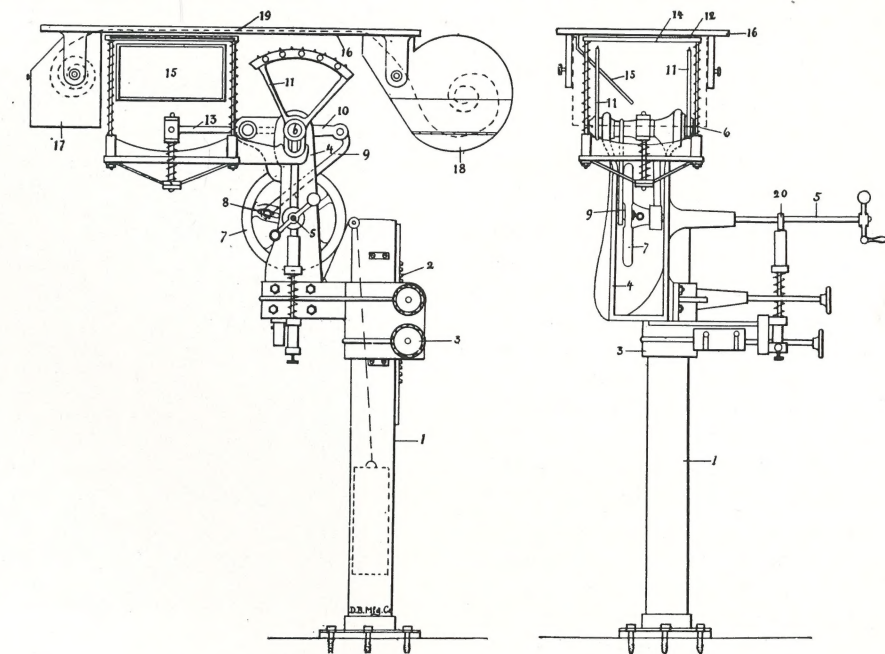
Fig. 1. Drawing of Roentgenocinematographic Apparatus.
