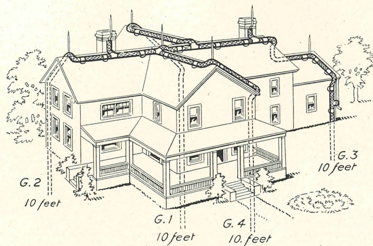
HOUSE Detailed Electra Installation
