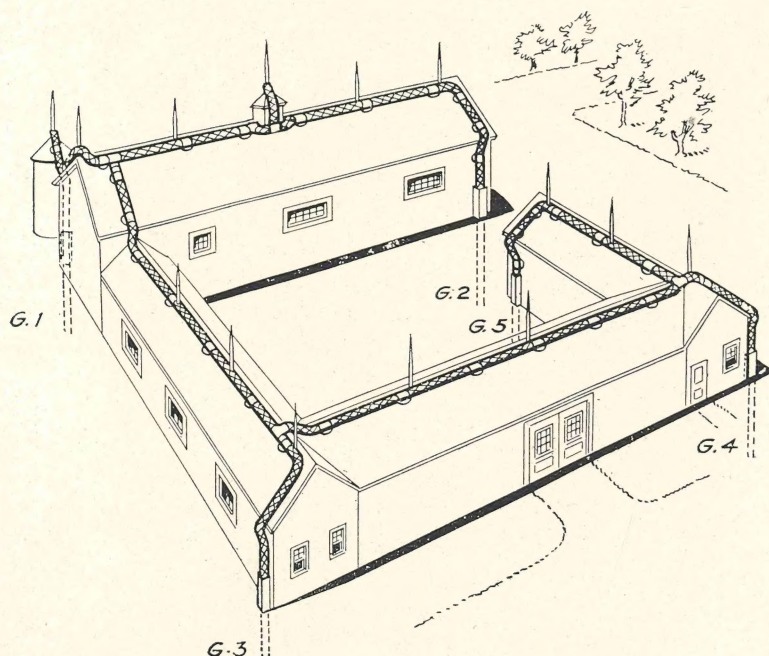
CHAIN OF CATTLE BUILDINGS WITH SILO Detailed Electra Installation
