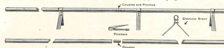
Method For Increasing Length of Copper Upright Points
