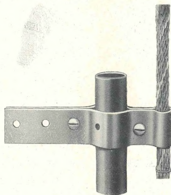
Adjustable Copper Bonding Clamp for connecting to underground water-pipes and other metals.
