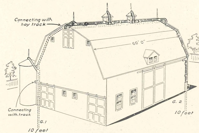
BARN Detailed Electra Installation
