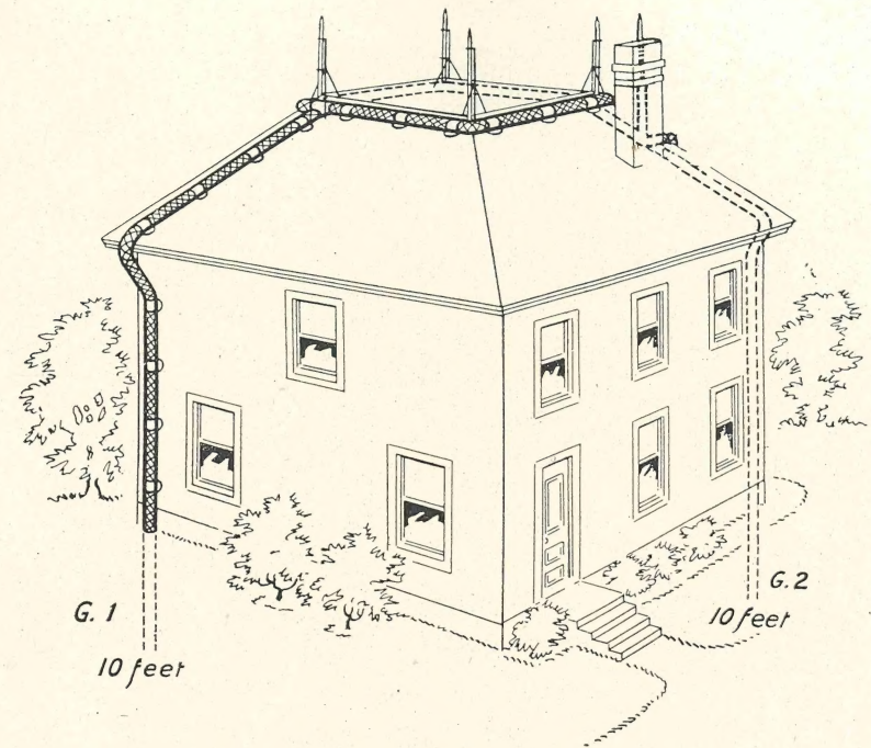
HOUSE Detailed Electra Installation
