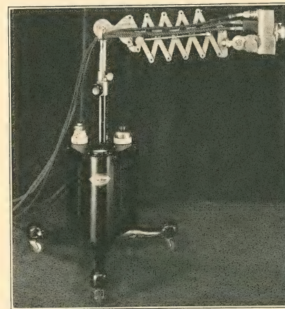
Water-cooled lamp used for compression treatments.
