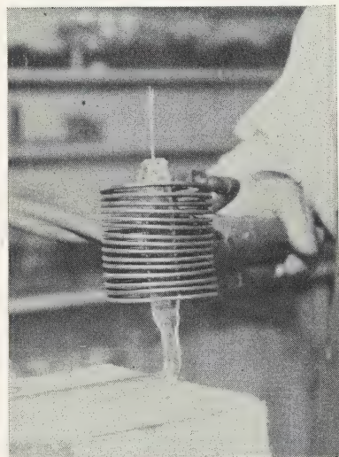
FIG. 78.—Heating electrodes by external bombarding coil, connected to high-frequency generator.
