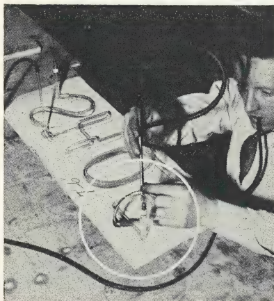
Fig. 57.—Sealing electrode to letter.
