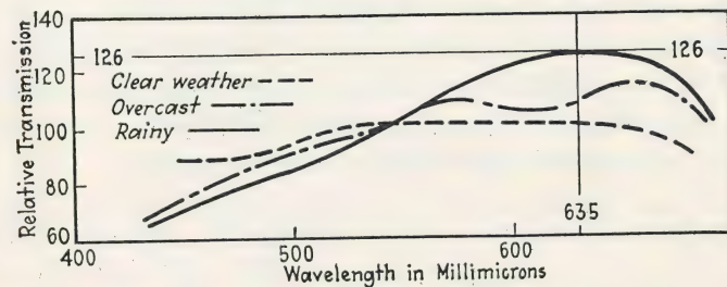
FIG. 11.—Relative transmission of different colors under various weather conditions. At 635 millimicrons, the wave length of neon light, the transmission is highest in the poorest weather.
