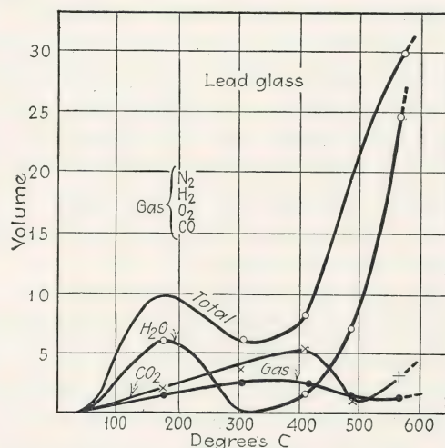
FIG. 76.—Curves showing gases released from lead glass when heated to various degrees of temperature. The following symbols are used: H 2 O water vapor; CO 2 carbon dioxide; "gas" N 2 nitrogen; O 2 oxygen; CO carbon monoxide. Note that above 400°C., the released gas comes from within the glass structure. (Curve due to Sherwood, Westinghouse Electric and Manufacturing Company.)
