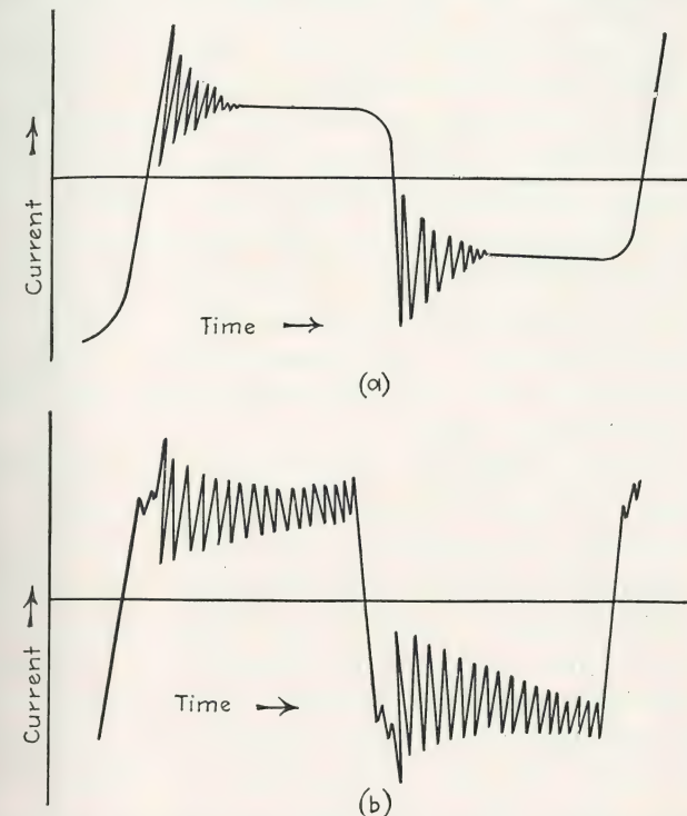
FIG. 20.—(a) Secondary current of neon transformer, properly loaded. (b) Current when transformer is overloaded. The tubing is then near the flickering point.
