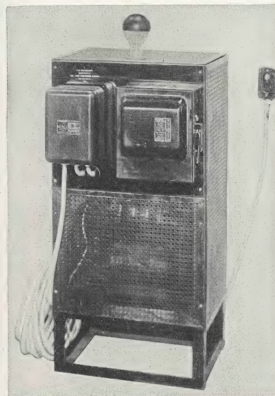
FIG. 72.—Bombarding transformer, showing magnetic switch mounted on casing, and push-button control (at end of BX cable).
