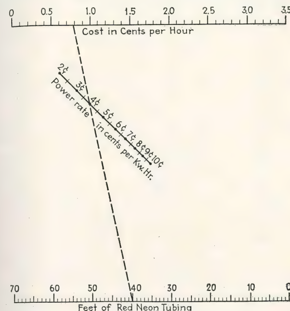
FIG. 36.—Chart for determining the approximate cost per hour. Place a rule so that it connects the number of feet of tubing and the power rate per kilowatt-hour. The point where the rule intersects the top scale will indicate the approximate cost in cents per hour. In the example given by the dotted line, 40 feet of tubing at 4 cents per kilowatt-hour is found to cost about 0.8 cent per hour.
