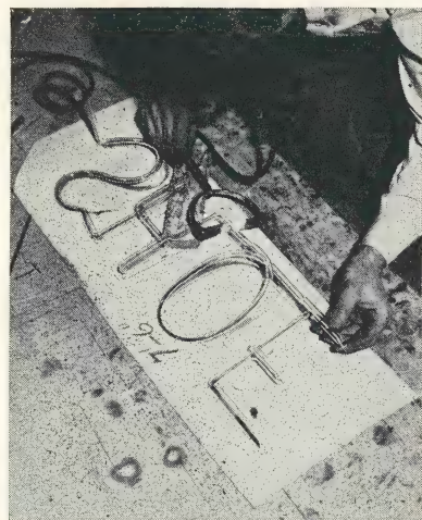
FIG. 53.—Glass blower splicing two letters with hand torch over asbestos layout.
