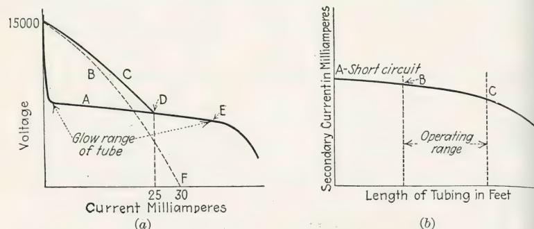
FIG. 19.—(a) Curves illustrating the action of a neon-tube transformer. A is the tube-characteristic curve showing high initial break-down voltage. B, transformer-regulation curve (if load were non-capacitive). C, actual transformer-regulation curve, shifted by capacitance of tubing. D, stable operating point, due to current being limited by transformer regulation. Operating current at this point is approximately 17 per cent less than the short-circuit current shown at point F. F, short-circuit current from high-voltage winding. (b) The current regulation curve of a typical neon transformer. Between points B and C is the safe operating range.
