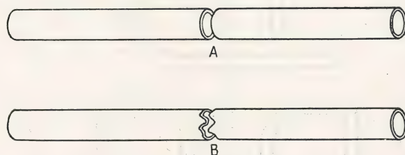
FIG. 51.—(A) A properly made cut in glass tubing. (B) A jagged cut, which cannot be used for a successful seal.
