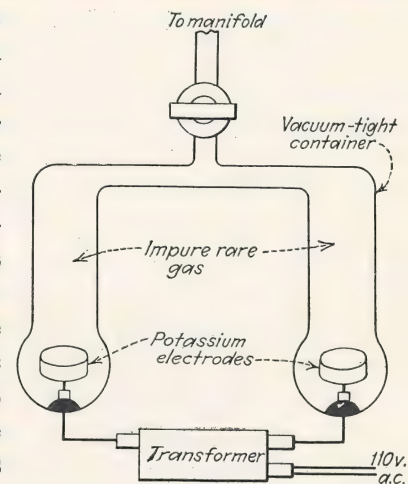
FIG. 101.—Potassium purifier for reclaiming impure rare gas.
