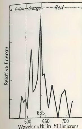
FIG. 9.—Relative light energy from a neon-filled tube. The light energy is confined primarily to the red and orange regions.
