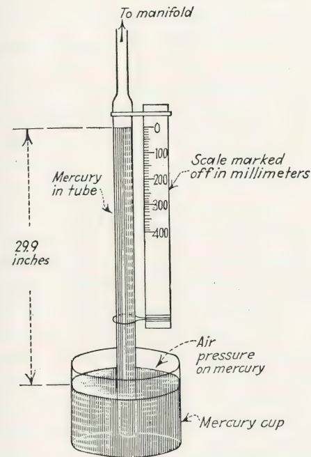
FIG. 65.—Straight gauge.
