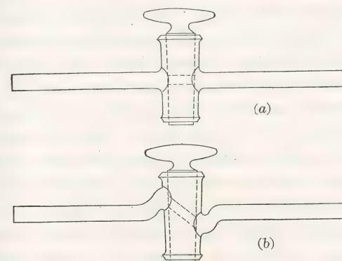
FIG. 61.—Two types of stopcocks: (a) Straight bore, (b) Oblique bore.
