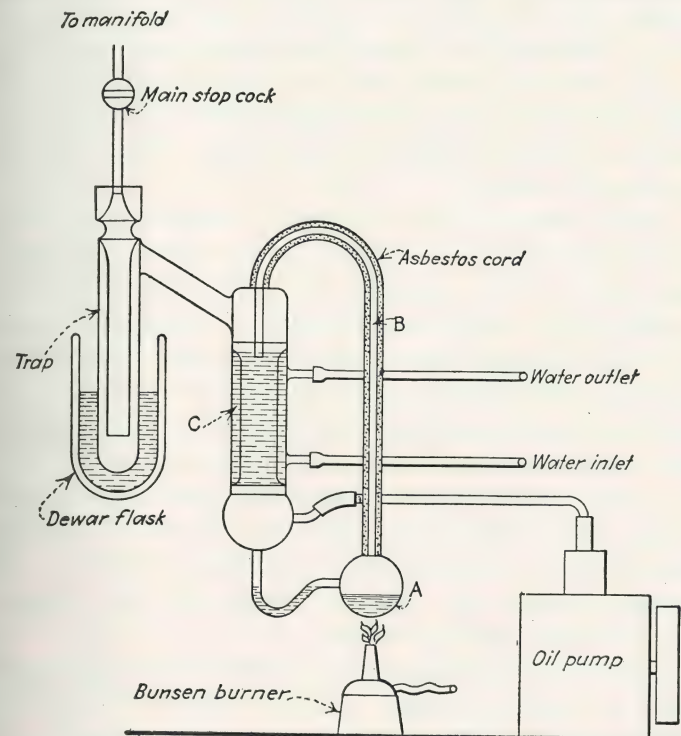
Fig. 63.—Water-cooled mercury condensation pump. A. Mercury reservoir. B. Asbestos covered vapor chamber. C. Cooling chamber.
