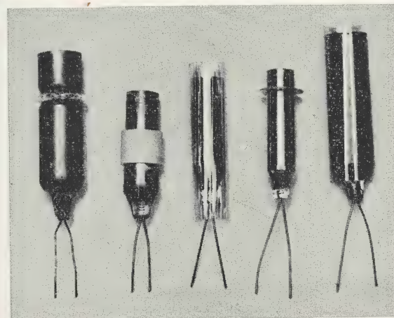
FIG. 13.—Electrode insulation. Left to right: glass beads, ceramic collar, corrugated mica, mica ring, and mica cylinder.
