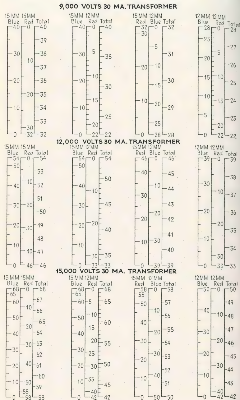
FIG. 104.—Chart for determining the combinations of red and mercury tubing which may be run from a single transformer. The use of the chart is explained in the text on the opposite page.
