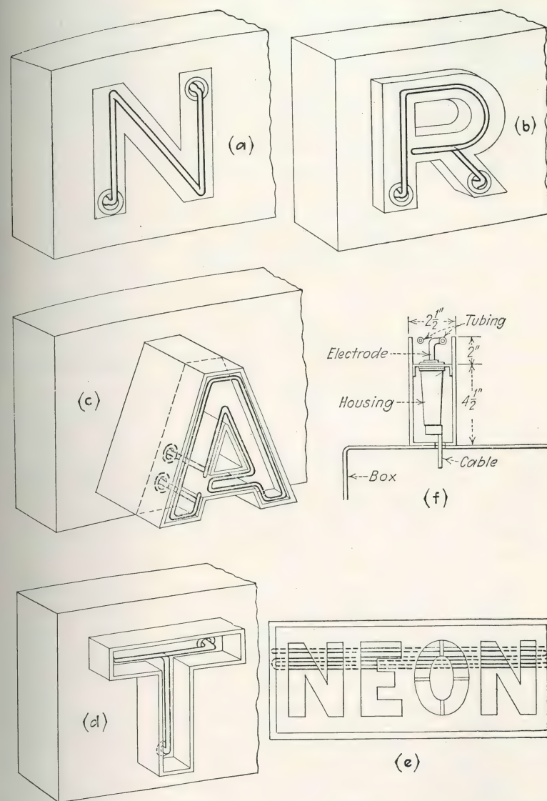
FIG. 33.—(a) The flat painted letter. (b) The raised letter. (c) Raised letter with shallow channel. (d) The channel letter. (e) The cut-out letter. (f) Section through a raised-channel letter showing electrode housing in place.
