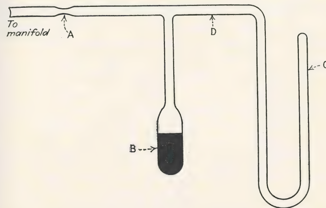
FIG. 102.—Method of constructing a mercury U gauge. The tube is pumped out thoroughly, sealed off at A, and the mercury in B poured into the U section until it fills the arm C. The gauge is then cut off and sealed to the manifold in the usual manner, at D. Tube and mercury should be heated with a soft flame before pumping.
