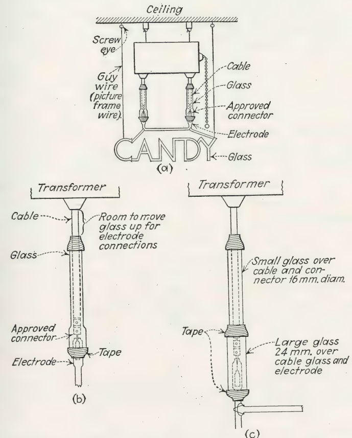
FIG. 85.—(a) Hanging transformer and skeleton sign. Note method of protecting electrodes and cable with glass tubing. (b) Detail of glass sleeve for electrode and cable protection. (c) Two pieces of tubing may be used in place of the one shown in (b).
