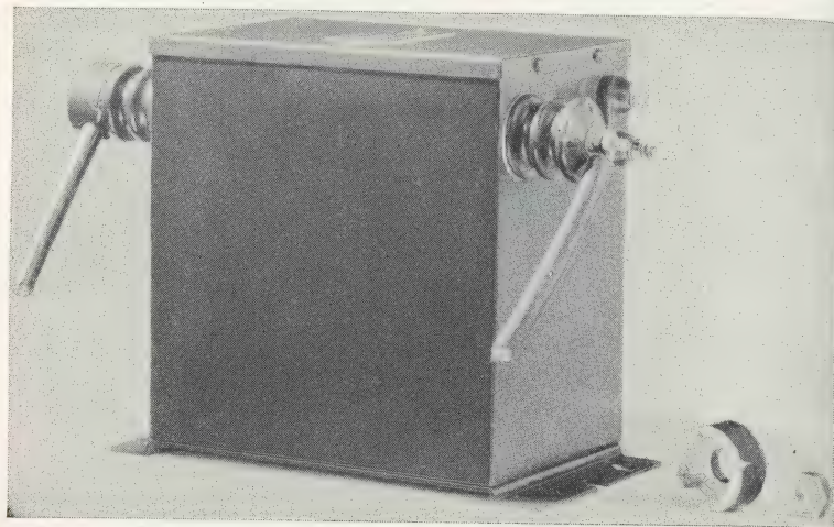
Fig. 24.—A 15,000-volt transformer of the high-power-factor type. The case contains a capacitor for improving the power factor.
