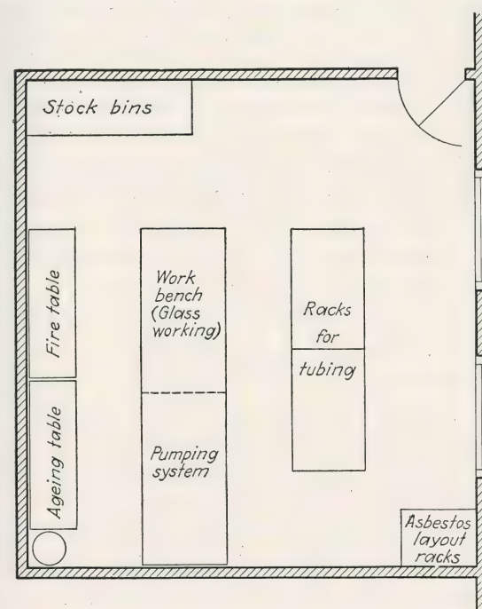
FIG. 7.—Typical neon-tube manufacturing plant layout.
