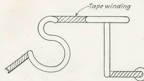
FIG. 84.—Blocking out crossovers with tape.
