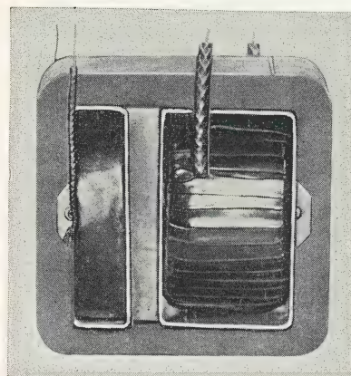
FIG. 21.—Internal construction of low-voltage type (2000 to 5000 volts) neon transformer. Only one magnetic shunt is used, whereas two are usually used in the higher-voltage types (see Fig. 17).
