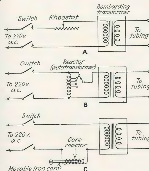
FIG. 73.—Three methods of controlling the bombarding voltage. (A) Rheostat control. (B) Autotransformer. (C) Reactor with movable iron core.
