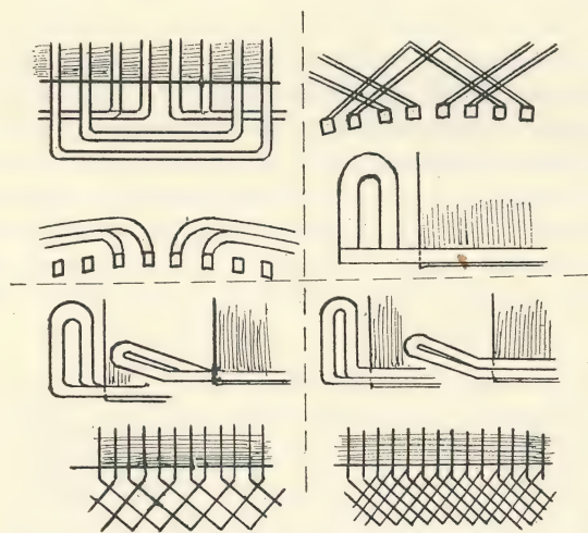
FIG. 11—VARIOUS TYPES OF EARLY STATIONARY ARMATURE WINDINGS
