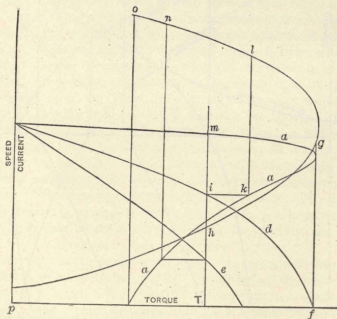
Fig. 7—STARTING CONDITIONS WITH VARIABLE SECONDARY RESISTANCE
