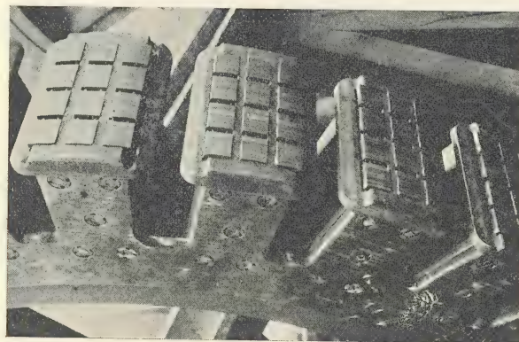
FIG. 17—GRID DAMPERS ON FIELD POLES
