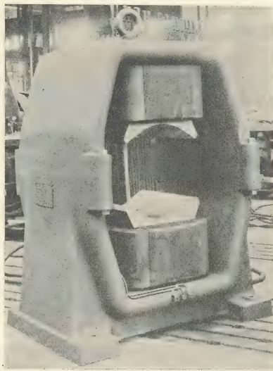
FIG. 20—FIELD OF EARLY ROTATING ARMATURE TURBO-GENERATOR
