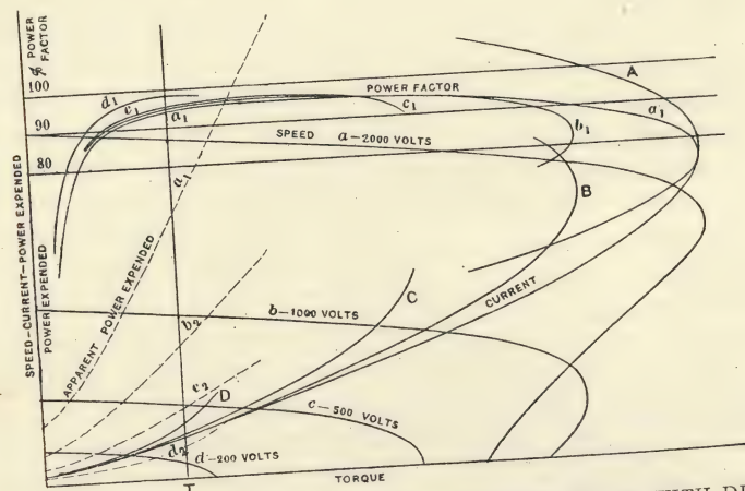
FIG. 18—PERFORMANCE CURVES OF POLYPHASE MOTOR WITH DIFFERENT ALTERNATIONS AND ELECTRO-MOTIVE FORCES.
