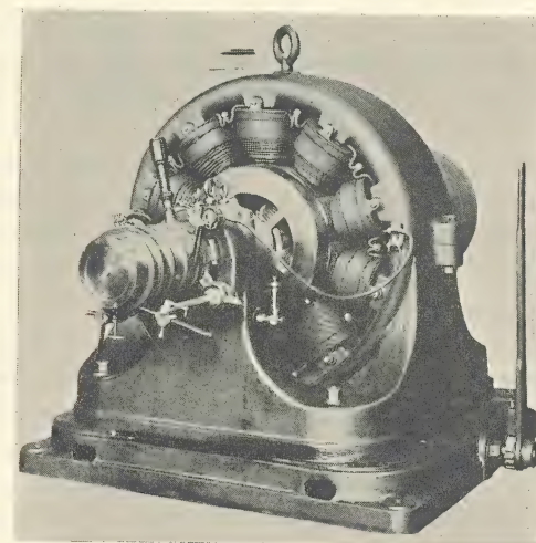
FIG. 5—EARLY WESTINGHOUSE 60 KILOWATT ALTERNATOR WITH COMPENSATING WINDING
