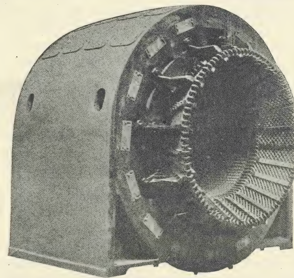
FIG. 31—STATOR OF LARGE MODERN TURBO-ALTERNATOR
