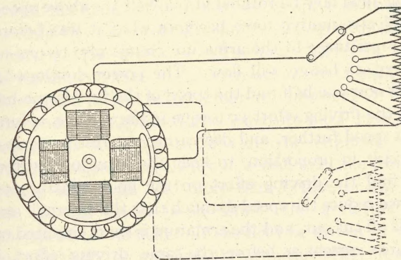
FIG. 2—DIAGRAM OF TWO-PHASE ALTERNATING-CURRENT GENERATOR, ROTATING-FIELD TYPE.
