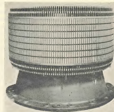
FIG. 10—STATOR OR ARMATURE OF NIAGARA ALTERNATOR
