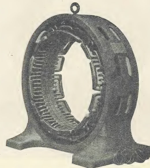
FIG. 14—DETAIL VIEW OF THREE-PHASE CONCENTRIC WINDING
