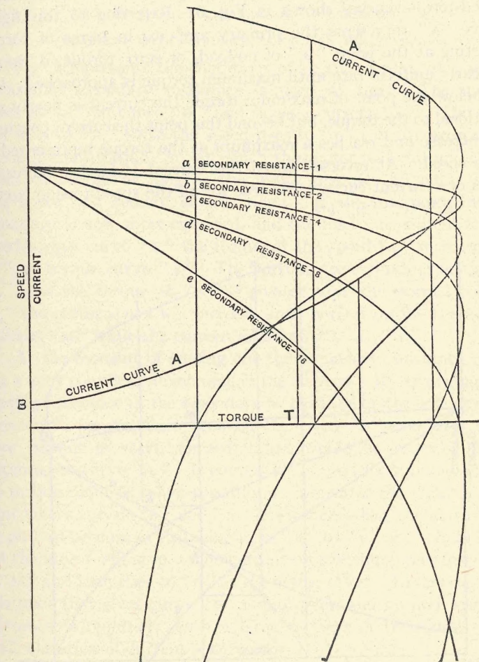
FIG. 6—SPEED-TORQUE AND CURRENT-TORQUE CURVES OF POLYPHASE MOTOR WITH SECONDARIES OF DIFFERENT RESISTANCE
