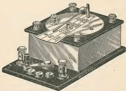
Galvanic Interrupter.
