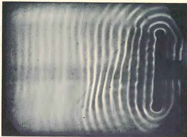
A. Ripples passing over a rectangular piece of glass laid on the floor of the ripple tank; showing the temporary change of alignment. (p. 69)
