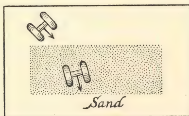
Fig. 21. The dotted portion of the diagram represents sand spread upon a table. The pair of freely running wheels is rolled towards the sanded area and swings round on reaching it.
