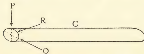
Fig. 84. A steel rod of elliptical section sounds a higher note when struck at Q than at P, the latter being on the flatter side. When struck at R, it emits both the high note of Q and the low note of P, but not a note of intermediate pitch.
