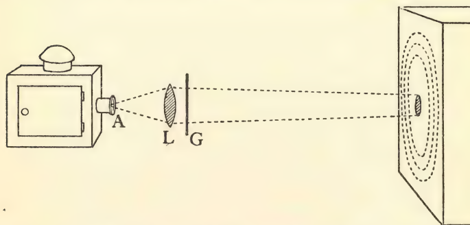
Fig. 75. Light from the lantern issues through a small opening at A and is focused by the lens L upon a hole in the side of the box shown on the right of the diagram. Passing through the hole into the box, which is blackened inside, it is lost to view. The glass sheet G covered with fine dust or drops of moisture causes the halo which appears on the side of the box: the disappearance of the main beam allows the relatively faint halo to be easily visible.
