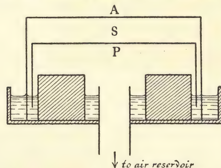
Fig. 110. This drawing shows the main principles of Wilson's expansion apparatus. Within the chamber of which the lid A is made of glass, a piston P can slide up and down. The space below P is connected to a reservoir of air the pressure of which can be varied. It is in the space S that the tracks are observed. It is cut off from the space under P and from the outside air by a water seal as used in a gasometer. If the pressure under P is raised a little, P rides up into the position shown. If then the pressure under P is reduced very suddenly, P comes down with a thud: the air in S expands and is chilled. If there are any tracks of electrons or alpha particles, fog settles on them. They can then be photographed in a bright light.
