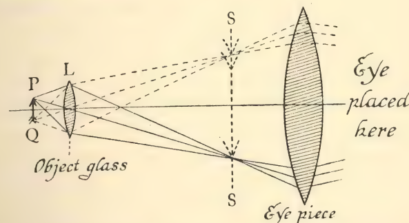
Fig. 33. The plan of the microscope. The brightly illuminated object P Q, scatters rays of light from which the lens L, called the object glass, forms an image at s s, much larger than the object. This is examined by a second lens called the eyepiece in the manner of the previous drawing, Fig. 32.
