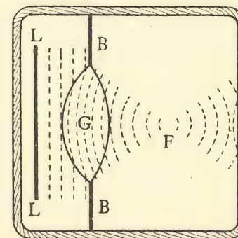
Fig. 22. The ripple tank is seen from above. A sheet of glass G cut in the form of a section of a lens is laid on the floor of the tank, diminishing the depth of the water which is usually about a quarter of an inch. The ripples travel more slowly in the shallow water. Thus they are made to converge upon a point F ; after passing through F they diverge. The ripples are started by a lath L which dips in and out; the barriers B B prevent the ripples from passing by the sides of the lens.
