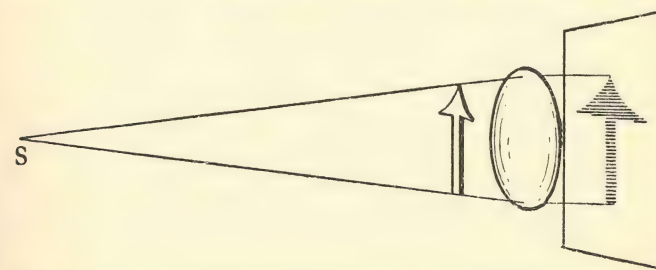
Fig. 27. A source of light s throws a shadow of an object upon a screen close to it. The interposition of a lens - of not too short a focus - between the object and the screen does not make much difference to the shadow, merely causing slight reduction and blurring.
