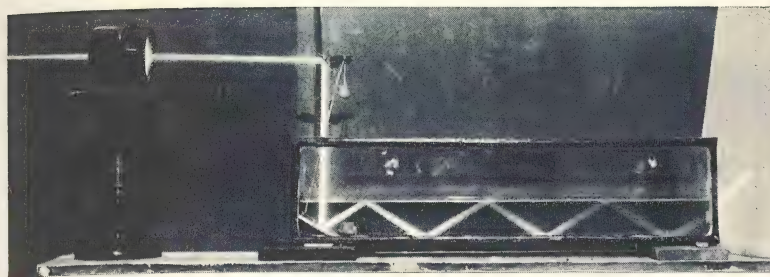
A. This photograph of the actual experiment shows several total reflections at the surface of the water. It may be observed that the ray that finally issues is refracted in doing so. The mirror M_2 (Fig. 45) is rather more tilted than in the photograph of Plate VIII B. (p. 74)
