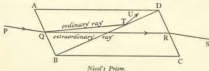
Fig. 86. A long piece of Iceland spar is cut into two pieces which are cemented by Canada balsam. The cut is so made in relation to the form of the crystal that only one of the two rays into which incident light is divided is able to get through the apparatus.
