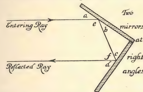
Fig. 6. Double reflection at two mirrors which are at right angles to each other. The two rays are parallel if the junction of the mirrors is at right angles to them; because a + d = b + c = 90^\circ ; \therefore e + f = 360^\circ - (a + b + c + d) = 180^\circ .
