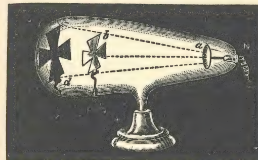
Fig. 96. The cathode or negative terminal is on the right at a . The rays proceed in straight lines across the tube and excite fluorescence on the opposite wall. A metal cross b casts a sharp shadow.
