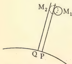
Fig. 94. To the observer at P the star s appears to be eclipsed by the moon when the latter is in the position M_1 ; at Q the eclipse takes place when the moon is at M_2 . The distance M_1M_2 is the same as PQ , which is known. Hence the velocity of the moon is found.
