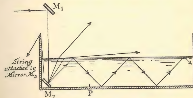
Fig. 45. Sectional diagram of a water tank arranged to show total internal reflection. A ray of light from the lantern is directed upon the mirror M_1 and there reflected so as to strike the mirror M_2 . The latter can be tilted by means of a string attached to it. In one position it reflects a ray which emerges from the water easily; in another the ray just emerges and skims the surface; in a third it is internally reflected at the surface of the water. A mirror lies along the floor of the tank.
