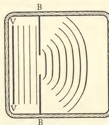
Fig. 63. Ripples started by the vibrating bar v move up to the barrier B in which there is a relatively wide opening. The continuation of the advance of the waves shows for some time the form of the opening.
