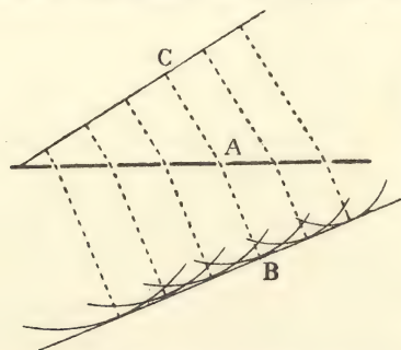
Fig. 79. A set of waves passing through apertures in a screen into a medium where its velocity is less than before. Circular ripples are shown forming one of the wave fronts.
