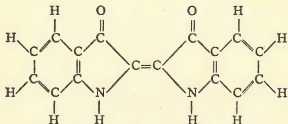
Fig. 61. The indigo molecule, drawn to show the result of the determination of its atomic arrangement by chemical methods.
