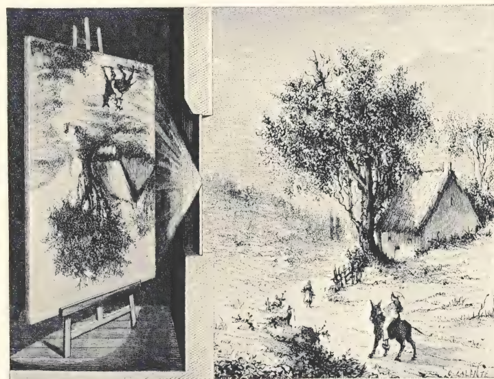
C. From a drawing in Guillemin's Forces of Nature , illustrating the action of a pinhole camera. (p. 32)
