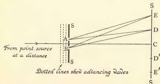
Fig. 73. Two small openings in a screen admit waves of light from the left. At C the two sets of spherical waves that open out from A and B reinforce one another and there is light. If DB is longer than DA by half a wave-length there is no light at D because the two sets of waves interfere on Young's principle. There is light again at E, when EB is longer than EA by a whole wave-length, and the two sets of waves are again in the same phase. Other lines of light and darkness occur alternately. The positions of the lines depend on the wave-length, for blue they are closer together than for red.
