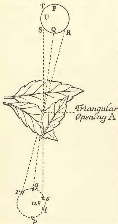
Fig. 16. The upper circle represents the sun and the lower its image upon the ground, due to the passage of sunlight through the triangular opening between the leaves. Each bright point upon the sun makes its own bright triangular patch upon the ground; the sum of all is the circle on the ground, with its penumbra.
