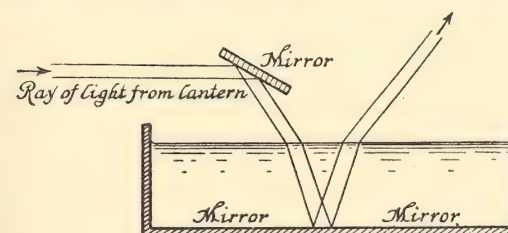
Fig. 39. The tank in the figure is filled with a slightly coloured liquid: and the front of the tank is made of glass, so that the path of the ray can be followed. A mirror forms the bottom of the tank.
