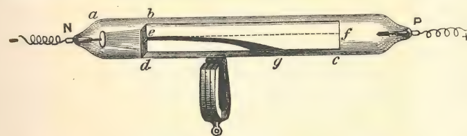
Fig. 98. The cathode rays are limited to a narrow pencil by means of a slot placed in front of the cathode at a . The deflections of the stream by a horse-shoe magnet are then observed easily.
