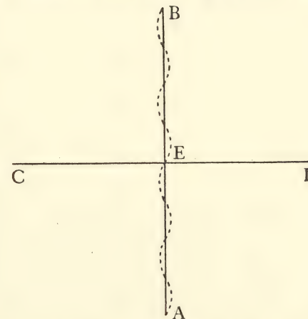
Fig. 91. Two ropes knotted together at E and held at the four ends. If a vibration in the plane of the diagram, as indicated by the wavy line, is originated at A, it will set BE in motion but not EC, nor ED: but if the vibration is perpendicular to the plane, EC and ED will be set into motion as well as EB.
