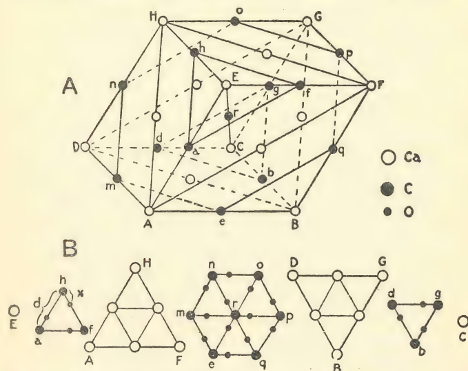
Fig. 82. The figure A represents the arrangement of the atoms of which Iceland spar, \text{CaCO}_3 is composed. The clear white circles represent atoms of calcium, and the black circles represent carbon. The oxygen atoms are not shown in this figure, in order to avoid confusion. The arrangement of the atoms in successive layers, perpendicular to the principal axis EC are shown in the figure B. The oxygens are represented here by small black circles. The figures show the relative positions of the atoms and no more. The distance between the successive layers of B is 2.79 Angström units, about the hundred millionth part of an inch. The sizes and shapes of the atoms are not indicated in the figure, being far less easily determined than the relative positions of the centres of the atoms.
