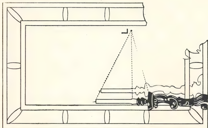
Reflection in a plane mirror. The image of the camera is dimly seen on the right just above the flowers. A straight line joining the lens of the camera to its image is perpendicular to the top of the candle to its image. The drawing illustrates this point. (p. 22)
