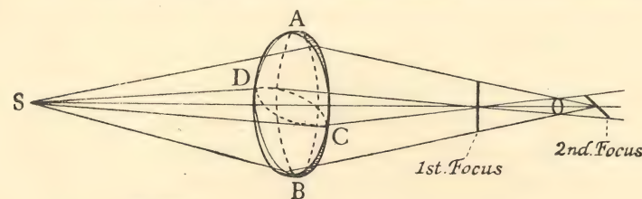
Fig. 34. An astigmatic lens is so formed that cross sections through its centre such as are outlined by the dotted lines in the figure are not all alike. For instance, the faces of the section D C are more curved than those of A B. The rays from S after passing through the lens do not converge upon a point, but upon two short line foci, as shown in the figure. The first line is in the plane of the diagram, the second is perpendicular to it.
