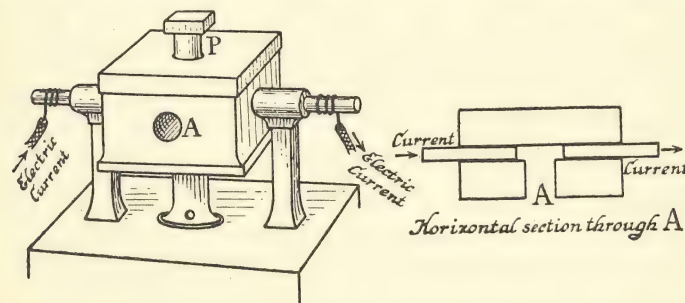
Fig. 95. The little furnace is made of refractory materials. Inside it an arc is formed by the electric current. Metals are dropped in at the hole on top. When the hole is left open the vapours escape and the light that issues at A can be resolved into a bright line spectrum. When the plug P is inserted, the vapour fills the tunnel ending in A, and the light has to go through it. Dark lines now appear in the spectrum where there were bright lines before.
