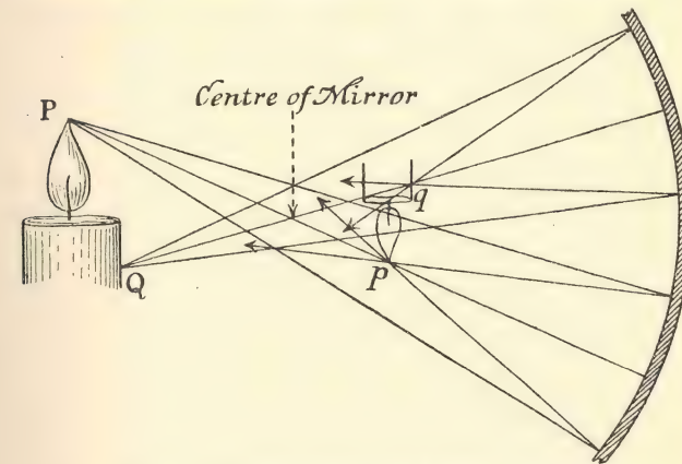
Fig. 15. Optical reflection at a concave mirror.
