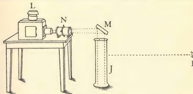
Fig. 92. Light from the lantern L is polarised by the Nicol prism N and reflected by the mirror M into the tall jar, which is filled with liquid containing finely divided matter in a state of suspension. The amount of light scattered varies with the direction of scattering as explained in the text.
