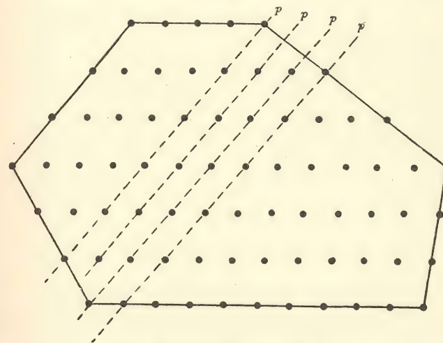
Fig. 102. The points in the figure can be arranged in rows in various ways.
