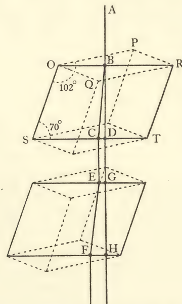
Fig. 77. The figure is redrawn from that which Huygens gives in his Treatise . For convenience of representation the crystal is supposed to be cut so that OP , OQ and OS are all equal, in which case OT is the axis through O , and ORTS is a section containing the axis. The ray AB is perpendicular to the face OPRQ ; it divides into the ordinary ray BD , which is in line with AB , and BC which is not: both rays lie in the plane ORTS . On leaving the crystal they resume their original direction.
