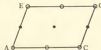
Fig. 83. The figure shows the arrangement of the atoms of the spar in the plane EACG (Fig. 82). This corresponds to the plane OSTR of Fig. 77.
