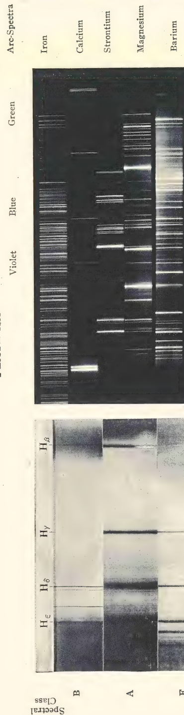
B. Spectra of the luminous gases of various elements vaporised in the electric arc. (A. Fowler). (p. 212)
