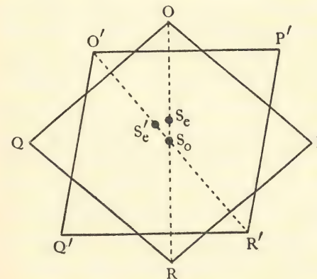
Fig. 78. This diagram shows the relation between the ordinary and extraordinary images of a black spot seen through the crystal of Iceland spar. The observer sees black spots at S_o and S_e of which the former is the nearer. If the crystal is turned round, to O'P'R'Q' for example, the spot S_o does not move, but S_e moves to S'_e ; which latter point lies on O'R' . If the crystal is moved about on the paper without rotation, neither spot moves.
