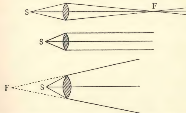
Fig. 24. These diagrams show the converging action of the lens for various relative positions of lens and source.
