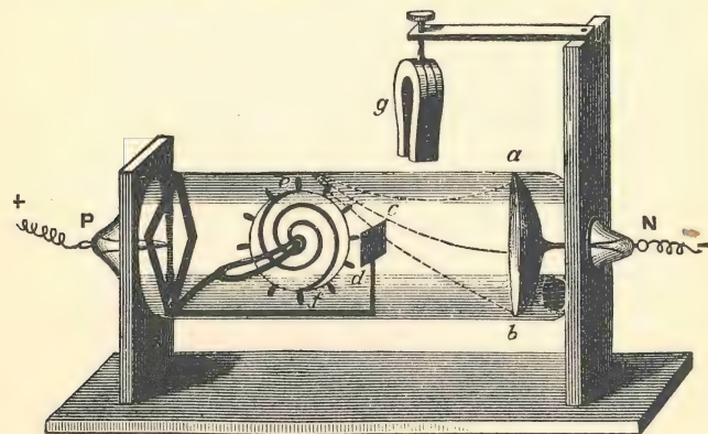
Fig. 99. The cathode a is made in the shape of a saucer: this is found to have the effect of concentrating the rays to a point. Normally a screen c intercepts the rays, but the magnet g deflects them so that they get over the top of the screen and strike the vanes of the little wheel ef , which then spins rapidly. If the disposition of the magnet is reversed, the rays go under c and the wheel spins the opposite way.
