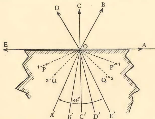
Fig. 51. The refractive index of diamond is very large. A ray A'O A just succeeds in emerging. Rays such as Q O Q' are reflected internally. The paths may be followed in either direction.
