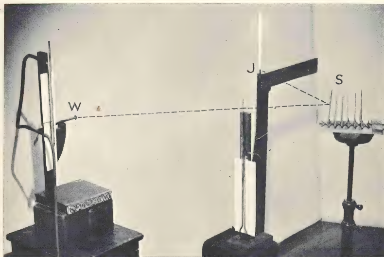
C. A photograph of the apparatus used by Lord Rayleigh and described on pp. 245-6. The whistle is at W, the set of screens at S, and the luminous gas jet at J. The dotted lines show roughly the course of the sound waves that affect the jet. The photograph shows the appearance of the jet when there is no sound, or when the screens (seen edge-ways in the picture) are not placed so that their reflections reinforce one another. Owing to a peculiarity in the form of the nozzle at J, the jet does not respond to sound proceeding directly from W to J. When the screens are properly spaced the jet broadens and ducks to a fraction of its normal height.
