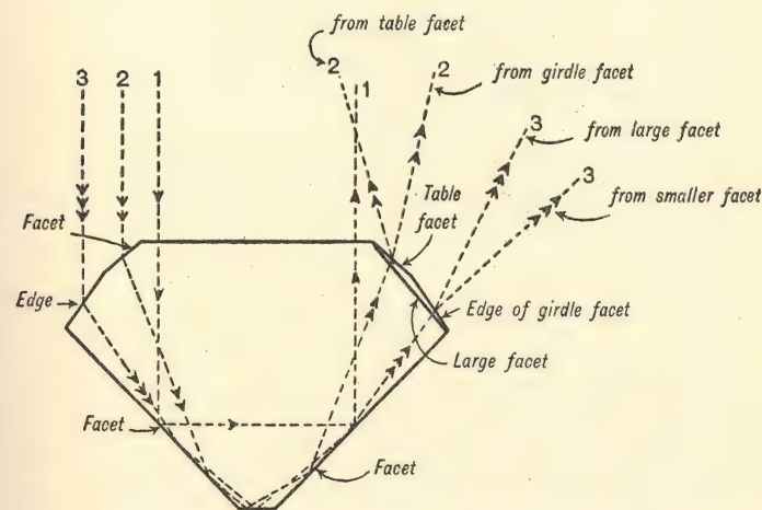
Fig. 50. The figure shows a few of the various paths by which a ray of light entering the brilliant from the front is refracted and 'totally internally' reflected until it leaves again through the front, never succeeding in getting through the diamond.
