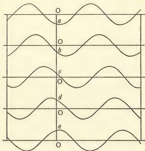
Fig. 106. A diagram to show how the reflected waves of Fig. 105 add up to nothing unless they are all exactly in phase with one another. The quantity 0a + 0b + 0c + \dots is zero because there are as many positive as negative terms in the millions that must be added together. The exception is when the reflections are all in phase, the crests of one set being exactly above or below (in this kind of figure) crests of all the other sets.
