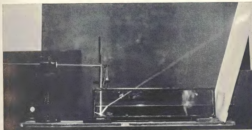
B. A photograph of an experimental arrangement showing the refraction of a beam of light as it crosses a surface between water and air. (p. 68)
