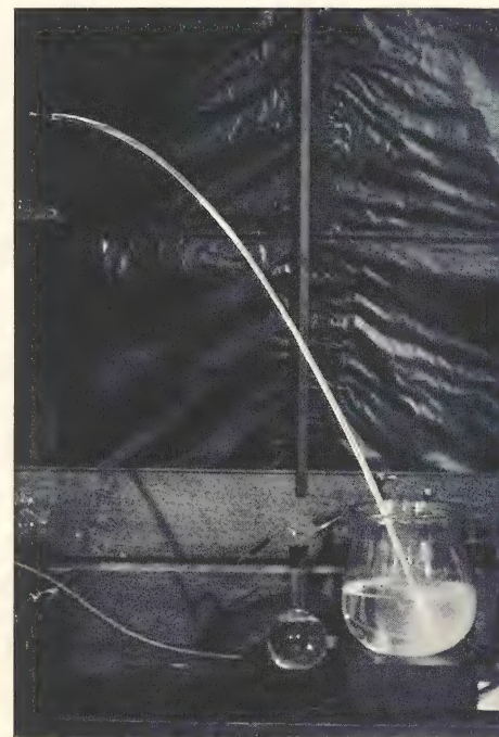
B. An experiment due to Tyndall illustrating total internal reflection. Light enters the jet of falling water at its point of issue from the tank and is carried down by the stream. The light is supplied by an electric arc outside the tank and focussed upon the jet by a lens in the tank wall. The arc and the lens do not appear in the photograph. (p. 74)
