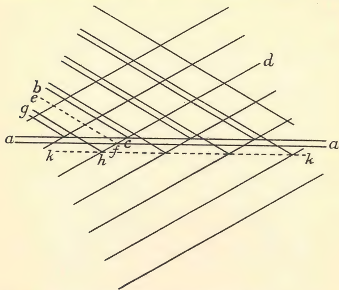
Fig. 71. A train of waves falls upon the thin film a a . The film may be of any transparent material. The waves strike the upper surface and are reflected as shown, as for example b c d where b c is the reflected portion and the part c d has not yet met the film. If c d is the crest of one part of the wave, b c is the crest of the other. The waves pass on, losing only a part of their energy by reflection at the first surface, and meet the second. Here they lose half a wave-length in the act of reflection, as explained in the text. The dotted line e f shows where the crest of the reflected wave would have been if the reflection at the second face had been of the same character as that at the first. The loss of the half wave-length puts the reflected wave back to g h . Reflection takes place as if at the surface shown by the dotted line k k : the extra delay has the effect of adding apparently to the thickness of the film.
