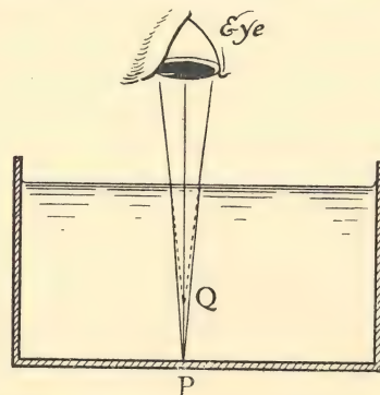
Fig. 42. The rectangular outline is the section of a tank of water. An eye looks at an object P at the bottom of the tank immediately below. Owing to refraction the pencil of rays from P which enters the eye is opened out on leaving the water and seems to come from Q. The eye has to be drawn out of proportion so that the spreading of the pencil can be shown. The depth of Q is three-quarters of the depth of the water.
