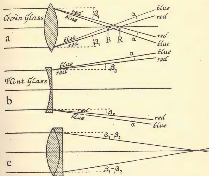
Fig. 56. The top figure shows a lens of crown glass. Its converging power is indicated by the magnitude of the angle \beta_1 . The amount by which it separates blue from red is indicated by the angle \alpha . The middle figure shows a flint glass lens, with a diverging power indicated by \beta_2 , less than \beta_1 ; but it produces the same separation of red from blue as the other lens. The two together, in the third figure, do not separate blue from red, but possess a converging power \beta_1 - \beta_2 .
