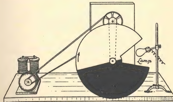
Fig. 53. The disc is rotated in the direction which is indicated by the arrow. The lamp, which is red, is visible at intervals through the open sector. It appears green, and not red. The disc must be well illuminated.
