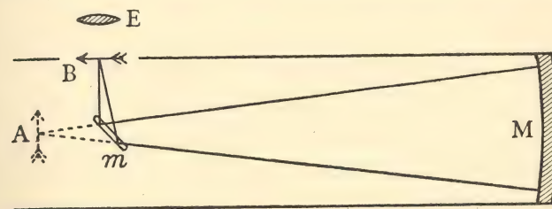
Fig. 55. A diagram showing the arrangement of Newton's telescope.
