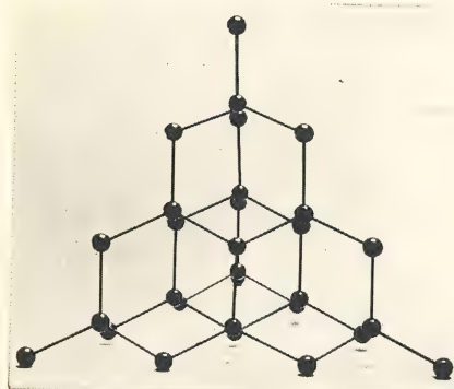
A. A model showing the structure of diamond. Each ball represents a carbon atom in respect to position only, but not in respect to form or size. The distance between the centres of two neighbouring atoms is 1.54 Angstrom Units (One unit is the hundred-millionth of a centimetre.) (p. 249)
