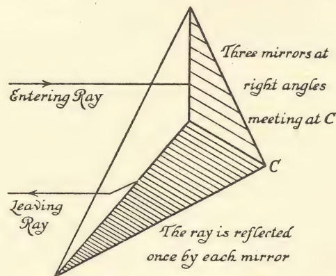
Fig. 8. Reflection from three mirrors at right angles. However the mirrors are held the entering and returning rays are parallel.
