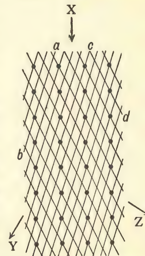
Fig. 107. The dots represent the units of a cubic crystal. The scale would be about 100,000,000 to one. The direction marked x is that of the incident X-rays. There are reflections in the direction y due to planes parallel to ab , and in the direction z due to planes parallel to cd ; also in other directions not indicated.
