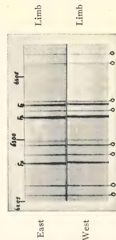
A. A few star spectra showing the shift of the maximum intensities from hot white stars of class F, such as Procyon and Canopus, to cooler red stars of class M, Antares and Betelgeuse. (p. 200) From The Sun, The Stars and The Universe , by W. M. Smart.
