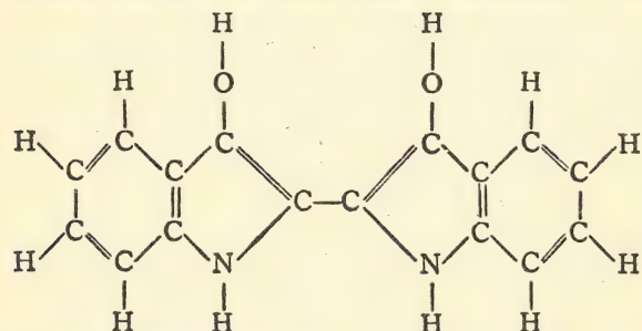
Fig. 62. The indigo molecule, altered so as to become soluble.
