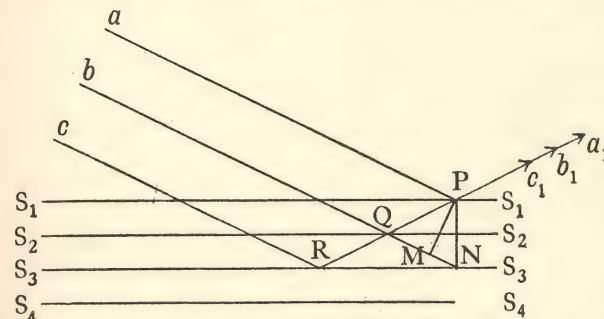
Fig. 105. The diagram illustrates the reflection of a train of waves by a series of regular spaced sheets, each capable of reflecting a small fraction of the energy of the train.
