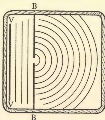
Fig. 64. In this case the opening in the barrier is relatively small, and the continuation of the advance of the waves takes the form of semicircular ripples.
