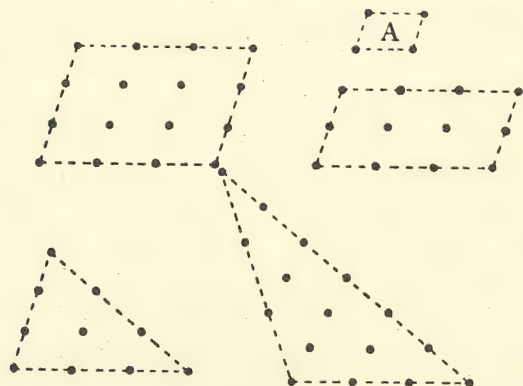
Fig. 101. The unit of a planar design is included in the outline A. The multiplication of the unit may assume various forms, a few of which are shown. The mutual inclinations of the edges are limited to certain definite angles.
