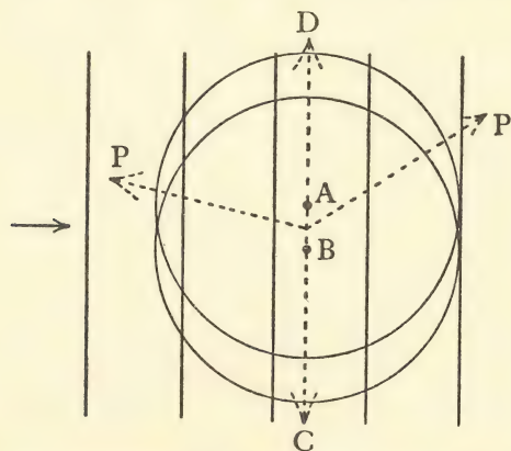
Fig. 103. Waves represented by the vertical lines are moving upon the two atoms A and B which scatter a small fraction of their energy. The two are half a wave-length distant from one another. The spherical waves that spread away annul one another in the directions A B C or B A D, because the crest of one fits into the hollow of the other. But energy is scattered in all other directions such as are indicated by the arrows marked P. This is really a particular case of Fig. 73.
