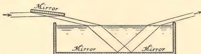
Fig. 40. This figure shows the path of a ray entering the water more obliquely than in Fig. 39.
