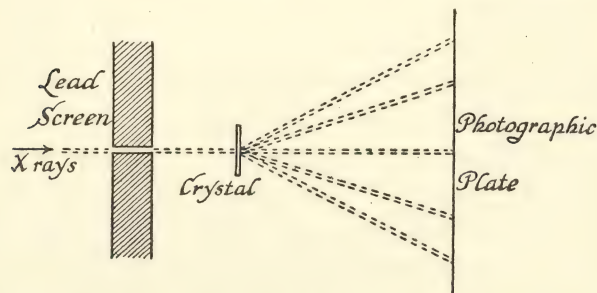
Fig. 100. The X-rays pass through a fine opening in a lead screen and impinge upon the crystal as shown. Laue's diffraction pattern is formed upon the photographic plate.
