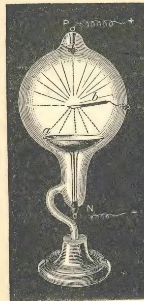
Fig. 108. This figure like those of Figs. 96, 97, 98 and 99 is from a block used to illustrate the lecture given by Crookes at the Royal Institution in 1879. The glass is blown into the form of a bulb; the negative pole or cathode is at the bottom: there is an anode or positive pole at the top but its position is immaterial. The target is a piece of platinum wire b : which might also have served as the anode. The cup-shaped cathode concentrates the stream upon the target. As Crookes described it, 'The platinum wire not only gets white hot, but you can see the sparks coming from it on all sides, showing that it is actually melting.' The experiment was arranged to illustrate the development of heat, it was not known then nor for twenty years afterwards that the platinum was radiating X-rays. The bulb in the figure is about six inches high.
