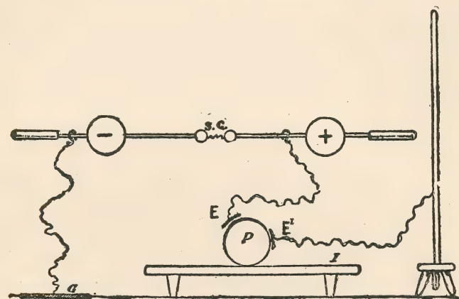
FIG. 2. Showing Arrangement with an Insulated Capacity. I, Insulated Platform; P, Patient; E, Electrode; E', Second Electrode; G, Ground Connection; S. G., Spark Gap.
