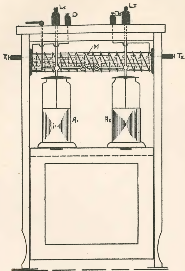
FIG. 43. DeKraft's High Frequency Resonator.
