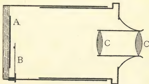
FIG. 24.—Details of spinthariscopes.
