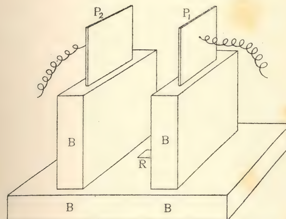
FIG. 13.—Curie's method of showing magnetic deviation of the \beta -rays.
