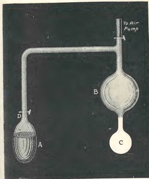
PLATE VII.—A DIAGRAM OF CURIE'S CONDENSATION EXPERIMENT, SHOWING APPEARANCE OF APPARATUS WHEN THE BULB C IS IMMERSSED IN LIQUID AIR.
