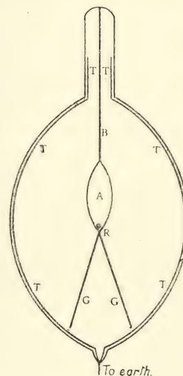
FIG. 10.—Strutt's apparatus for showing the effects of electrical charges carried by the \beta -rays particles.
