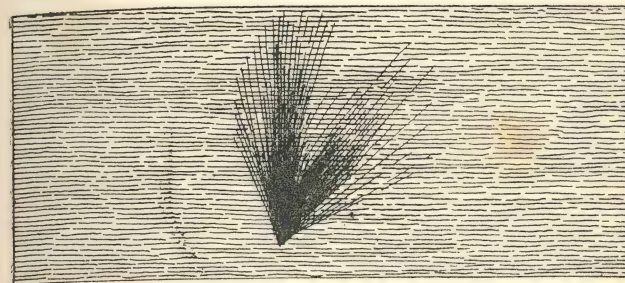
FIG. 11.—Illustrating magnetic deviation of \beta -rays.
