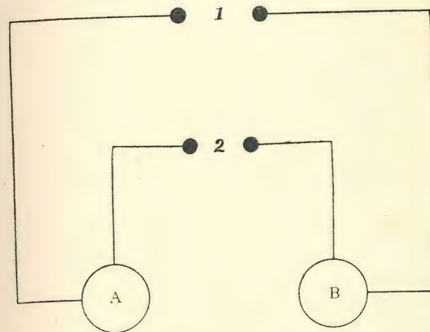
FIG. 16.—Diagram of spark gap experiment.
