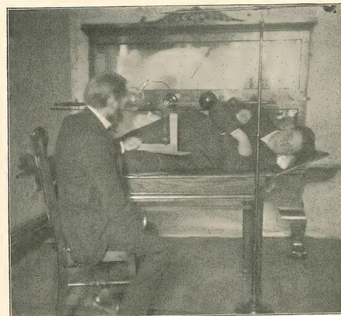
Fig. 26.—Method of Locating Foreign Bodies. First Exposure.
