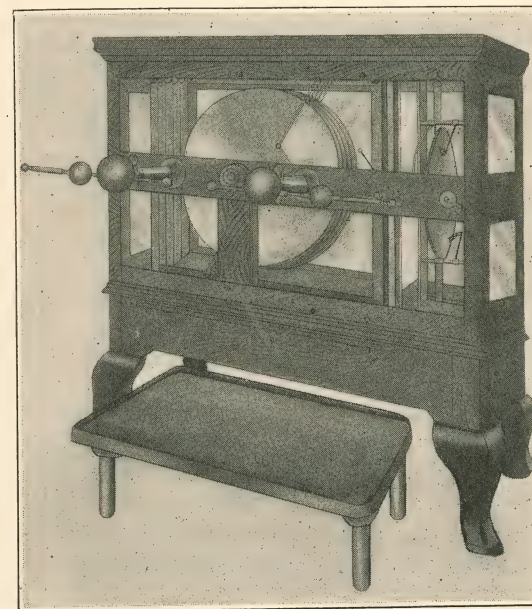
Fig. 2.—A Modern Holtz Machine.
