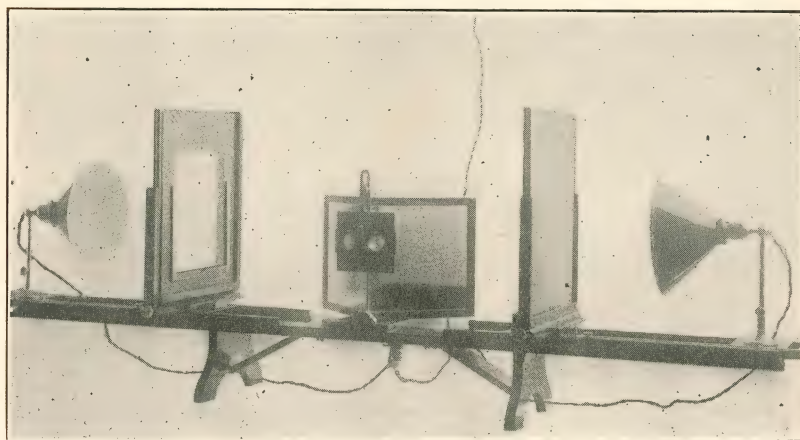
Fig. 22.—X-Ray Stereoscope.
