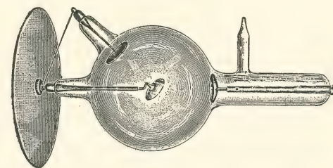
Fig. 11.—A German Tube.
