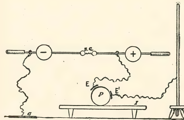
Fig. 35.—I, Insulated Platform; P, Patient; E, Electrode; E', Second Electrode; G, Ground Connection; S. G., Spark-Gap.
