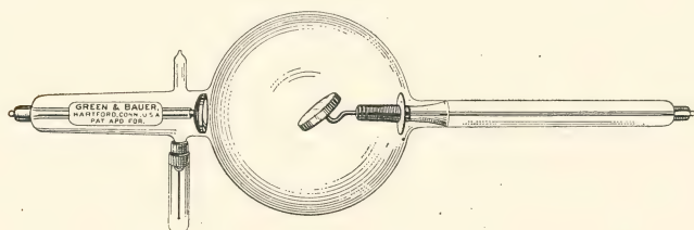
Fig. 16.—X-Ray Tube, Showing Heavy Metal Anti-Cathode.
