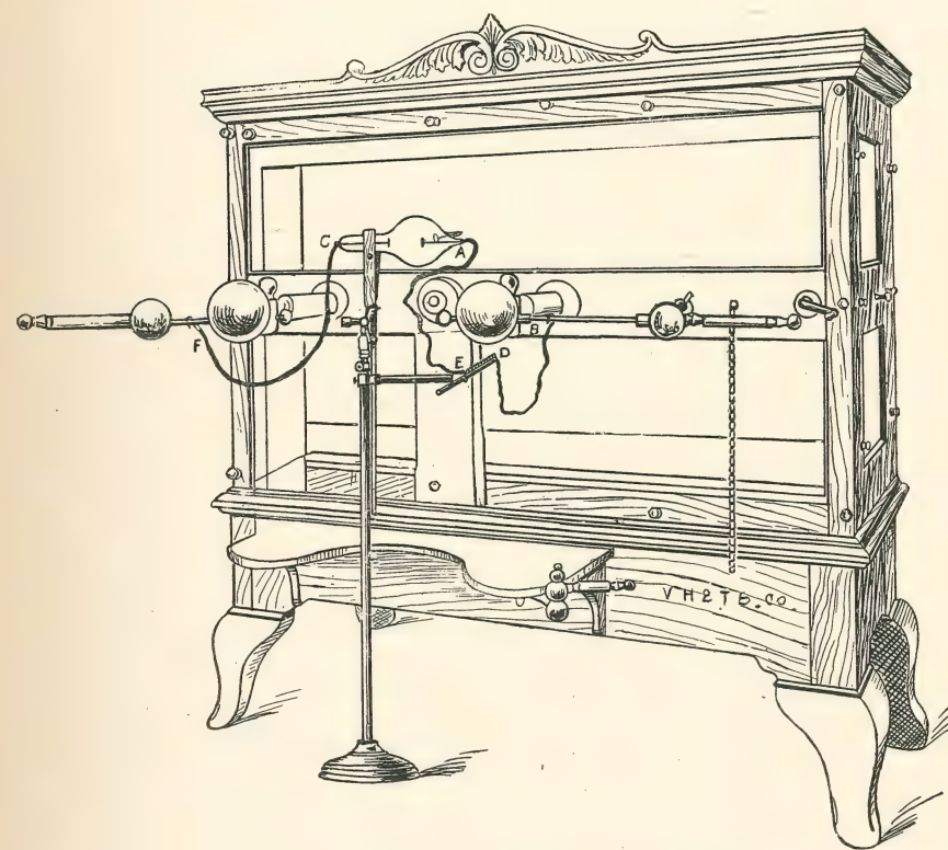
Fig. 5.—Files Interrupter in Circuit.
