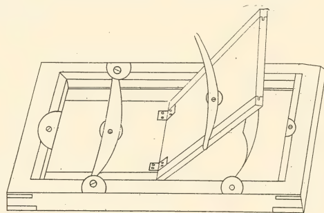
Fig. 21.—Printing Frame.
