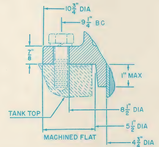
SECTION THROUGH MOUNTING FLANGE
