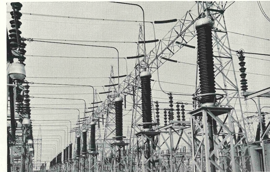
Underground cables from the transformers at the Robert Moses Niagara Power Plant provide six 230-kv circuits to the center of the Niagara Switchyard. All 18 cables are terminated at each end by O-B potheads.
