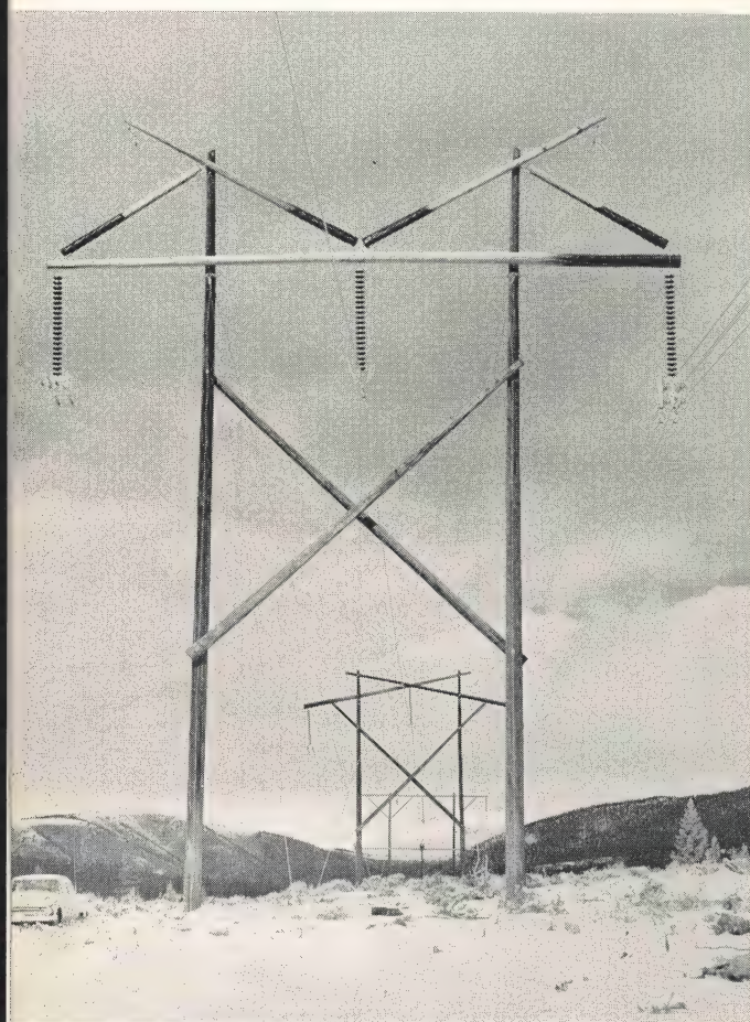
6. Structure number five is conventional spar H-frame design. Note that four-conductor bundle has been strung on right-hand phase. Tension on the bundle is 24,400 pounds at 0 degrees F., with no ice and no wind. The bottom half of the bundle was removed before heavy ice loading occurred.
