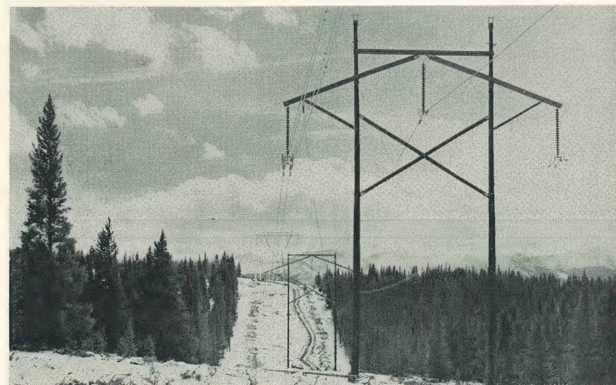
6. Structure number five is conventional spar H-frame design. Note that four-conductor bundle has been strung on right-hand phase. Tension on the bundle is 24,400 pounds at 0 degrees F., with no ice and no wind. The bottom half of the bundle was removed before heavy ice loading occurred.
