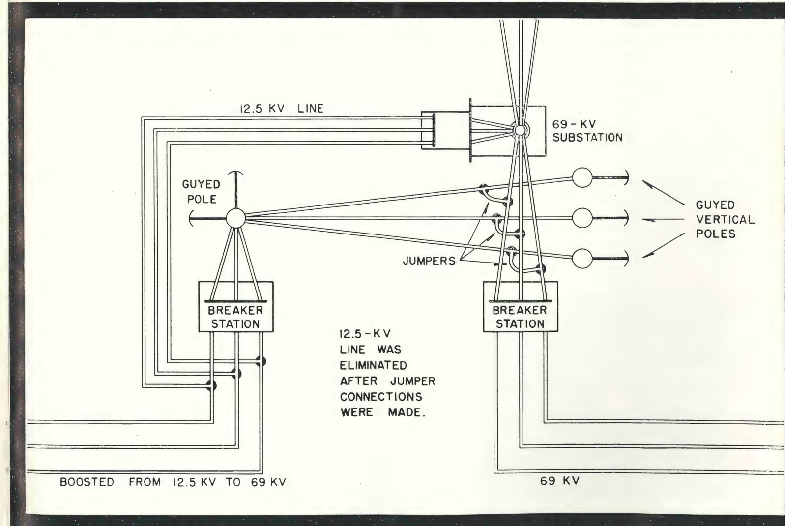
Three phases of a 69-kv cross bus being connected with permanent jumpers. Holan elbow safely puts crewmen within arm's reach of the job, relieves undue tension and eases problem of fatigue.
