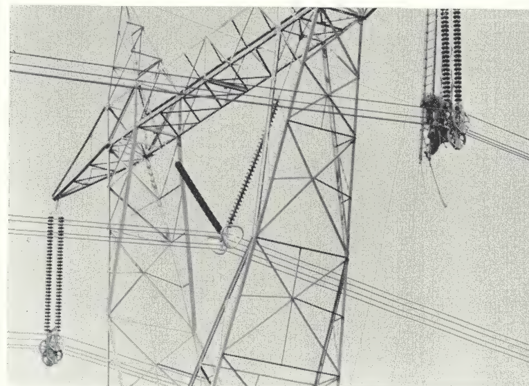
This view shows arrangement of sheave blocks for pulling conductors. Center phase V-string has already been clipped in.
