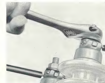
Not only do the Belleville washers provide a visual indication of proper pressure on the conductor, but you can actually feel the increase in torque as you turn the wrench.
