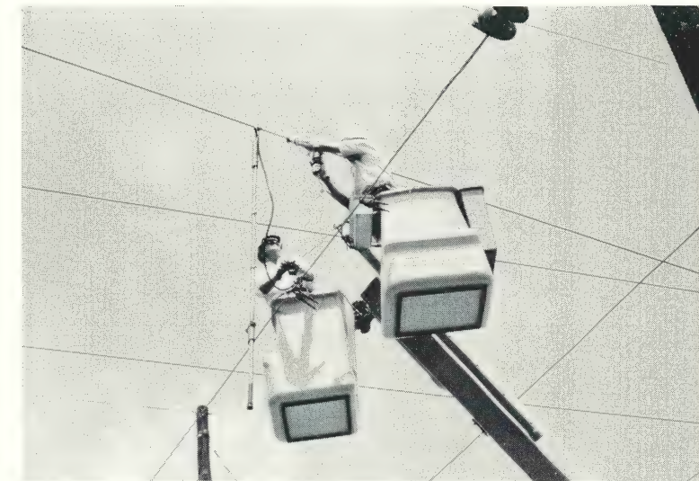
Temporary jumper has been installed with a hot stick and live line crewmen prepare conductor for permanent jumper. Bucket men are bonded to conductor and are using the LLBM.
