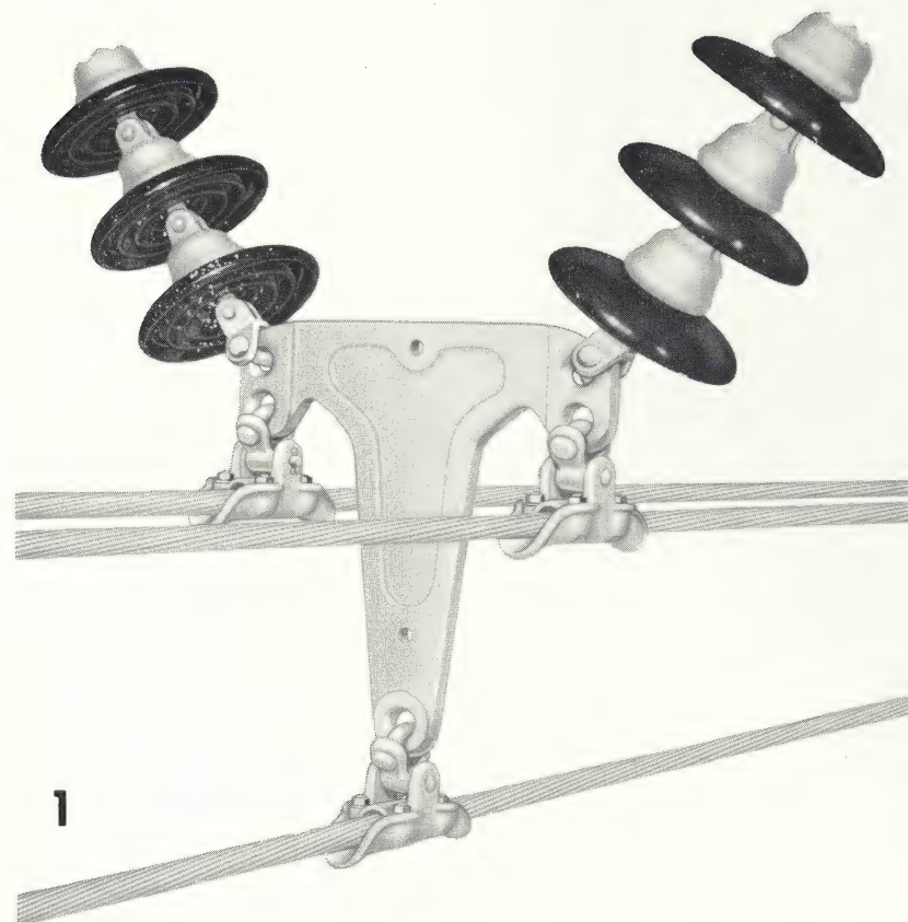
1. Detail of three-conductor bundle suspension. All line hardware and insulation for the 358-mile, 500-kv Arkansas Power & Light Company construction were furnished by O-B.
