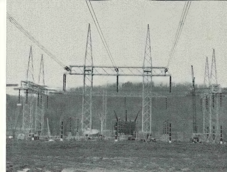
View of the test station during construction -- looking west. Ohio River is beyond transformer. Test lines "A" and "C" run north (right) and south (left), while line "B" runs toward the viewer.
