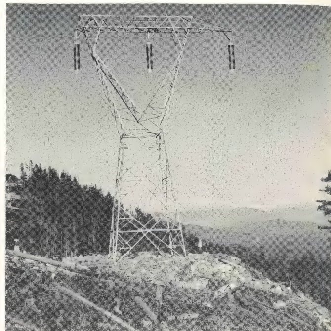
The second line in the EHV grid -- Rosedale, Creekside, Bridge River -- passes through mountainous country, which, according to Indian legend, was once the home of giants.
