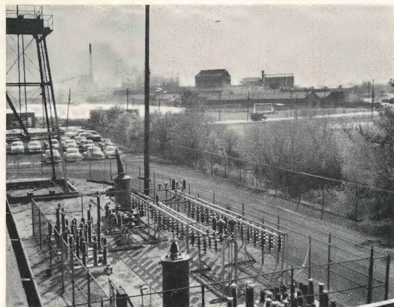
General view of the outdoor test location where Ohio Brass collects much of its data on surface leakage.
