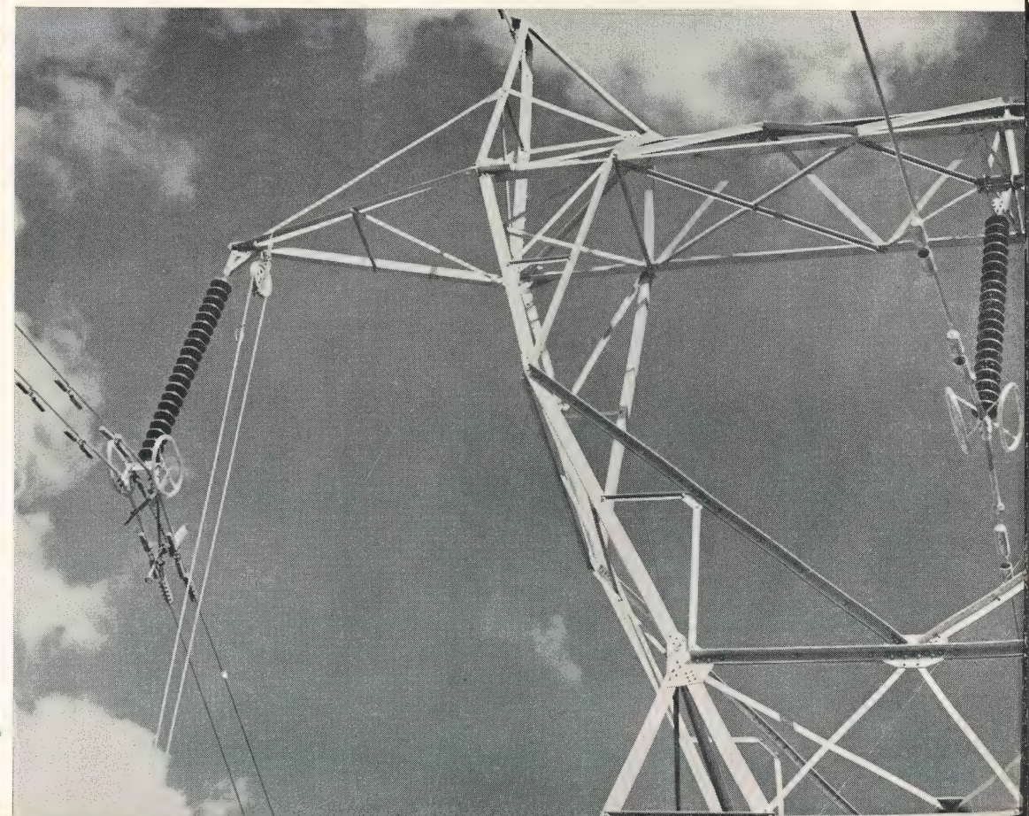
11. Test conductors are suspended on strings of 20 5/8-inch insulators. Tapered armored rods are used at each suspension point. Single stockbridge dampers for each conductor are provided except in the longest span (shown here) where two dampers are used.
