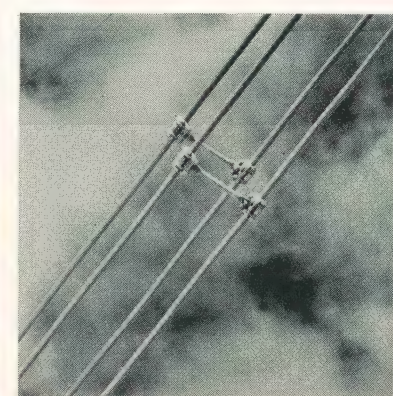
10. Tubular type of spacers on four-conductor bundle. Spacers were arbitrarily installed every 200 feet in each span.
