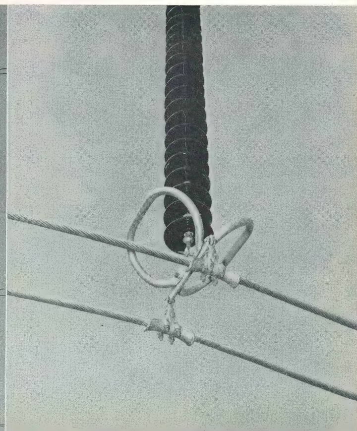
Ingledow-Wahleach hardware, conductor and insulation arrangement. Twenty-one 25,000-pound O-B insulators were used. Insulators and hardware were designed by O-B to hold corona characteristics and RIV to 230-kv level.
