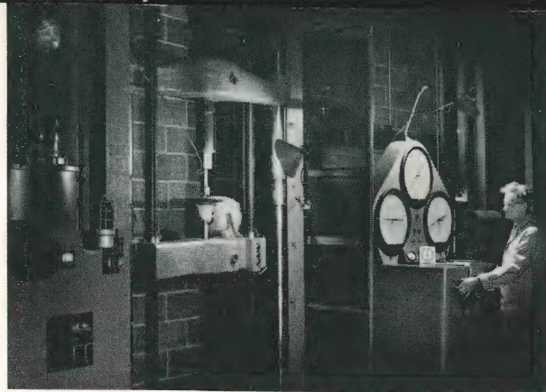
Mechanical and electrical load are applied simultaneously on assembled suspension unit.
