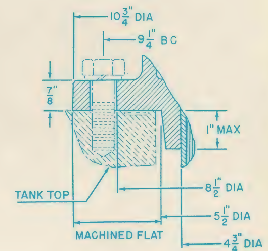
SECTION THROUGH MOUNTING FLANGE
