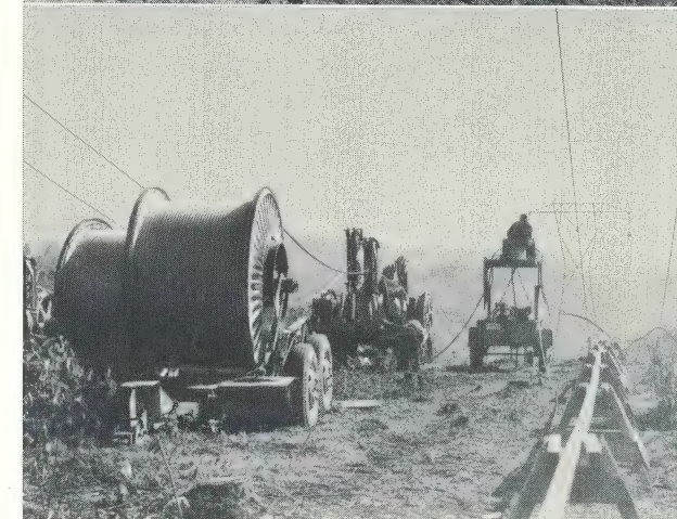
Three phases were strung simultaneously under tension.
