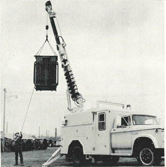
NO PROBLEM: Capacity at this angle, 7,400 pounds.
