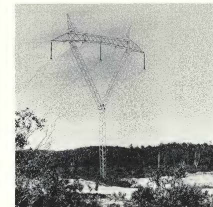
First use of a new guyed Y-type aluminum tower is noted on Ontario Hydro's 500-kv line.
