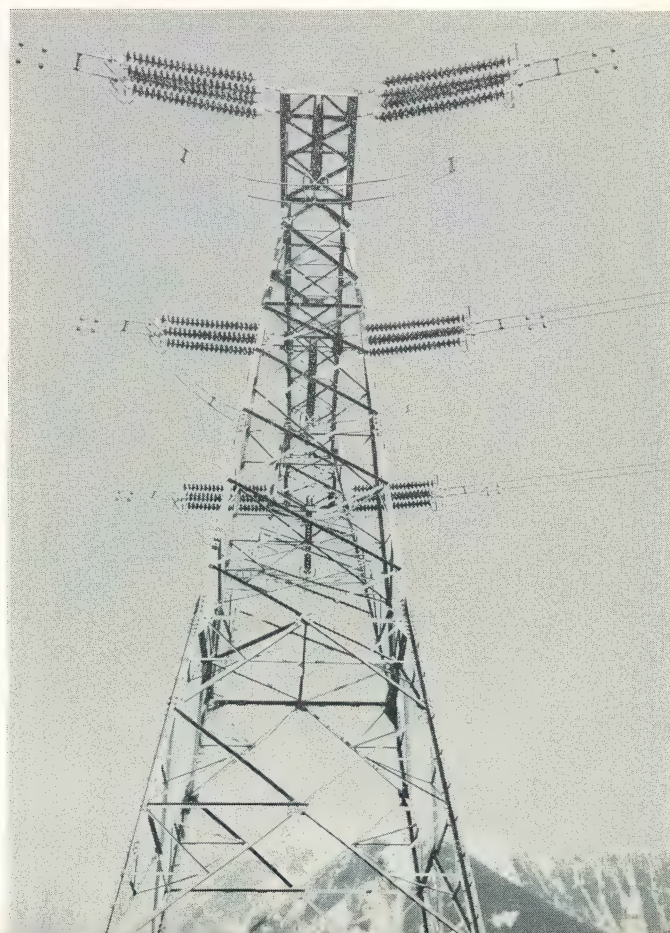
Angle tower on Rosedale, Creekside, Bridge River line. This line used lattice type steel towers, considered more suitable to rough terrain.
