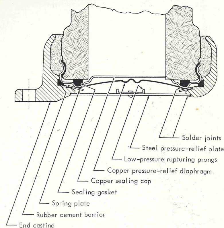
Figure 2 — Section drawing of base of GP intermediate arrester, illustrating arrangement of pressure-relief components. Note that position of relief diaphragm is concave upward at normal pressure.
