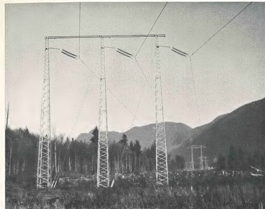
Ingledow-Wahleach angle tower. Line was initially built with single conductor. Second conductor has now been added.
