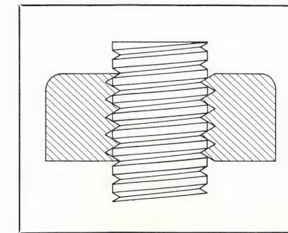
Brass nut has standard threads and is easily replaceable. Thread-stripping safety feature is provided by removing the crests of the stainless steel terminal stud threads.
