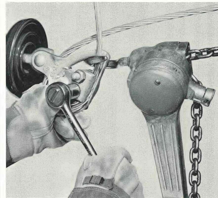
Clamp jaws are held apart in full open position by a spring on Universal Clamp Number 88500, with no loose pieces and nothing to take apart or put together.
