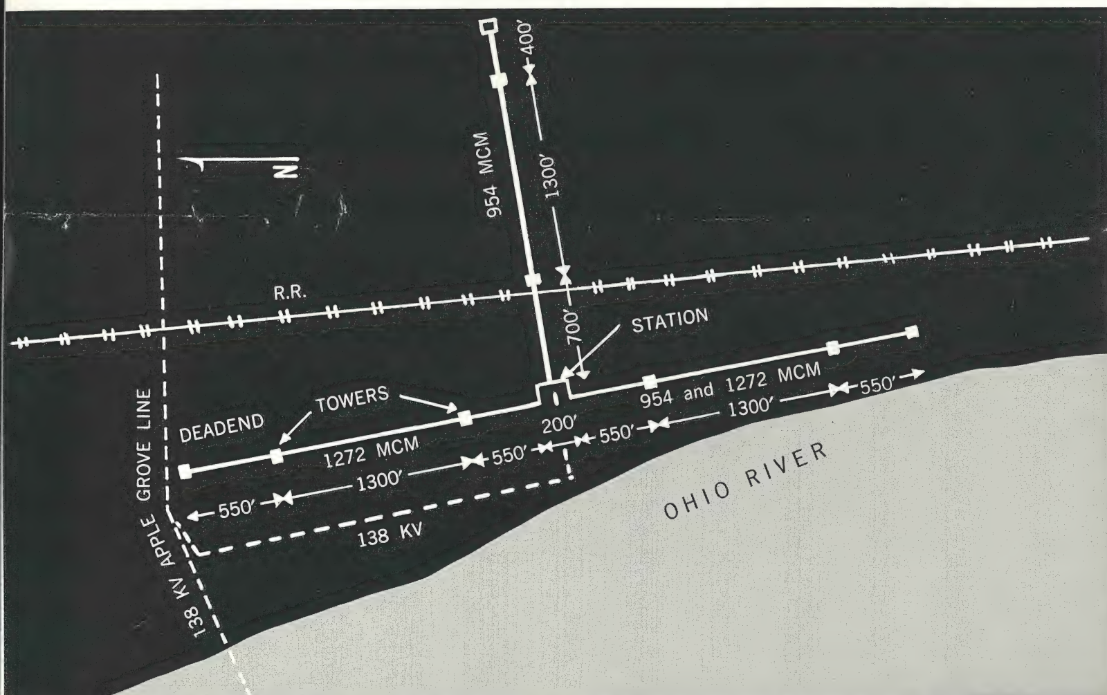
SKETCH A—Plan view of the Apple Grove 750-kv test project.
