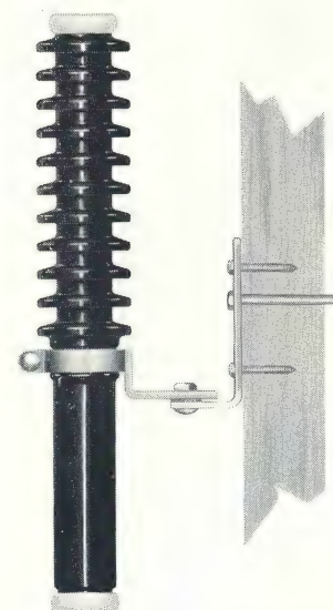
EEI-NEMA bracket can be ordered without back piece for pole top or surface mounting. Additional 11/16 -inch-diameter hole in angle piece permits use of 5/8 -inch through bolt.
