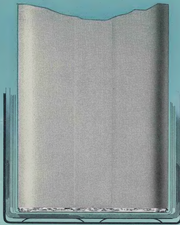
Working through the flexible secondary insulation, the springs press the contact plate firmly against the foil at the end of the element, putting the plate in contact with every layer of foil.
