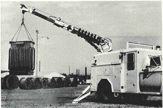
PROBLEM: Capacity at this angle 3,500 pounds -- overload device actuated.
