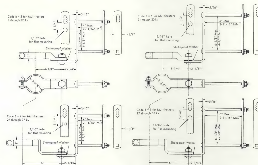
EEI-NEMA bracket can be ordered without back piece for pole top or surface mounting. Additional 11/16 -inch-diameter hole in angle piece permits use of 5/8 -inch through bolt.
