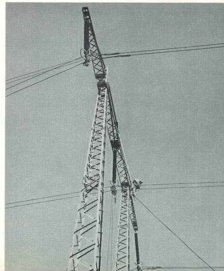
Ingledow-Wahleach restringing and tensioning of 795 MCM ACSR Drake conductors. It was necessary to resag the old conductor when tensioning in the added phase conductor.
