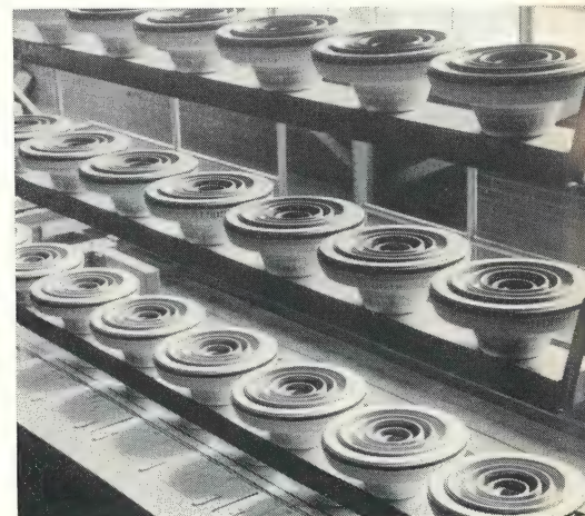
Conveyor filled with newly-formed insulators on their way to the mold release dryer typifies highly mechanized system now used to produce O-B insulators. Units harden sufficiently in the dryer to permit automatic release from the molds.
