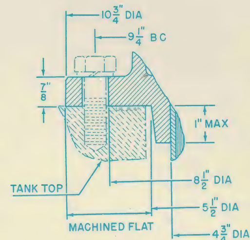
SECTION THROUGH MOUNTING FLANGE
