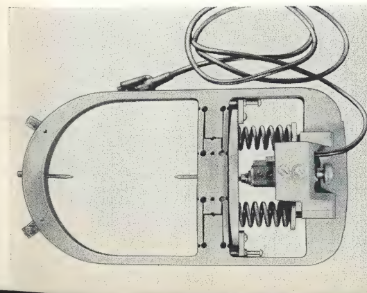
Gauging instrument, showing the two sharp probes which are positioned directly against the porcelain head of an assembled insulator through holes drilled in the malleable iron cap.
