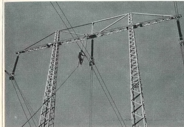
Ingledow-Wahleach hardware, conductor and insulation arrangement. Twenty-one 25,000-pound O-B insulators were used. Insulators and hardware were designed by O-B to hold corona characteristics and RIV to 230-kv level.
