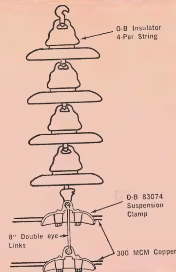
Tangent poles at The Dayton Power & Light Company before and after bundling. One insulator was removed to provide clearance for second conductor. Drawing shows detail of modification.
