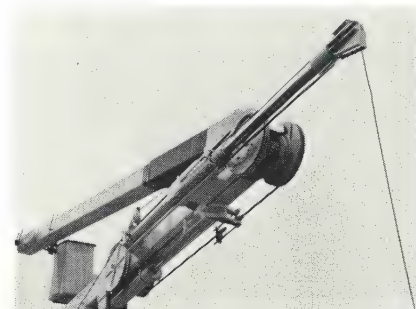
Many Holan Broncos are equipped with a "stinger" -- an hydraulic extension of the sheave head beyond the lower arm for greater working height.
