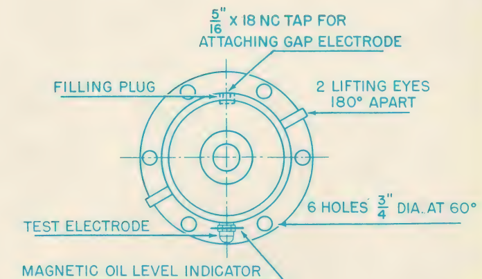
PLAN VIEW
