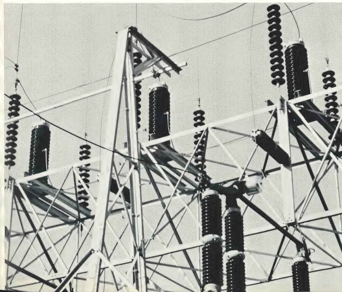
Jumper connection to terminal tap on arrester provides protection for system operation at 69 kv.
