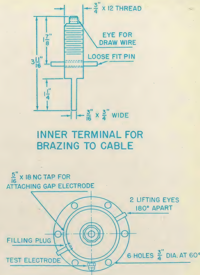
PLAN VIEW
