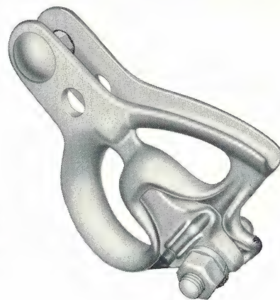
Number 81500 - has a reversible clamping piece; conductor diameters range from .16 inches to .44 inches; ultimate strength is 10,000 pounds; each unit weighs 2.3 pounds.
