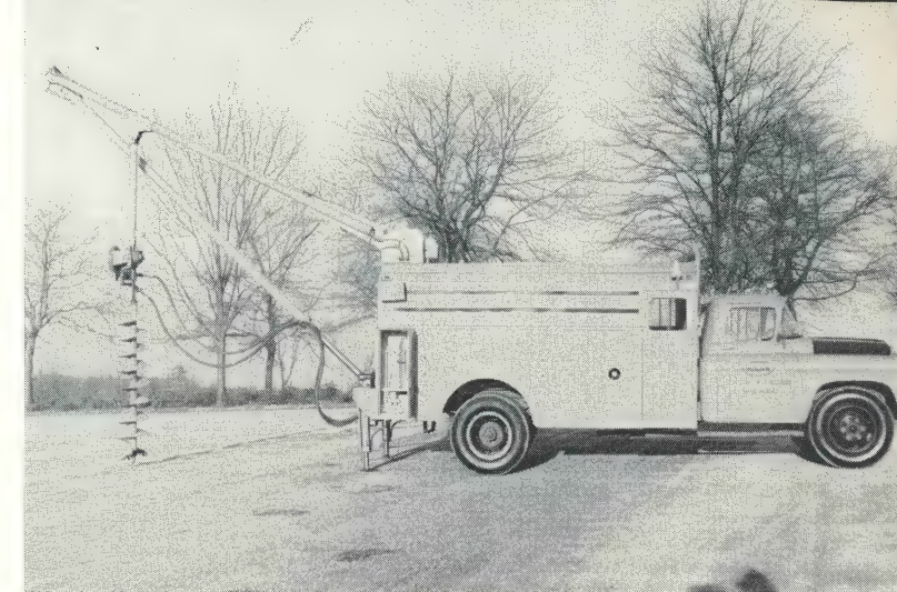
Griffin-designed Series 7000 Body is cost-engineered, built of low carbon steel. Series 3700 Derrick, also shown on the cover and below, is the powerhouse of the industry... tested at 22,000 pounds, handles 75-foot poles. Digger mounted on side leg for lower stowed clearance and more clearance when setting poles.
