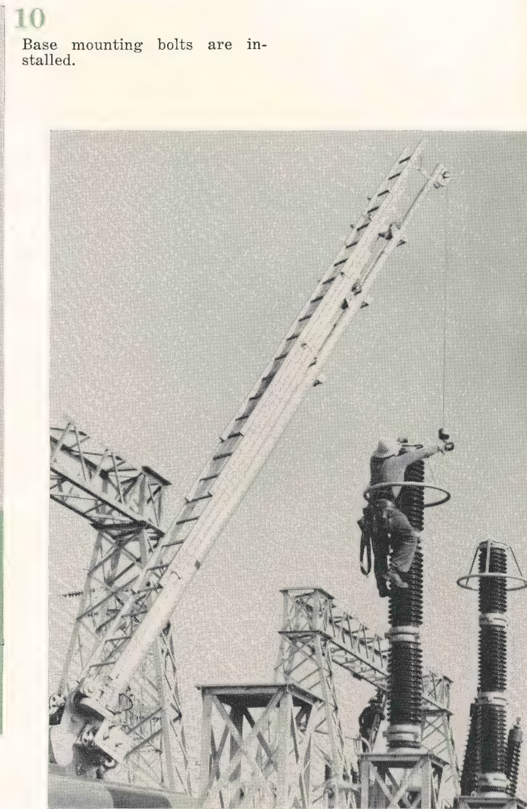
10 Base mounting bolts are installed.
