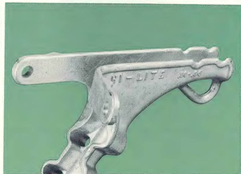
Malleable iron strain clamps withstand abrupt bending without fracture -- on test and in field service. Malleable iron combines excellent strength with high ductility.
