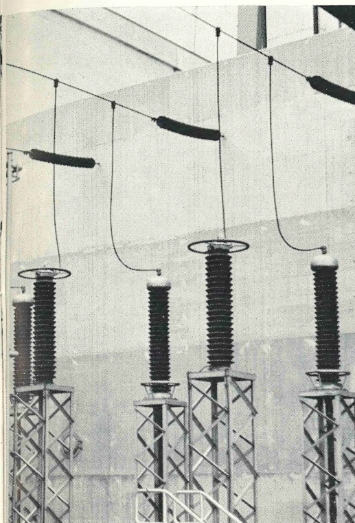
Underground cables from the transformers at the Robert Moses Niagara Power Plant provide six 230-kv circuits to the center of the Niagara Switchyard. All 18 cables are terminated at each end by O-B potheads.
