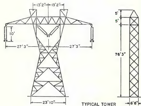
Figure 1. Dimensioned sketch of Ohio Edison narrow-base 345-kv tangent tower. Horizontally-bundled conductors sharply reduce probability of broken-conductor loading, permit very economical tower design. Angle towers and deadends have broad, square base.
