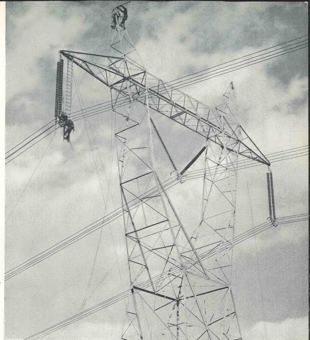
Apple Grove project energized at 750-kv (see page 2)
