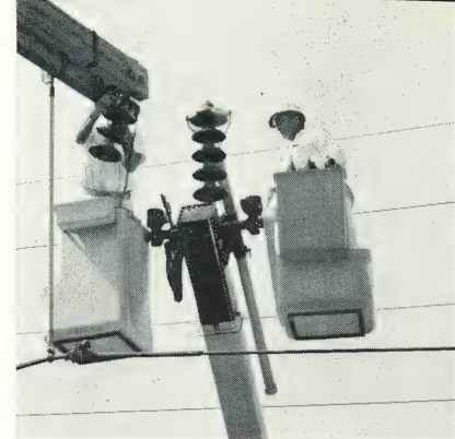
Dishpan attachment on the end of a standard-equipment gin pole picks up string of suspensions during changeout of broken insulators.
