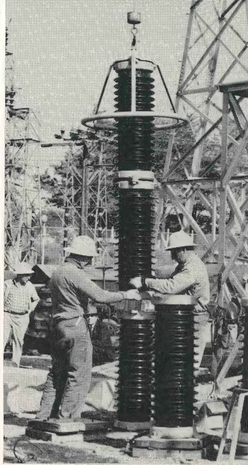
4 Top two units are moved into position on base unit.
