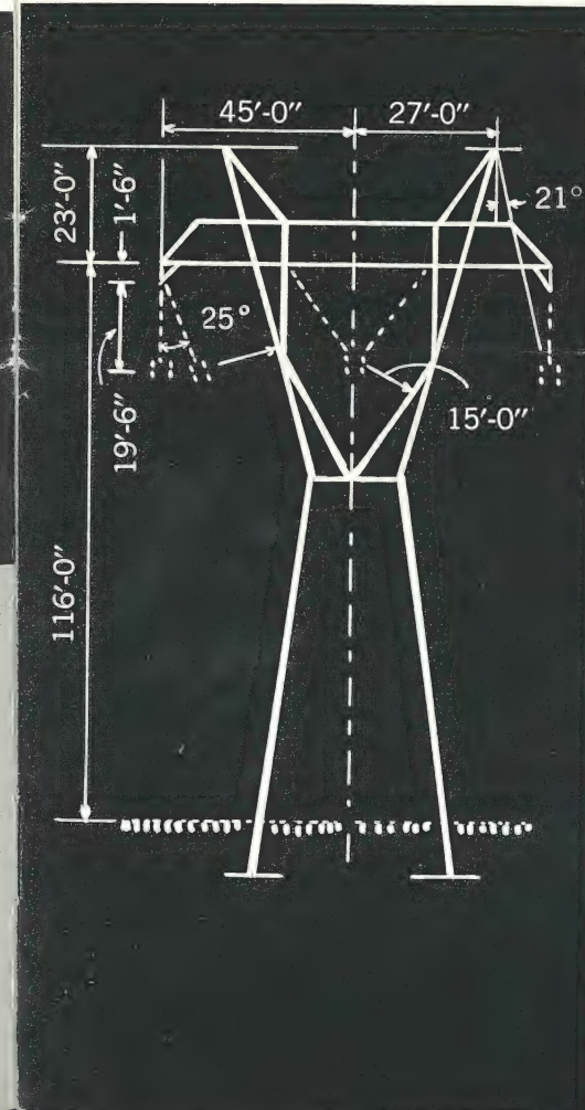
SKETCH B—Dimensioned sketch of tower.
