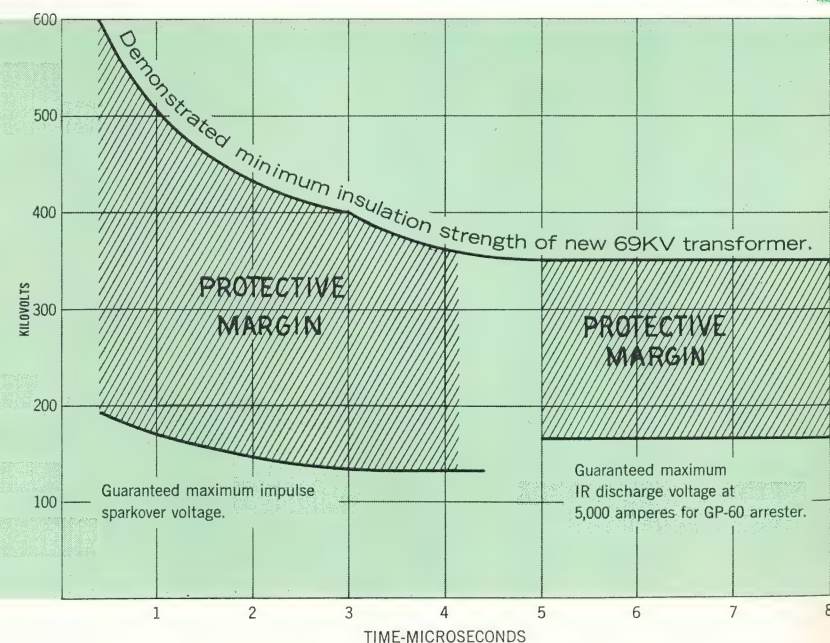
Application of 80% arrester (Thorex GP-60) to a transformer on a 69-kv effectively-grounded neutral system.
