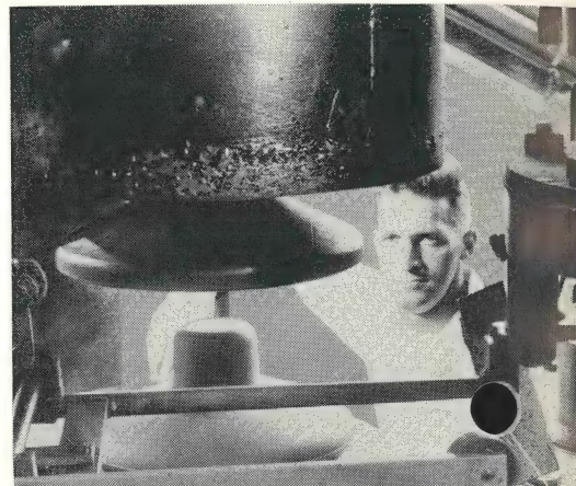
The pug mill extrudes the required amount of clay onto the forming platen, and the exterior (top) shape of the insulator is hot pressed.
