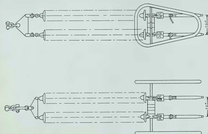
SKETCH E—Quadruple string deadend assembly.
