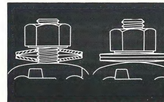
With 10 foot-pounds of torque applied, the Belleville springs flatten, indicating the proper clamping pressure is applied to conductor.
