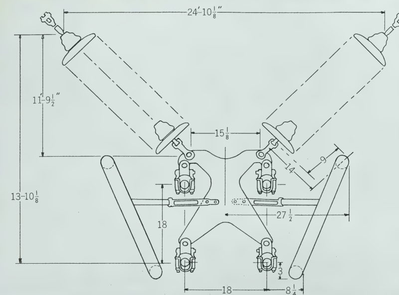
SKETCH C—V-string (center phase) suspension assembly.
