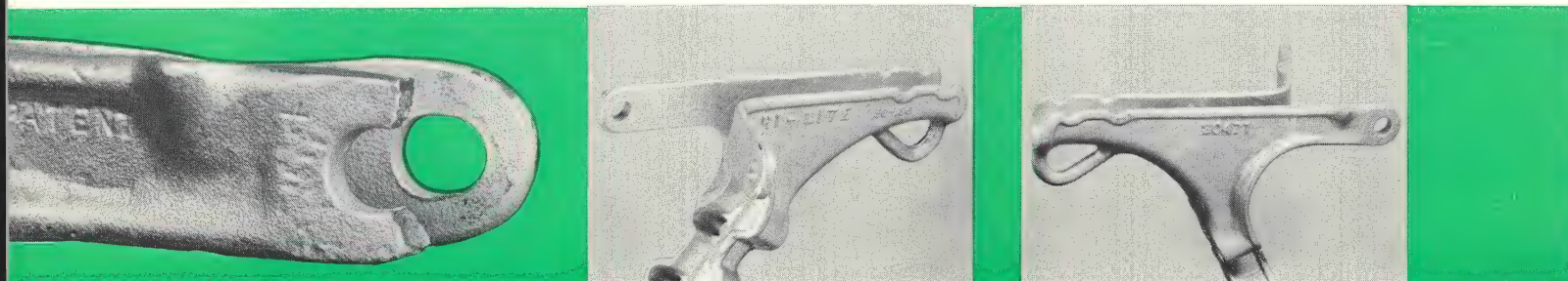
On tensile test, at 25 per cent above published ultimate strength, one clevis connection of this clamp failed. The intact hole has been stretched almost 1/4-inch out of round. This is a graphic demonstration of the elasticity of malleable iron as used in O-B hardware.
