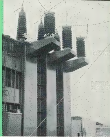
Three O-B Station Class arresters installed directly on a 138 kv transformer in a southern power station are closely connected to the transformer's bushings.
