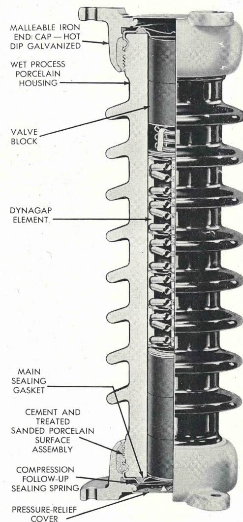
Figure 1 — GP Dynagap intermediate arresters have pressure-sensitive relief system which operates directly as a result of abnormal increases in gas pressure within the sealed arrester.
