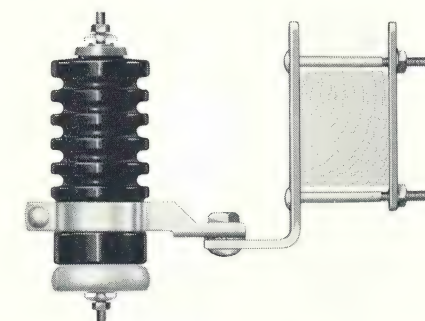
EEI-NEMA crossarm bracket provides sturdy, universal-type mounting facilities for all kv ratings of O-B Multiresters.
