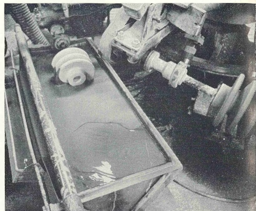
Clay body (left) turns in glazing bath. Notice glazed unit (right) drying on spindle after dipping. This operation on the finishing machine is automatic.
