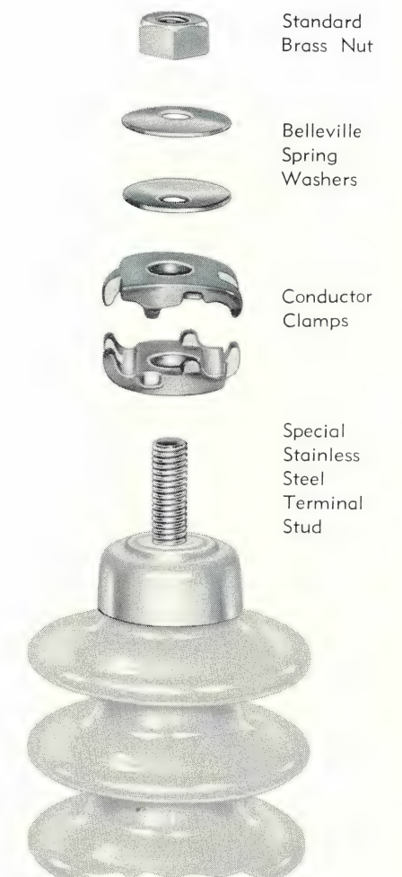
Mark IV Capacitors incorporate field-proved Varex design terminal assembly.
