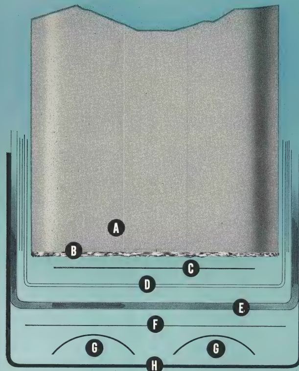
Looking down on one side of a Varex capacitor: Element is (A); extended foil (B); contact plate (C); element separator (D); pack envelope (E); spring carrier (F); springs (G); and capacitor case (H).
