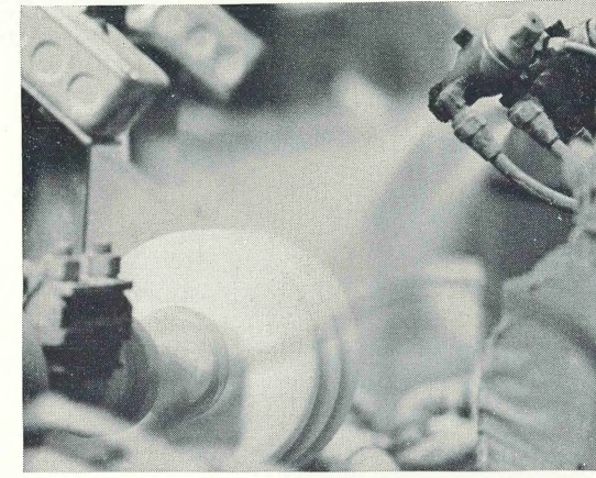
Clay units spin on individual stations as finishing wheel revolves and pauses at production steps such as this spraying operation.
