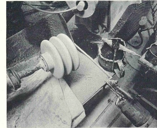
A two-step operation takes place at this station -- application of adherent sand glaze and sand to the rims. This prepares the unit for mating with metal clamptops and mounting bases according to type after the clay body is vitrified.
