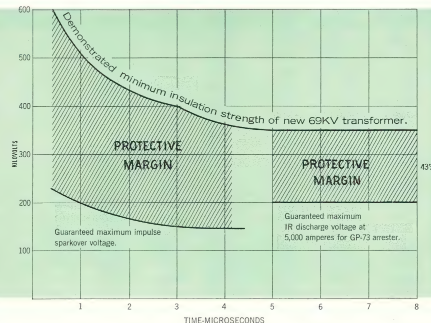
Application of 100% arrester (Thorex GP-73) to a transformer on a 69-kv ungrounded neutral system.
