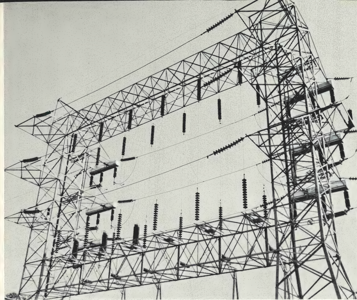
Carrollton Substation of Texas Power & Light is scheduled for 1965 voltage conversion from 69 to 138 kv.
