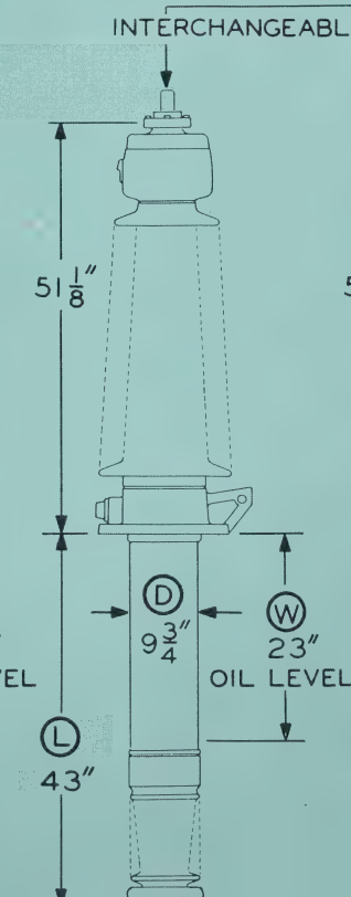
CIRCUIT BREAKER APPLICATION TRANSFORMER APPLICATION INTERCHANGEABLE TERMINALS
