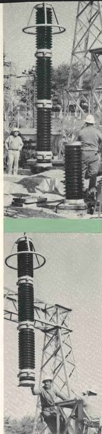
8 The arrester, ready for final installation, leaves the ground.
