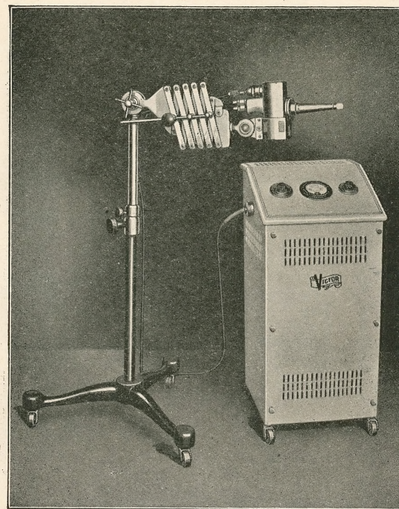
Water-Cooled Outfit, mounted on adjustable floor stand, with extension truss. RECTIFIER control for ALTERNATING current
