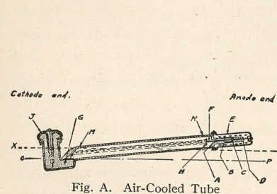
Fig. A. Air-Cooled Tube
