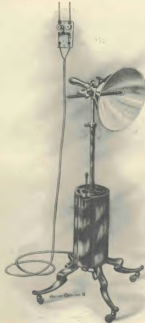
Fig. 18. The Solar Therapeutic Arc Lamp—Latest Model. See page 88.
