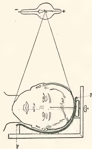
FIG. 160.—AUTHOR'S HEAD REST.—FF, flexible photographic film, conforming to the shape of the skull and employed for locating foreign bodies, etc., in the brain. A lead wire is run from the glabella to the inion and also over the position of the fissure of Rolando.
