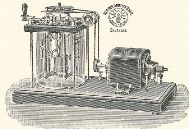
FIG. 71.—Mercury interrupter.
