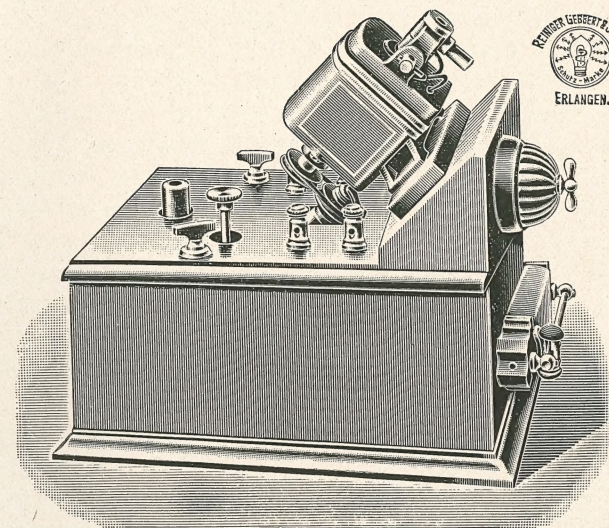
FIG. 72.—Davidson's interrupter.
