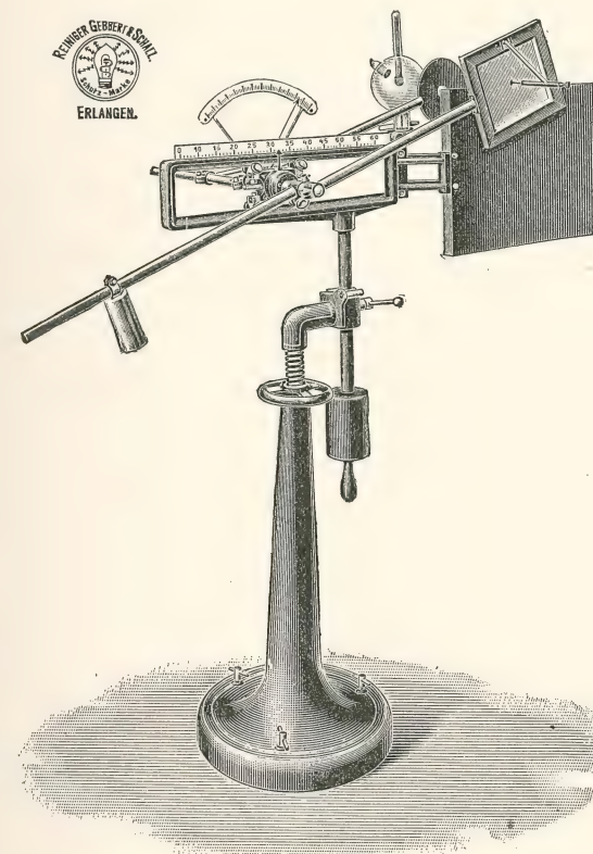
FIG. 181.—Levy-Dorn's orthodiagraph for the standing position.
