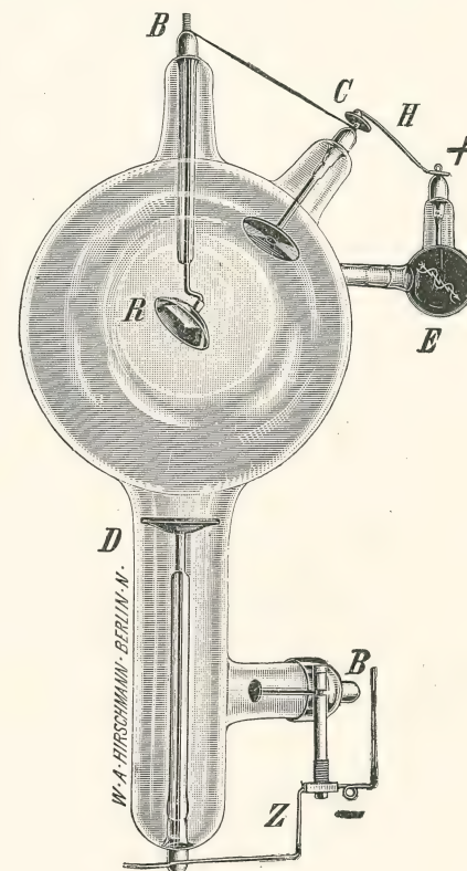
FIG. 91.—Monopol tube. The vacuum may be altered during the process by the generation of air through the disconnection of the movable conductor "Z," or by the absorption of air through the disconnection of the movable conductor "H." The flexible wire "Z" is raised for some seconds by means of an isolated rod until a spark leaps over to the auxiliary cathode at "B," by means of which air is generated and the resistance of the tube lowered. Tubes in which the degree of generation has become excessive are modified by raising the movable conductor "H" as shown in the sketch. Air is generated by the disconnection of the flexible conductor "Z" and the leaping over of sparks to "B," and accordingly the degree of the vacuum in the tube is lowered. Air is absorbed by disconnecting the flexible conductor "H," and the resistance of the tube is increased.
