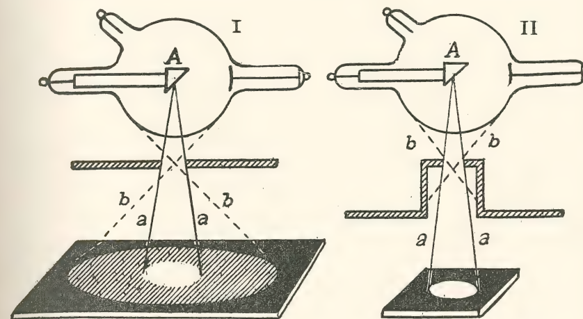
FIG. 98.—Ordinary diaphragm.
