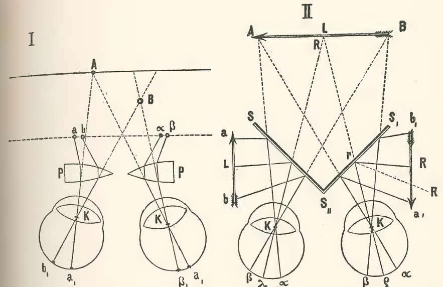
Fig. 111.—Principles of Wheatstone's reflecting stereoscope.
