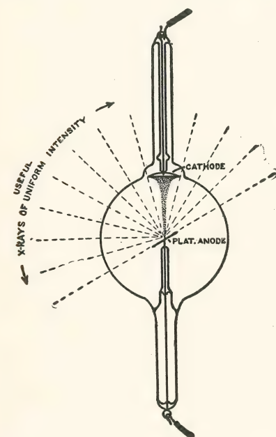
FIG. 88.—Essential features of an X-ray tube.
