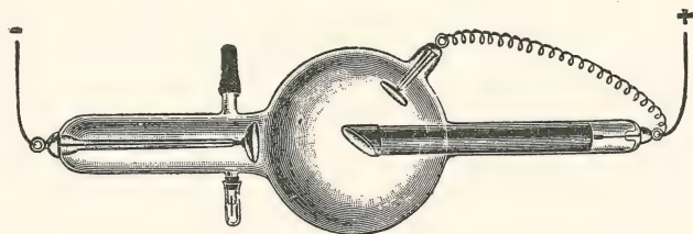
FIG. 92.—Osmosis regulating tube of Gundelach.
