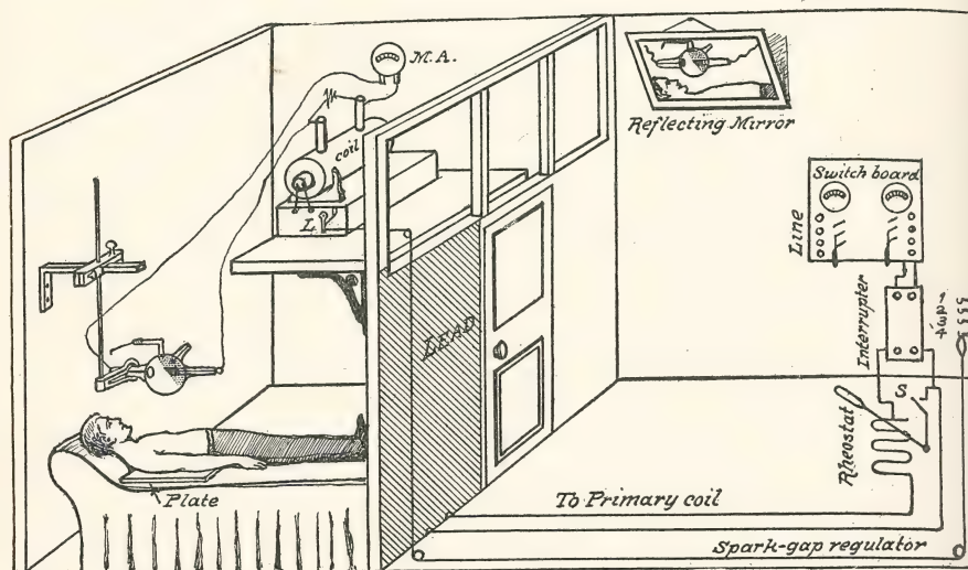
FIG. 210.—Author's scheme for the operator's protection.
