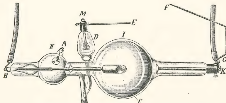
FIG. 214.—Dr. J. Ronsenthal's tube for therapy, as employed by him in the hospitals of Munich.
