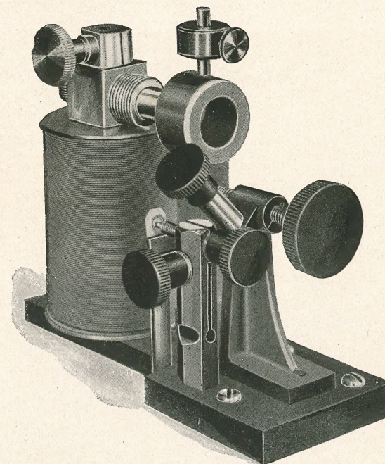
FIG. 69.—Self-starting interrupter.
