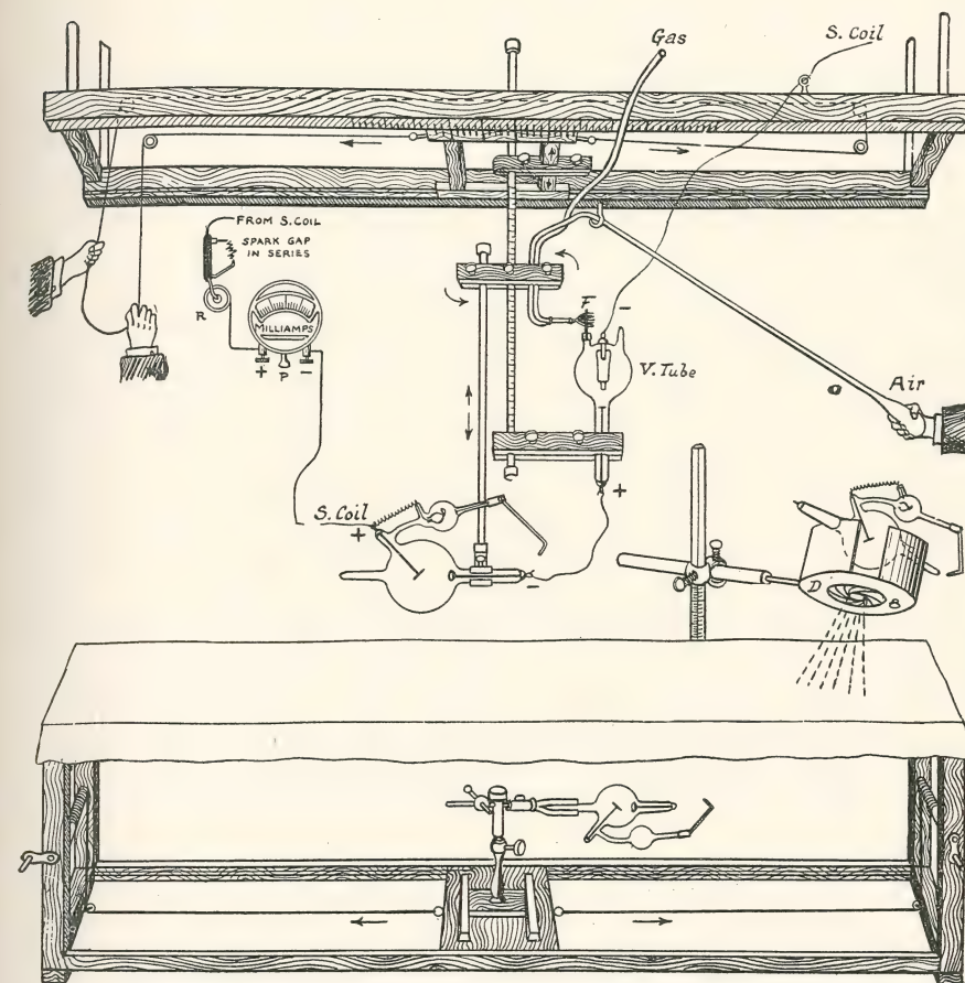
FIG. 100.—AUTHOR'S TABLE AND TUBE-HOLDER.—The pulley moves the tube-holder to and fro. The ventricle tube is connected in series with the Crookes tube and lessens the "reverse current," whose vacuum can be lowered, at pleasure, by the operator compressing, at a distance from the tube, a bulb, which drives a blast of air into a gas flame, thus allowing the heating of the platinum in the ventricle tube.
