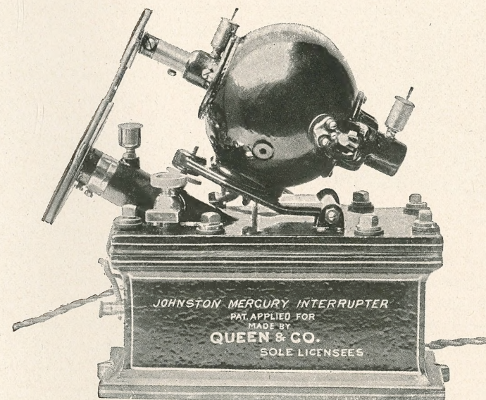
FIG. 73.—Johnston's mercury interrupter.
