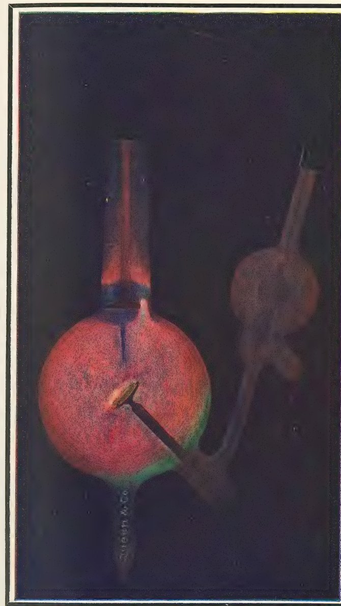
SELF-REGULATING X-RAY TUBE. PUNCTURED OR CRACKED. BULB PARTIALLY FILLED WITH AIR.
