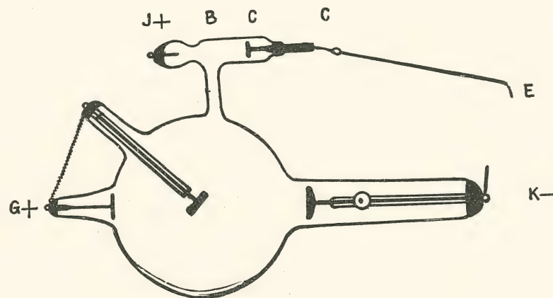
FIG. 90.—Müller's regulation tube.
