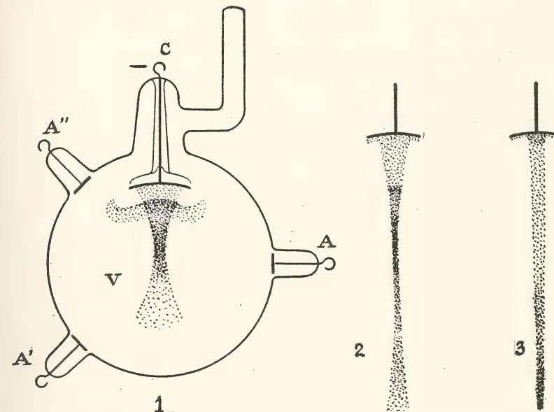
FIG. 86.—Illustrating the effect of one cathode and several anodes under different degrees of vacuum. (Bouchard.)
