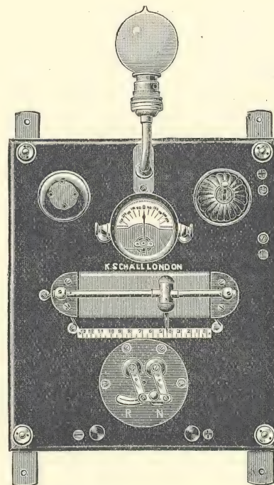
FIG. 56.—GALVANIC SWITCHBOARD.
