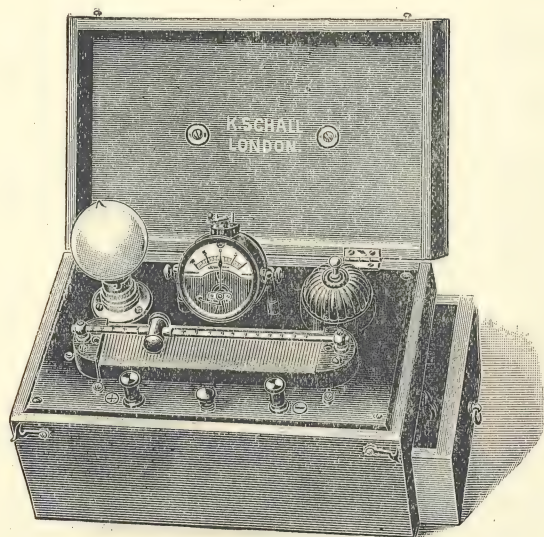
FIG. 57.—RESISTANCE BOX OR PORTABLE SWITCHBOARD FOR GALVANISM.
