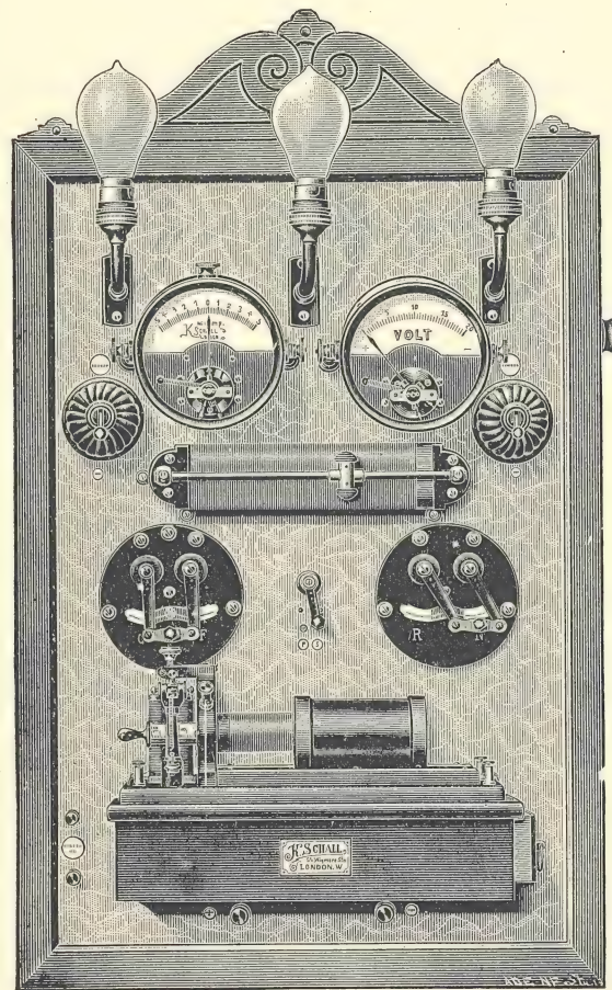
FIG. 55 — COMBINED SWITCHBOARD.
