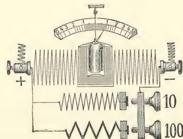
FIG. 25.—DIAGRAM SHOWING TWO SHUNT CIRCUITS OF GALVANOMETER.
