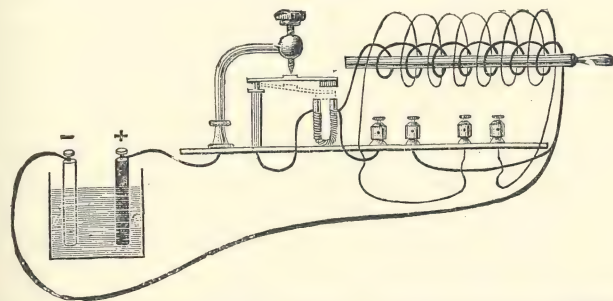
FIG. 43.—DIAGRAM SHOWING PRIMARY AND SECONDARY WINDINGS OF SLEDGE COIL.
