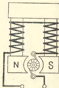
FIG. 53.—SERIES-WOUND DYNAMO.
