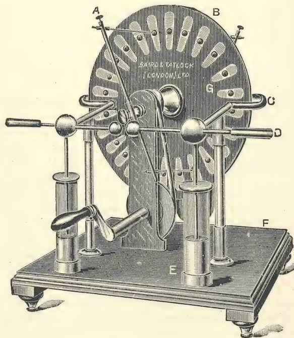
FIG. 1.—THE WIMSHURST MACHINE.
