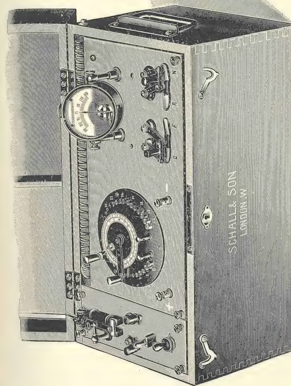
FIG. 49.—COMBINED GALVANIC AND FARADIC BATTERY WITH DOUBLE CELL COLLECTOR AND DE WATTEVILLE COMMUTATOR.
