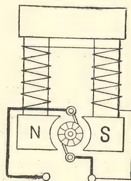
FIG. 52.—SHUNT-WOUND DYNAMO.
