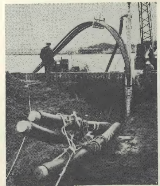
HYDRO-JETTER UNIT: 1-water-pressure hose; 2-injector; 3-plastic conduit to be embedded in river bottom; 4-winch line; 5-free-running conduit coils
