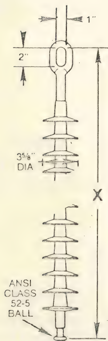
Figure 1 10,000 Lbs. Maximum Design Tension 5/8
