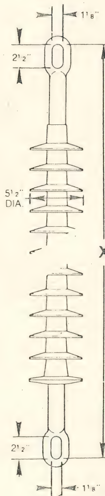
Figure 3 40,000 Lbs. Maximum Design Tension 1 1/4
