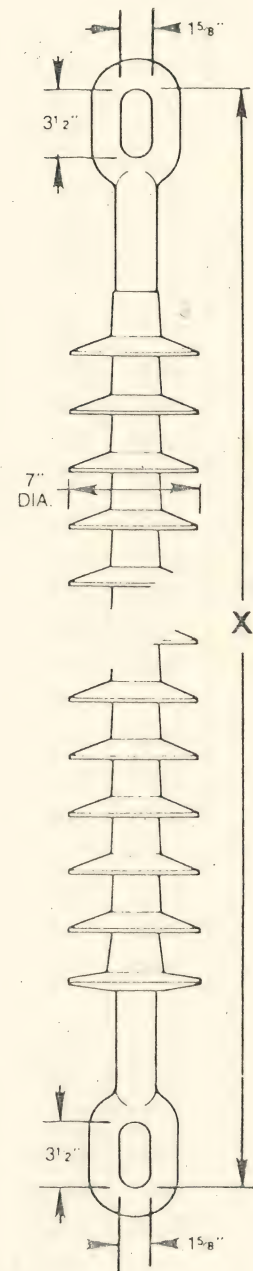
Figure 4 80,000 Lbs. Maximum Design Tension 1 3/4
