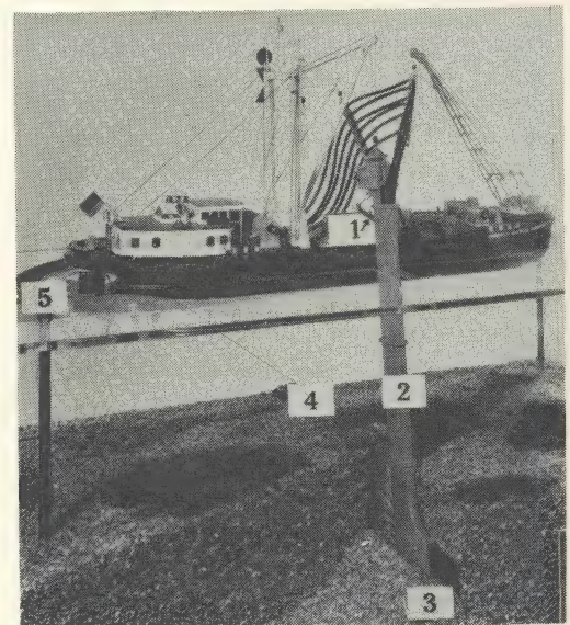
HYDRO-JETTER UNIT: 1-water-pressure hose; 2-injector; 3-plastic conduit to be embedded in river bottom; 4-winch line; 5-free-running conduit coils
