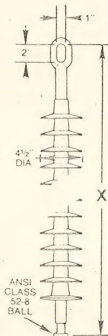
Figure 2 20,000 Lbs. Maximum Design Tension 7/8
