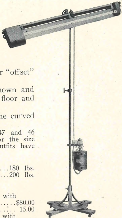
Portrait Outfit No. 49 Equipped with 45 degree Reflector, showing tube horizontal Right hand Outfit
