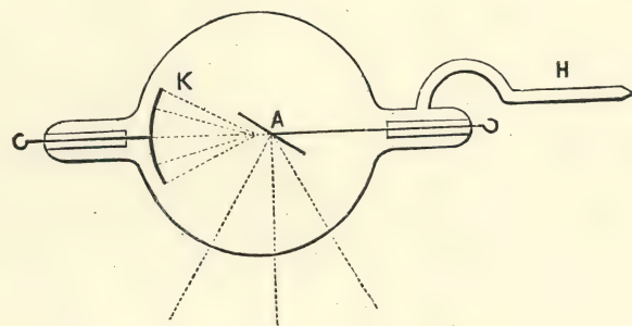
TYPICAL FOCUS TUBE.
