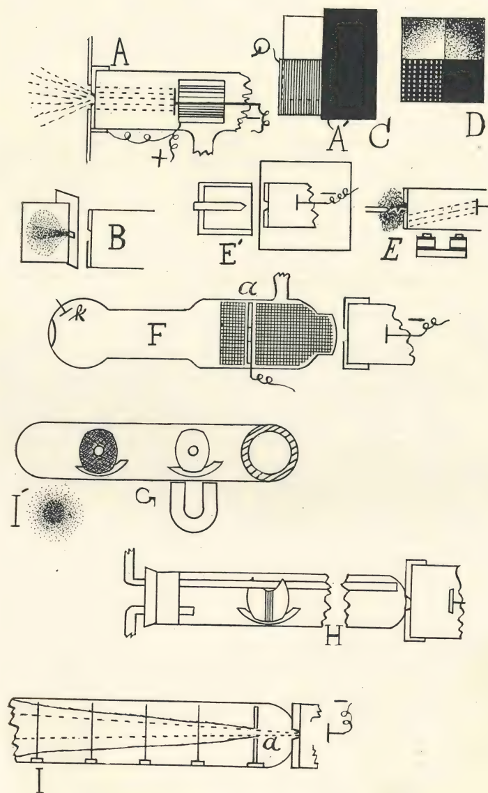
DIAGRAM OF LENARD'S APPARATUS. pp. 53 to 69.
