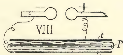
ARRANGEMENTS FOR TAKING ELECTROGRAPHS. § 35, p. 19.
