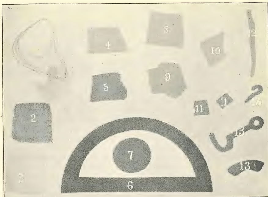
FROM MAGNETOGRAPHS BY PROF. MCKAY. p. 25.
