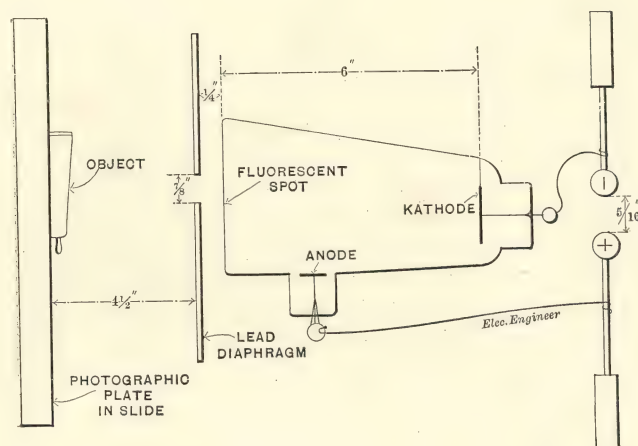
RICE'S EXPERIMENT. FIG. 1, § 106, p. 99. Diagram.
