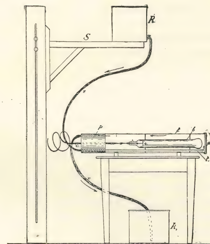
DISCHARGE TUBE IMMERSSED IN OIL, § 147, PAGE 156.
