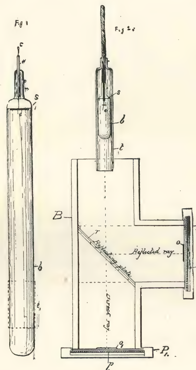
TESLA'S FIGS. 1 AND 2, REFLECTION AND TRANSMISSION OF X-RAYS BY DIFFERENT SUBSTANCES. § 145 and § 146a.
