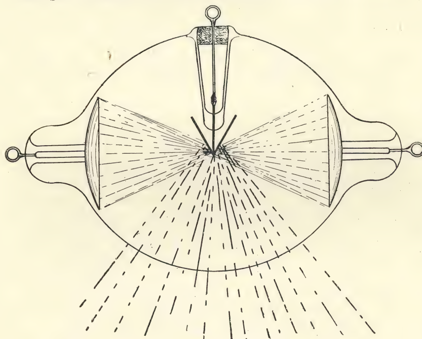
STANDARD X-RAY TUBE.
