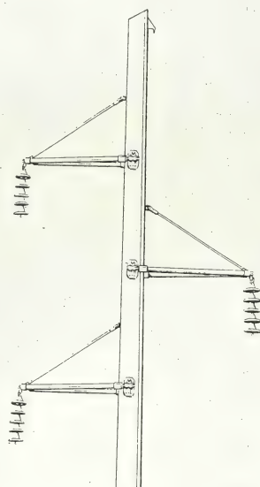
Fig. 20. Planned installation of ECA crossarms for single-pole construction in project to convert existing 44-kV circuit to 161 kV.
