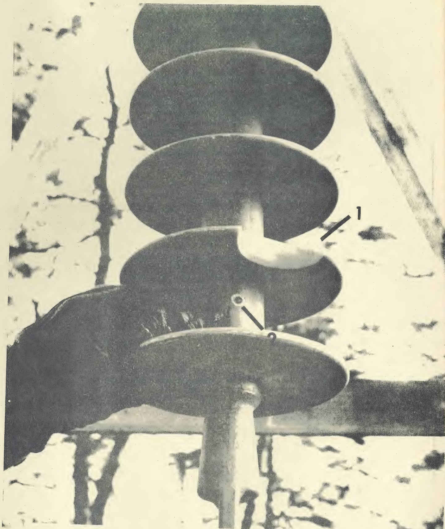
Locke Polymer - 22 long rifle - broke hood - no apparent damage to center column (2 shots).
