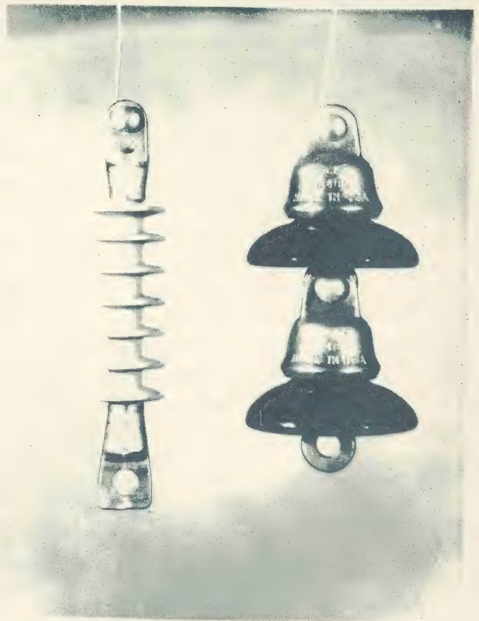
Figure 13. The 15 KV distribution GEPOL insulator compared with its porcelain counterpart.
