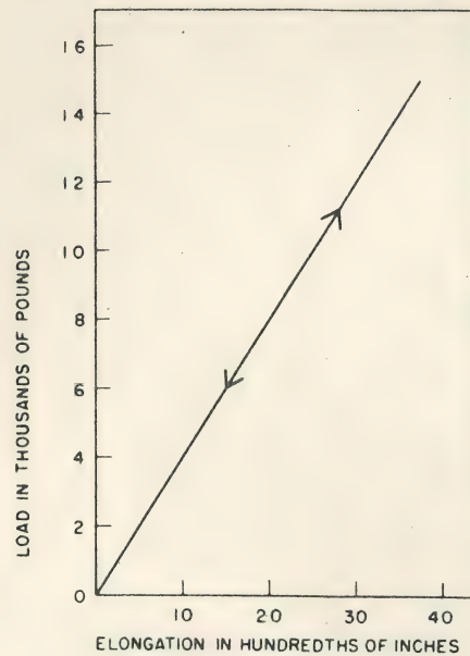
Fig. 13. Elongation of the Polymer Insulator showing its elastic properties.
