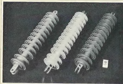
Fig. 14. 25kv trolley line resin insulator
