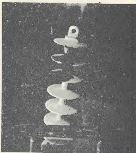
Fig. 7. Insulator damaged in laboratory test by special burning test with leakage current.
