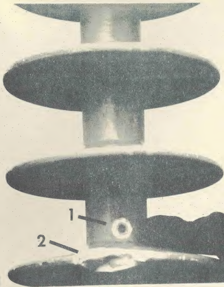
Locke Polymer - 45 cal. pistol - broke hood - no apparent damage to center column (2 shots).
