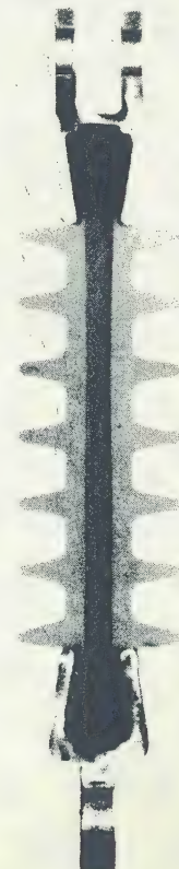
Fig. 4 - 15KV Polymer Insulator Cross-section
