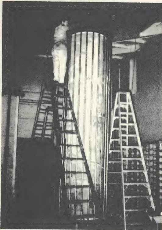
11. Epoxy Fiber Glass Core for 500 Kv Insulator - Pressure Test
