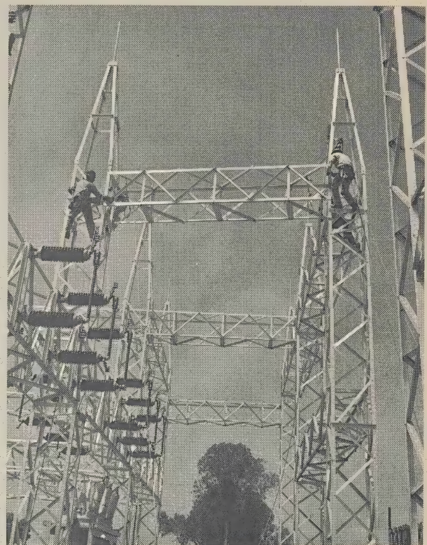
Installation of Type "S" Side-break switches in a Chance aluminum substation
