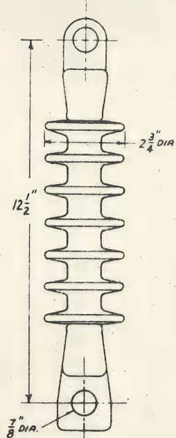
FIG. 12 --- 15 KV POLYMER STRAIN INSULATOR
