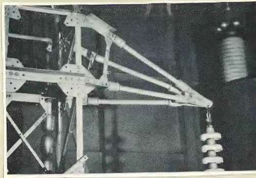
Fig. 16. FRP arm for transmission tower
