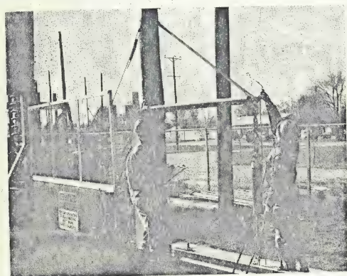
Fig. 14. Six-foot ECA crossarm undergoing cantilever test.
