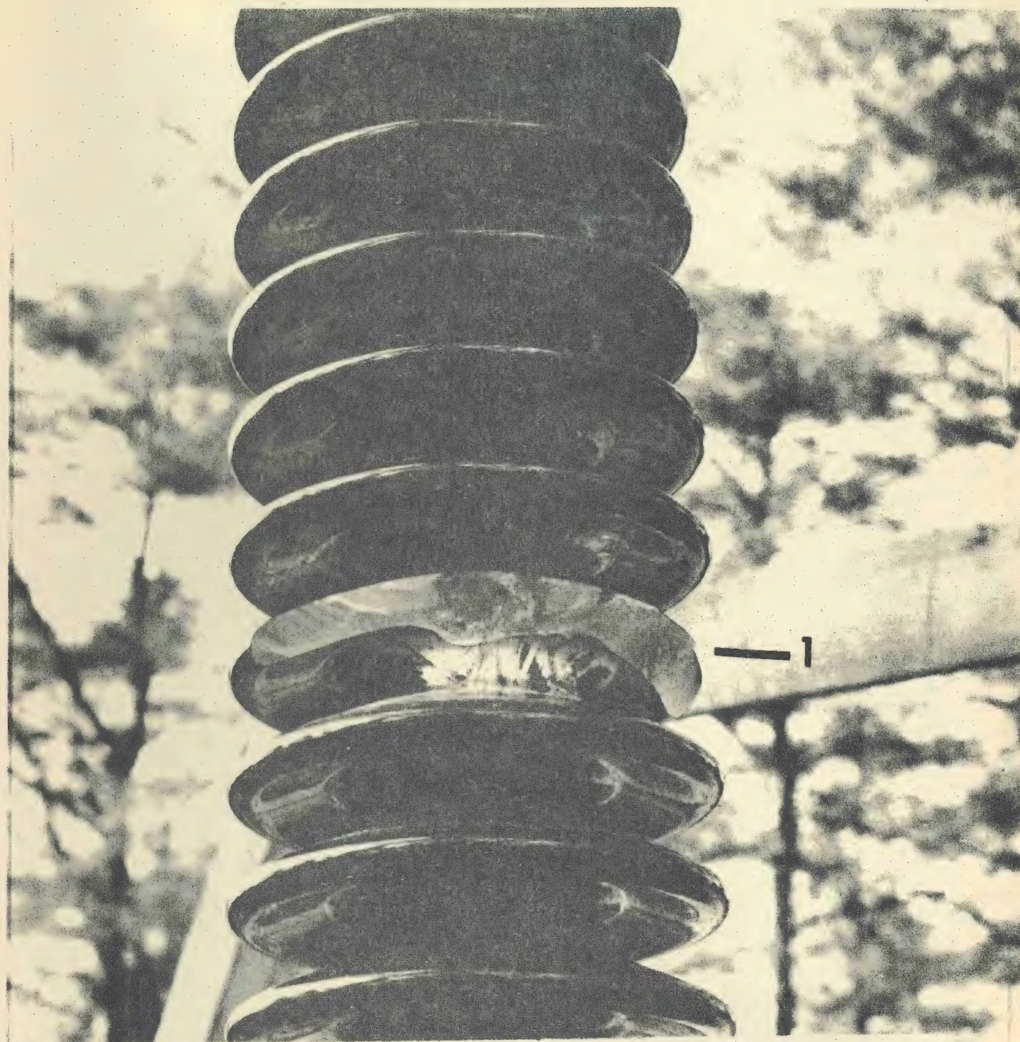
Lapp Strut - 22 long rifle - broke hood - no apparent damage to center column (1 shot).
