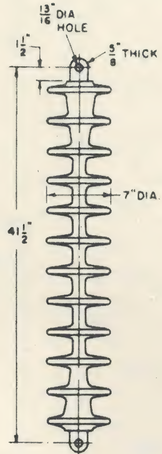
FIG. 6 --- 115 KV POLYMER SUSPENSION INSULATOR
