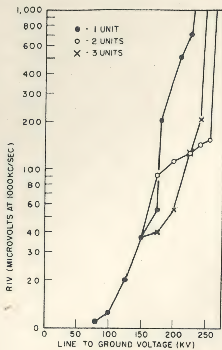
Fig. 5. Radio influence voltage curves of polymer insulators.
