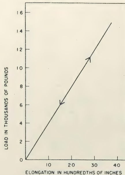
Fig. 13. Elogation of the Polymer Insulator showing its elastic properties.
