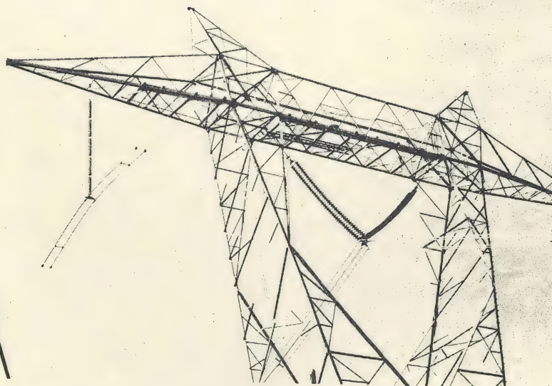
Fig. 6. 700 kv tower with five polymer insulators mounted for switching surge tests.
