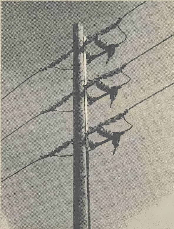
Chance 27 kv "D" Switch and Interrupter side-mounted on 3-phase aluminum support
