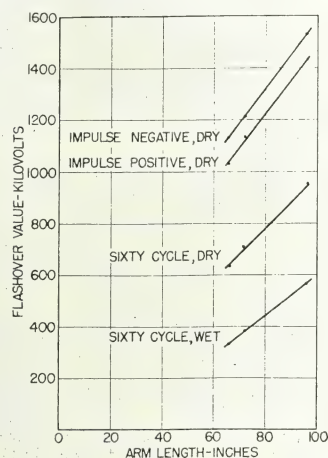
Fig. 5. Impulse and 60-Hz flashover values of several ECA crossarms. All tests conducted with five suspension insulators. Data corrected to standard atmospheric conditions.
