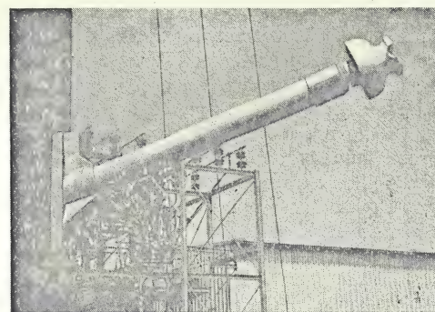
Fig. 3. Standoff type ECA for service through 34.5 kV. Electrical characteristics: 60 Hz flashover—283 kV dry, 162 kV wet. Impulse flashover—436 kV positive, 493 kV negative.
