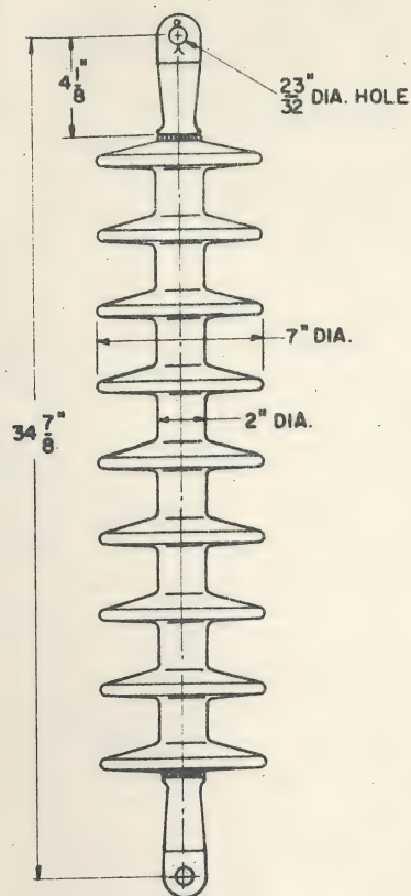
FIG. 1 --- 69 KV POLYMER SUSPENSION INSULATOR
