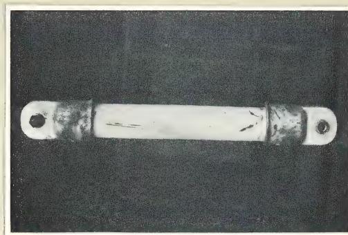
Fig. 17. FRP specimen insulator for transmission tower member
