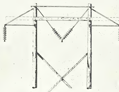
Fig. 19. Planned structure conversion for upgrading existing 115-kV line to 230 kV, utilizing ECA crossarms.
