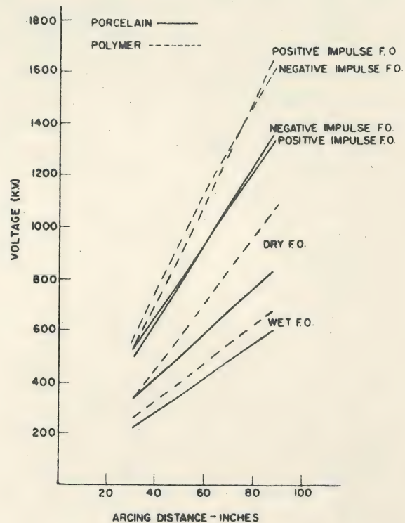
FIG. 2 --- A COMPARISON OF THE ELECTRICAL CHARACTERISTICS OF POLYMER INSULATORS WITH RATED VALUES OF PORCELAIN SUSPENSION INSULATORS 10" IN DIAMETER, 5-3/4" SPACED
