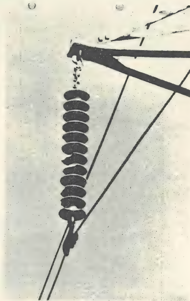
Fig. 6. Insulator on Boston Edison Co. system damaged by rifle fire.
