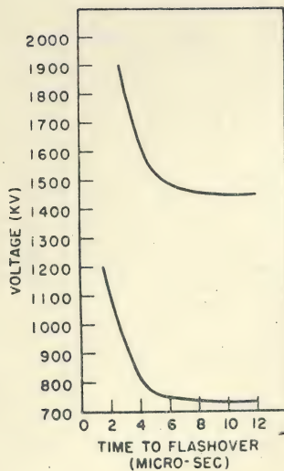
Fig. 8. Volt time curves for one and two polymer insulators, positive polarity.
