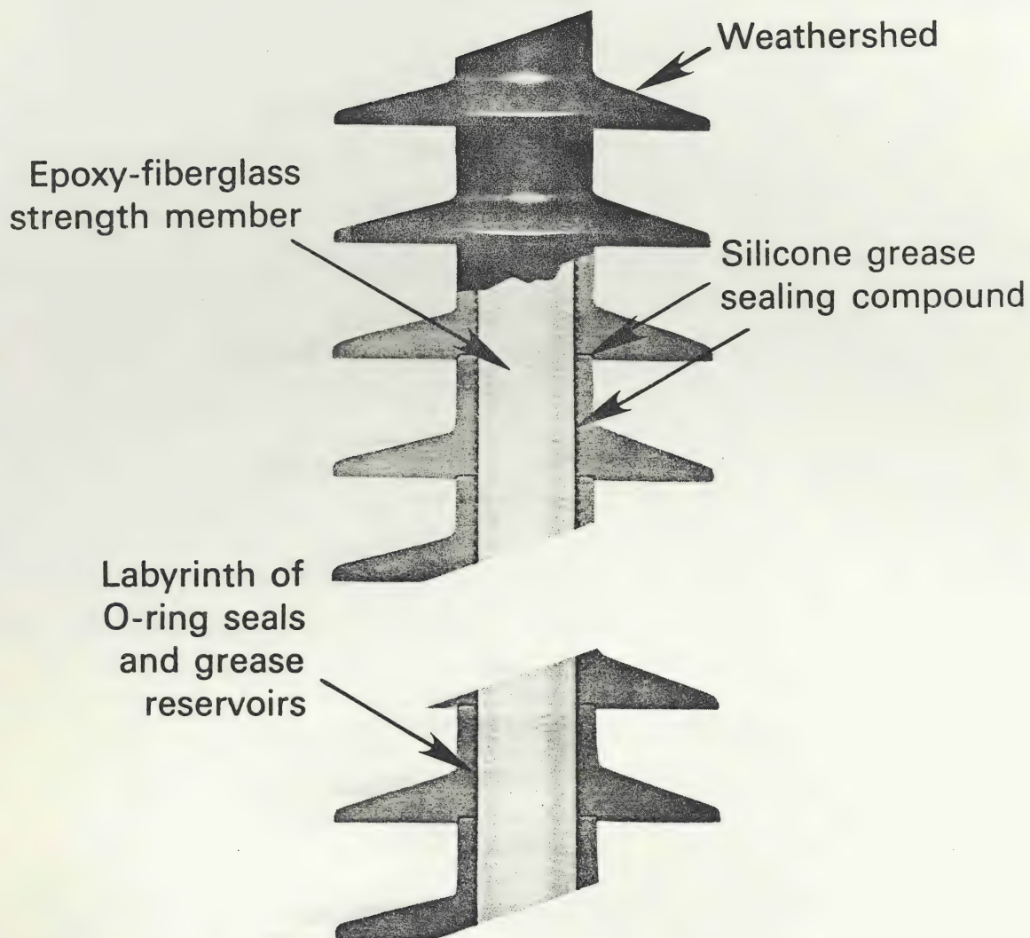
Schematic cross section of Hi-Lite insulator, showing general construction and detail of interface sealing system.
