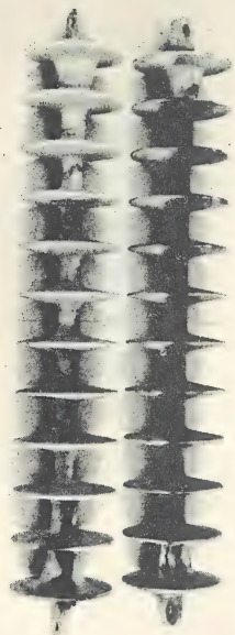
Fig. 5. Insulators returned from Tampa Electric Co. contaminated in service with heavy coating of phosphate and burned by leakage currents.
