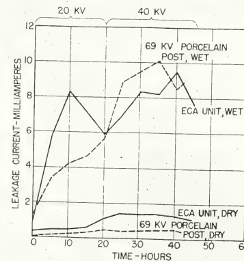
Fig. 10. Leakage current variation as a function of time during wet cycling tests for ECA of Fig. 4.
