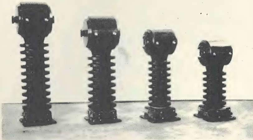
17. Current Transformer with Butyl Insulation
