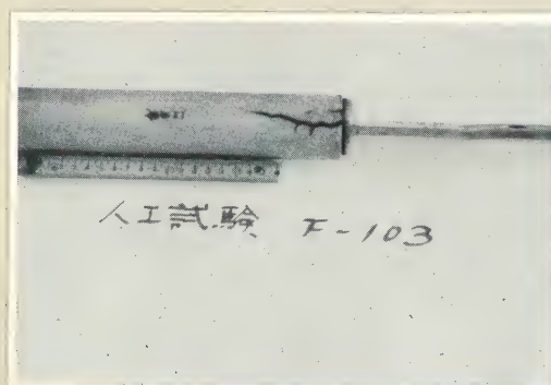
Fig.11. Tracking observed on No.6 specimen, cycloaliphatic epoxy resin, by water spraying leakage current test.
