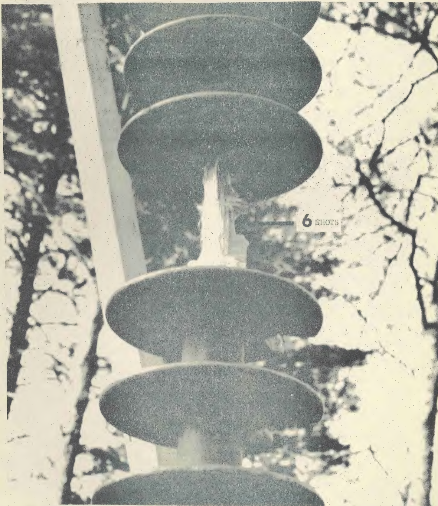
Locke Polymer - M-1 rifle - broke hood, stripped cast epoxy from glass fibre core, and broke some strands of glass fibre (6 shots).
