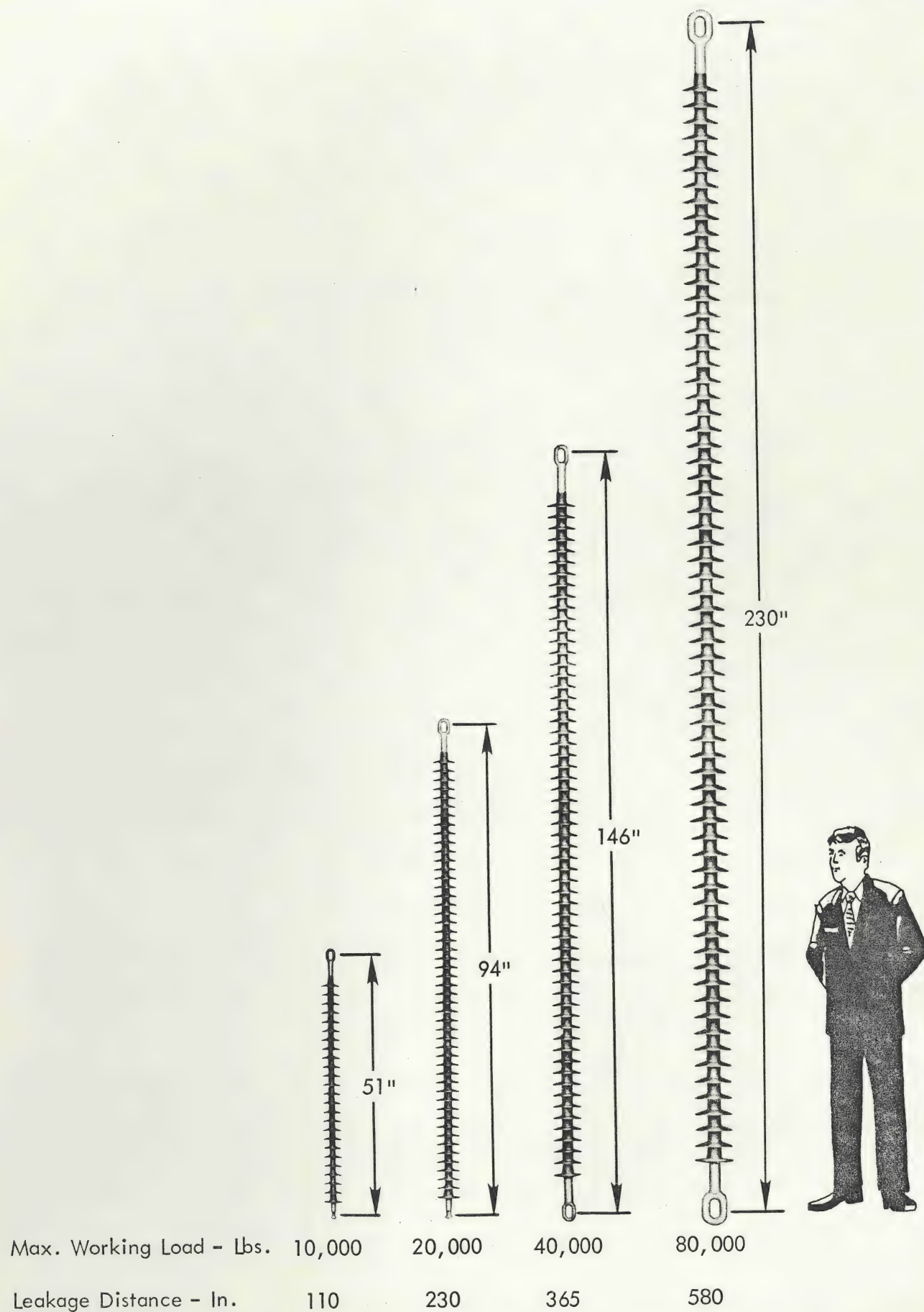
FOUR STRENGTH CLASSES OF O-B HI-LITE SUSPENSION INSULATORS
