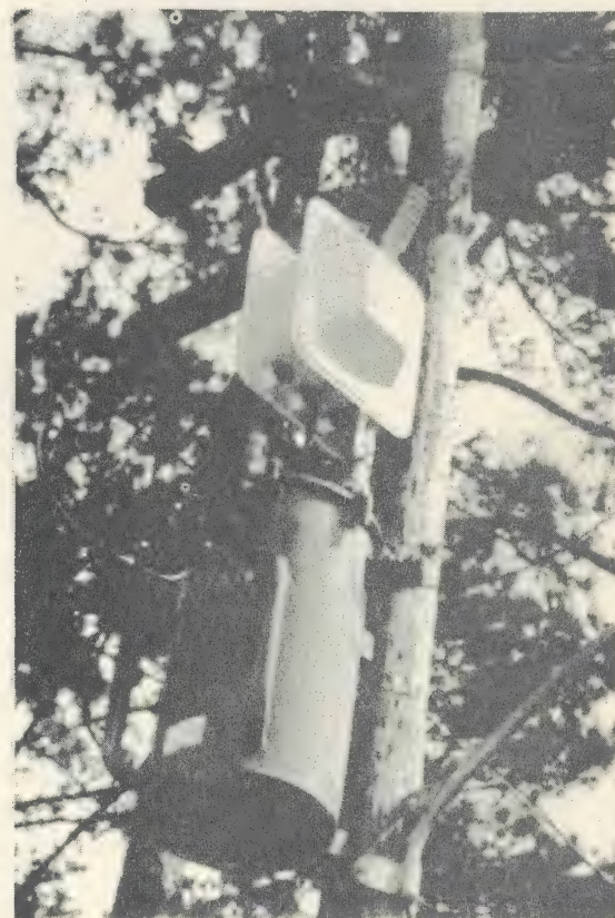
FIG. 23 --- 25 KVA TRANSFORMERS. NOTE EPOXY BUSHING ON TOP TRANSFORMER
