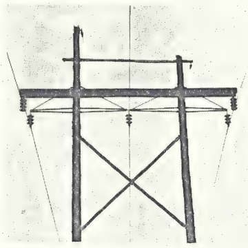
Fig. 18. Field test of ECA crossarms at 110 kV on existing H-frame construction.
