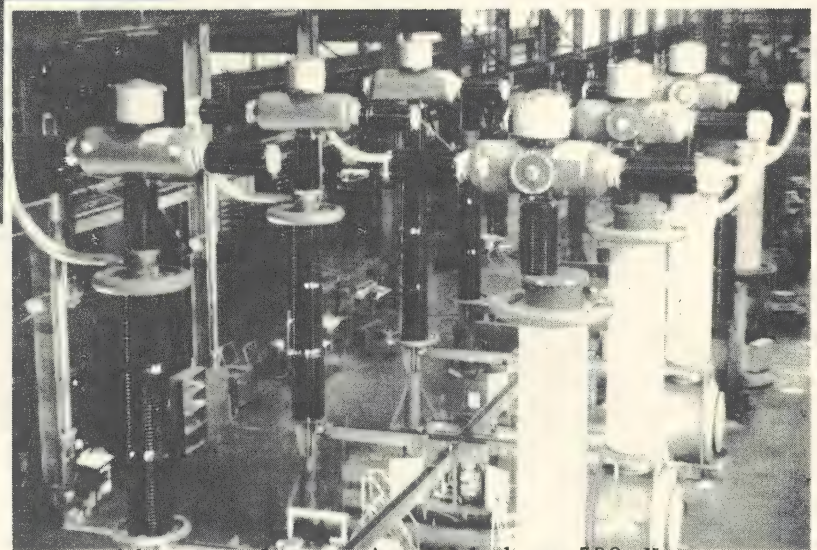
16. Insulators Assembled on 500 Kv Air Blast Breaker - Philadelphia
