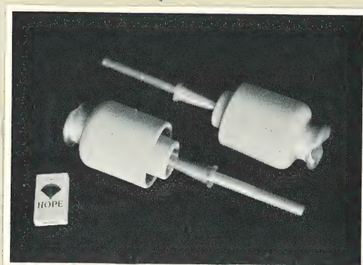
(c) 6 kv pin type insulator (fog type)
