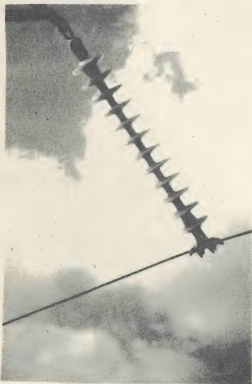
FIG. 10 --- INITIAL INSULATOR PUNCTURE AT BROWNSVILLE, TEXAS, SITE
