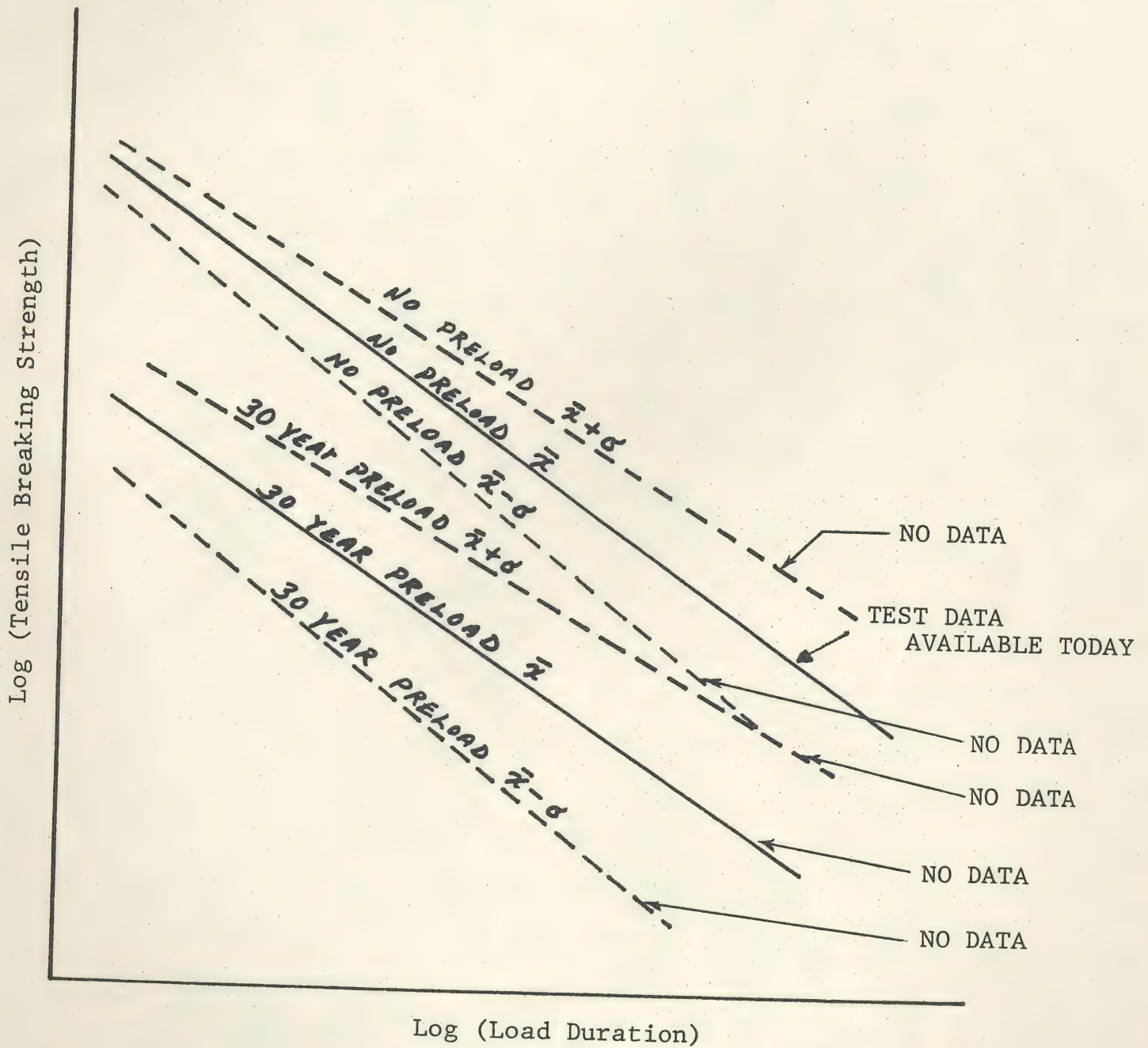
Figure 1. Hypothetical Load Duration - Strength Curves for Non-Ceramic Insulator
