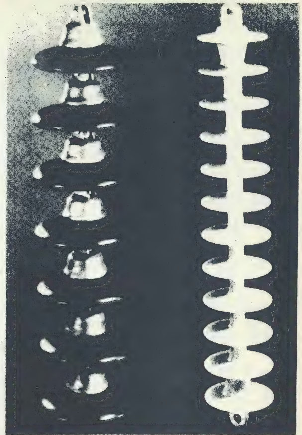
Fig. 2 - 115KV Insulators - Porcelain and Polymer
