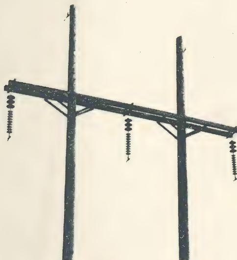
Fig. 7. Polymer Insulators in series with standard porcelain suspension insulators on a 115 kv line of The Baltimore Gas and Electric Company.
