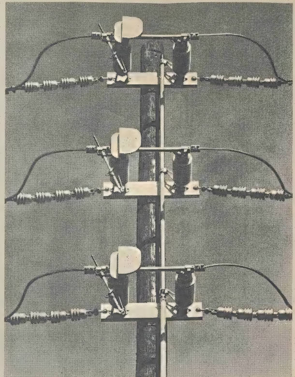
Side-mounted phase-over-phase Chance 34.5 kv "DP" Switch with Saf-T-Gap expulsion Interrupter
