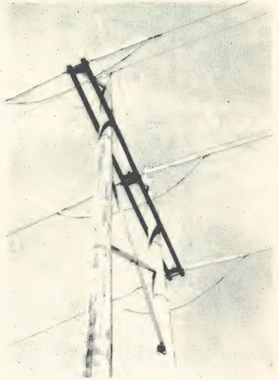
2. Polymer Insulators - Baltimore Gas & Elec. Co. 110 Kv
