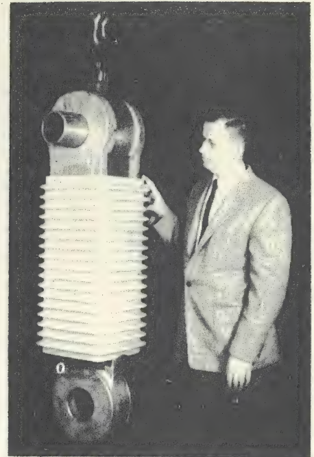
10. Polymer Antenna Insulator - 1 Million Lb. Strength
