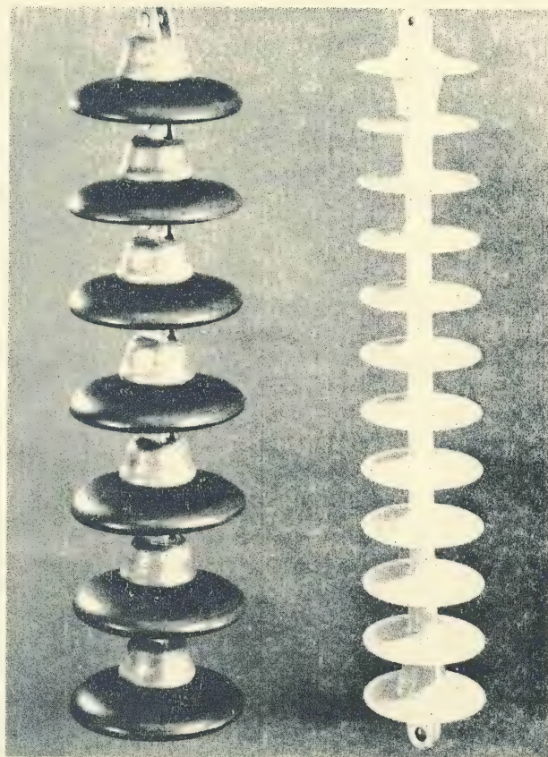
Fig. 2. Polymer insulator compared with a string of (7) seven suspension insulators.
