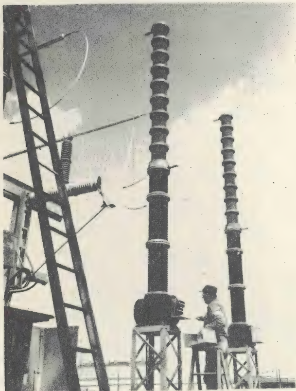
FIG. 22 --- STACK OF NINE POLYMER VACUUM INTERRUPTER HOUSINGS BEING INSTALLED
