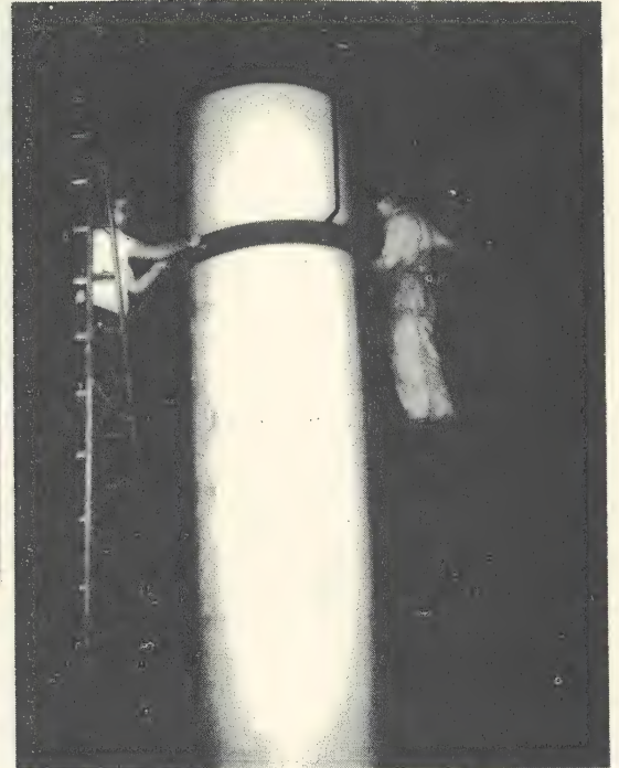
14. 500 Kv Insulator - Preparation for Electrical Tests
