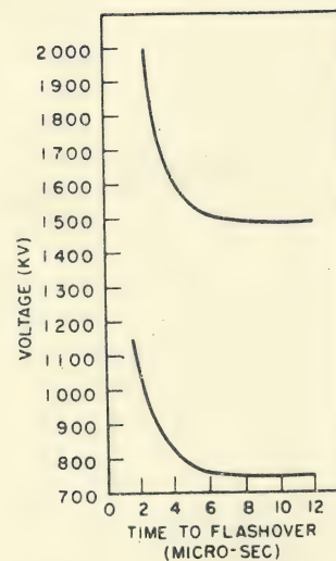
Fig. 9. Volt time curves for one and two polymer insulators, negative polarity.
