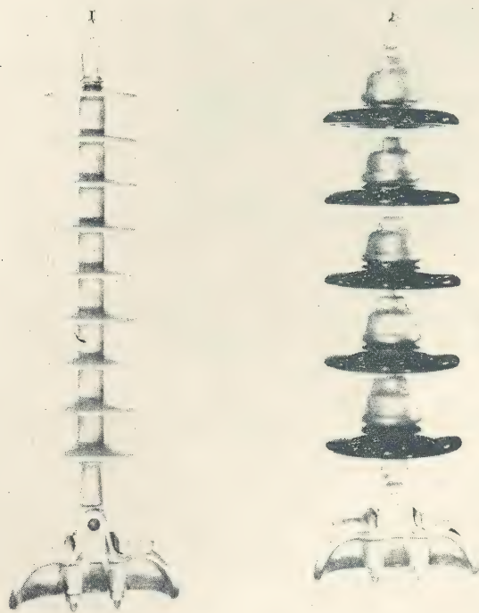
Fig. 1. Polymer Insulator compared with a string of five suspension insulators 10" in diameter, 5-3/4" spaced.
