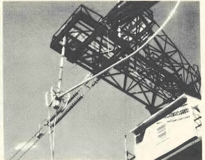
4. Polymer Insulators - Pittsfield EHV Project
