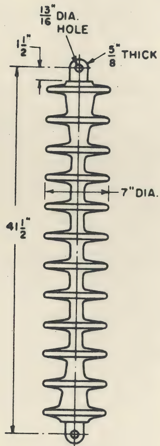
Fig. 1. Outline drawing of the polymer insulator.
