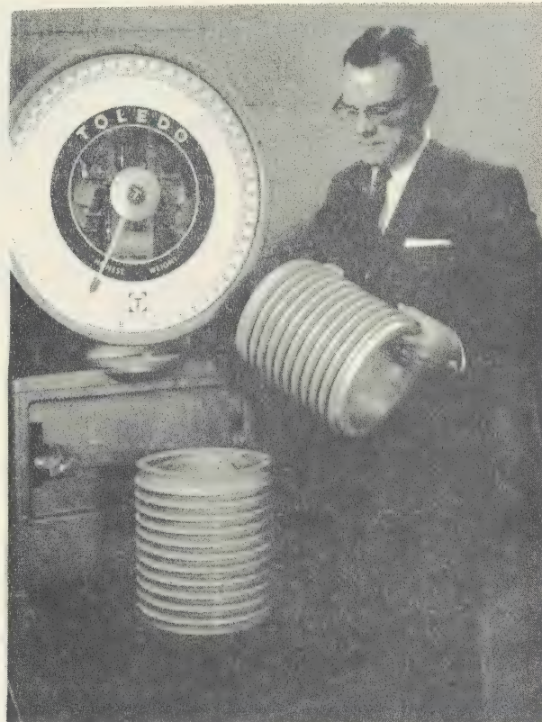
FIG. 21 --- 230 KV POLYMER VACUUM INTERRUPTER HOUSINGS
