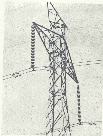
A 60-day insulator wash schedule is used on this tower in the 15-mile section of HVDC transmission line in Sylmar. Los Angeles Department of Water and Power selected the tower for long-term tests of silicone-coated insulator strings.
