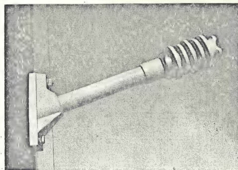
Fig. 4. ECA unit with suggested upper limit for application, at present, of 46 kV. See Fig. 8 for electrical characteristics.
