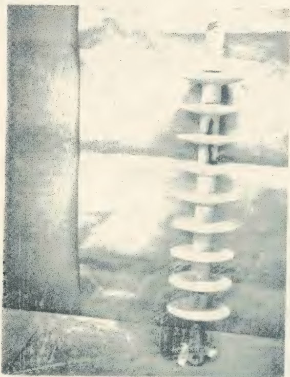
Figure 4. 69 KV Insulator after seven years of service in a salt contaminated area.
