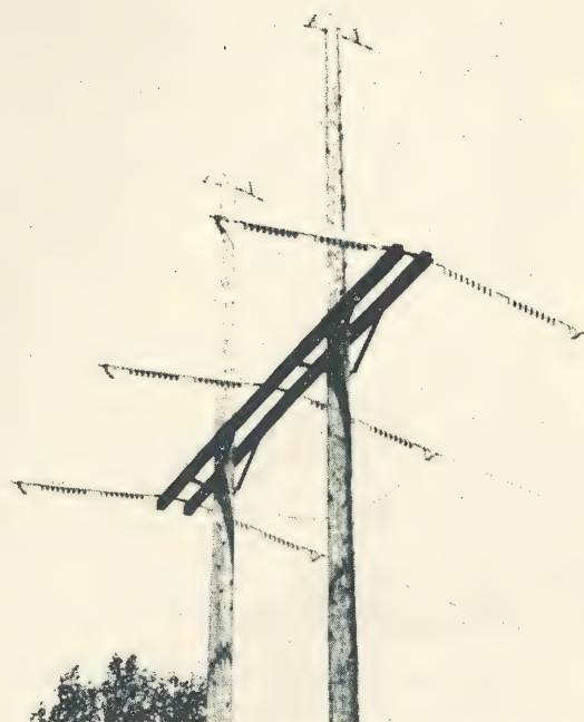
Fig. 6. Polymer Insulators installed on a 115 kv line of The Baltimore Gas & Electric Company.
