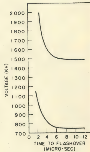
Fig. 9. Volt time curves for one and two polymer insulators, negative polarity.
