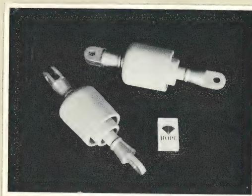
(b) 6 kv strain insulator (fog type)
