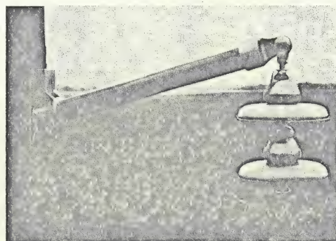
Fig. 2. ECA suspension unit intended for application at voltage up through 69 kV. Electrical characteristics: 60-Hz flashover—268 kV dry, 213 kV wet. Impulse flashover—456 kV positive, 601 kV negative.
