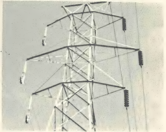
6. Stringing Conductor - GEPOL Insulators - Duke Power Co. 100 Kv
