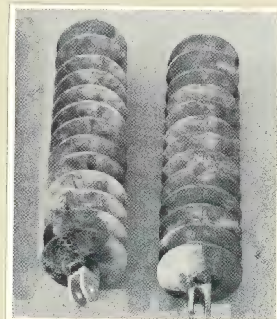
(b) Resin insulators after power arc test, Insulators are traced by fuse wire vaporization
