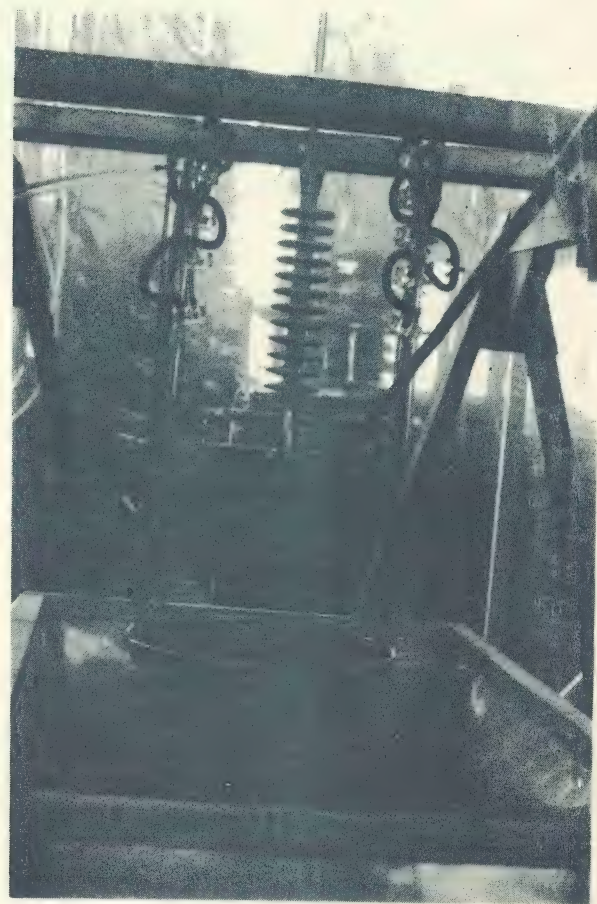
Figure 10. The salt-sugar spray test as run in the R&D Center on a 34 KV GEPOL insulator.
