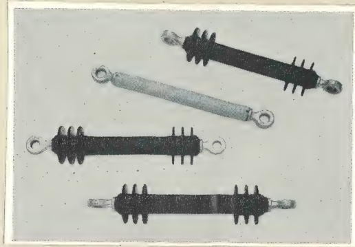
Fig. 18. Strain insulator for trolley line
