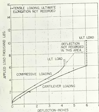
Fig. 13. Mechanical characteristics of 6-foot ECA crossarm.
