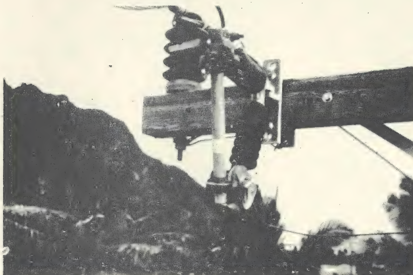
20. Cutout with Butyl Insulation in Service
