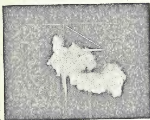
Fig. 15. Power follow test of 6-foot ECA crossarm at 23 000 amperes.
