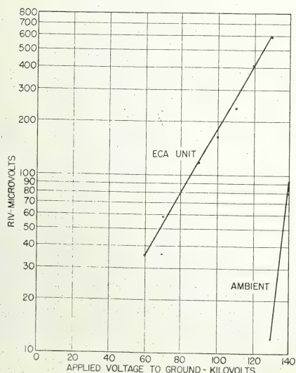
Fig. 7. Radio influence voltage characteristic of 72-inch ECA crossarm with five suspension insulators at 1000 kHz.
