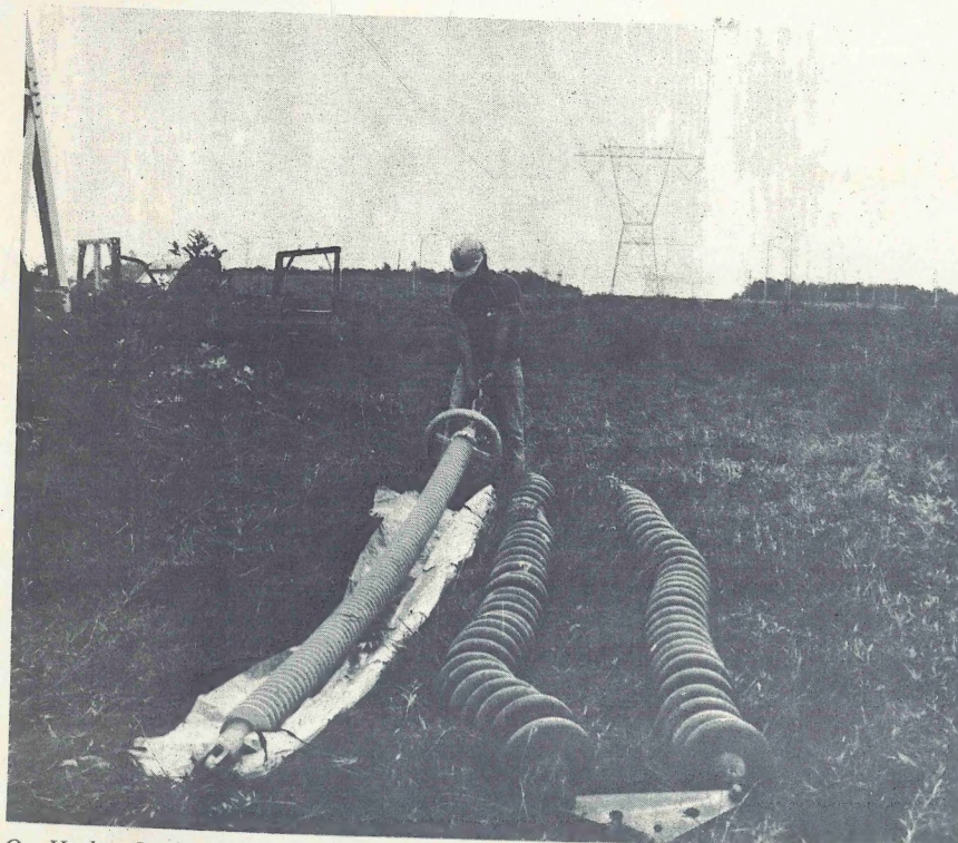
On Hydro-Quebec's 735-kv transmission lines a single element synthetic insulator weighing only 32 kilograms may replace two-string porcelain insulators (right) weighing 548 kilograms.
