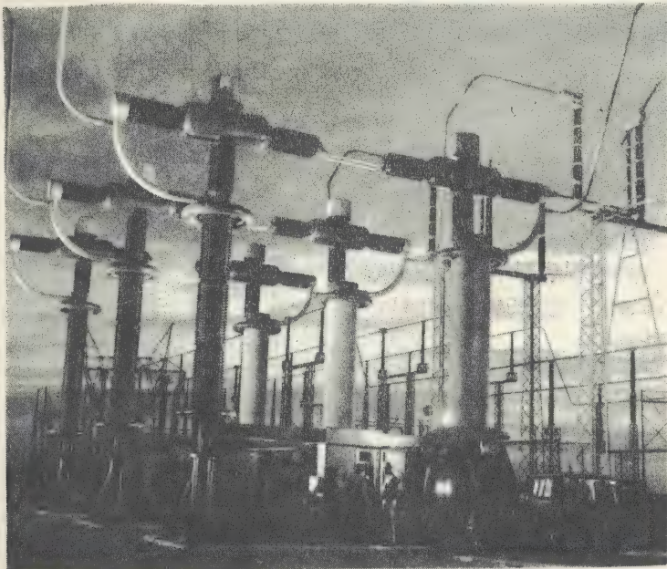
FIG. 20 --- 500 KV AIR BLAST BREAKER WITH 15 FT. POLYMER INSULATORS
