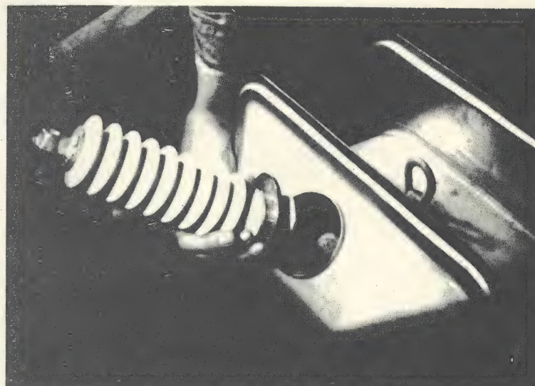
22. Polymer Bushing on "SEAL PAC" Transformer
