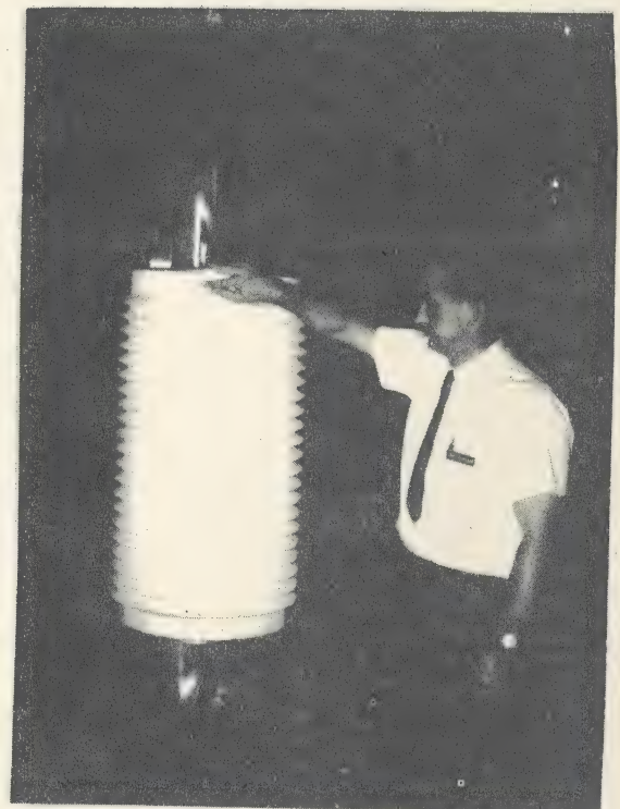
FIG. 19 --- POLYMER RADIO ANTENNA GUY INSULATOR
