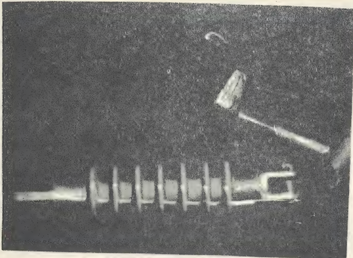
FIG. 16 --- DEMONSTRATION OF POLYMER INSULATOR'S HIGH IMPACT RESISTANCE
