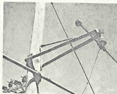
Fig. 11. Six-foot ECA crossarm with one 6-inch suspension insulator undergoing sustained 60-Hz test at 80 kV. Unit has been energized since November 1963.
