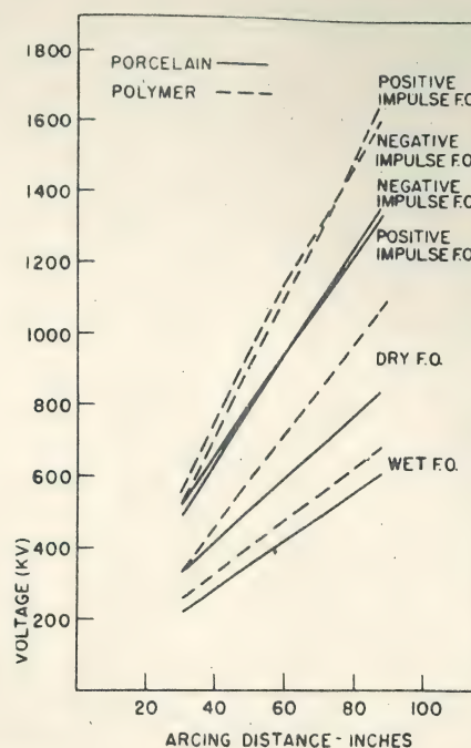
Fig. 2. A comparison of the electrical characteristics of Polymer Insulators with rated values of porcelain suspension insulators 10" in diameter 5-3/4" spaced.
