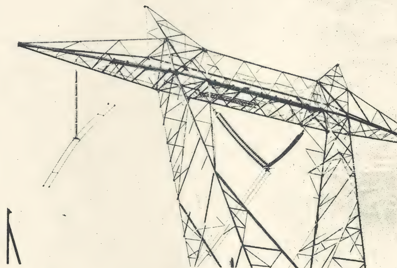
Fig. 6. 700 kv tower with five polymer insulators mounted for switching surge tests.
