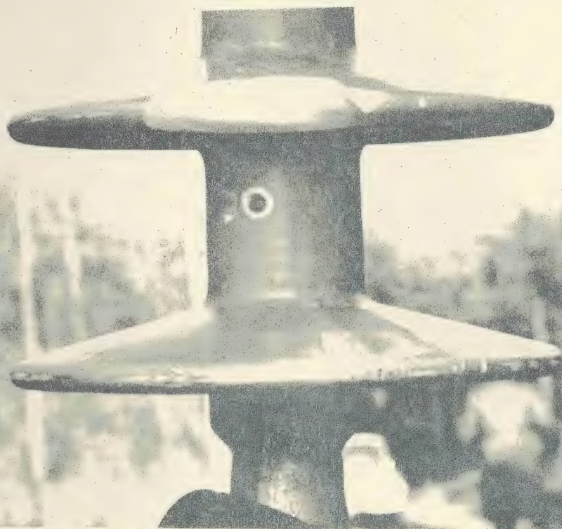
Locke Polymer - 45 cal. pistol - broke hood - no apparent damage to center column (2 shots).
