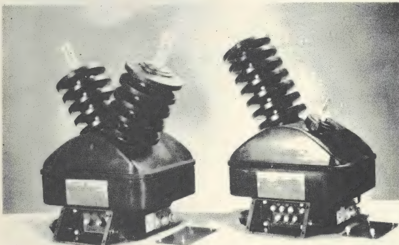
18. Potential Transformer with Butyl Insulation
