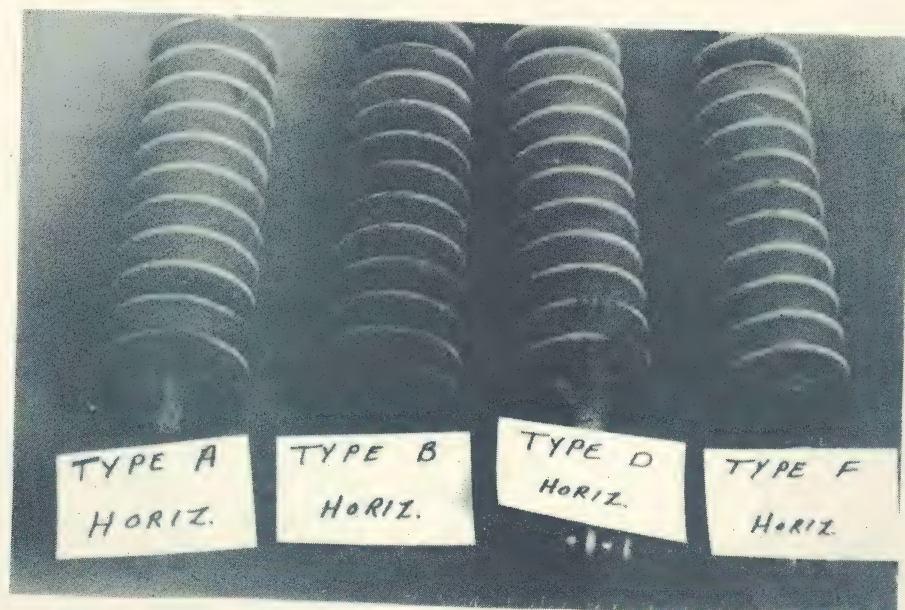
Figure 11. Four different designs of a 34 KV GEPOL insulator after tests in the salt-sugar spray test cabinet
