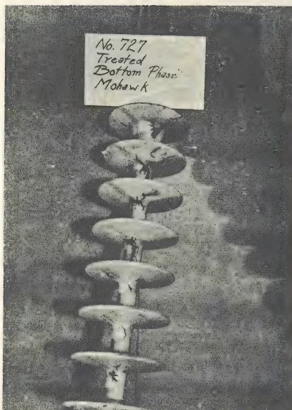
Fig. 3. Insulator returned from Niagara Mohawk Power Corp. having been in service with silicone grease coating damaged by leakage currents.
