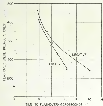
Fig. 6. Volt-time characteristic for 66-inch ECA crossarm with five suspension insulators. Data corrected to standard atmospheric conditions.
