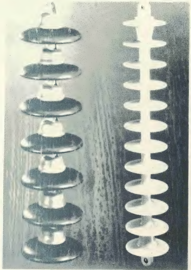
Figure 7. The 115 KV GEPOL insulator compared with its porcelain equivalent.
