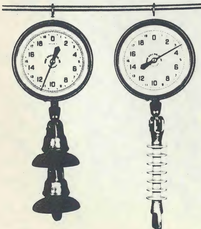
Fig. 3 - 15KV Weight Comparisons - Porcelain and Polymer
