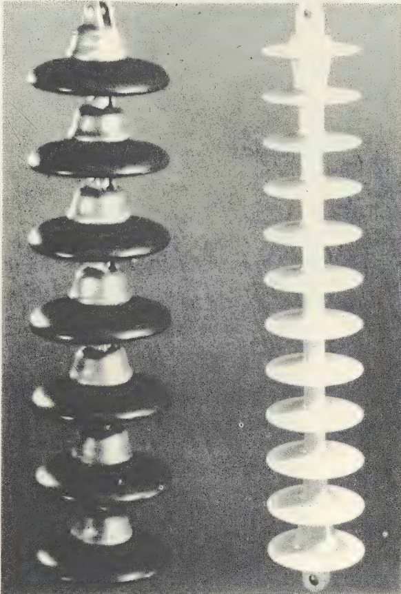
5. 115 Kv GEPOL Insulator and Equivalent Porcelain Insulators
