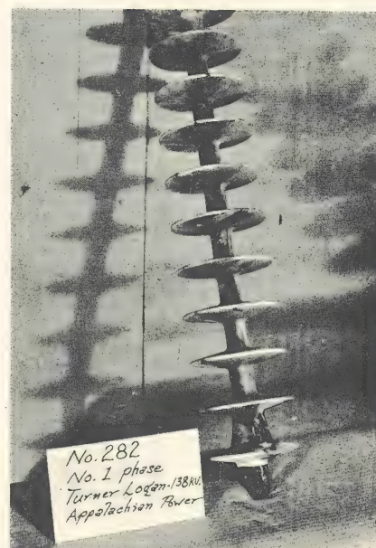
Fig. 4. Insulator returned from Appalachian Power Co. after flashover in service.
