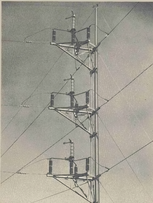
115 kv, 3-way Chance GOABS with vacuum Monoruptr on a steel Unipole
