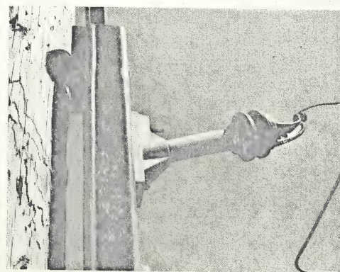
Fig. 12. ECA standoff designed for 15-kV distribution service, energized at 80 kV to ground since June 1965.
