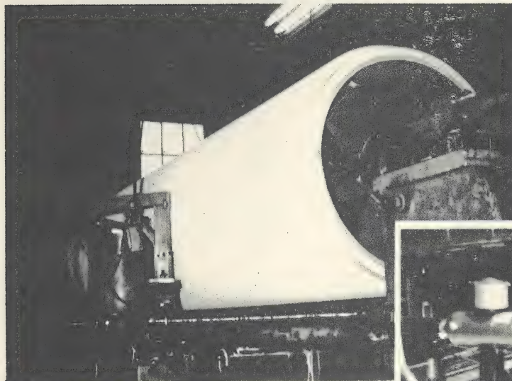
15. Machining 500 Kv Polymer Insulator
